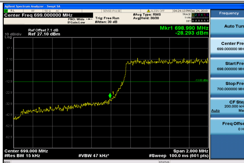
Band12-1.4MHz-QPSK-23017-6RB#0
