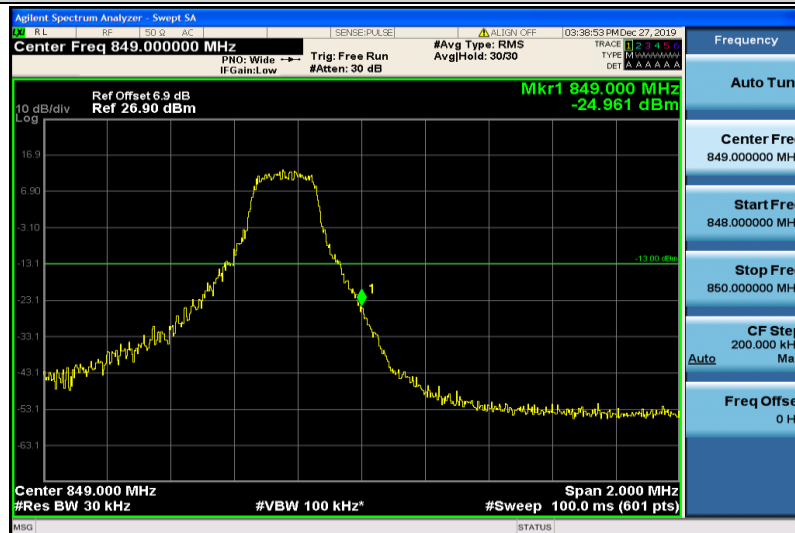
Band26-3MHz-QPSK-27025-1RB#14
