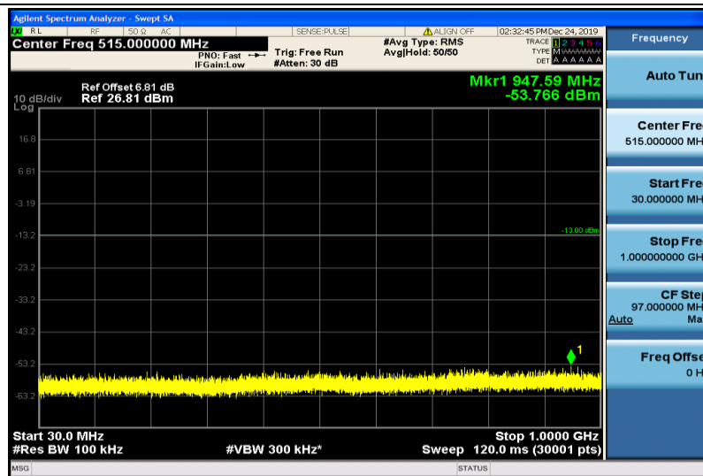
Band2-10MHz-QPSK-18650-1RB#0-30~1000MHz
