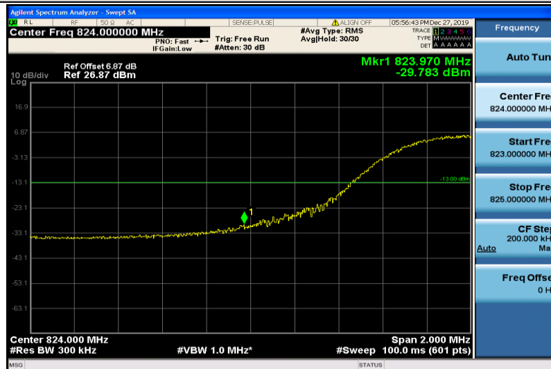
Band26-15MHz-16QAM-26865-75RB#0
