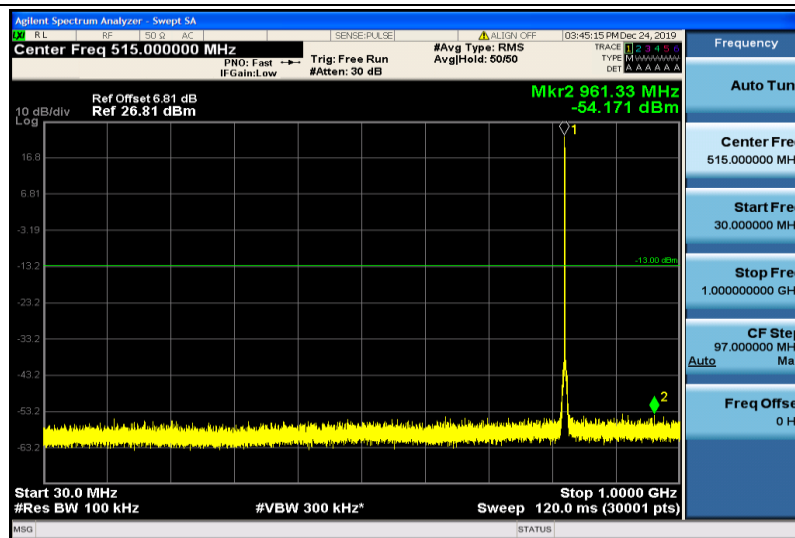
Band5-1.4MHz-16QAM-20407-1RB#0-30~1000MHz
