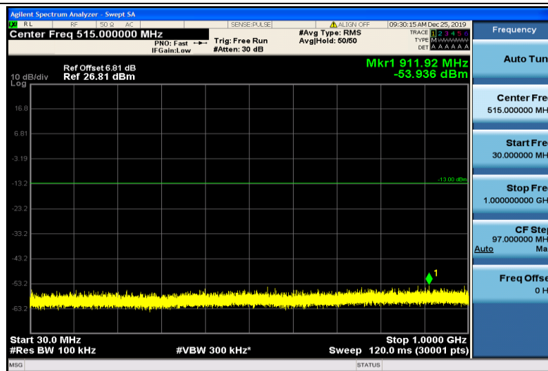
Band25-5MHz-16QAM-26065-1RB#0-30~1000MHz
