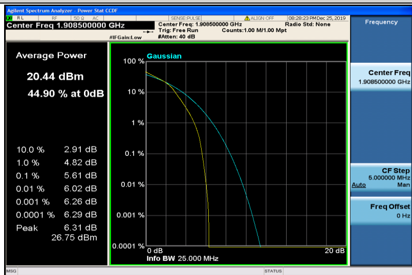
Band2-3MHz-16QAM-19185-15RB#0
