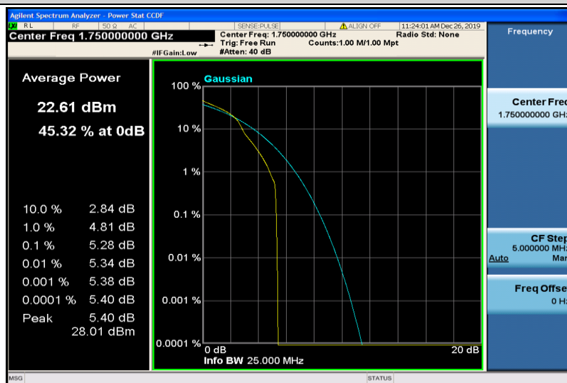
Band4-10MHz-16QAM-20350-1RB#0
