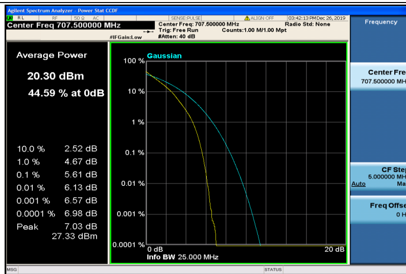
Band12-5MHz-QPSK-23095-25RB#0
