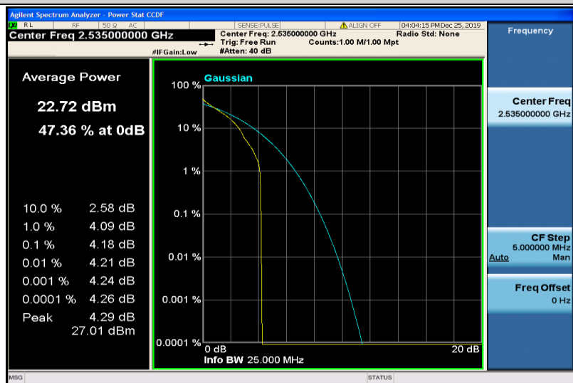
Band7-15MHz-QPSK-21100-1RB#0
