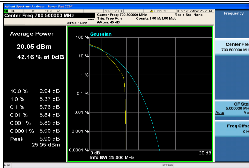
Band12-3MHz-16QAM-23025-1RB#0
