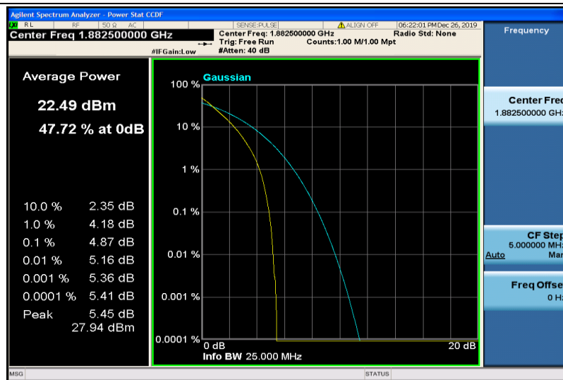
Band25-15MHz-QPSK-26365-75RB#0
