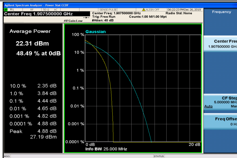
Band25-15MHz-QPSK-26615-75RB#0
