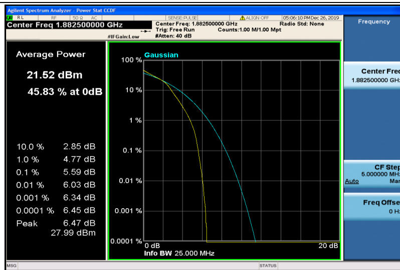
Band25-3MHz-16QAM-26365-15RB#0
