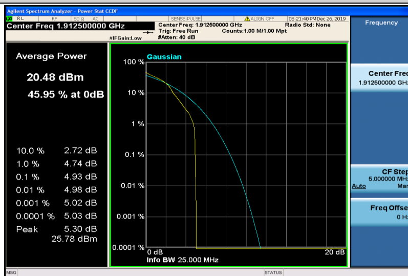
Band25-5MHz-16QAM-26665-1RB#0
