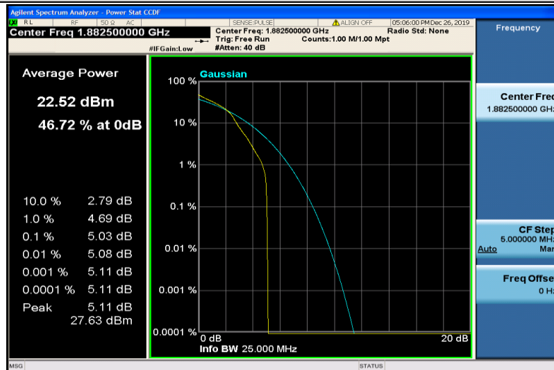
Band25-3MHz-16QAM-26365-1RB#0
