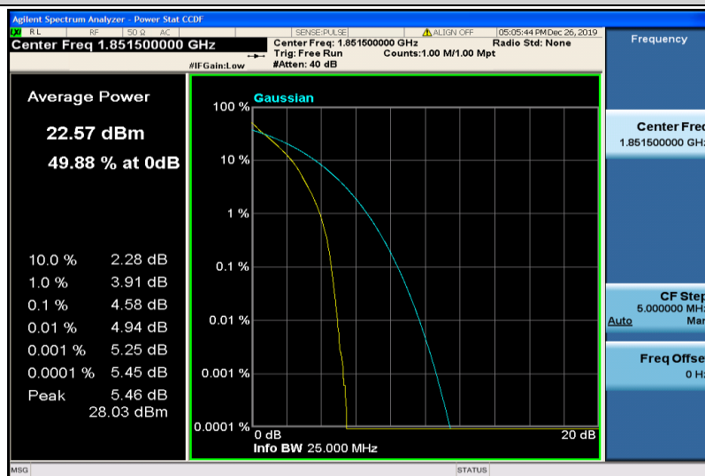
Band25-3MHz-QPSK-26055-15RB#0
