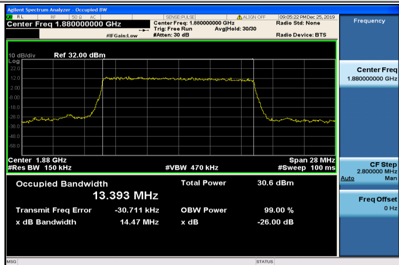
Band2-15MHz-QPSK-18900-75RB#0-13.393
