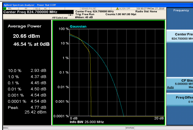
Band26-1.4MHz-16QAM-26797-1RB#0
