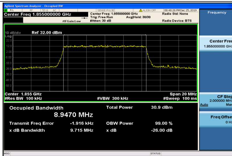
Band2-10MHz-QPSK-18650-50RB#0-8.9470
