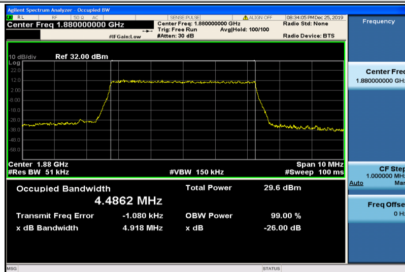
Band2-5MHz-16QAM-18900-25RB#0-4.4862
