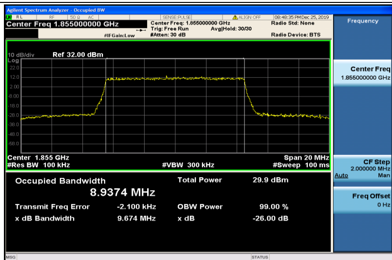
Band2-10MHz-16QAM-18650-50RB#0-8.9374
