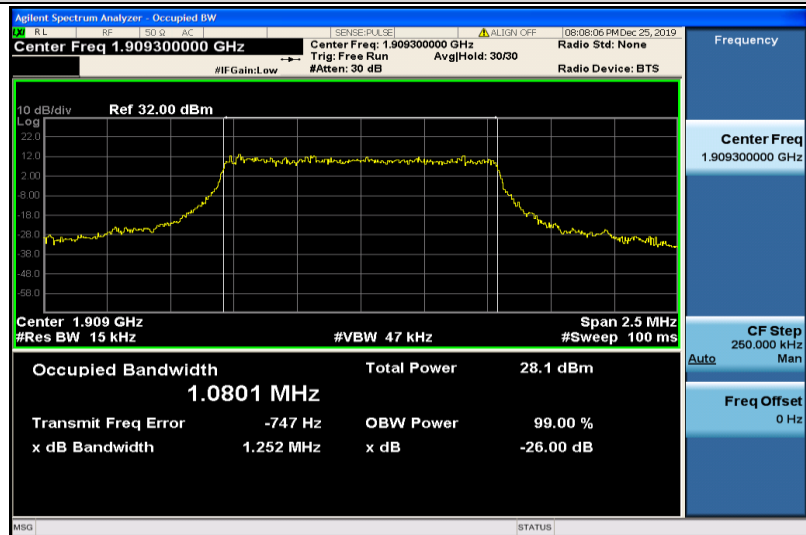
Band2-1.4MHz-16QAM-19193-6RB#0-1.0801
