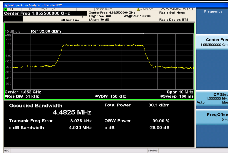
Band2-5MHz-16QAM-18625-25RB#0-4.4825
