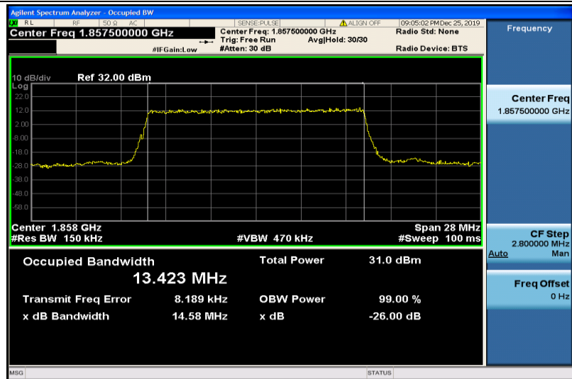
Band2-15MHz-QPSK-18675-75RB#0-13.423
