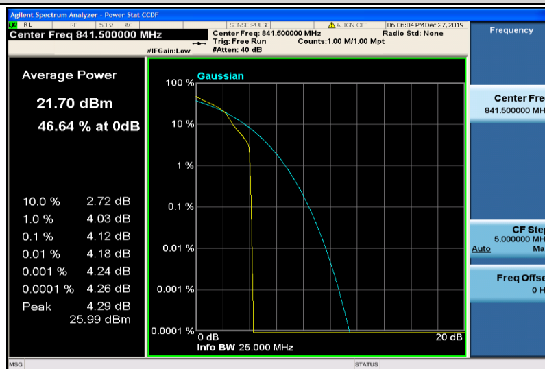
Band26-15MHz-16QAM-26965-1RB#0
