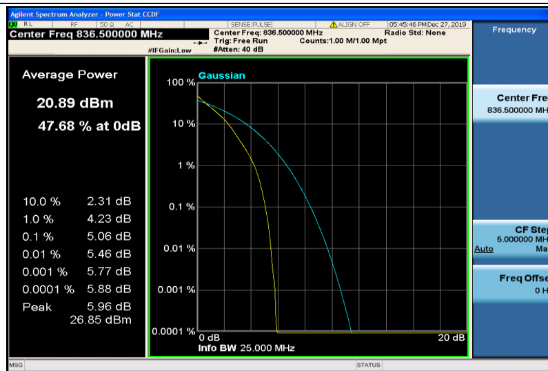
Band26-5MHz-QPSK-26915-25RB#0
