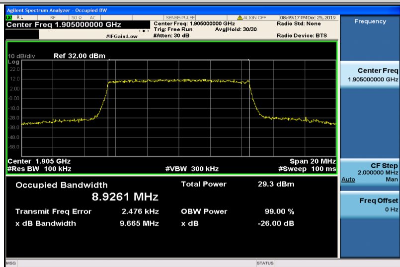
Band2-10MHz-16QAM-19150-50RB#0-8.9261
