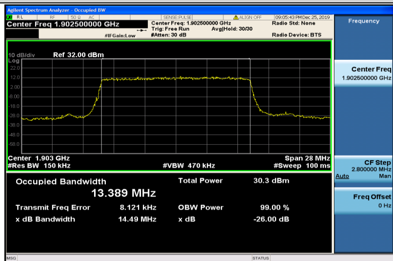
Band2-15MHz-QPSK-19125-75RB#0-13.389
