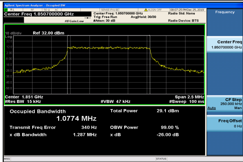
Band2-1.4MHz-16QAM-18607-6RB#0-1.0774
