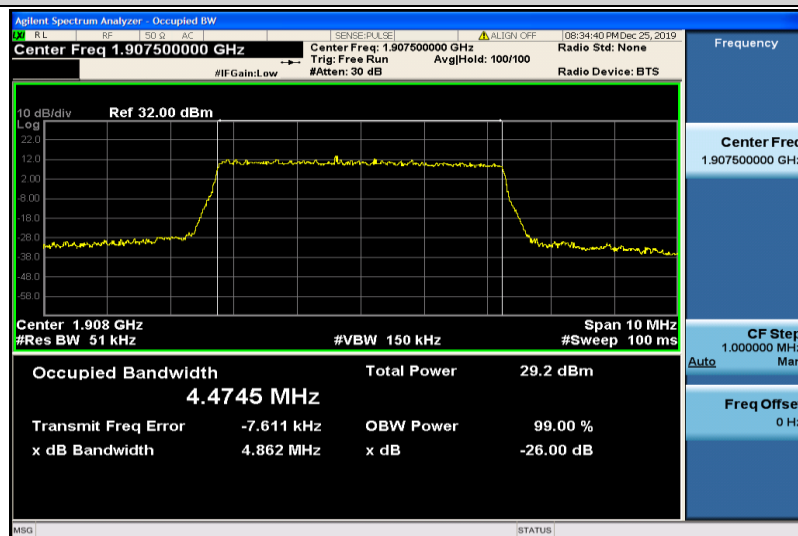
Band2-5MHz-16QAM-19175-25RB#0-4.4745
