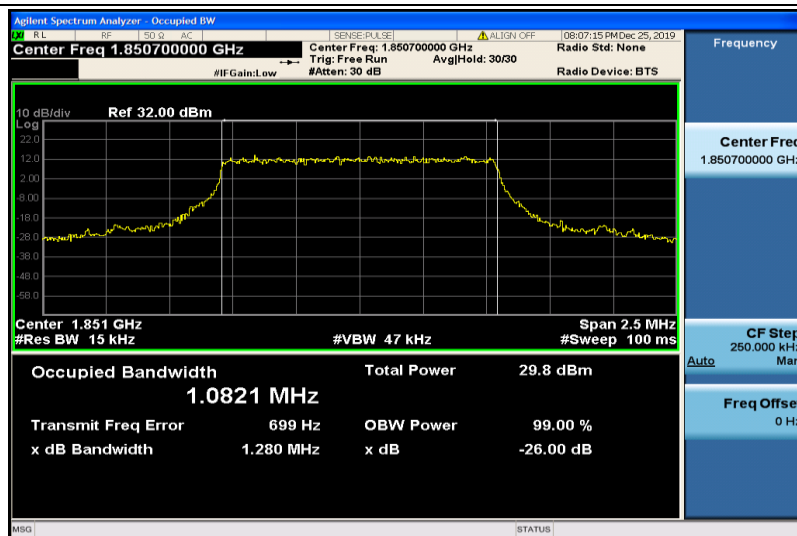
Band2-1.4MHz-QPSK-18607-6RB#0-1.0821
