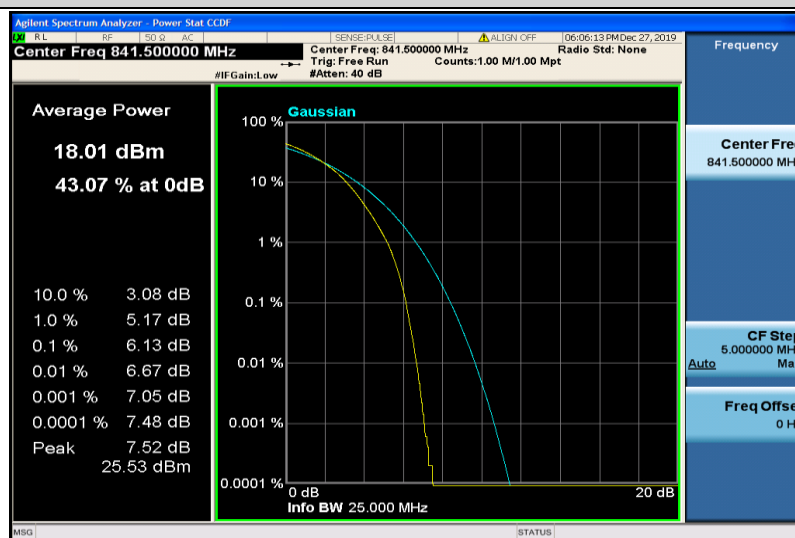
Band26-15MHz-16QAM-26965-75RB#0
