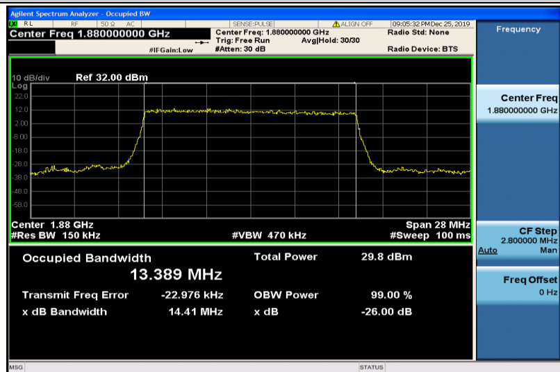
Band2-15MHz-16QAM-18900-75RB#0-13.389
