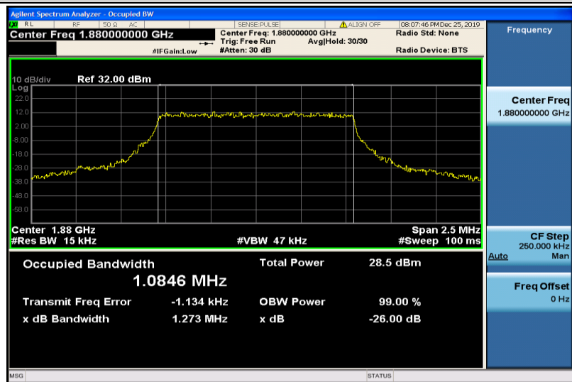
Band2-1.4MHz-16QAM-18900-6RB#0-1.0846
