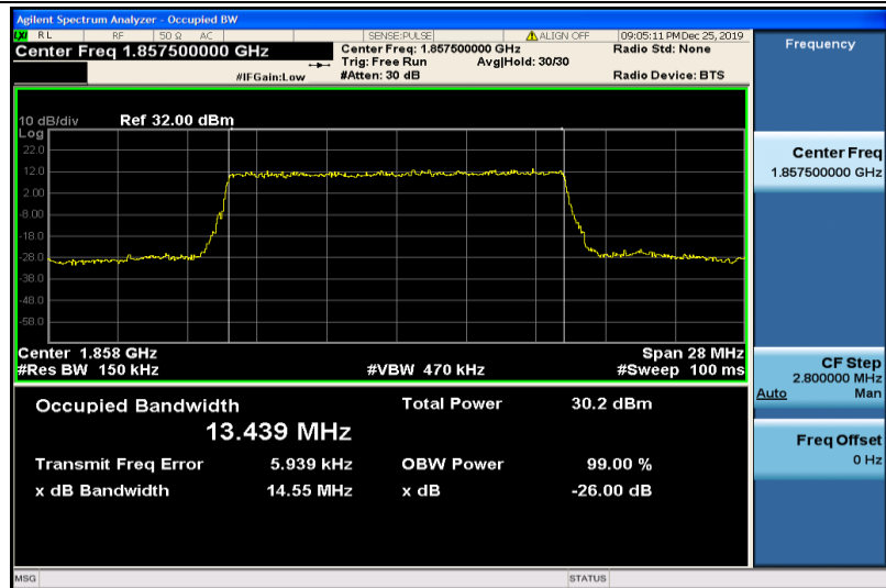
Band2-15MHz-16QAM-18675-75RB#0-13.439
