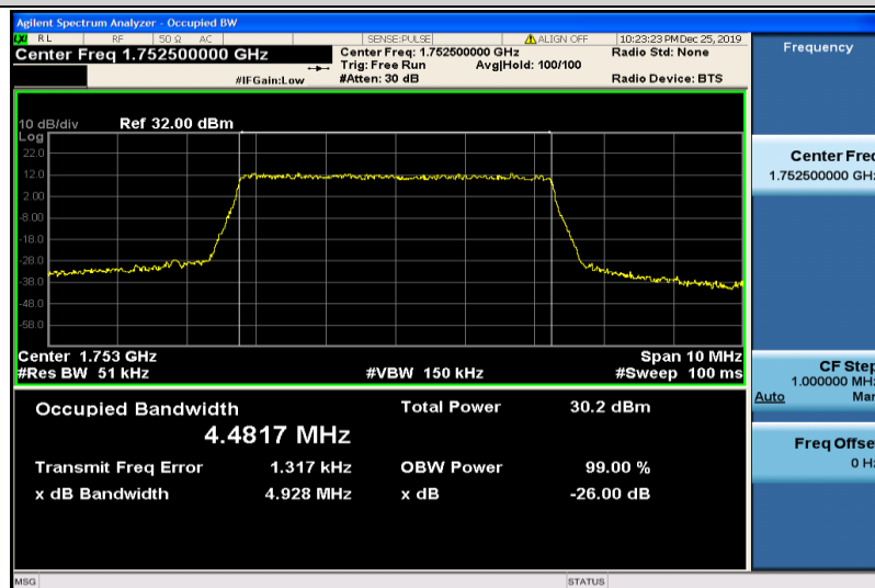
Band4-5MHz-16QAM-20375-25RB#0-4.4817
