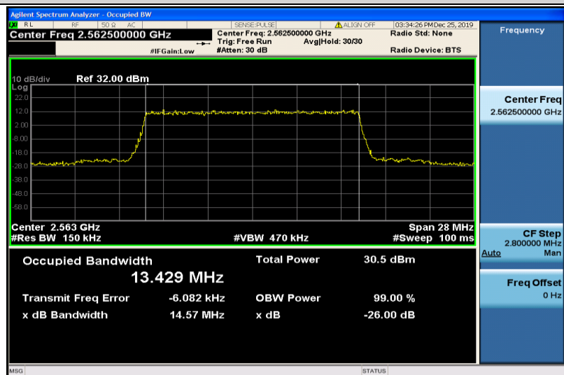
Band7-15MHz-QPSK-21375-75RB#0-13.429
