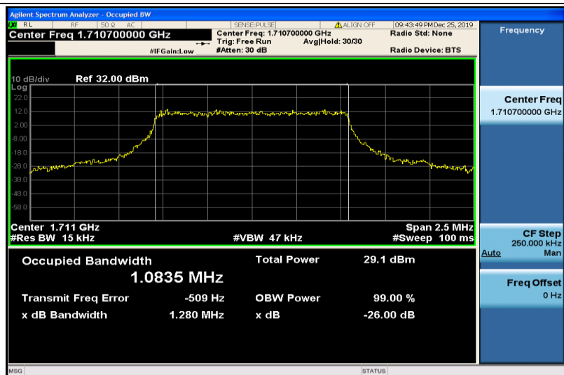
Band4-1.4MHz-16QAM-19957-6RB#0-1.0835
