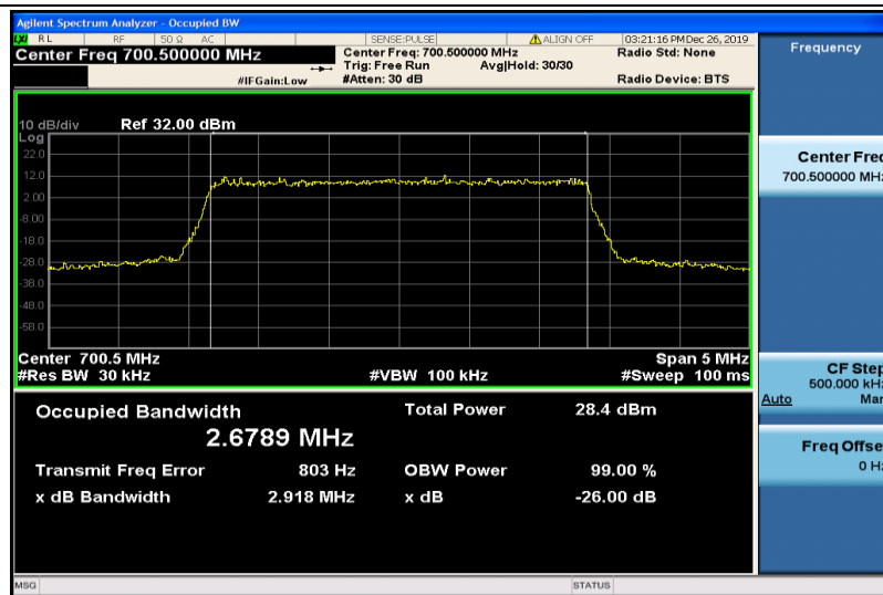
Band12-3MHz-QPSK-23025-15RB#0-2.6789
