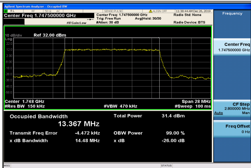
Band4-15MHz-QPSK-20325-75RB#0-13.367
