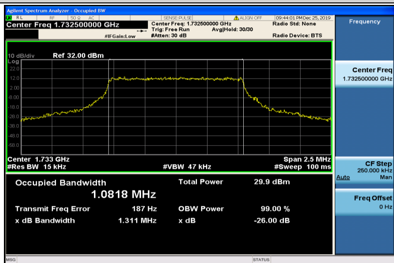
Band4-1.4MHz-QPSK-20175-6RB#0-1.0818
