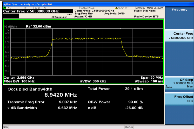
Band7-10MHz-16QAM-21400-50RB#0-8.9420
