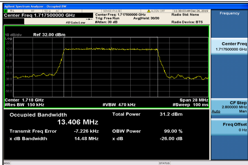
Band4-15MHz-QPSK-20025-75RB#0-13.406
