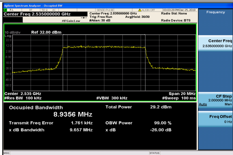
Band7-10MHz-16QAM-21100-50RB#0-8.9356
