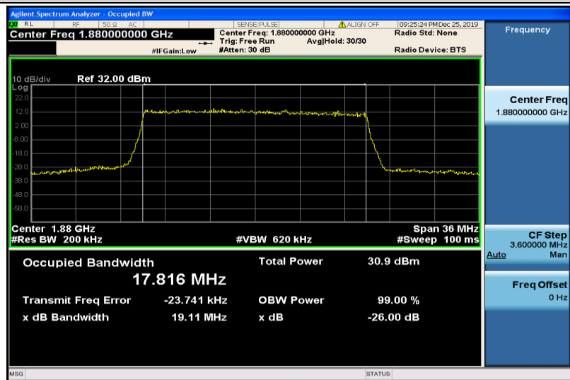
Band2-20MHz-QPSK-18900-100RB#0-17.816
