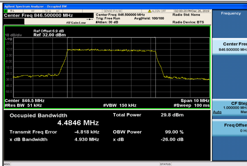
Band5-5MHz-QPSK-20625-25RB#0-4.4846
