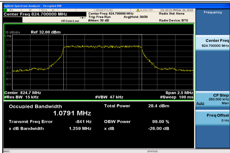
Band5-1.4MHz-QPSK-20407-6RB#0-1.0791
