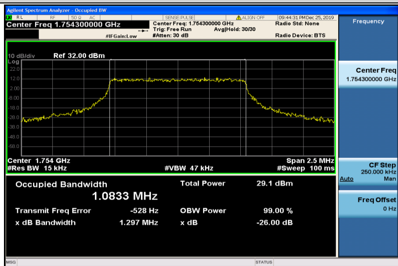
Band4-1.4MHz-16QAM-20393-6RB#0-1.0833
