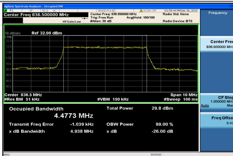
Band5-5MHz-QPSK-20525-25RB#0-4.4773
