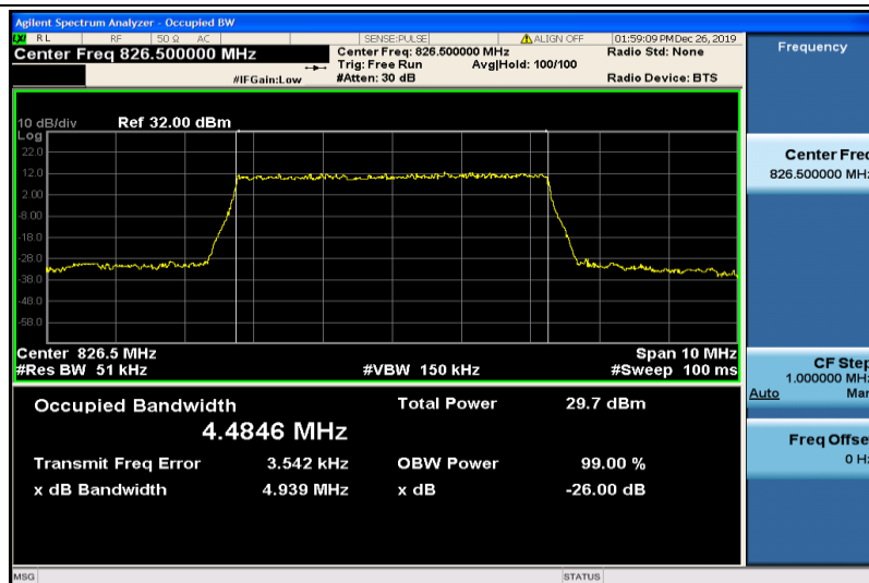
Band5-5MHz-QPSK-20425-25RB#0-4.4846
