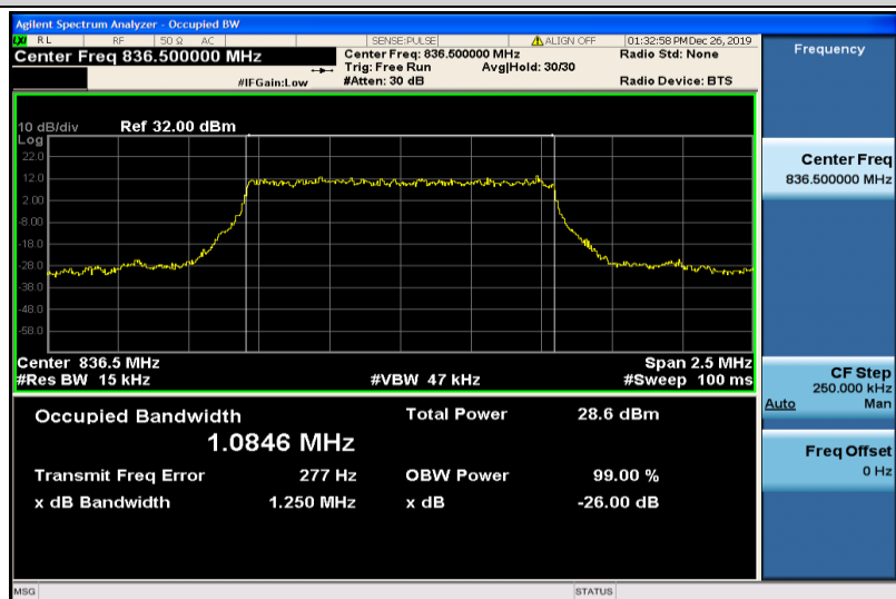
Band5-1.4MHz-QPSK-20525-6RB#0-1.0846
