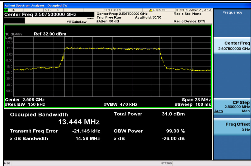
Band7-15MHz-QPSK-20825-75RB#0-13.444
