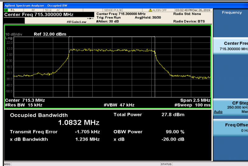
Band12-1.4MHz-QPSK-23173-6RB#0-1.0832
