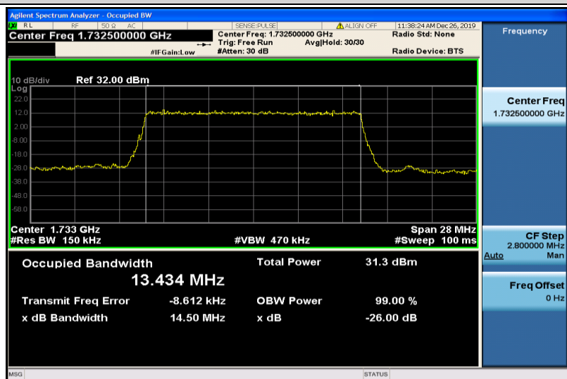
Band4-15MHz-QPSK-20175-75RB#0-13.434
