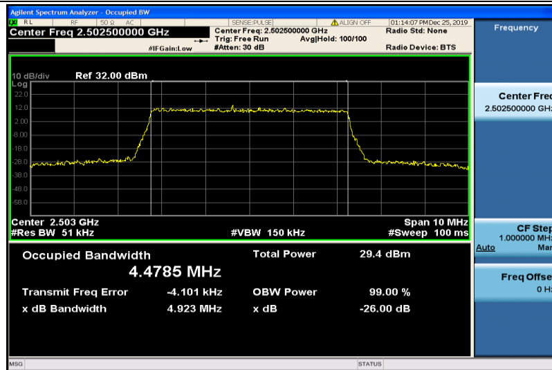
Band7-5MHz-16QAM-20775-25RB#0-4.4785
