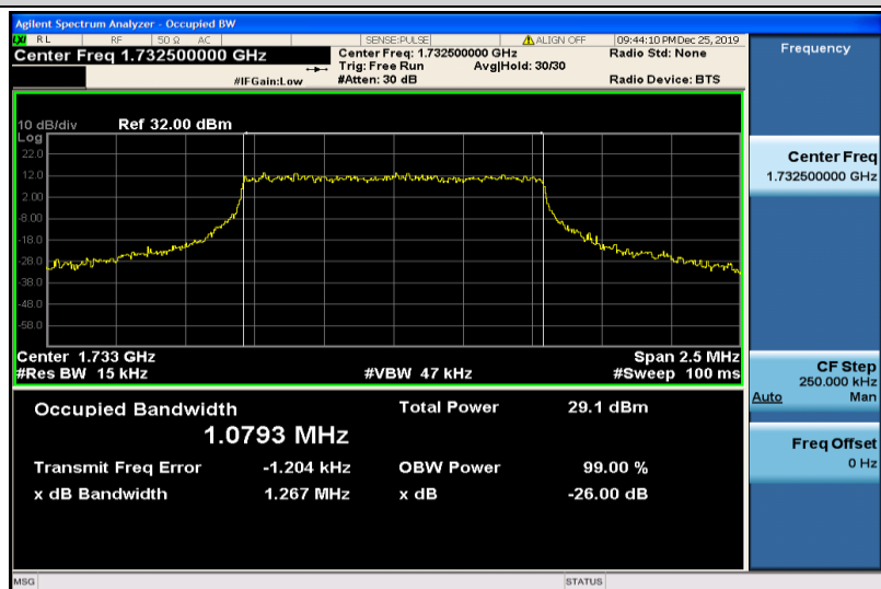
Band4-1.4MHz-16QAM-20175-6RB#0-1.0793
