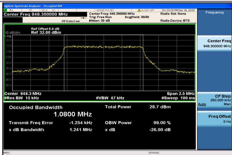
Band5-1.4MHz-QPSK-20643-6RB#0-1.0800
