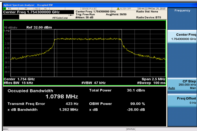
Band4-1.4MHz-QPSK-20393-6RB#0-1.0798
