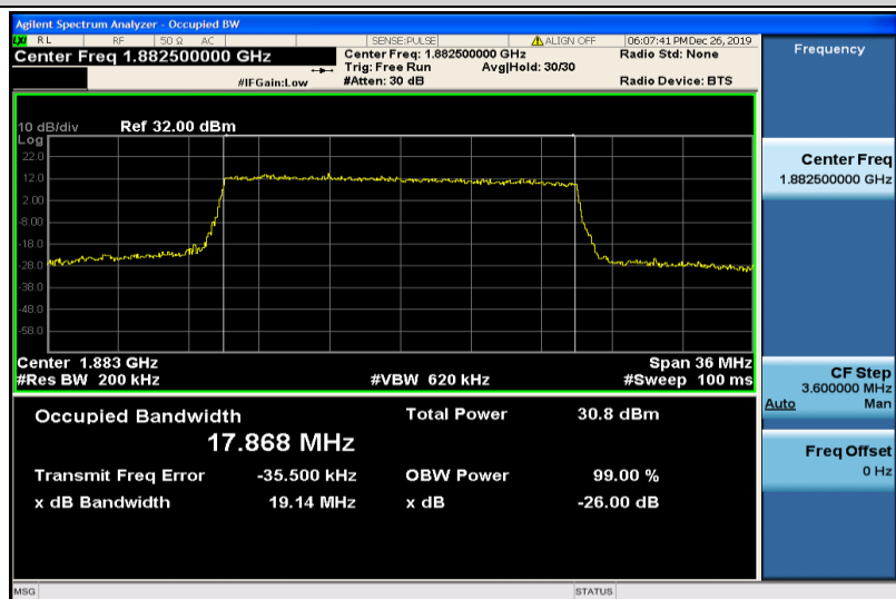
Band25-20MHz-16QAM-26365-100RB#0-17.868
