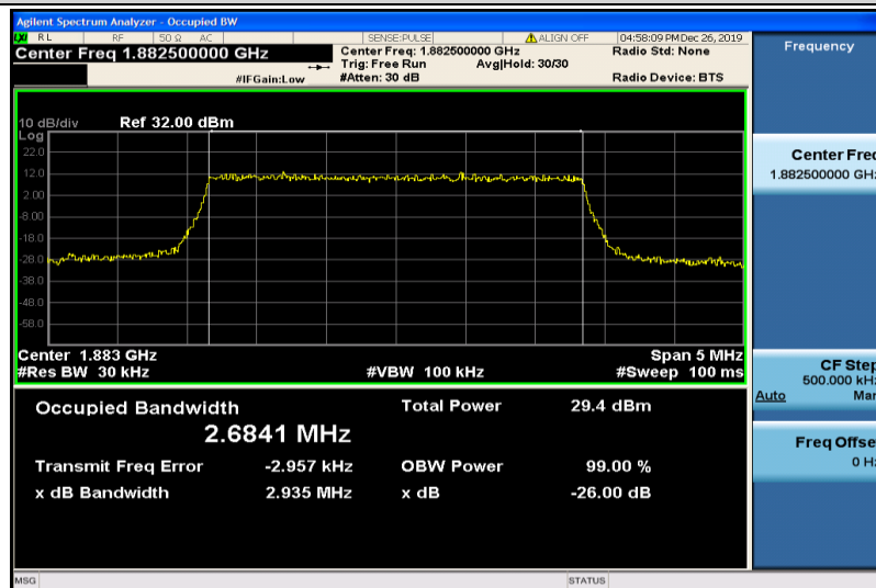
Band25-3MHz-16QAM-26365-15RB#0-2.6841
