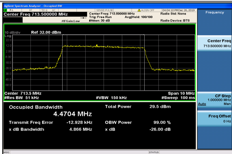
Band17-5MHz-16QAM-23825-25RB#0-4.4704
