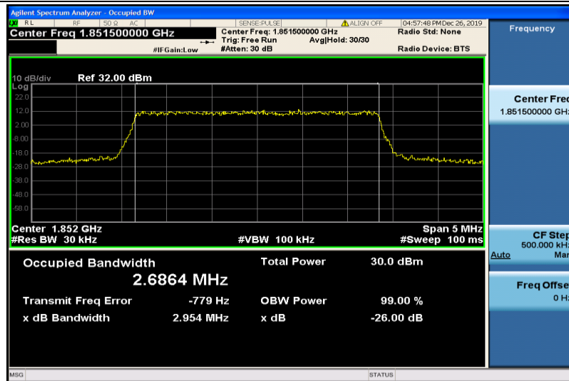
Band25-3MHz-16QAM-26055-15RB#0-2.6864
