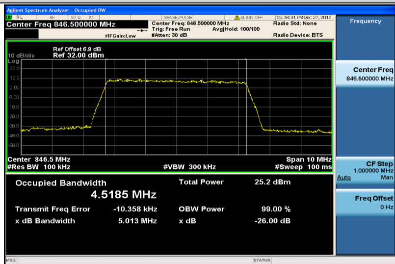
Band26-5MHz-QPSK-27015-25RB#0-4.5185
