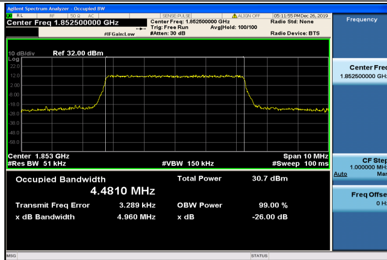
Band25-5MHz-16QAM-26065-25RB#0-4.4810
