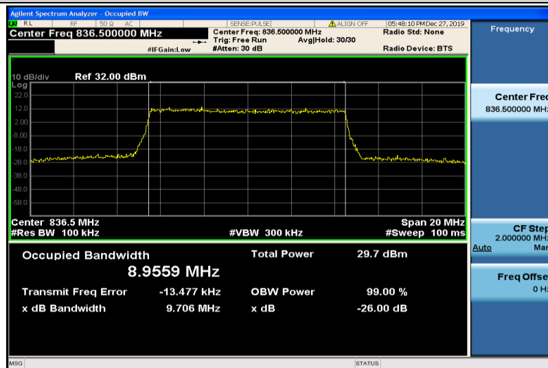
Band26-10MHz-QPSK-26915-50RB#0-8.9559
