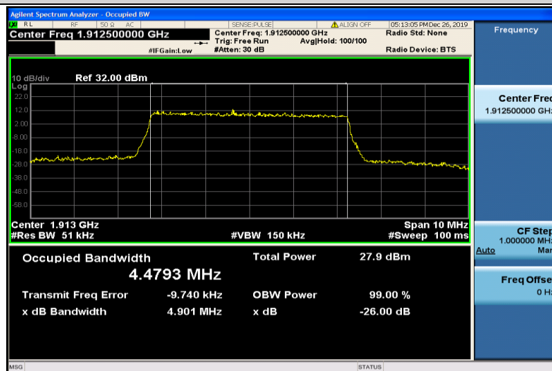
Band25-5MHz-16QAM-26665-25RB#0-4.4793
