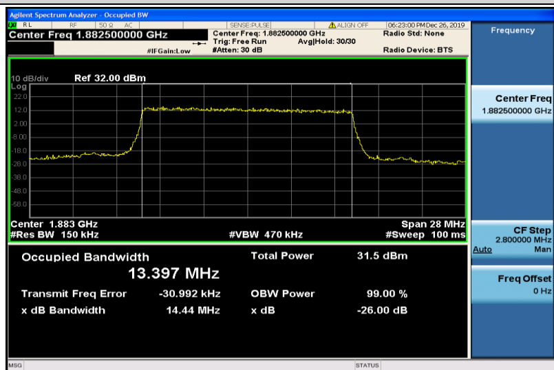
Band25-15MHz-QPSK-26365-75RB#0-13.397
