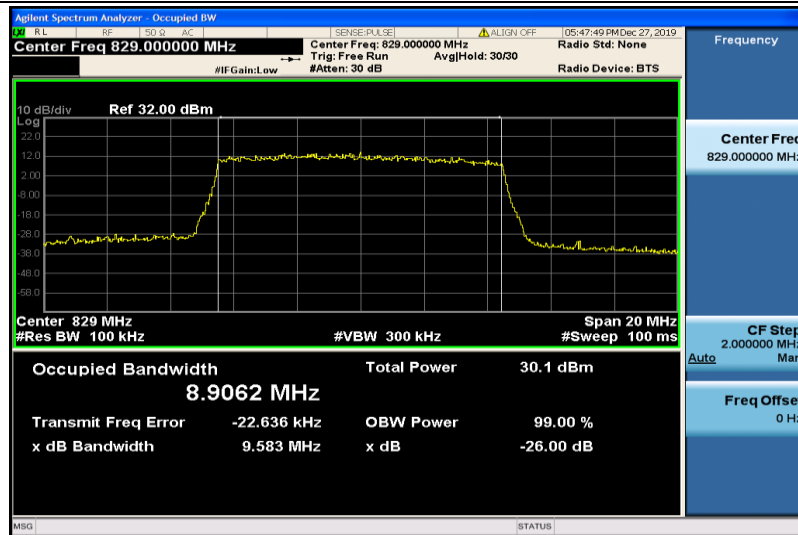
Band26-10MHz-QPSK-26840-50RB#0-8.9062
