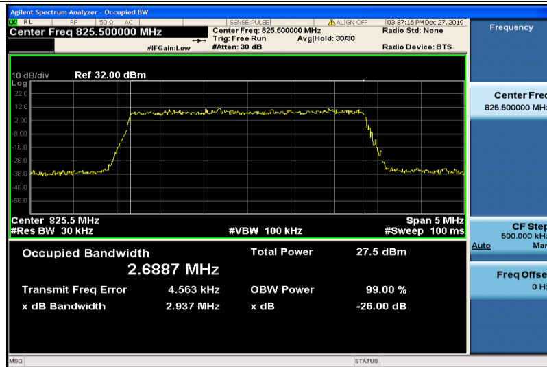
Band26-3MHz-16QAM-26805-15RB#0-2.6887
