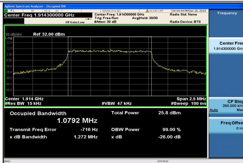
Band25-1.4MHz-16QAM-26683-6RB#0-1.0792
