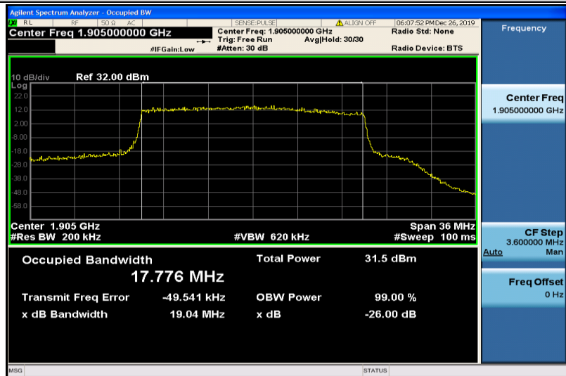
Band25-20MHz-QPSK-26590-100RB#0-17.776
