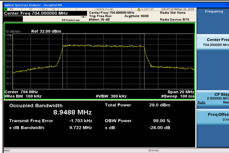
Band12-10MHz-QPSK-23060-50RB#0-8.9488
