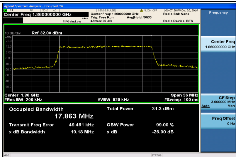
Band25-20MHz-16QAM-26140-100RB#0-17.863
