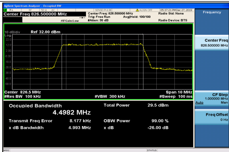
Band26-5MHz-QPSK-26815-25RB#0-4.4982
