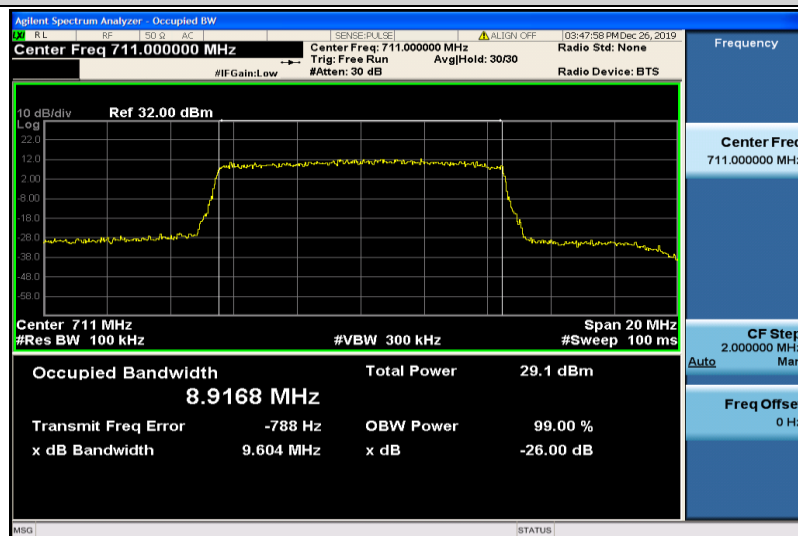
Band12-10MHz-QPSK-23130-50RB#0-8.9168
