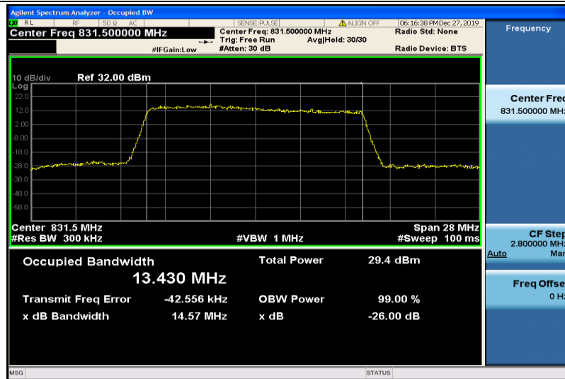
Band26-15MHz-16QAM-26865-75RB#0-13.430
