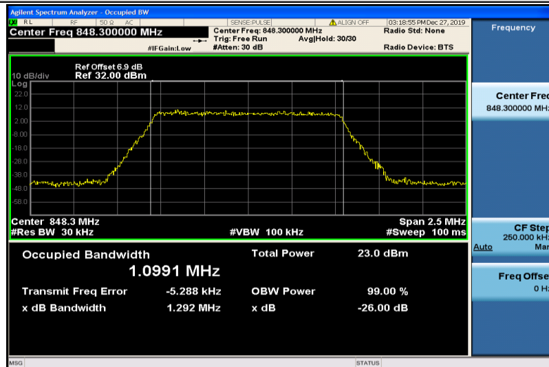
Band26-1.4MHz-16QAM-27033-6RB#0-1.0991
