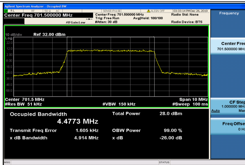
Band12-5MHz-16QAM-23035-25RB#0-4.4773
