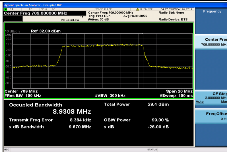
Band17-10MHz-16QAM-23780-50RB#0-8.9308
