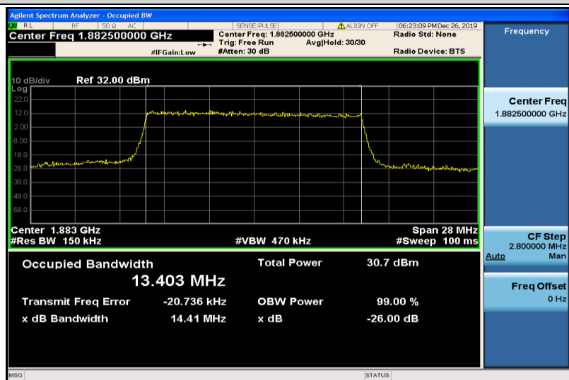
Band25-15MHz-16QAM-26365-75RB#0-13.403
