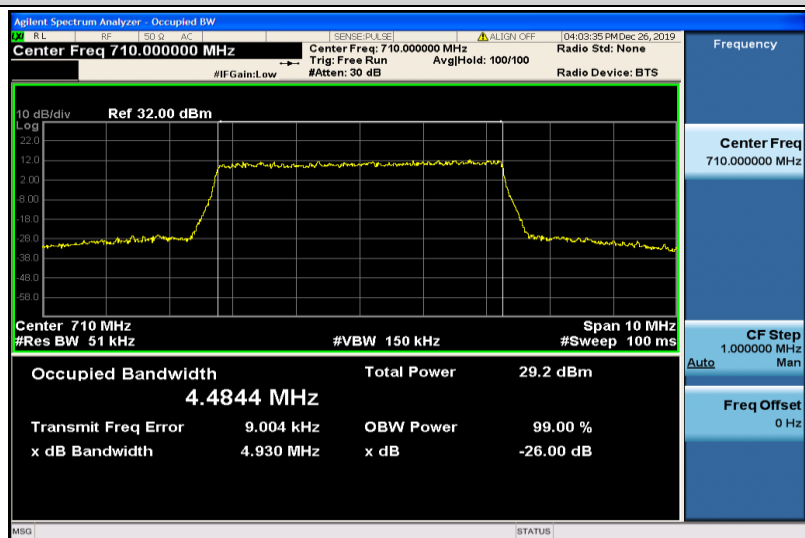
Band17-5MHz-16QAM-23790-25RB#0-4.4844
