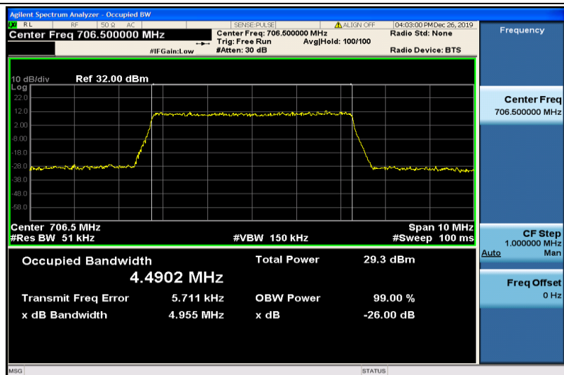
Band17-5MHz-16QAM-23755-25RB#0-4.4902
