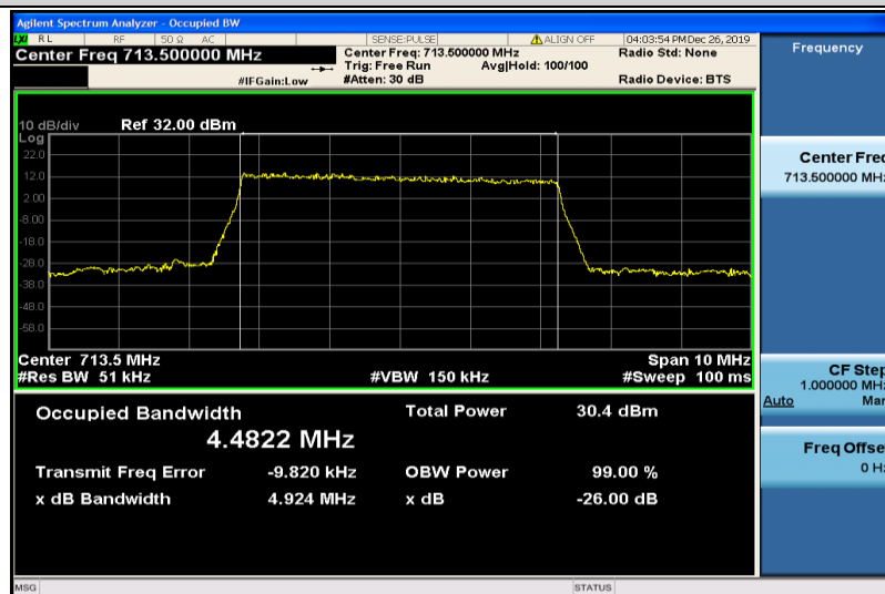
Band17-5MHz-QPSK-23825-25RB#0-4.4822
