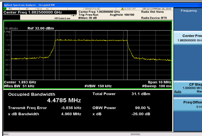
Band25-5MHz-QPSK-26365-25RB#0-4.4785
