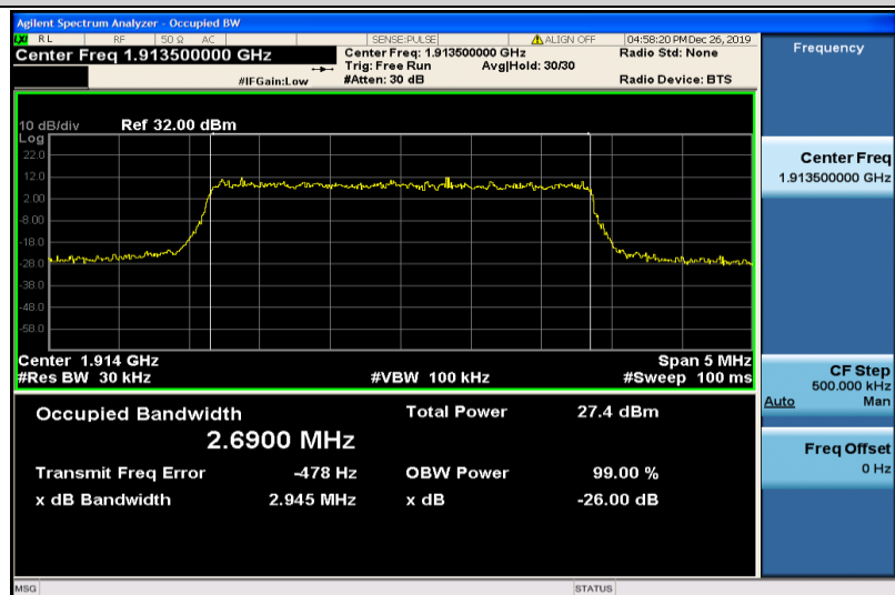
Band25-3MHz-QPSK-26675-15RB#0-2.6900
