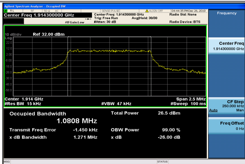
Band25-1.4MHz-QPSK-26683-6RB#0-1.0808
