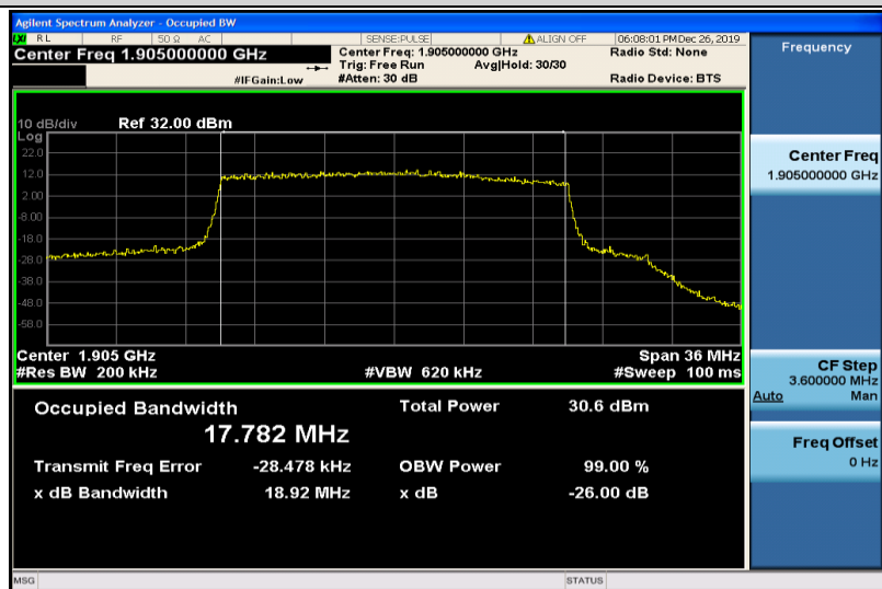
Band25-20MHz-16QAM-26590-100RB#0-17.782
