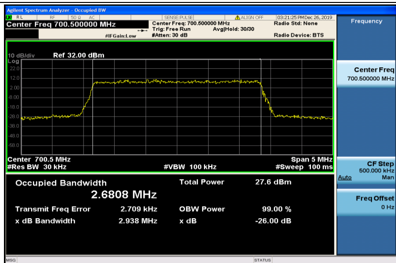
Band12-3MHz-16QAM-23025-15RB#0-2.6808
