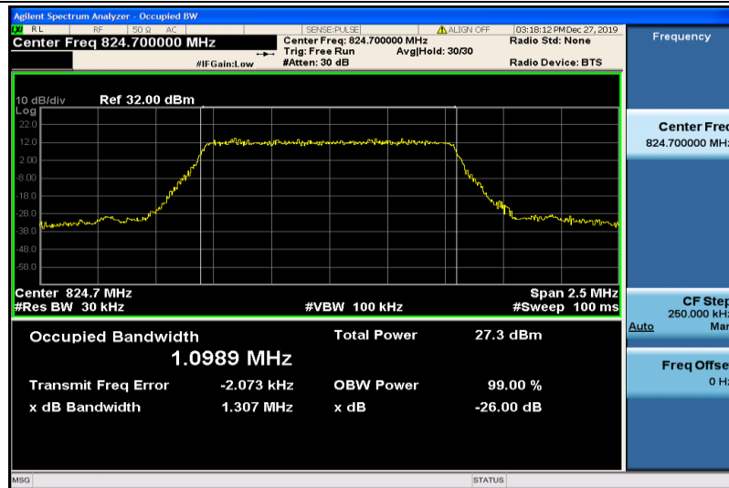
Band26-1.4MHz-16QAM-26797-6RB#0-1.0989
