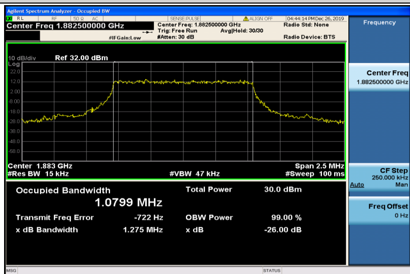
Band25-1.4MHz-QPSK-26365-6RB#0-1.0799
