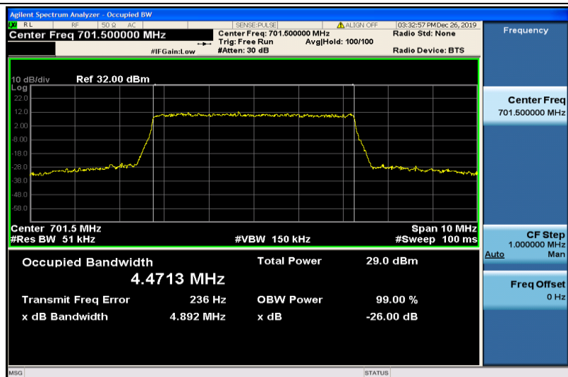
Band12-5MHz-QPSK-23035-25RB#0-4.4713
