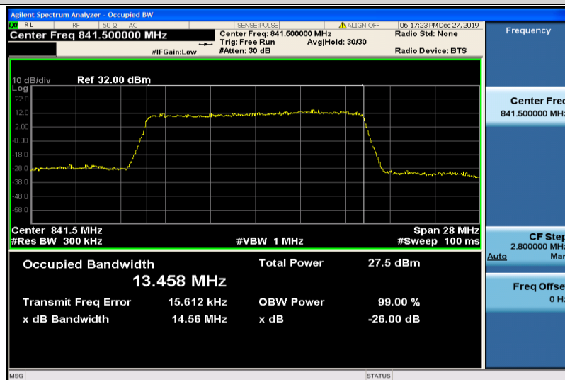
Band26-15MHz-16QAM-26965-75RB#0-13.458
