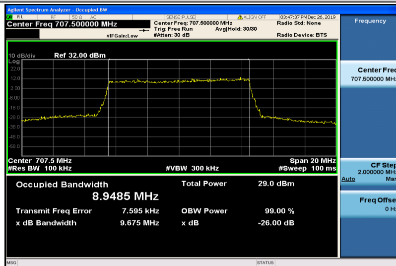
Band12-10MHz-QPSK-23095-50RB#0-8.9485
