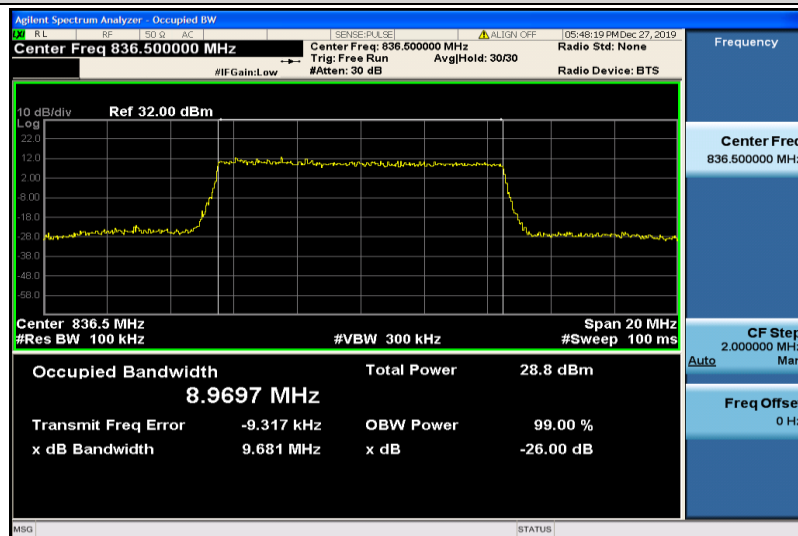
Band26-10MHz-16QAM-26915-50RB#0-8.9697
