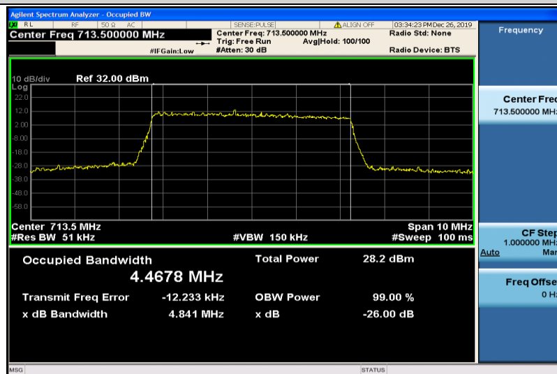
Band12-5MHz-16QAM-23155-25RB#0-4.4678
