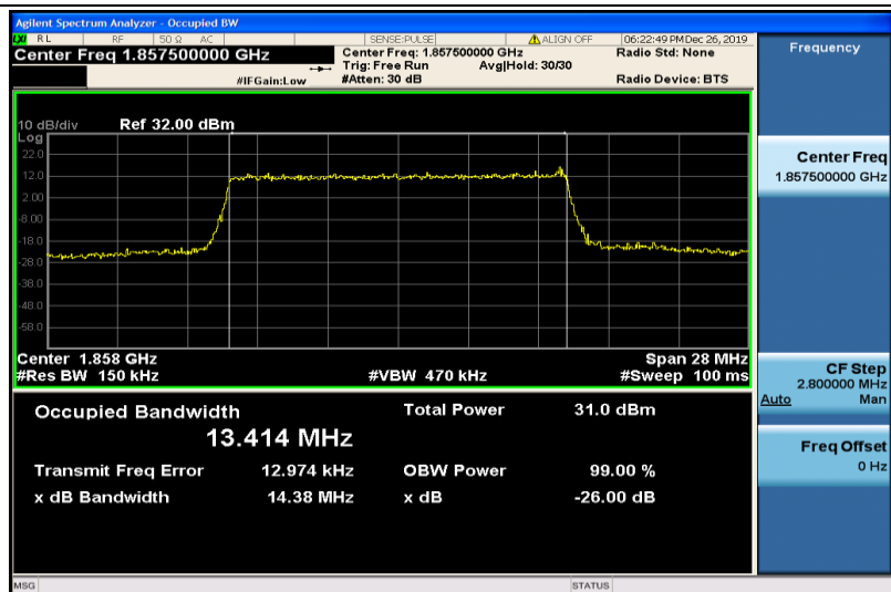
Band25-15MHz-16QAM-26115-75RB#0-13.414
