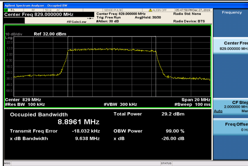
Band26-10MHz-16QAM-26840-50RB#0-8.8961
