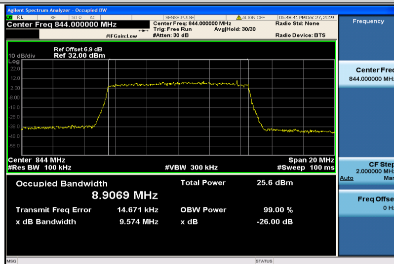
Band26-10MHz-16QAM-26990-50RB#0-8.9069
