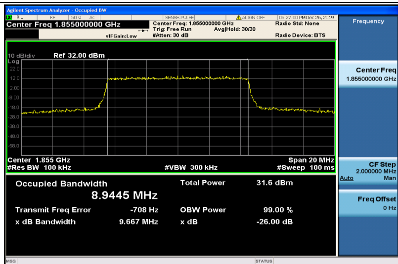
Band25-10MHz-QPSK-26090-50RB#0-8.9445
