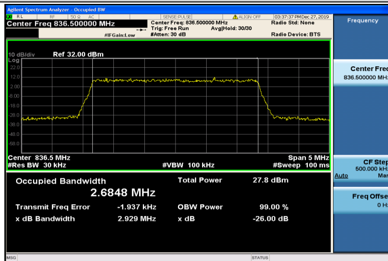
Band26-3MHz-16QAM-26915-15RB#0-2.6848
