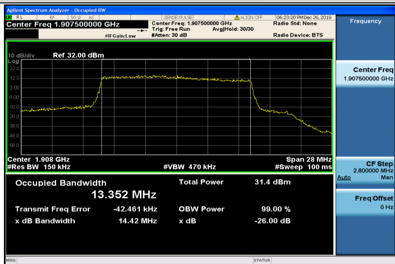
Band25-15MHz-QPSK-26615-75RB#0-13.352
