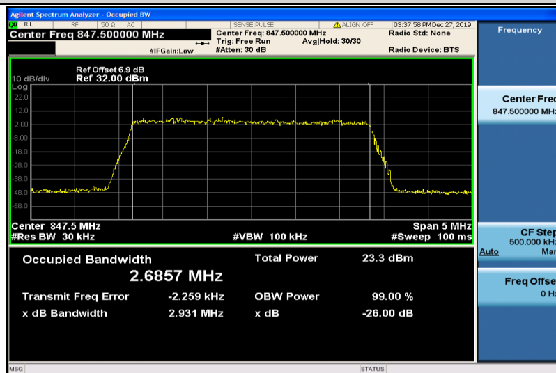
Band26-3MHz-16QAM-27025-15RB#0-2.6857
