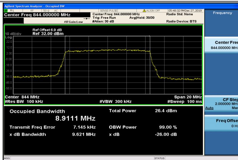
Band26-10MHz-QPSK-26990-50RB#0-8.9111
