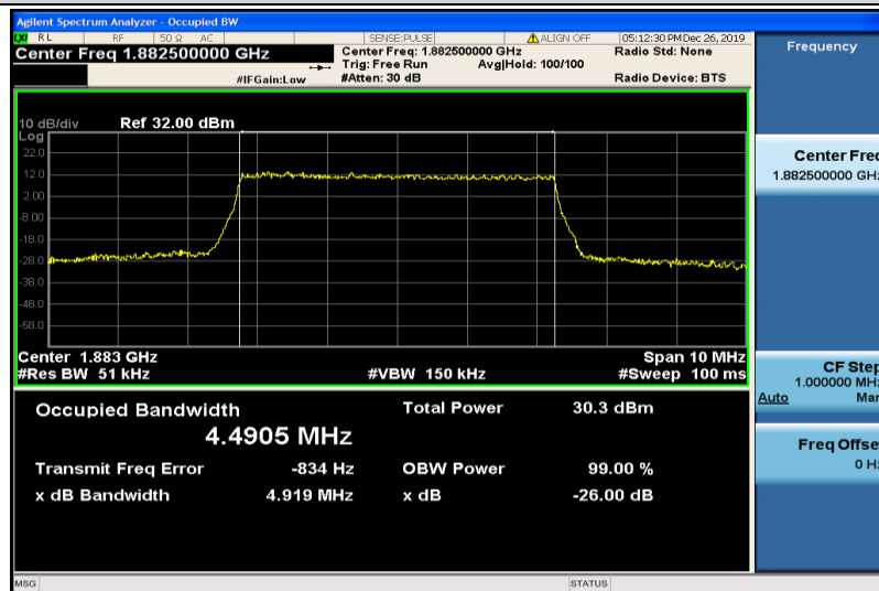
Band25-5MHz-16QAM-26365-25RB#0-4.4905
