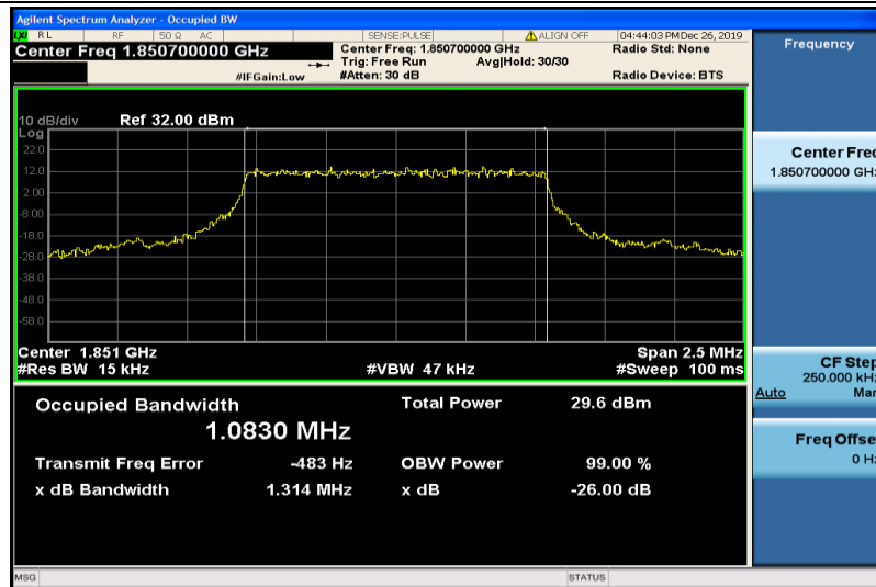
Band25-1.4MHz-16QAM-26047-6RB#0-1.0830
