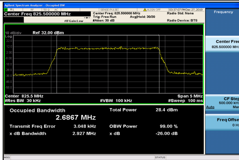
Band26-3MHz-QPSK-26805-15RB#0-2.6867
