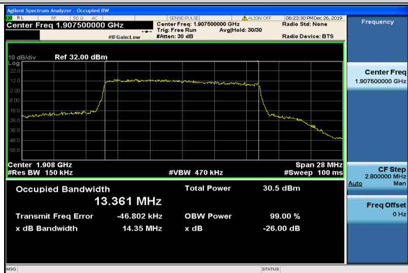
Band25-15MHz-16QAM-26615-75RB#0-13.361
