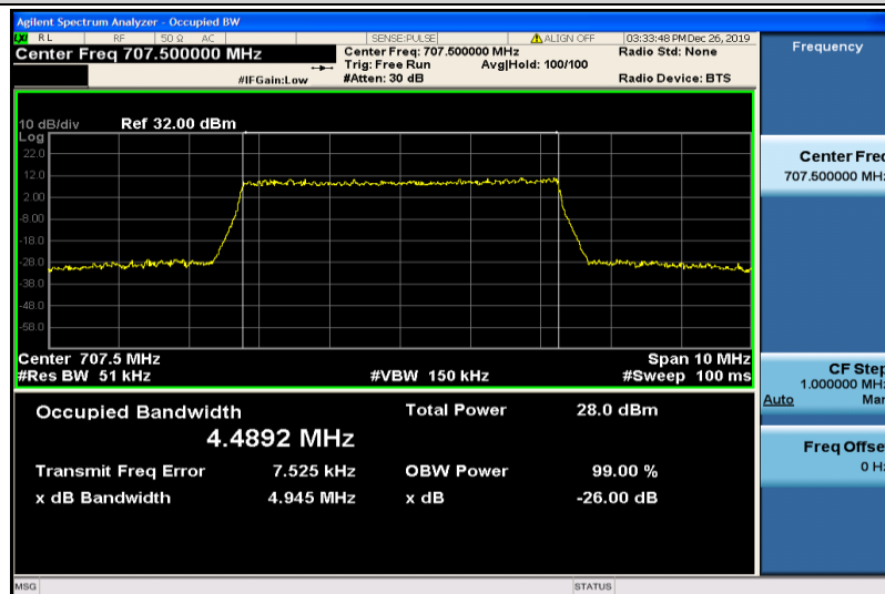
Band12-5MHz-16QAM-23095-25RB#0-4.4892
