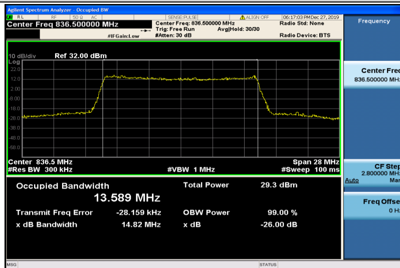
Band26-15MHz-16QAM-26915-75RB#0-13.589
