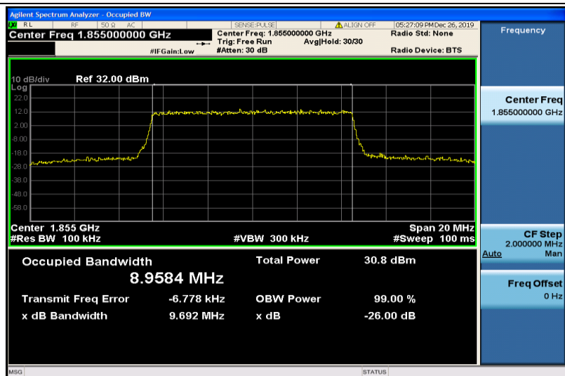
Band25-10MHz-16QAM-26090-50RB#0-8.9584
