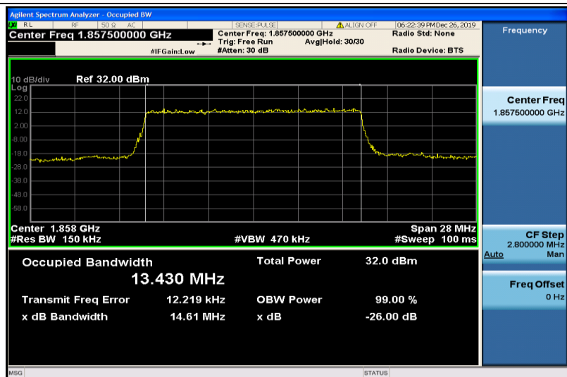
Band25-15MHz-QPSK-26115-75RB#0-13.430
