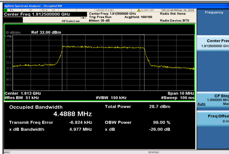
Band25-5MHz-QPSK-26665-25RB#0-4.4888
