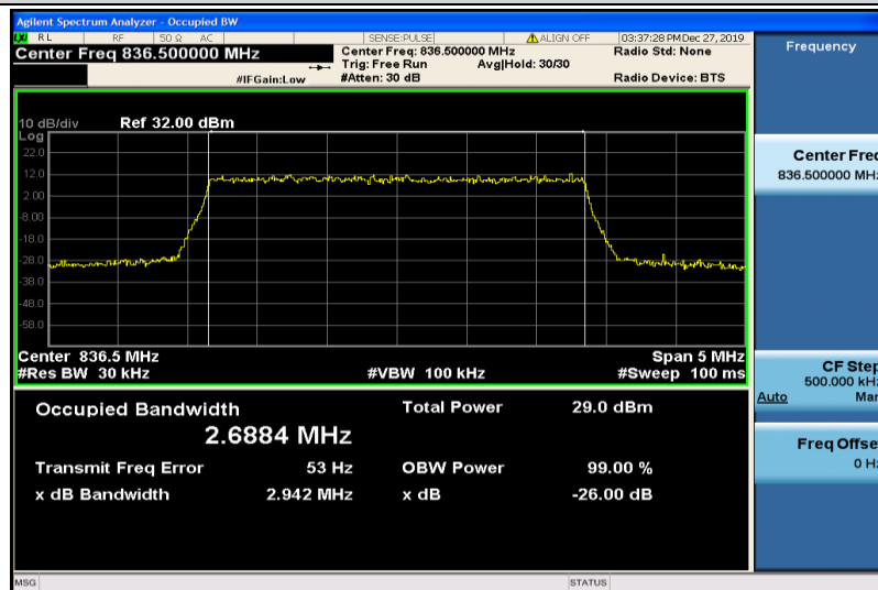
Band26-3MHz-QPSK-26915-15RB#0-2.6884
