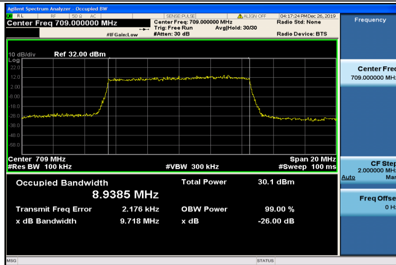
Band17-10MHz-QPSK-23780-50RB#0-8.9385
