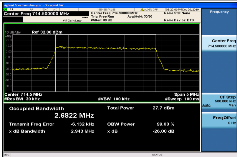
Band12-3MHz-16QAM-23165-15RB#0-2.6822
