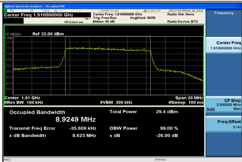
Band25-10MHz-16QAM-26640-50RB#0-8.9249
