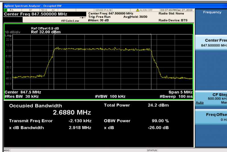
Band26-3MHz-QPSK-27025-15RB#0-2.6880
