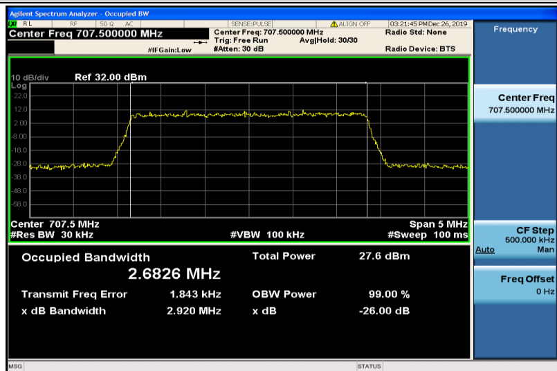
Band12-3MHz-16QAM-23095-15RB#0-2.6826
