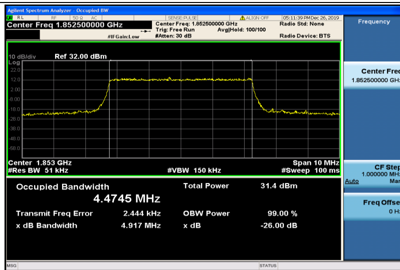
Band25-5MHz-QPSK-26065-25RB#0-4.4745
