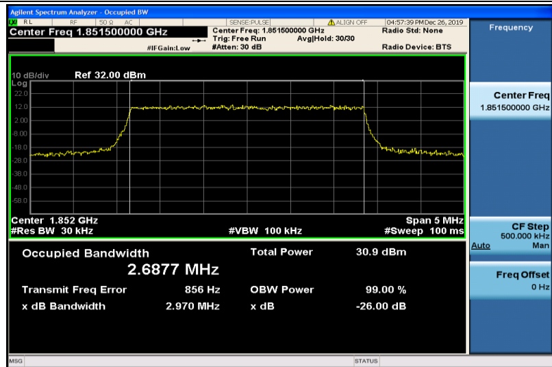
Band25-3MHz-QPSK-26055-15RB#0-2.6877
