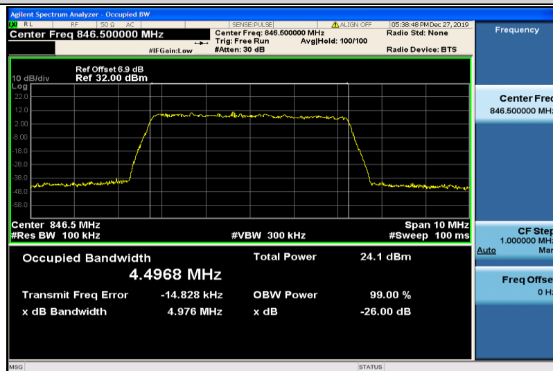
Band26-5MHz-16QAM-27015-25RB#0-4.4968
