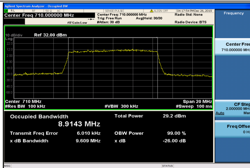
Band17-10MHz-16QAM-23790-50RB#0-8.9143
