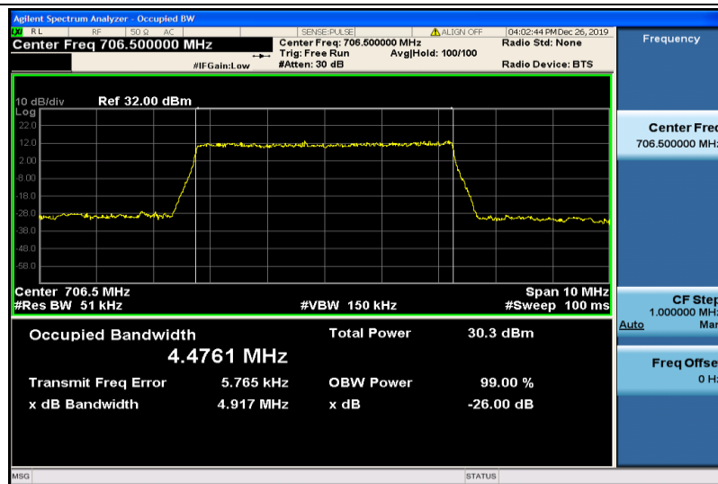
Band17-5MHz-QPSK-23755-25RB#0-4.4761
