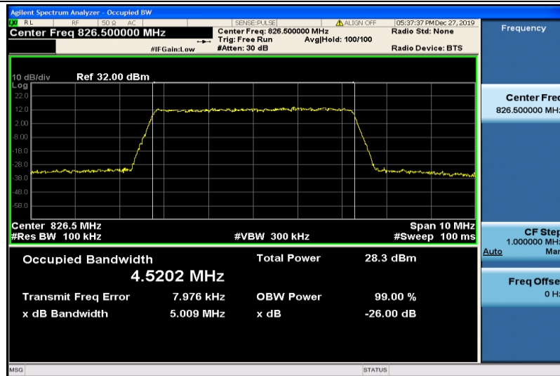
Band26-5MHz-16QAM-26815-25RB#0-4.5202
