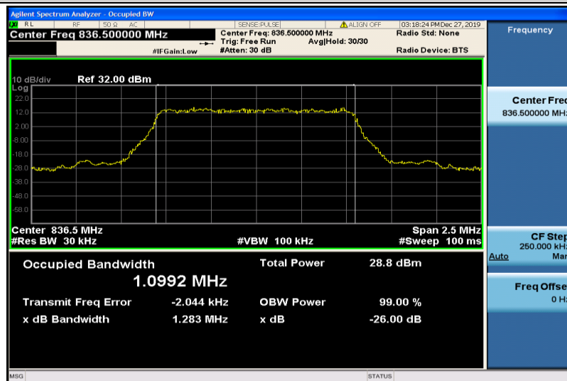
Band26-1.4MHz-QPSK-26915-6RB#0-1.0992
