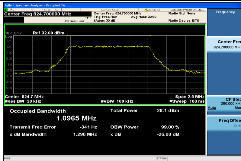
Band26-1.4MHz-QPSK-26797-6RB#0-1.0965
