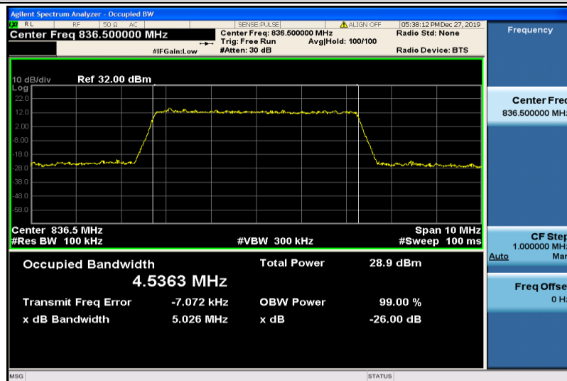
Band26-5MHz-16QAM-26915-25RB#0-4.5363
