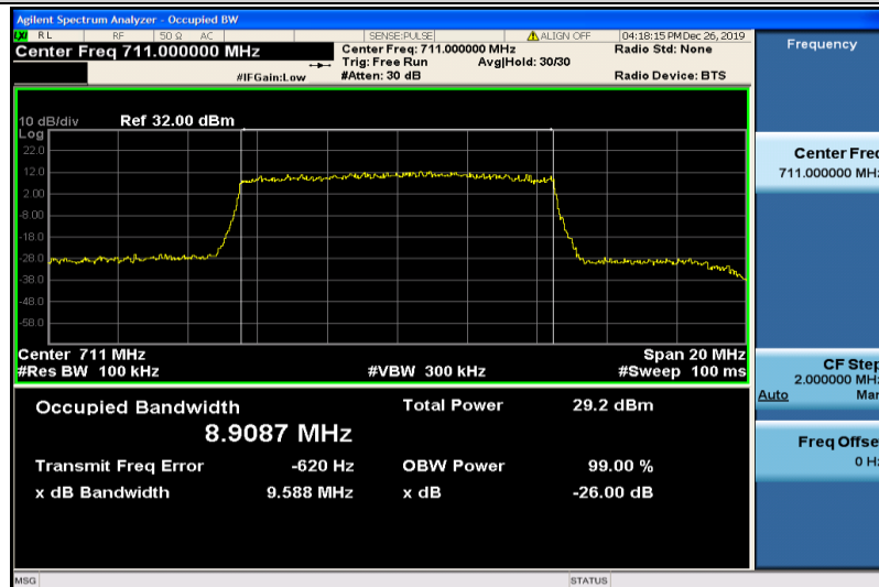
Band17-10MHz-16QAM-23800-50RB#0-8.9087
