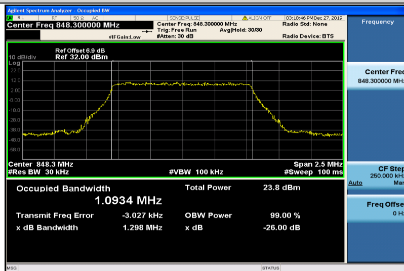
Band26-1.4MHz-QPSK-27033-6RB#0-1.0934
