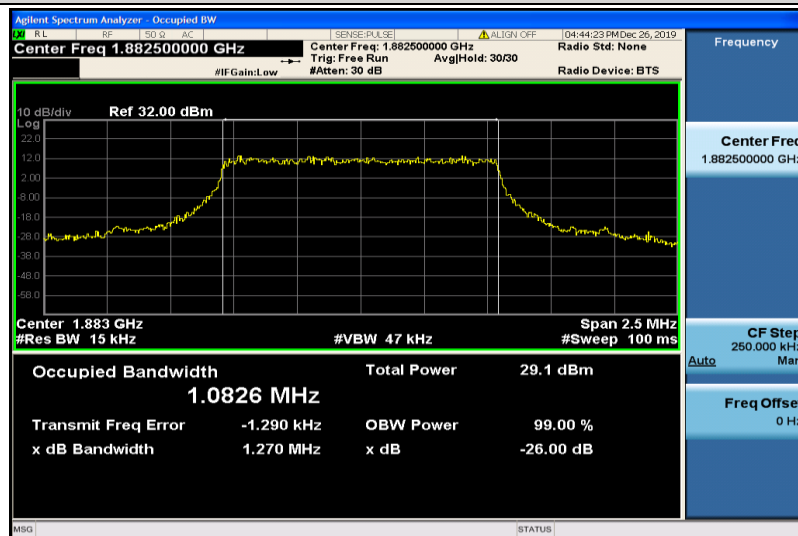
Band25-1.4MHz-16QAM-26365-6RB#0-1.0826
