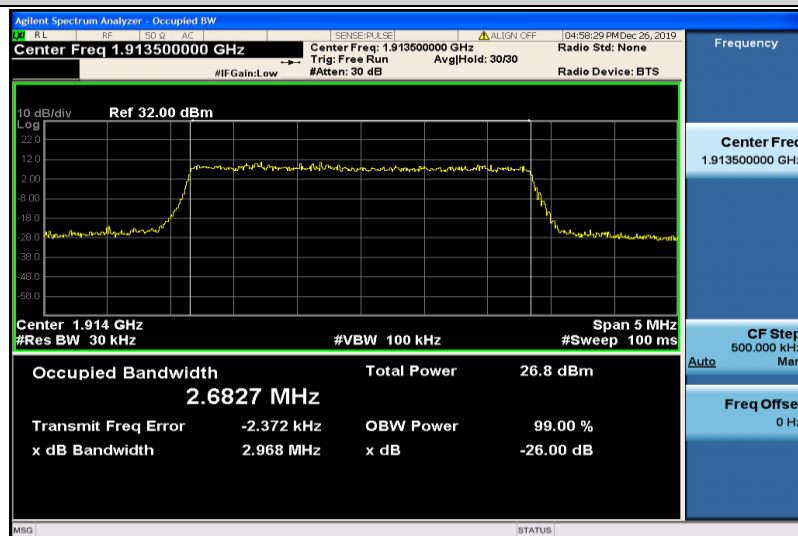
Band25-3MHz-16QAM-26675-15RB#0-2.6827
