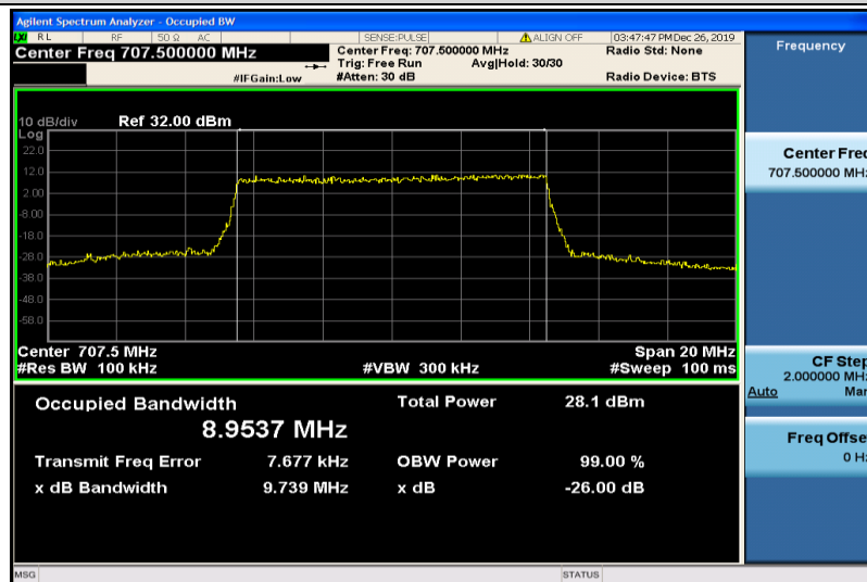
Band12-10MHz-16QAM-23095-50RB#0-8.9537
