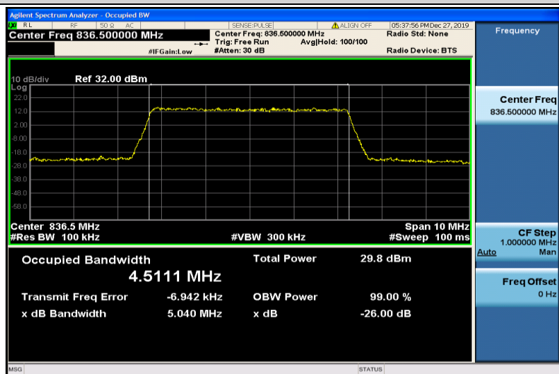
Band26-5MHz-QPSK-26915-25RB#0-4.5111
