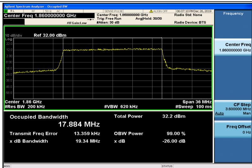
Band25-20MHz-QPSK-26140-100RB#0-17.884
