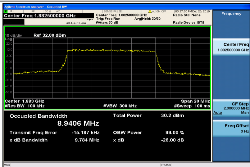
Band25-10MHz-16QAM-26365-50RB#0-8.9406
