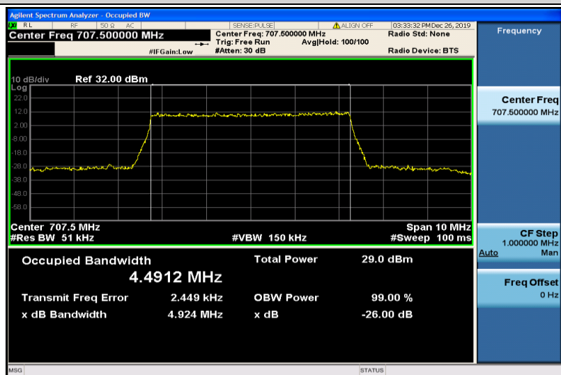
Band12-5MHz-QPSK-23095-25RB#0-4.4912
