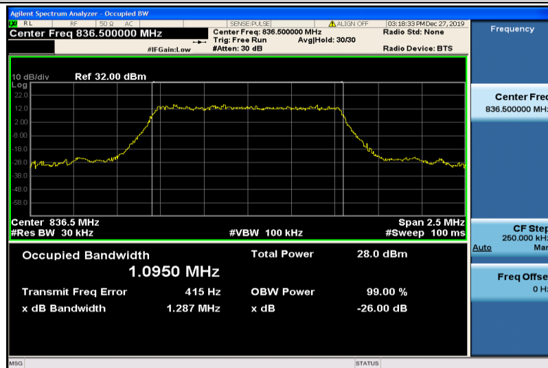
Band26-1.4MHz-16QAM-26915-6RB#0-1.0950
