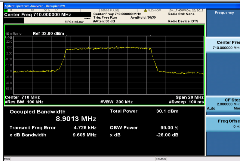
Band17-10MHz-QPSK-23790-50RB#0-8.9013
