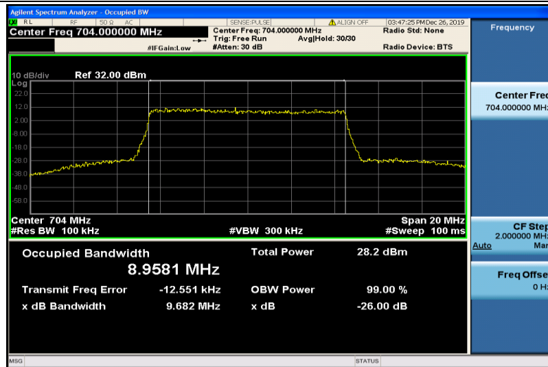
Band12-10MHz-16QAM-23060-50RB#0-8.9581
