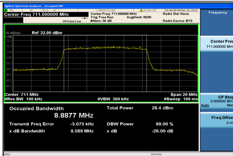
Band12-10MHz-16QAM-23130-50RB#0-8.8877
