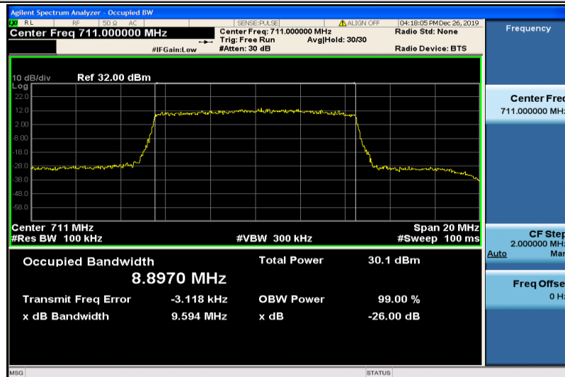
Band17-10MHz-QPSK-23800-50RB#0-8.8970
