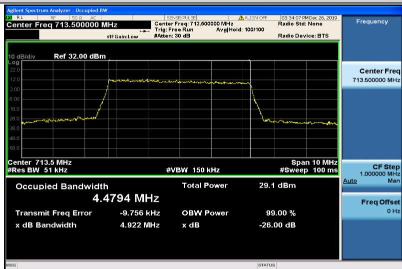
Band12-5MHz-QPSK-23155-25RB#0-4.4794
