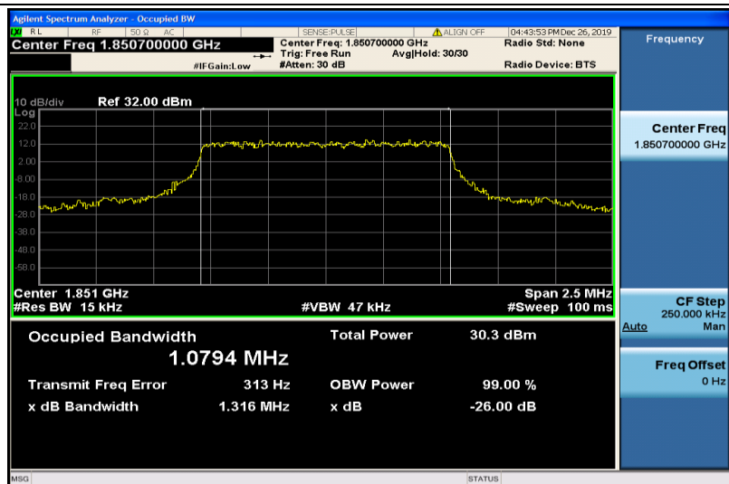
Band25-1.4MHz-QPSK-26047-6RB#0-1.0794
