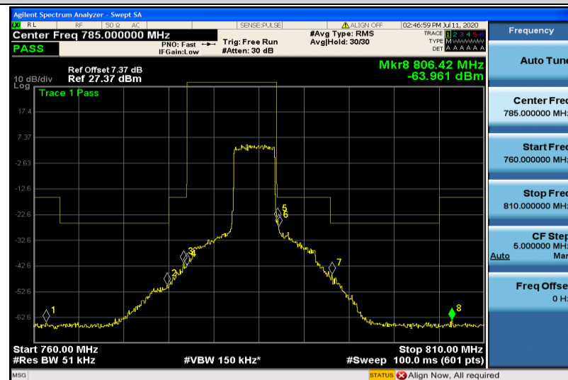
Band13-5MHz-QPSK-23255-25RB#0
