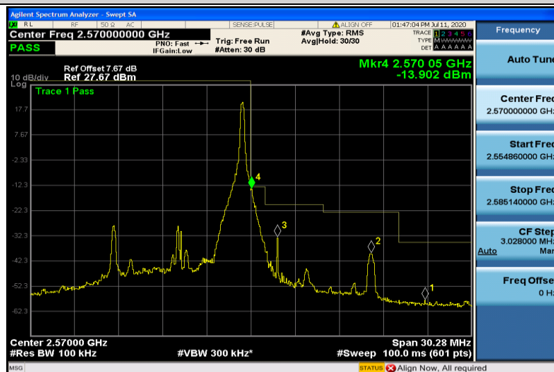
Band7-10MHz-QPSK-21400-1RB#49
