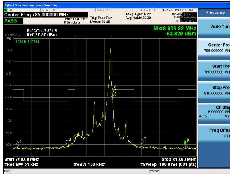
Band13-5MHz-QPSK-23255-1RB#24
