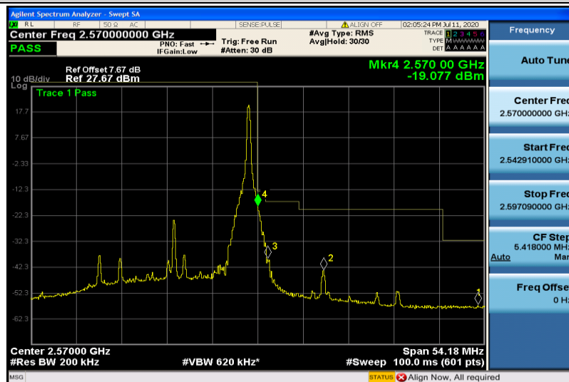
Band7-20MHz-16QAM-21350-1RB#99
