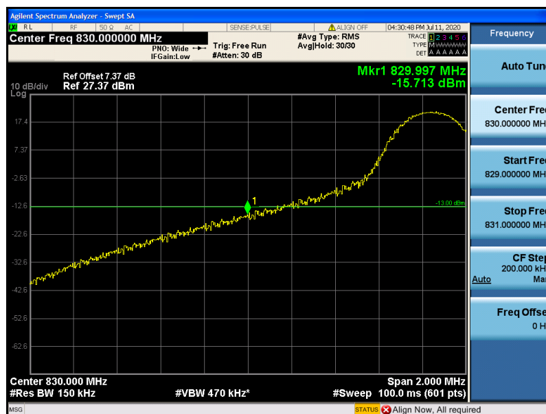
Band19-15MHz-QPSK-24075-1RB#0
