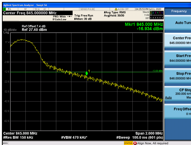
Band19-15MHz-16QAM -24075-1RB#74
