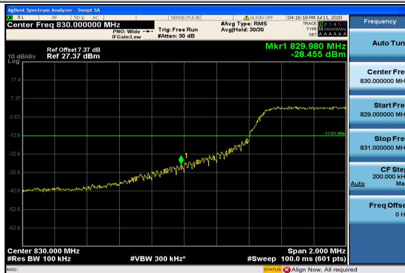
Band19-10MHz-QPSK-24050-50RB#0
