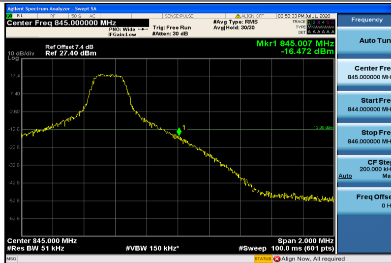
Band19-5MHz-QPSK-24125-1RB#24
