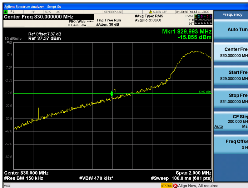
Band19-15MHz-16QAM-24075-1RB#0
