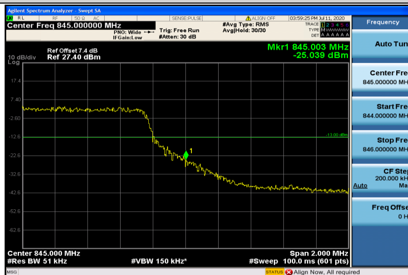
Band19-5MHz-16QAM-24125-25RB#0
