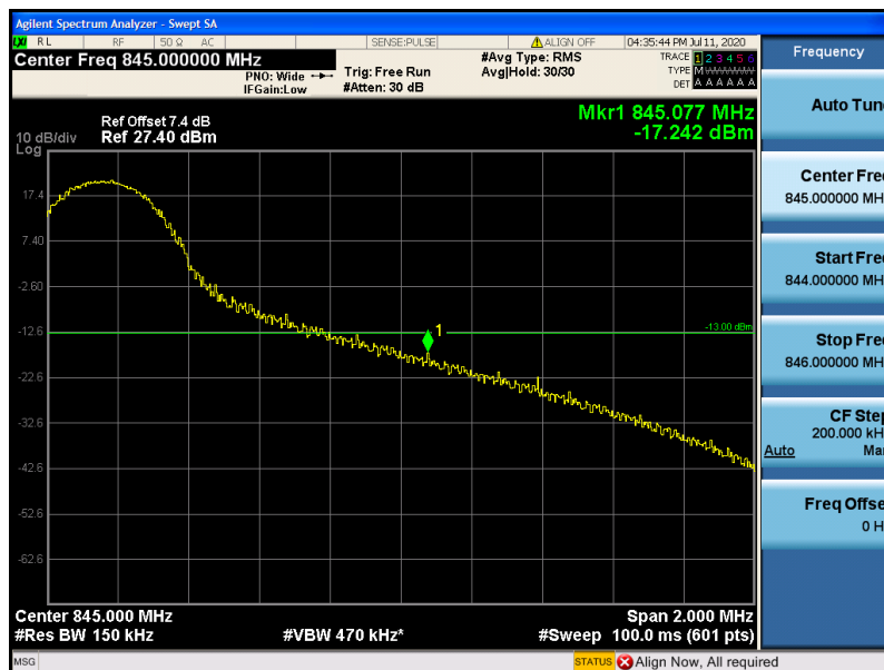
Band19-15MHz-QPSK-24075-1RB#74
