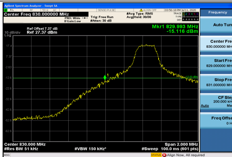
Band19-5MHz-QPSK-24025-1RB#0
