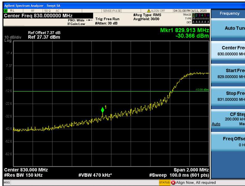
Band19-15MHz-QPSK-24075-75RB#0
