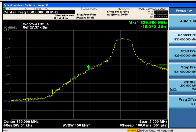
Band19-5MHz-16QAM-24025-1RB#0
