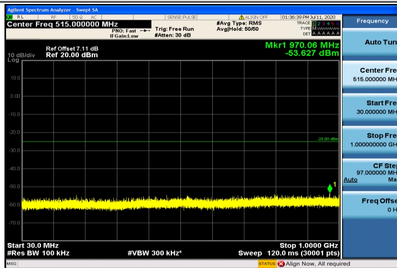
Band7-5MHz-QPSK-20775-1RB#0-30~1000MHz
