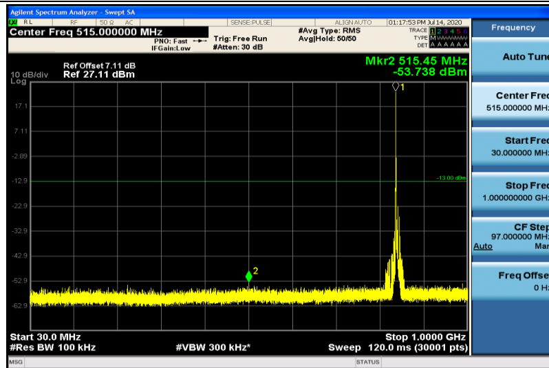
Band19-5MHz-16QAM-24125-1RB#0-30~1000MHz
