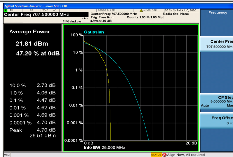
Band12-10MHz-QPSK-23095-1RB#0
