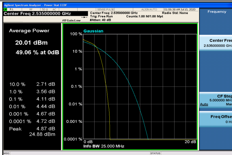
Band7-20MHz-16QAM-21100-1RB#0
