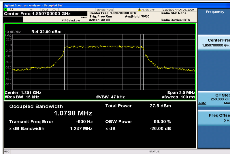
Band2-1.4MHz-QPSK-18607-6RB#0-1.0798
