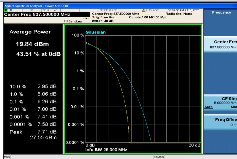
Band19-10MHz-16QAM-24075-50RB#0
