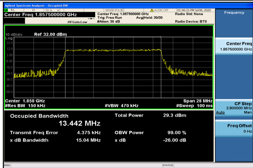
Band2-15MHz-QPSK-18675-75RB#0-13.442
