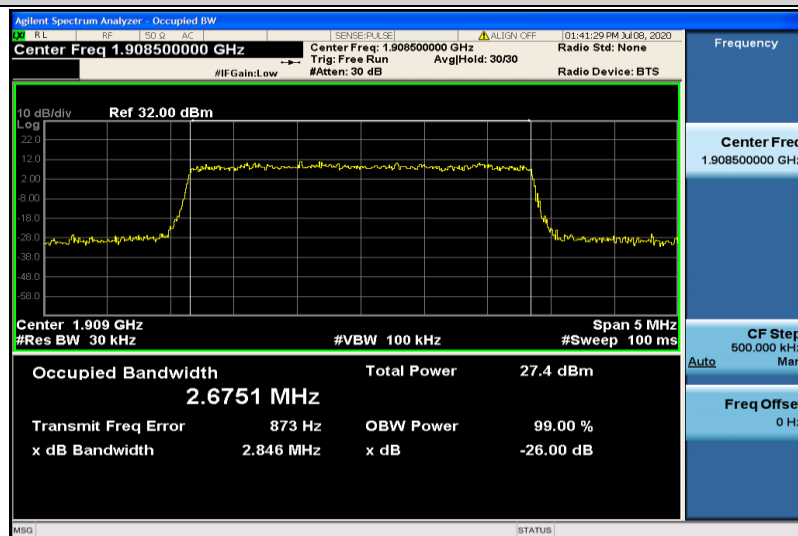
Band2-3MHz-16QAM-19185-15RB#0-2.6751
