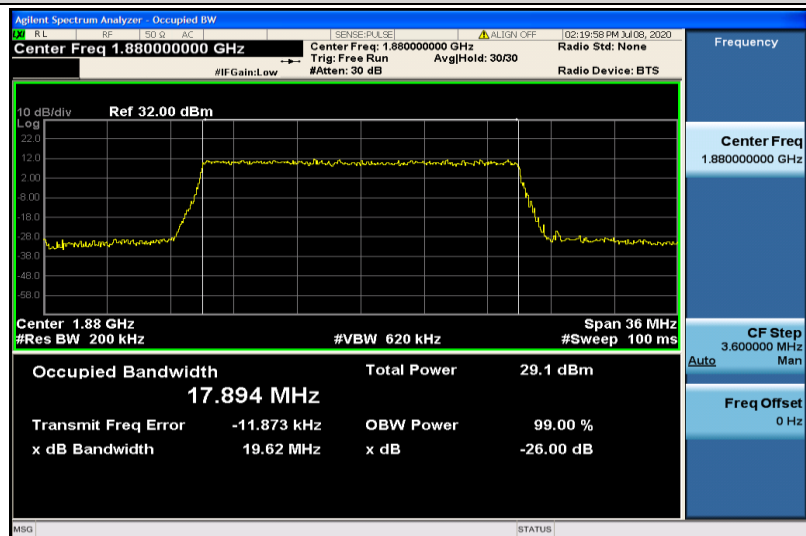
Band2-20MHz-QPSK-18900-100RB#0-17.894
