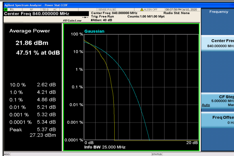
Band19-10MHz-QPSK-24100-1RB#0
