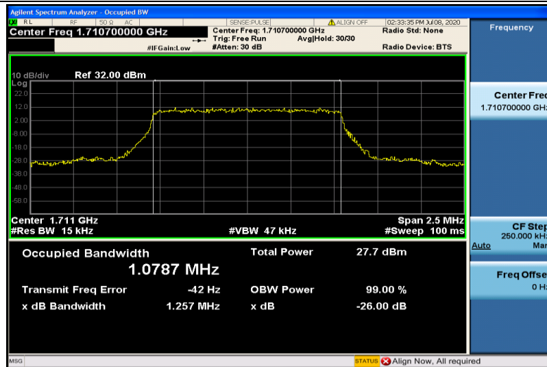
Band4-1.4MHz-QPSK-19957-6RB#0-1.0787
