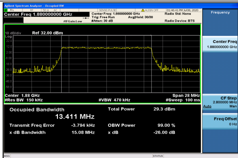
Band2-15MHz-QPSK-18900-75RB#0-13.411
