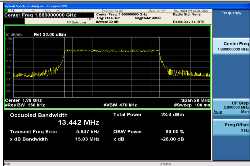
Band2-15MHz-16QAM-18900-75RB#0-13.442
