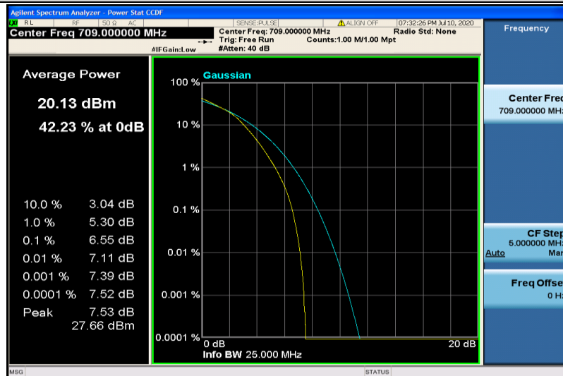
Band17-10MHz-16QAM-23780-50RB#0
