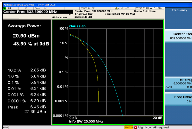
Band19-5MHz-16QAM-24025-1RB#0
