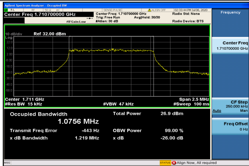
Band4-1.4MHz-16QAM-19957-6RB#0-1.0756
