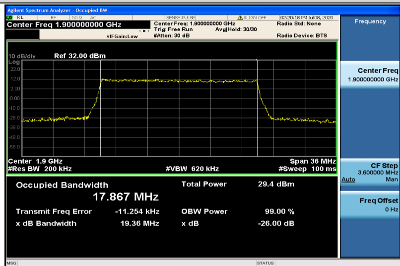
Band2-20MHz-QPSK-19100-100RB#0-17.867
