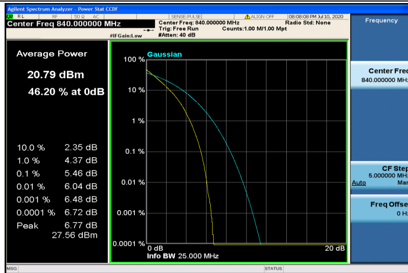
Band19-10MHz-QPSK-24100-50RB#0
