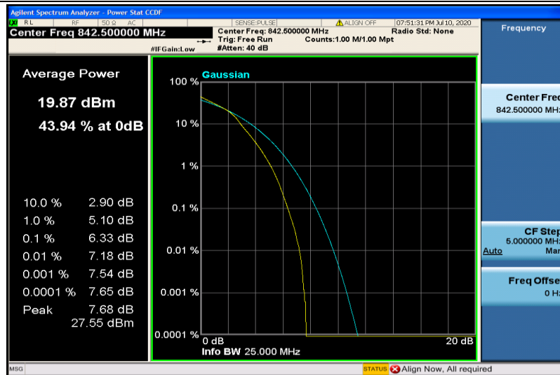
Band19-5MHz-16QAM-24125-25RB#0
