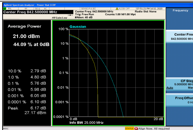
Band19-5MHz-16QAM-24125-1RB#0
