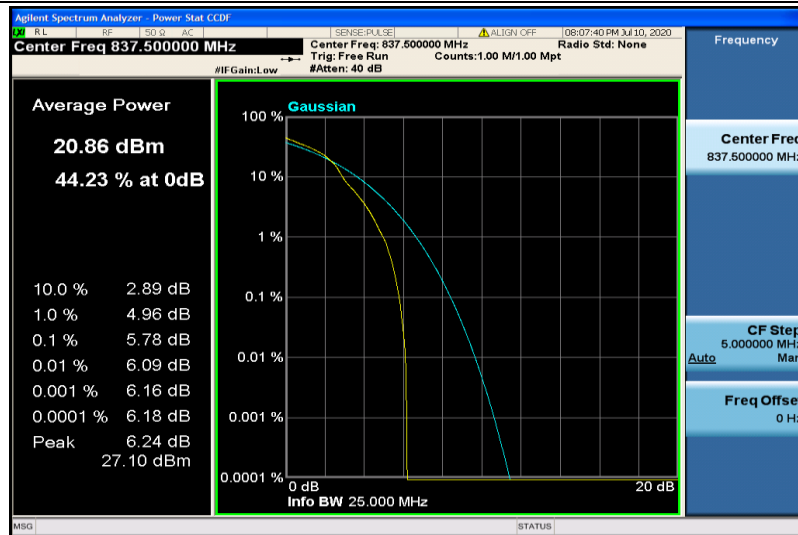
Band19-10MHz-16QAM-24075-1RB#0
