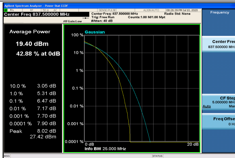
Band19-15MHz-16QAM-24075-75RB#0
