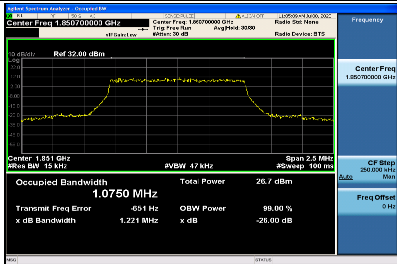
Band2-1.4MHz-16QAM-18607-6RB#0-1.0750
