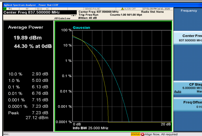
Band19-5MHz-16QAM-24075-25RB#0
