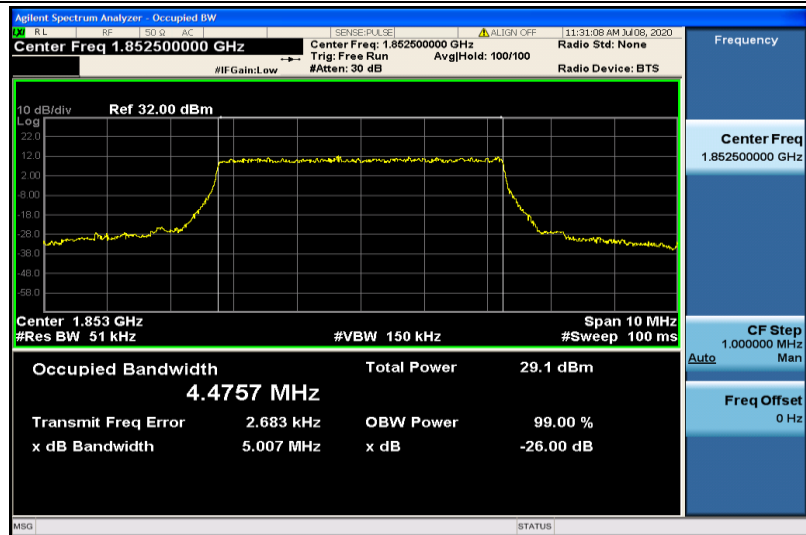
Band2-5MHz-QPSK-18625-25RB#0-4.4757
