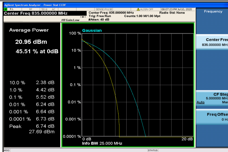
Band19-10MHz-QPSK-24050-50RB#0
