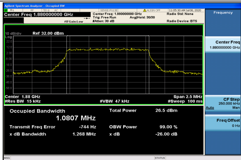
Band2-1.4MHz-16QAM-18900-6RB#0-1.0807
