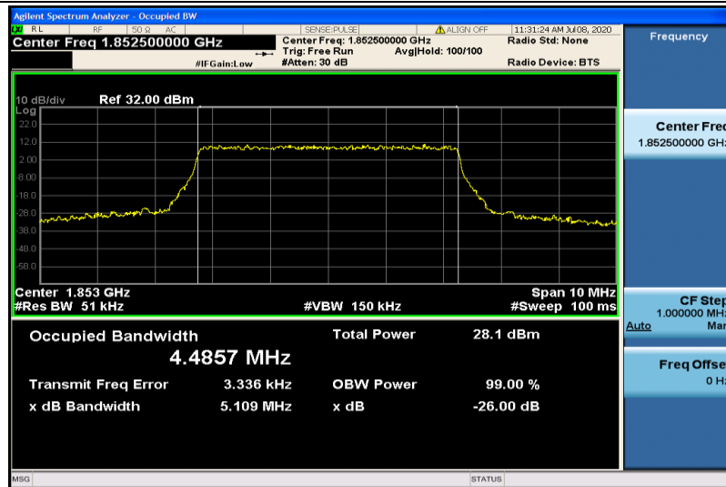
Band2-5MHz-16QAM-18625-25RB#0-4.4857
