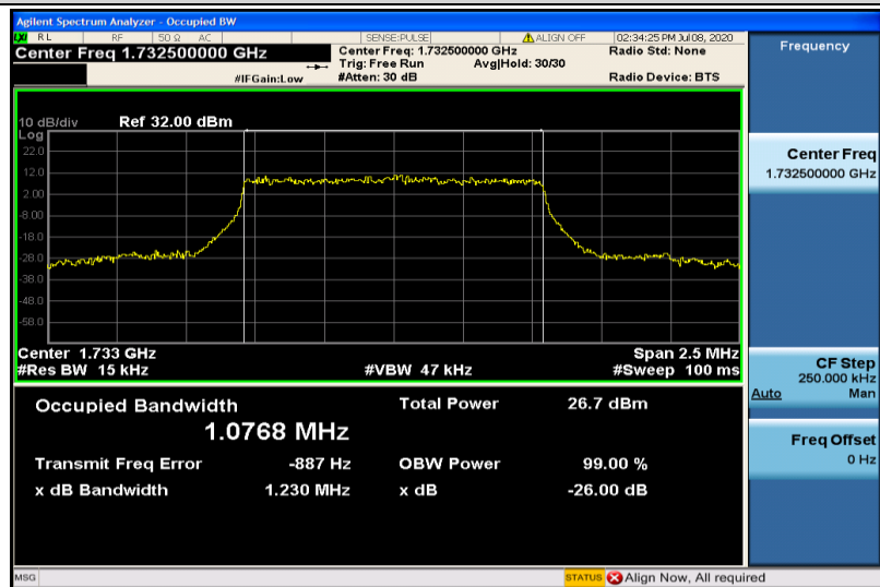
Band4-1.4MHz-16QAM-20175-6RB#0-1.0768
