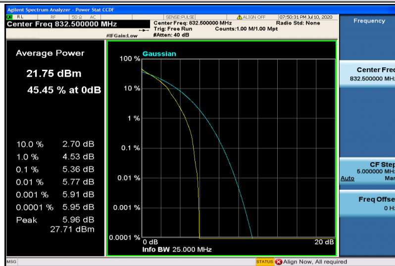
Band19-5MHz-QPSK-24025-1RB#0
