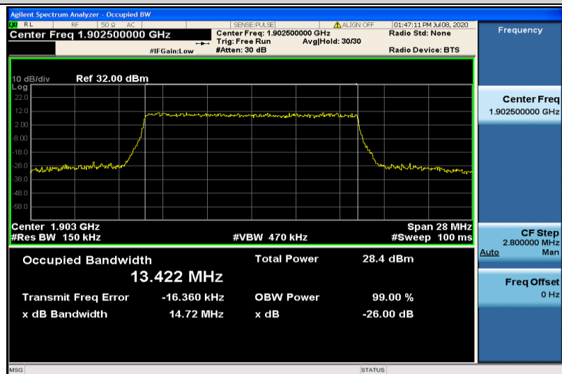
Band2-15MHz-16QAM-19125-75RB#0-13.422
