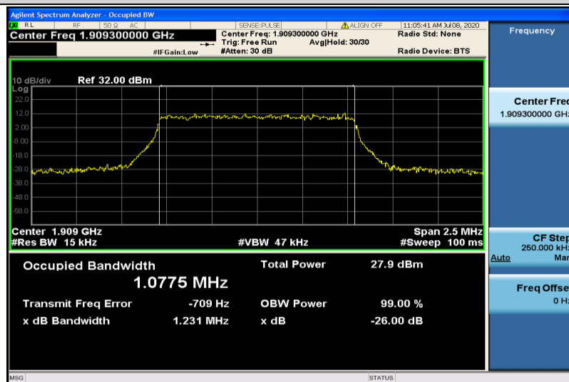
Band2-1.4MHz-QPSK-19193-6RB#0-1.0775
