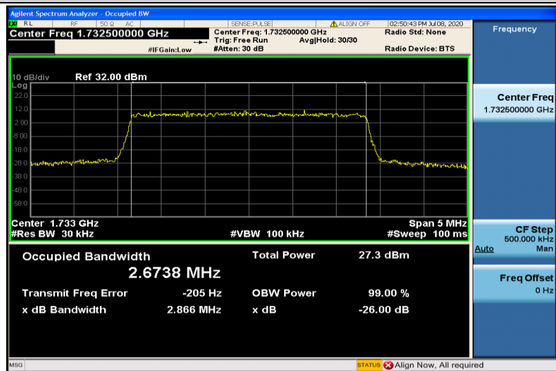
Band4-3MHz-16QAM-20175-15RB#0-2.6738
