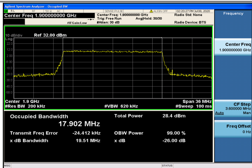
Band2-20MHz-16QAM-19100-100RB#0-17.902
