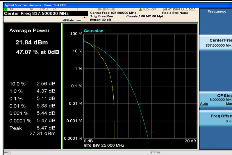
Band19-10MHz-QPSK-24075-1RB#0
