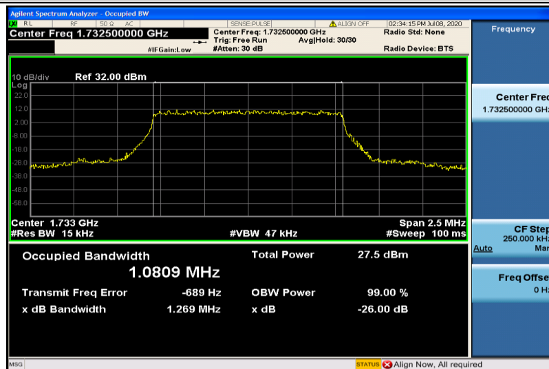
Band4-1.4MHz-QPSK-20175-6RB#0-1.0809
