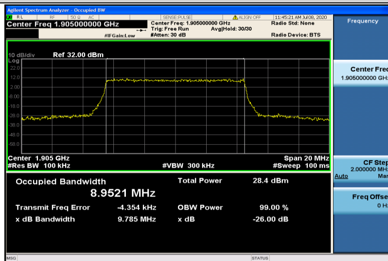
Band2-10MHz-16QAM-19150-50RB#0-8.9521
