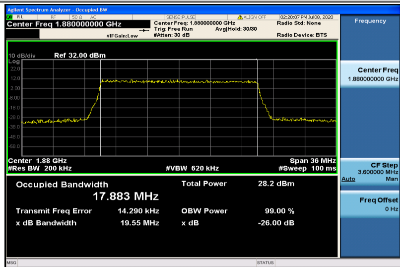
Band2-20MHz-16QAM-18900-100RB#0-17.883
