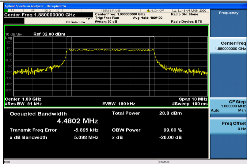
Band2-5MHz-QPSK-18900-25RB#0-4.4802
