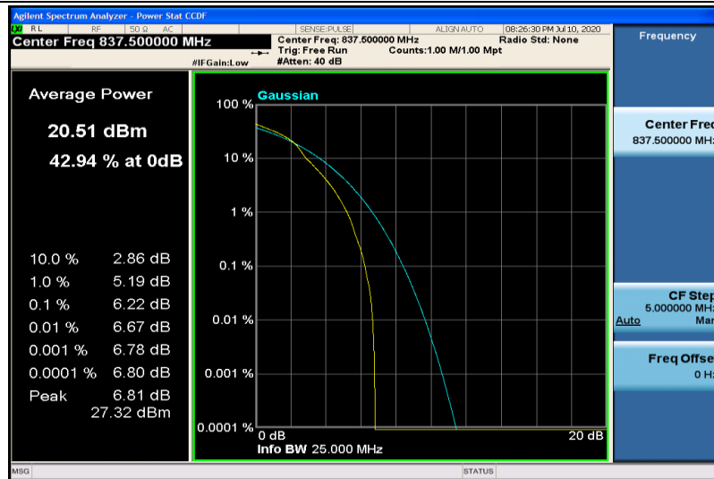
Band19-15MHz-16QAM-24075-1RB#0
