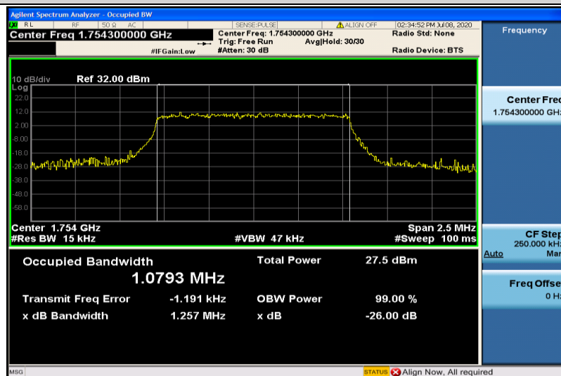
Band4-1.4MHz-QPSK-20393-6RB#0-1.0793
