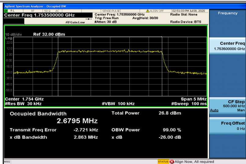
Band4-3MHz-16QAM-20385-15RB#0-2.6795
