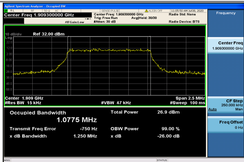
Band2-1.4MHz-16QAM-19193-6RB#0-1.0775
