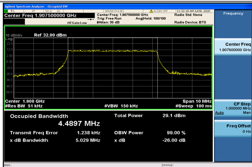
Band2-5MHz-QPSK-19175-25RB#0-4.4897
