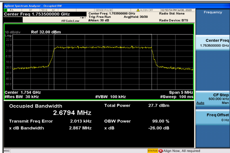
Band4-3MHz-QPSK-20385-15RB#0-2.6794
