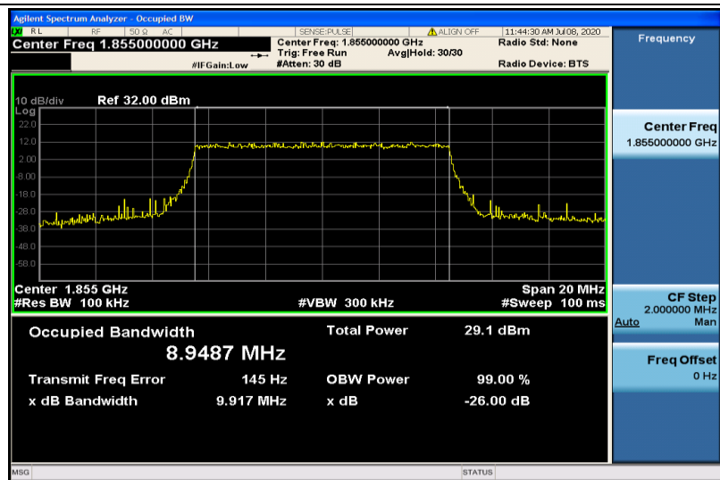
Band2-10MHz-QPSK-18650-50RB#0-8.9487
