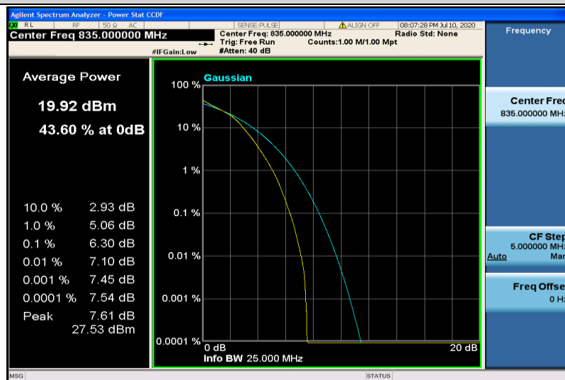
Band19-10MHz-16QAM-24050-50RB#0
