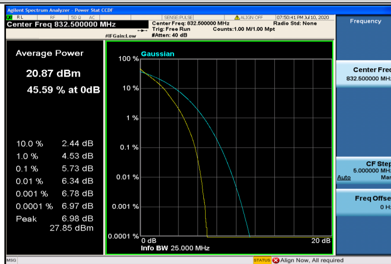
Band19-5MHz-QPSK-24025-25RB#0
