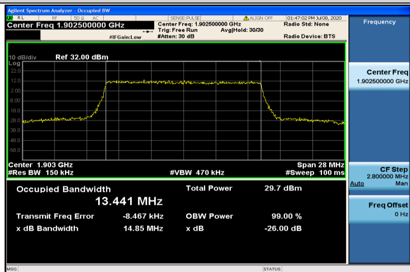
Band2-15MHz-QPSK-19125-75RB#0-13.441
