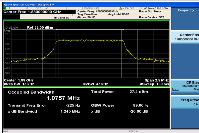
Band2-1.4MHz-QPSK-18900-6RB#0-1.0757
