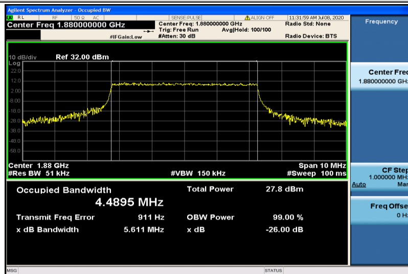
Band2-5MHz-16QAM-18900-25RB#0-4.4895
