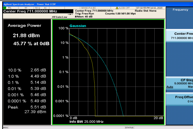
Band17-10MHz-QPSK-23800-1RB#0
