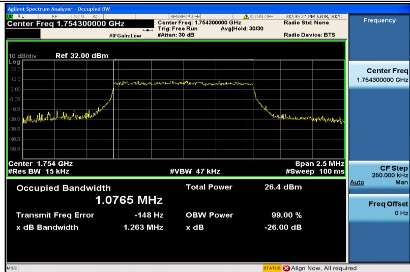
Band4-1.4MHz-16QAM-20393-6RB#0-1.0765
