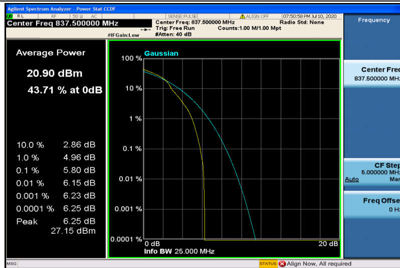
Band19-5MHz-16QAM-24075-1RB#0
