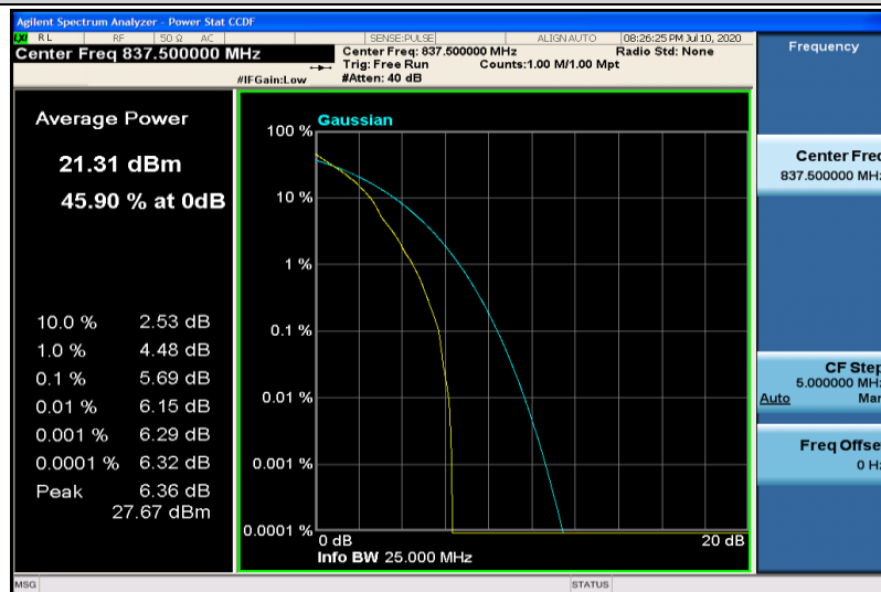
Band19-15MHz-QPSK-24075-1RB#0
