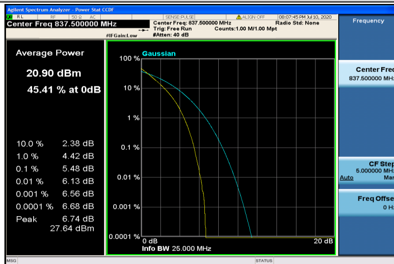
Band19-10MHz-QPSK-24075-50RB#0
