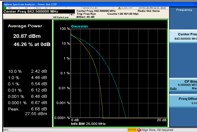
Band19-5MHz-QPSK-24125-25RB#0
