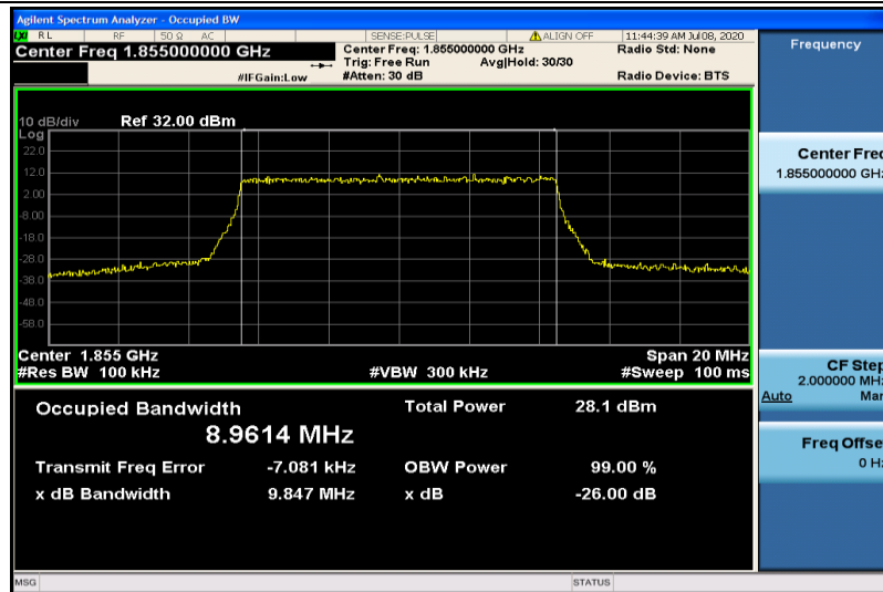
Band2-10MHz-16QAM-18650-50RB#0-8.9614
