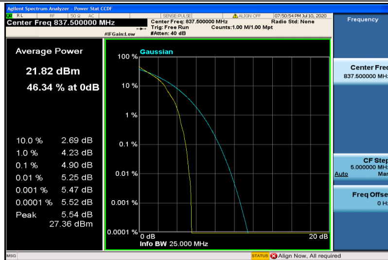
Band19-5MHz-QPSK-24075-1RB#0
