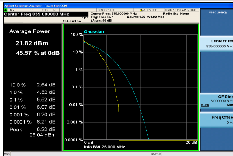
Band19-10MHz-QPSK-24050-1RB#0
