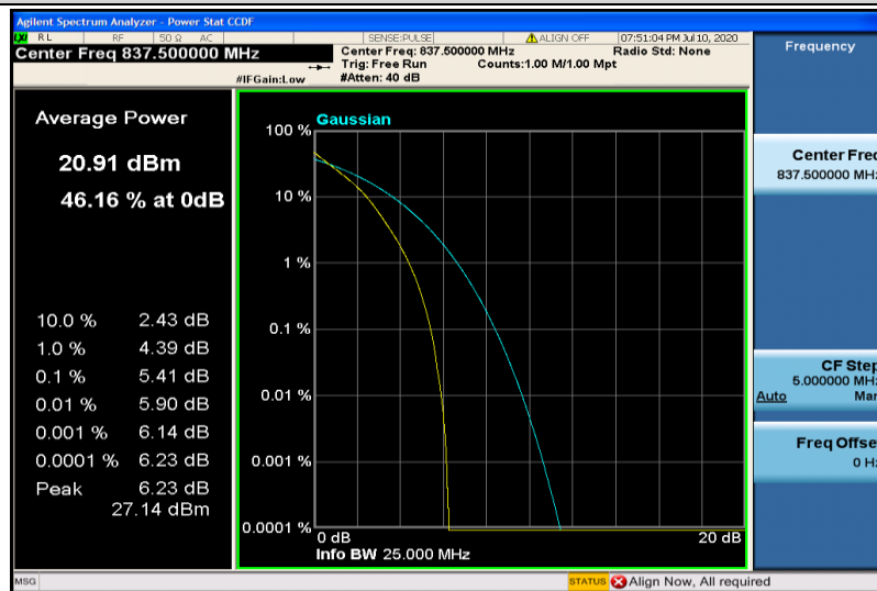
Band19-5MHz-QPSK-24075-25RB#0
