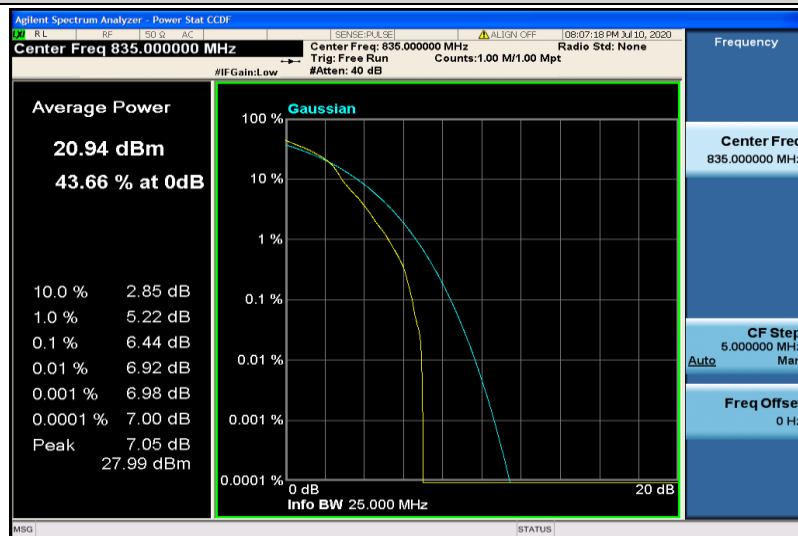
Band19-10MHz-16QAM-24050-1RB#0
