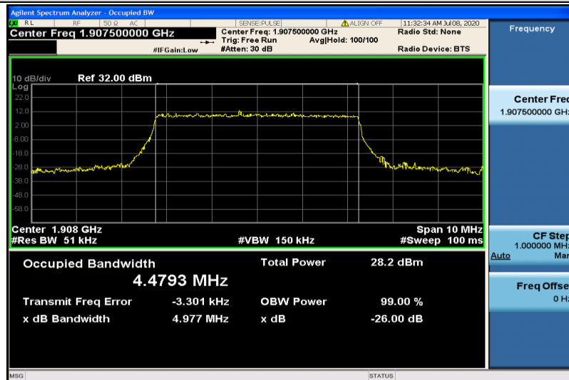
Band2-5MHz-16QAM-19175-25RB#0-4.4793
