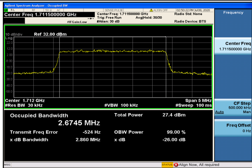
Band4-3MHz-16QAM-19965-15RB#0-2.6745
