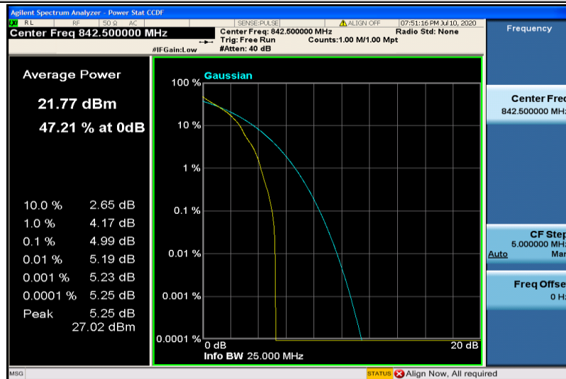
Band19-5MHz-QPSK-24125-1RB#0
