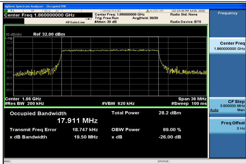
Band2-20MHz-16QAM-18700-100RB#0-17.911
