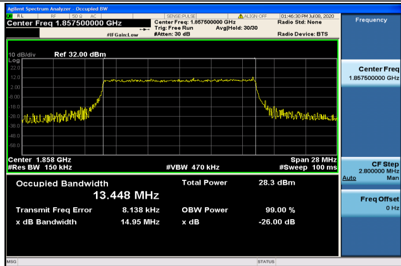
Band2-15MHz-16QAM-18675-75RB#0-13.448
