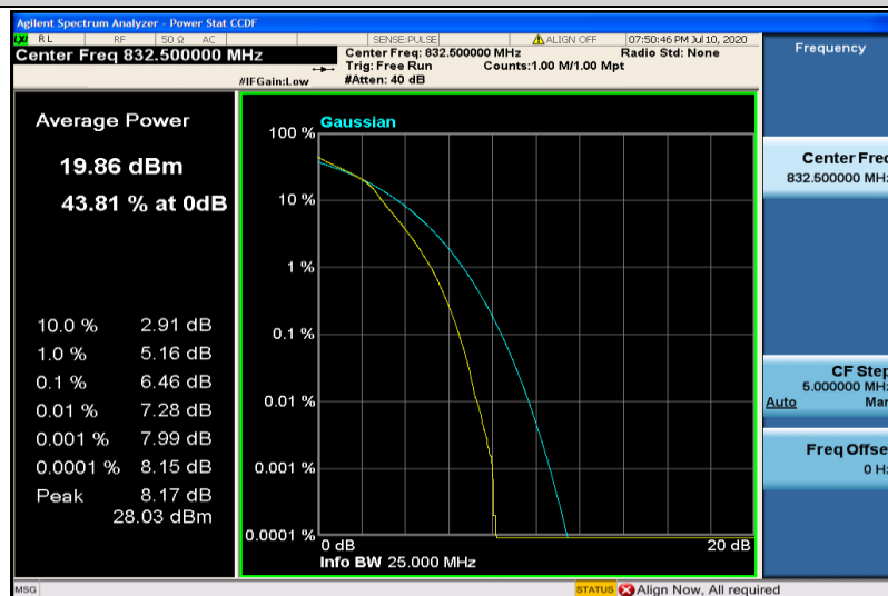
Band19-5MHz-16QAM-24025-25RB#0
