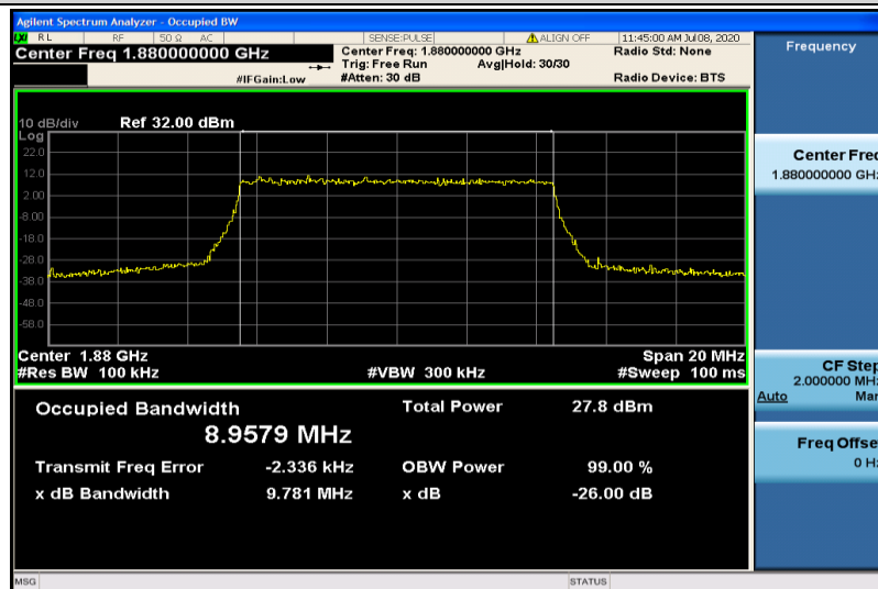
Band2-10MHz-16QAM-18900-50RB#0-8.9579
