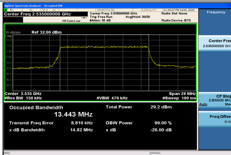
Band7-15MHz-QPSK-21100-75RB#0-13.443
