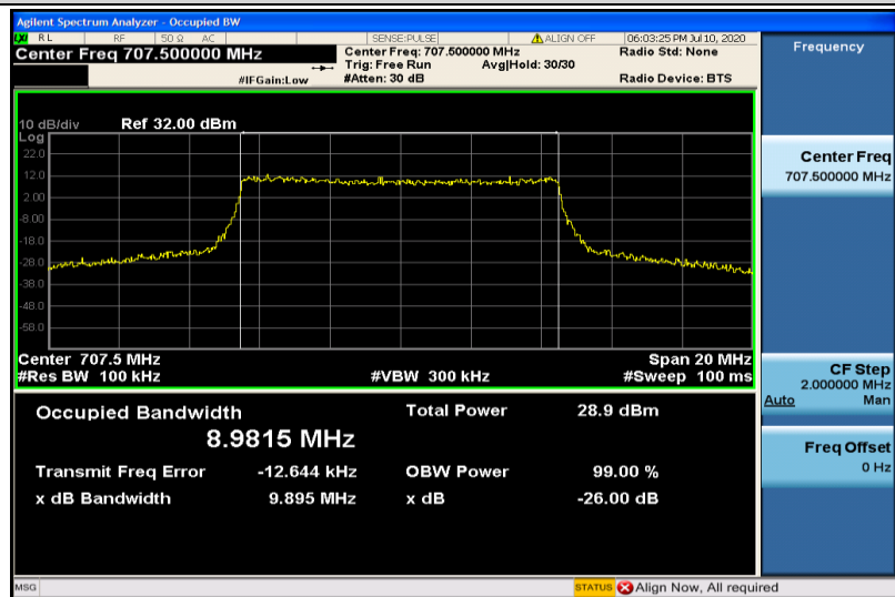
Band12-10MHz-16QAM-23095-50RB#0-8.9815
