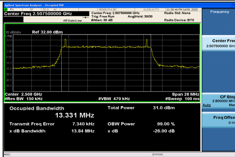
Band7-15MHz-QPSK-20825-75RB#0-13.331
