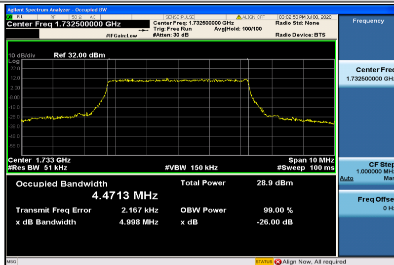
Band4-5MHz-QPSK-20175-25RB#0-4.4713
