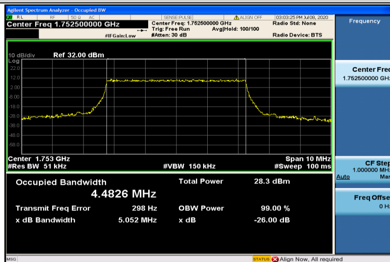
Band4-5MHz-QPSK-20375-25RB#0-4.4826
