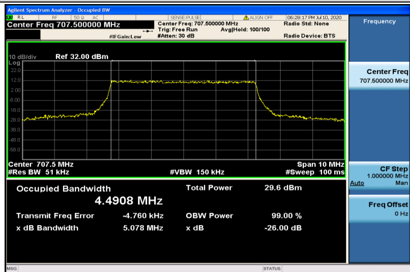
Band12-5MHz-QPSK-23095-25RB#0-4.4908
