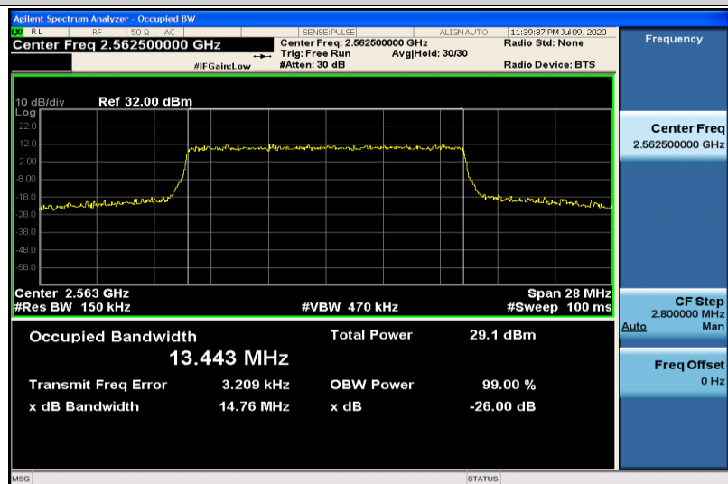
Band7-15MHz-16QAM-21375-75RB#0-13.443
