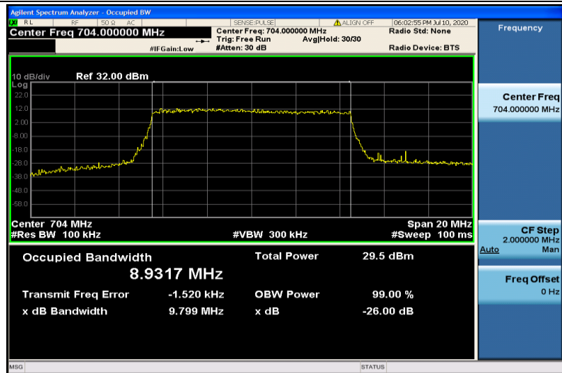
Band12-10MHz-QPSK-23060-50RB#0-8.9317
