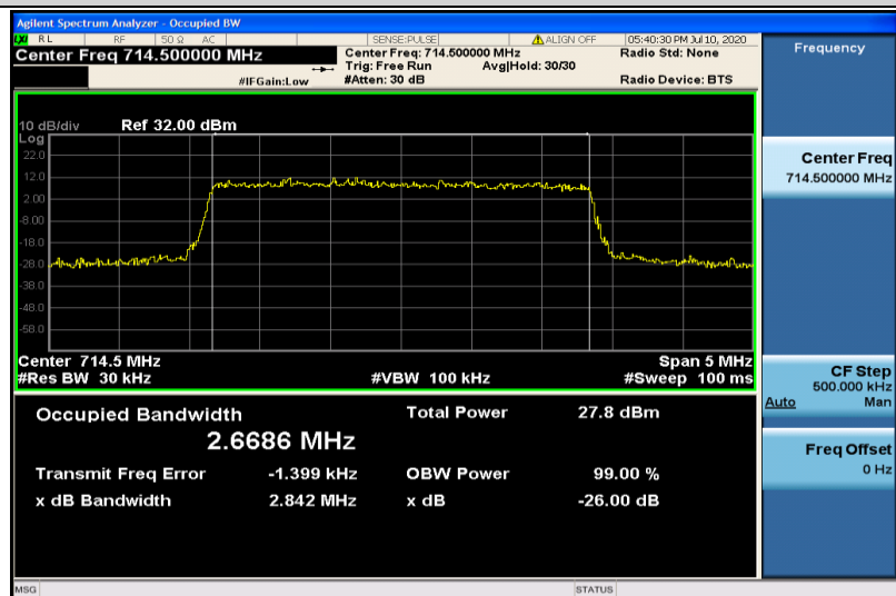
Band12-3MHz-16QAM-23165-15RB#0-2.6686
