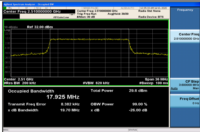
Band7-20MHz-QPSK-20850-100RB#0-17.925
