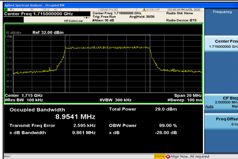
Band4-10MHz-QPSK-20000-50RB#0-8.9541
