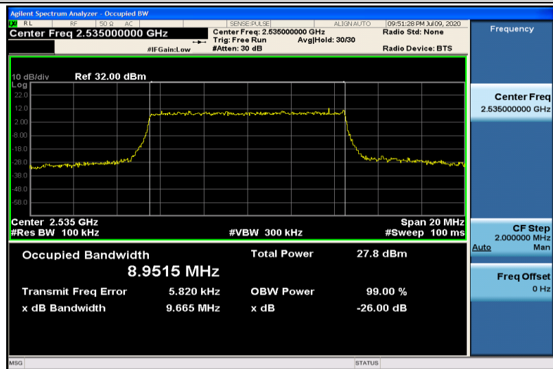
Band7-10MHz-16QAM-21100-50RB#0-8.9515
