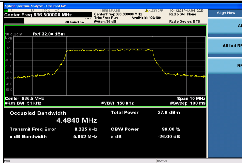
Band5-5MHz-16QAM-20525-25RB#0-4.4840
