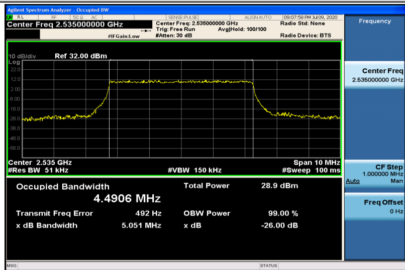
Band7-5MHz-QPSK-21100-25RB#0-4.4906
