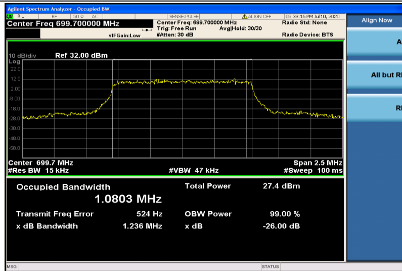
Band12-1.4MHz-16QAM-23017-6RB#0-1.0803
