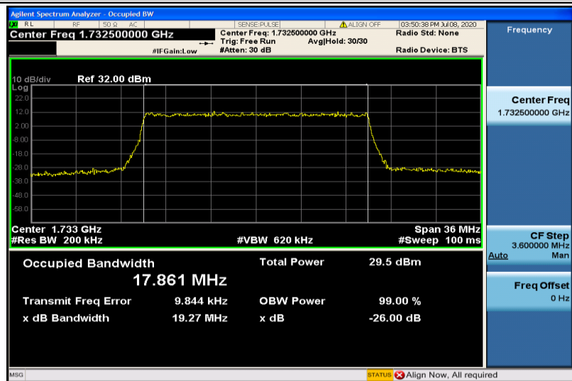
Band4-20MHz-QPSK-20175-100RB#0-17.861
