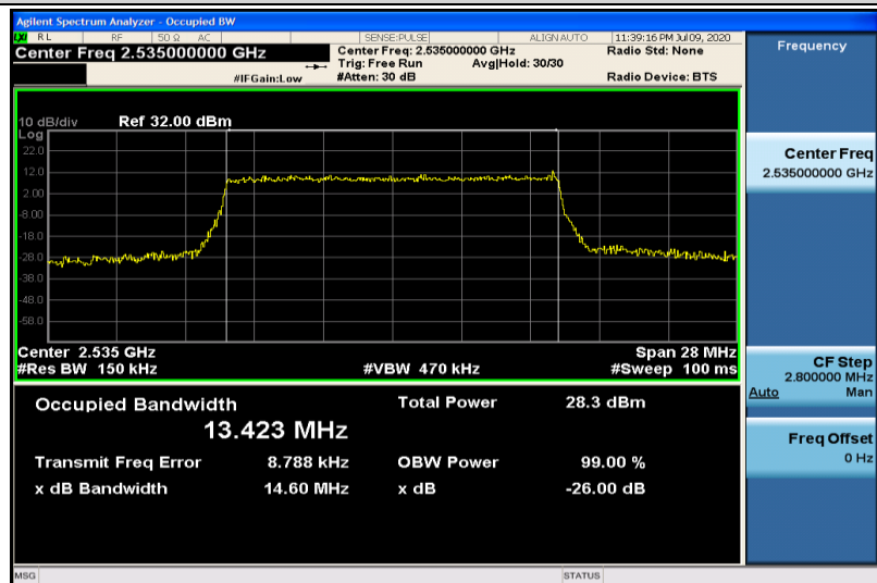
Band7-15MHz-16QAM-21100-75RB#0-13.423
