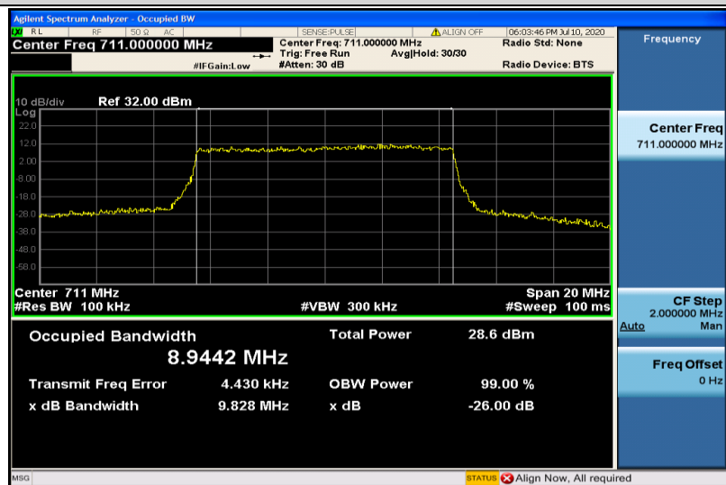
Band12-10MHz-16QAM-23130-50RB#0-8.9442
