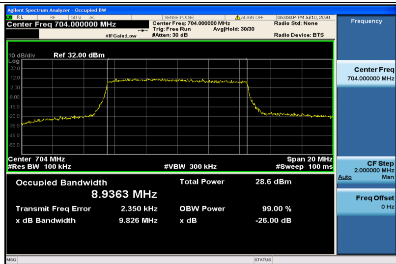
Band12-10MHz-16QAM-23060-50RB#0-8.9363
