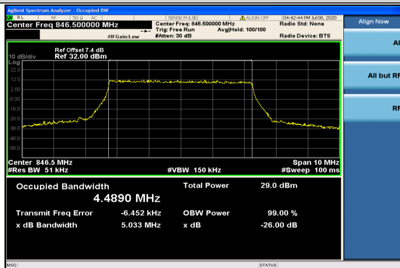
Band5-5MHz-QPSK-20625-25RB#0-4.4890
