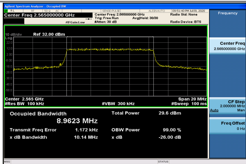
Band7-10MHz-QPSK-21400-50RB#0-8.9623
