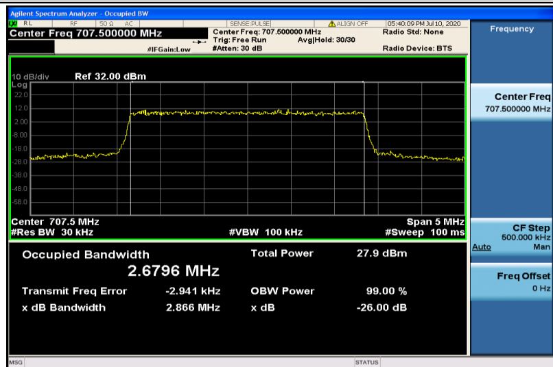
Band12-3MHz-16QAM-23095-15RB#0-2.6796
