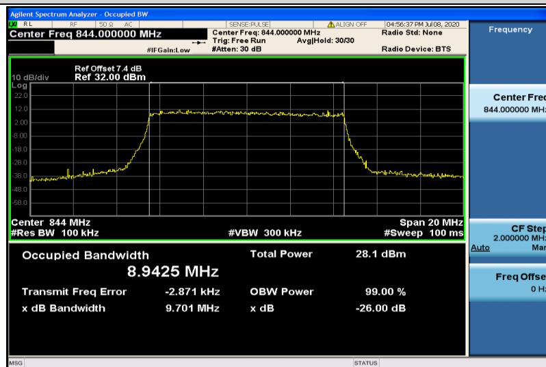
Band5-10MHz-16QAM-20600-50RB#0-8.9425
