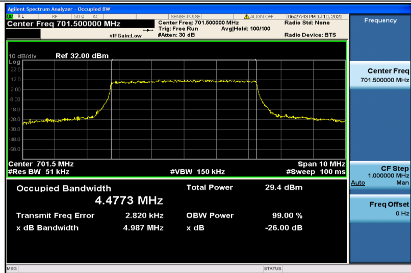
Band12-5MHz-QPSK-23035-25RB#0-4.4773
