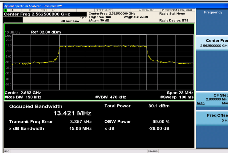
Band7-15MHz-QPSK-21375-75RB#0-13.421
