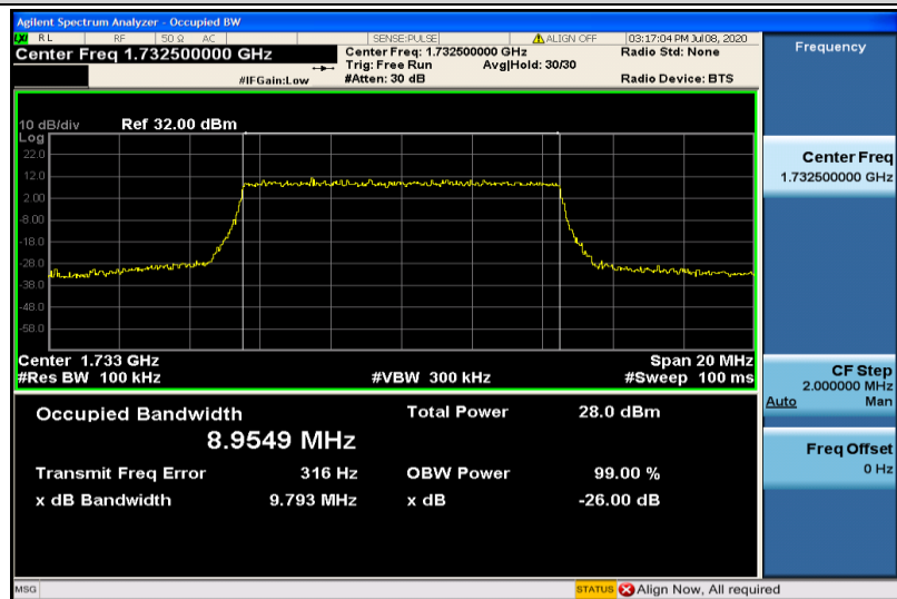
Band4-10MHz-16QAM-20175-50RB#0-8.9549
