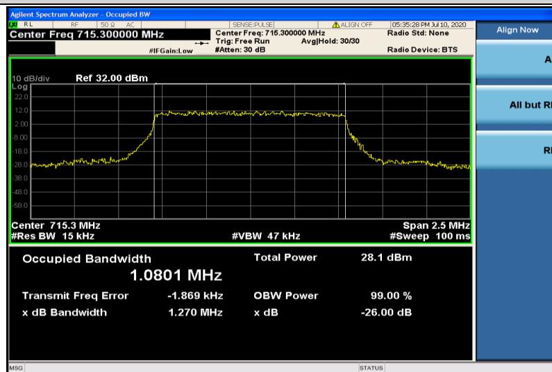
Band12-1.4MHz-QPSK-23173-6RB#0-1.0801
