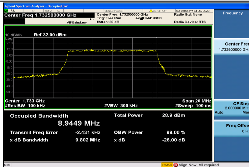
Band4-10MHz-QPSK-20175-50RB#0-8.9449
