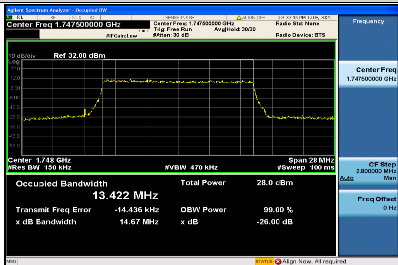
Band4-15MHz-16QAM-20325-75RB#0-13.422
