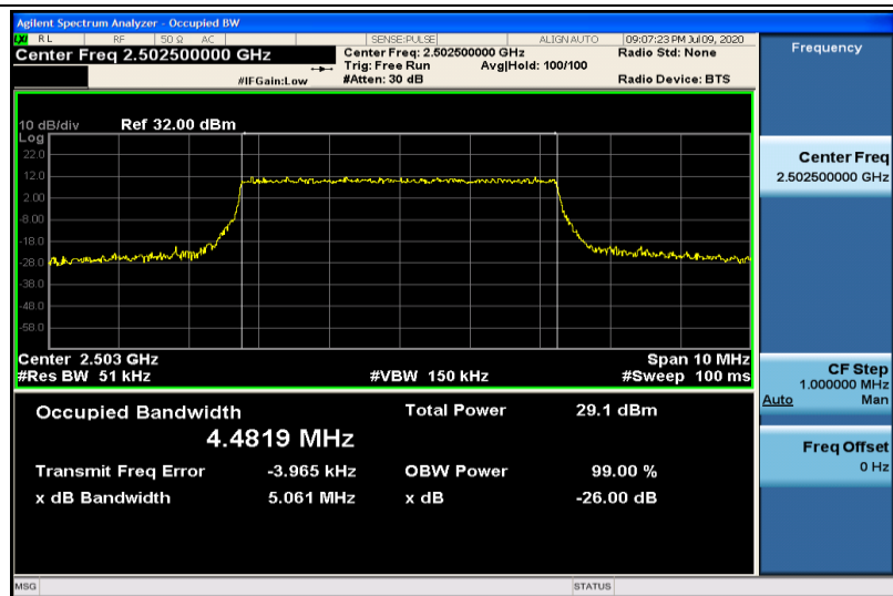
Band7-5MHz-QPSK-20775-25RB#0-4.4819
