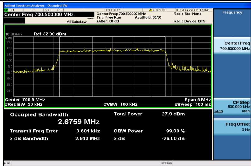
Band12-3MHz-16QAM-23025-15RB#0-2.6759
