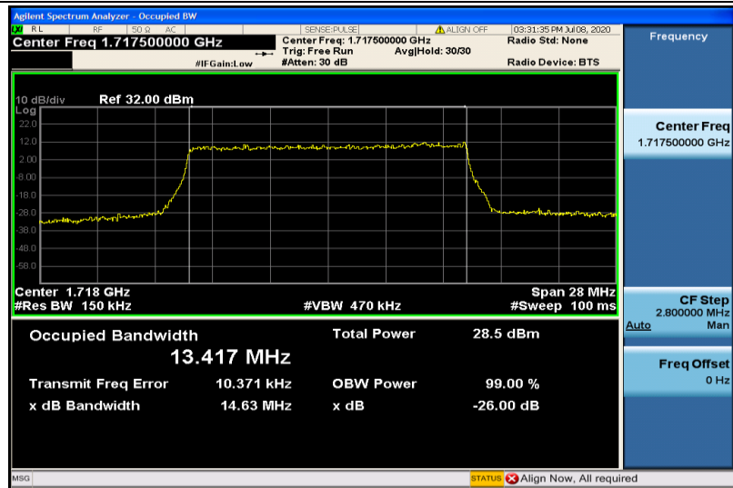
Band4-15MHz-16QAM-20025-75RB#0-13.417
