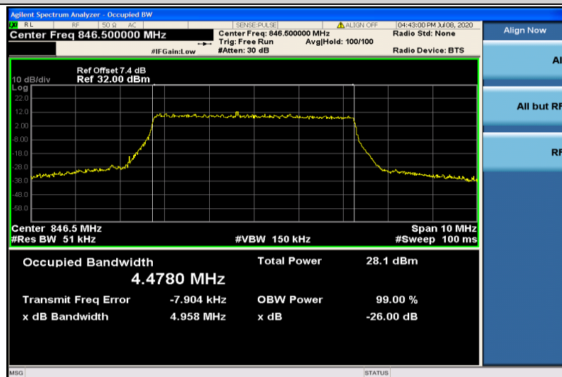
Band5-5MHz-16QAM-20625-25RB#0-4.4780
