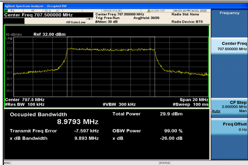
Band12-10MHz-QPSK-23095-50RB#0-8.9793
