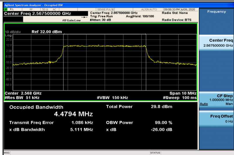
Band7-5MHz-QPSK-21425-25RB#0-4.4794
