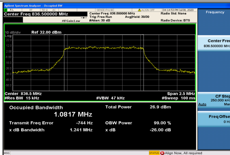
Band5-1.4MHz-16QAM-20525-6RB#0-1.0817
