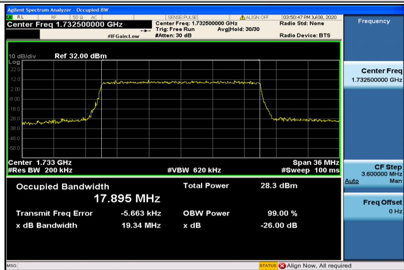
Band4-20MHz-16QAM-20175-100RB#0-17.895
