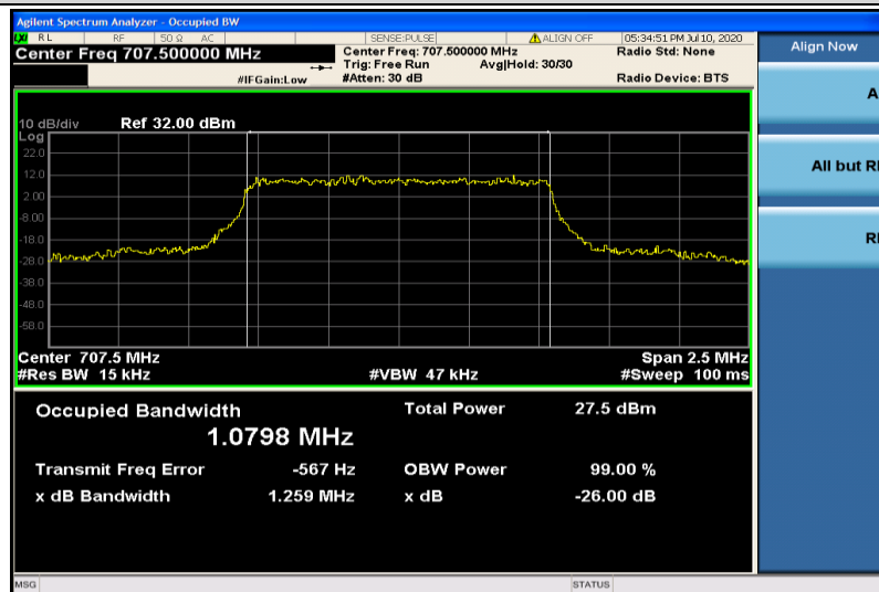
Band12-1.4MHz-16QAM-23095-6RB#0-1.0798
