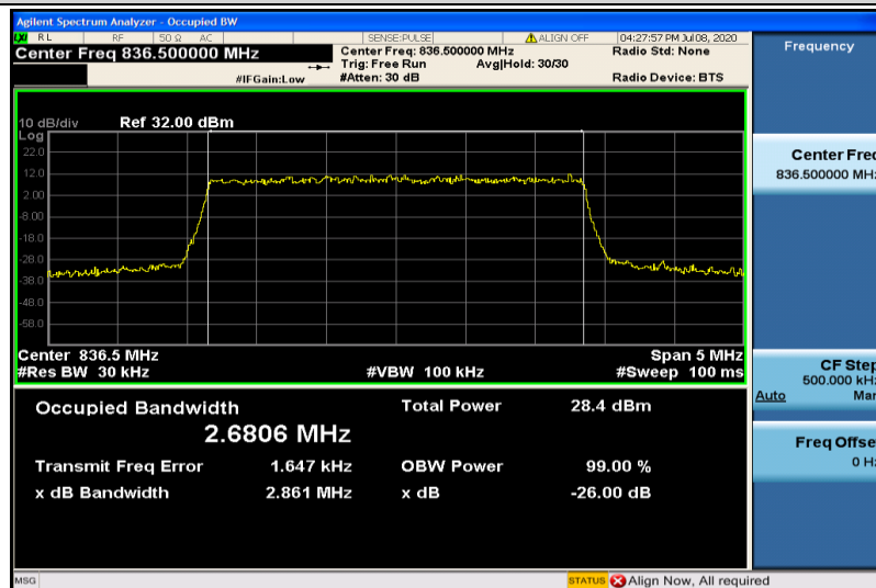
Band5-3MHz-QPSK-20525-15RB#0-2.6806
