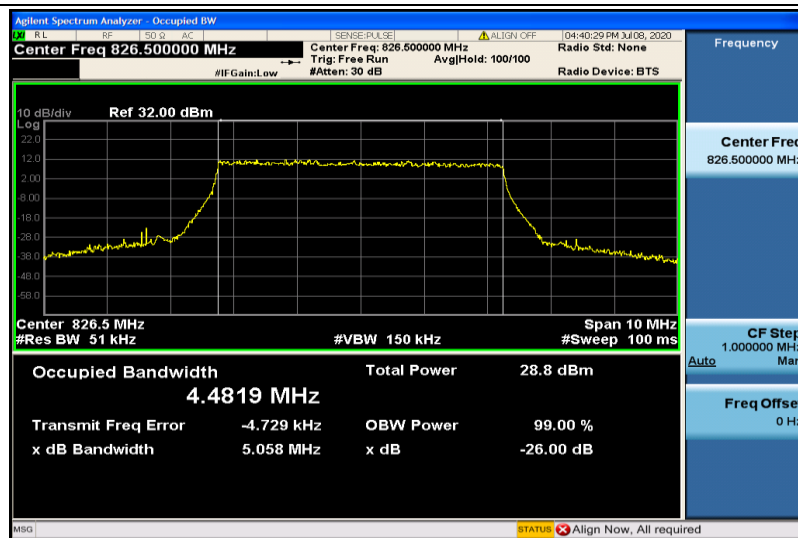
Band5-5MHz-QPSK-20425-25RB#0-4.4819
