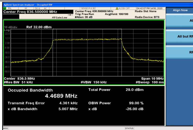
Band5-5MHz-QPSK-20525-25RB#0-4.4689
