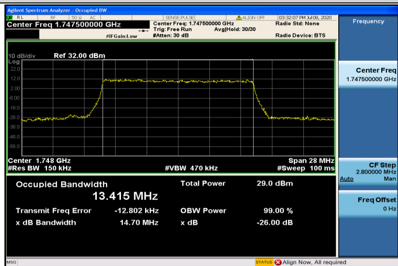
Band4-15MHz-QPSK-20325-75RB#0-13.415
