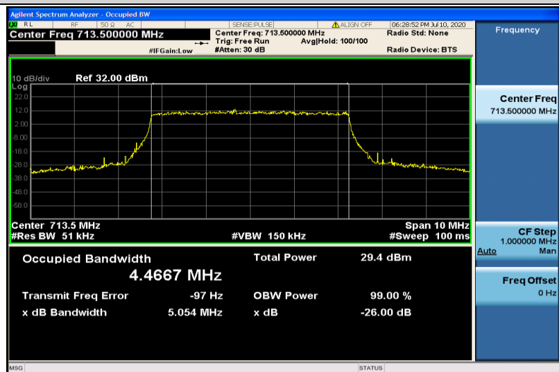
Band12-5MHz-QPSK-23155-25RB#0-4.4667
