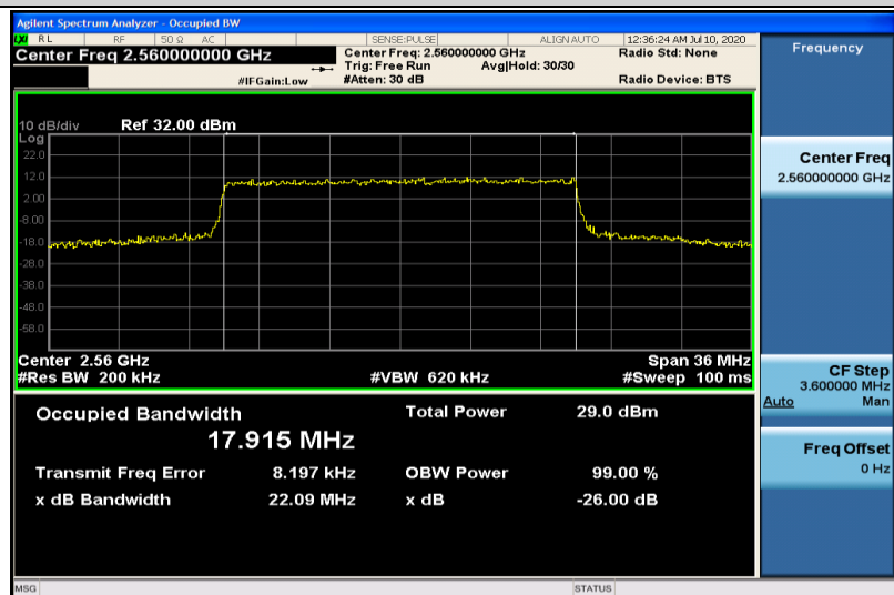
Band7-20MHz-16QAM-21350-100RB#0-17.915
