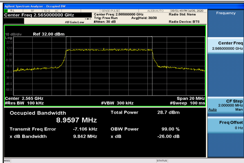
Band7-10MHz-16QAM-21400-50RB#0-8.9597
