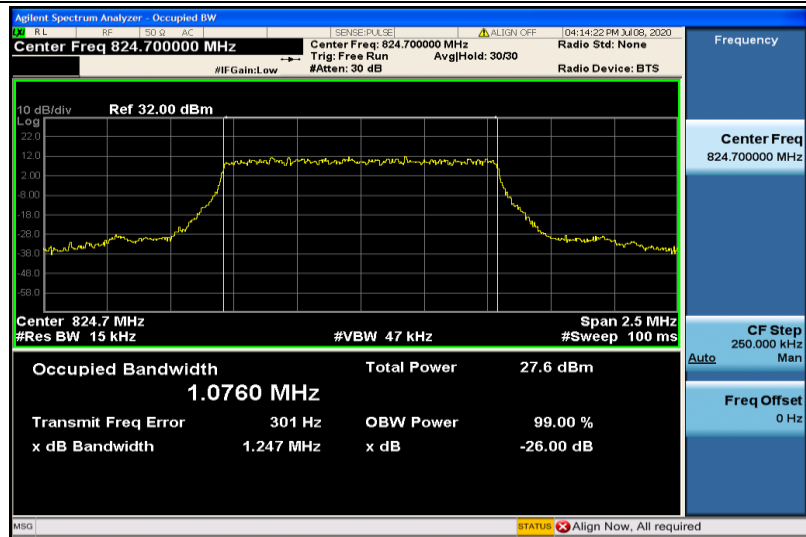
Band5-1.4MHz-QPSK-20407-6RB#0-1.0760
