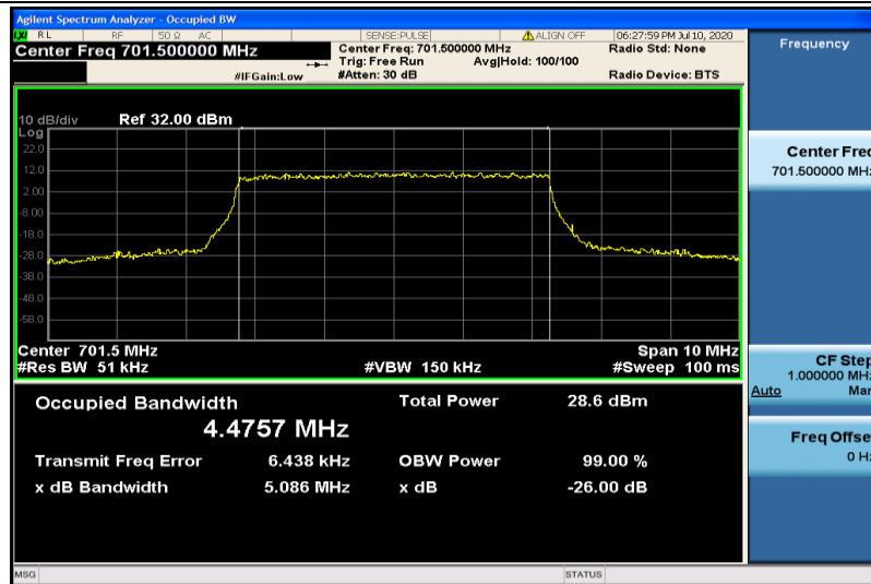
Band12-5MHz-16QAM-23035-25RB#0-4.4757
