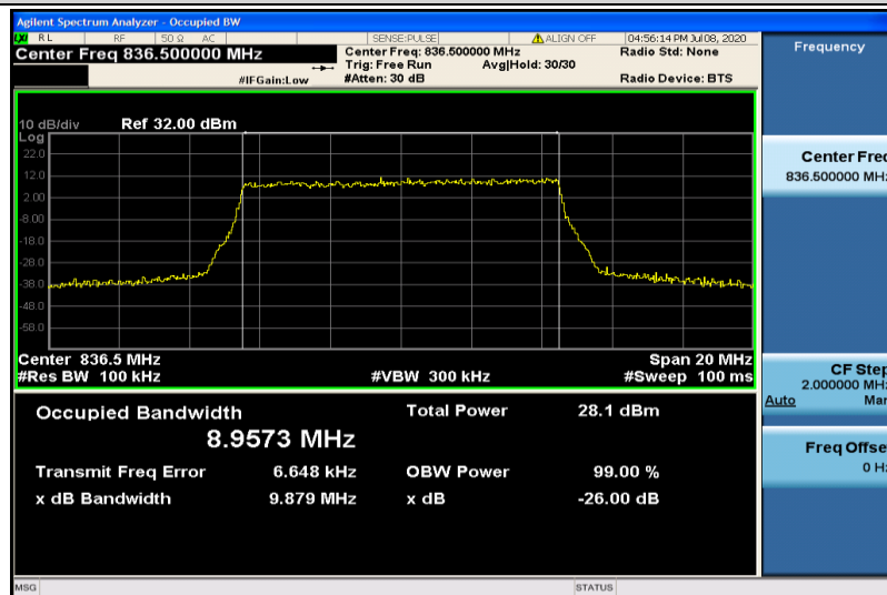
Band5-10MHz-16QAM-20525-50RB#0-8.9573
