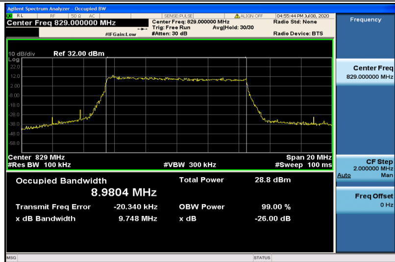
Band5-10MHz-QPSK-20450-50RB#0-8.9804
