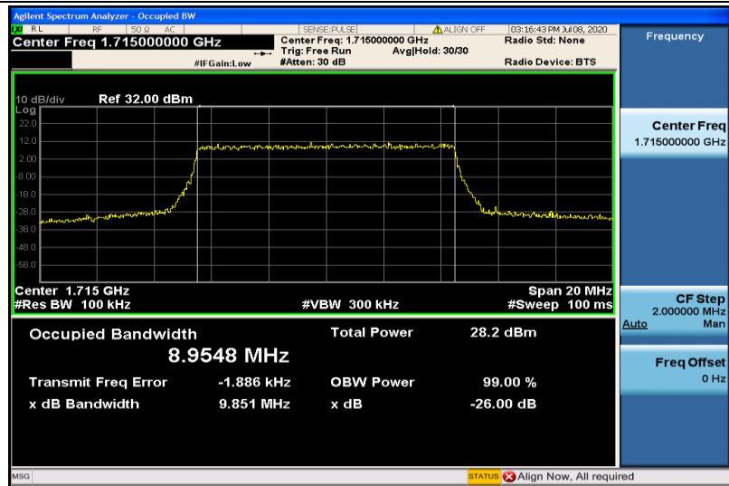
Band4-10MHz-16QAM-20000-50RB#0-8.9548
