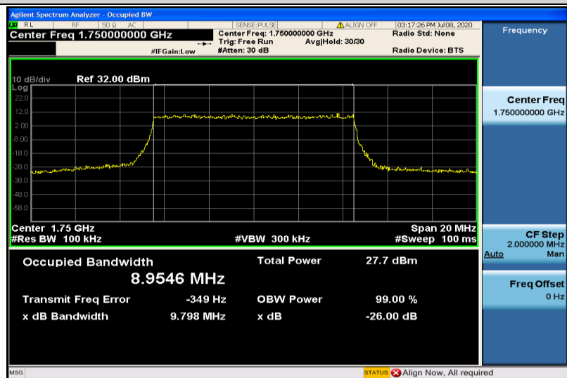
Band4-10MHz-16QAM-20350-50RB#0-8.9546
