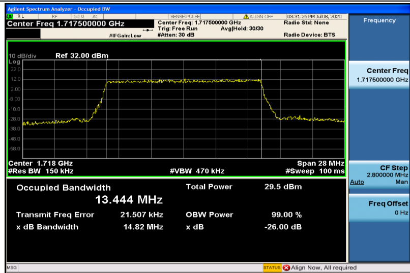
Band4-15MHz-QPSK-20025-75RB#0-13.444
