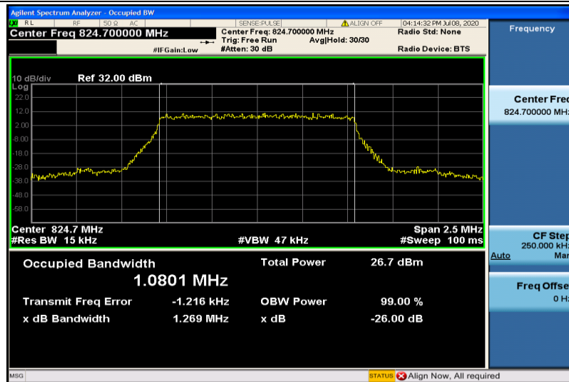
Band5-1.4MHz-16QAM-20407-6RB#0-1.0801
