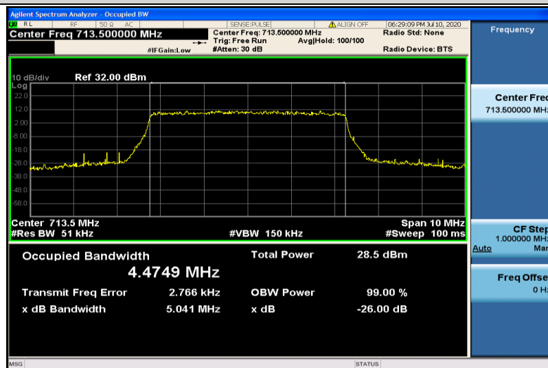
Band12-5MHz-16QAM-23155-25RB#0-4.4749
