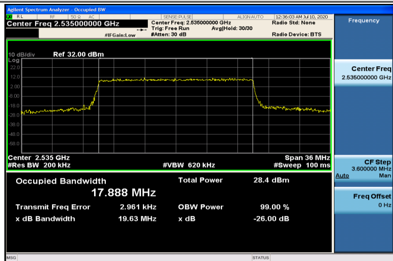
Band7-20MHz-16QAM-21100-100RB#0-17.888
