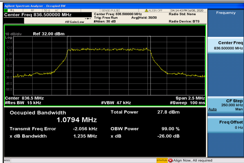
Band5-1.4MHz-QPSK-20525-6RB#0-1.0794
