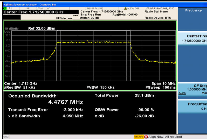
Band4-5MHz-16QAM-19975-25RB#0-4.4767
