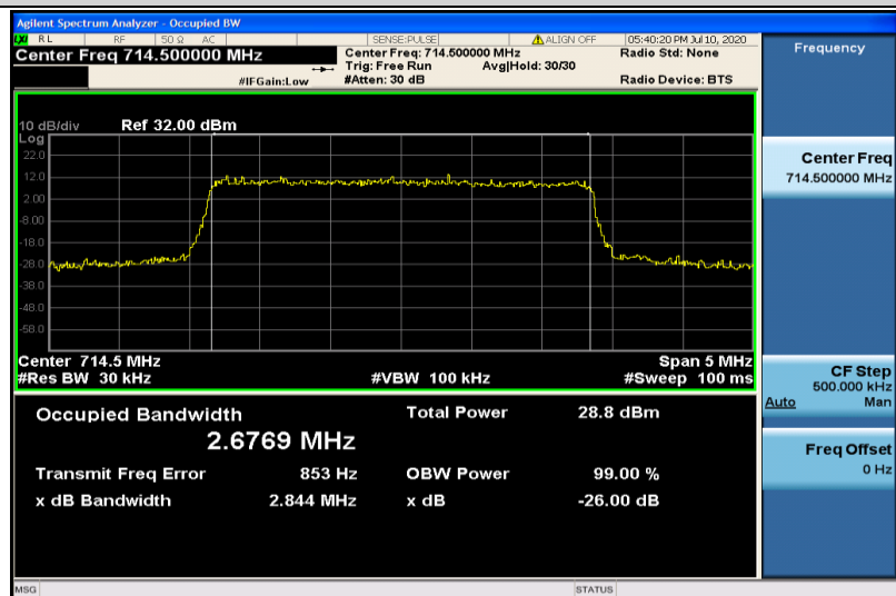
Band12-3MHz-QPSK-23165-15RB#0-2.6769
