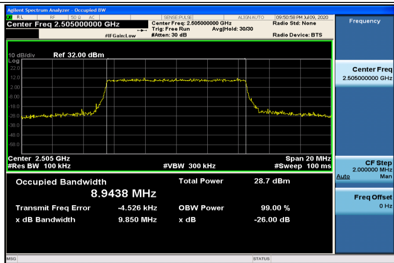
Band7-10MHz-QPSK-20800-50RB#0-8.9438
