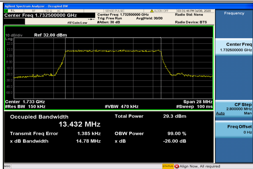
Band4-15MHz-QPSK-20175-75RB#0-13.432
