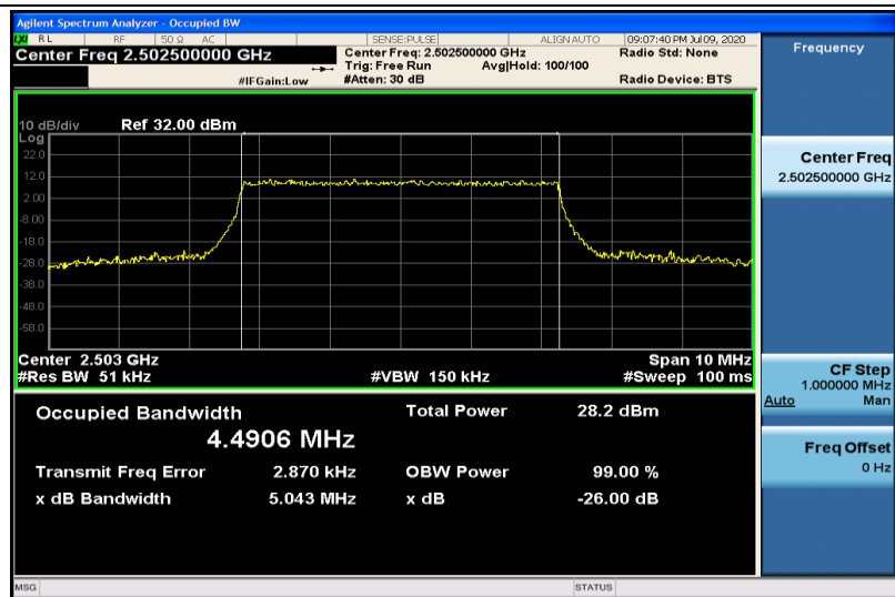
Band7-5MHz-16QAM-20775-25RB#0-4.4906
