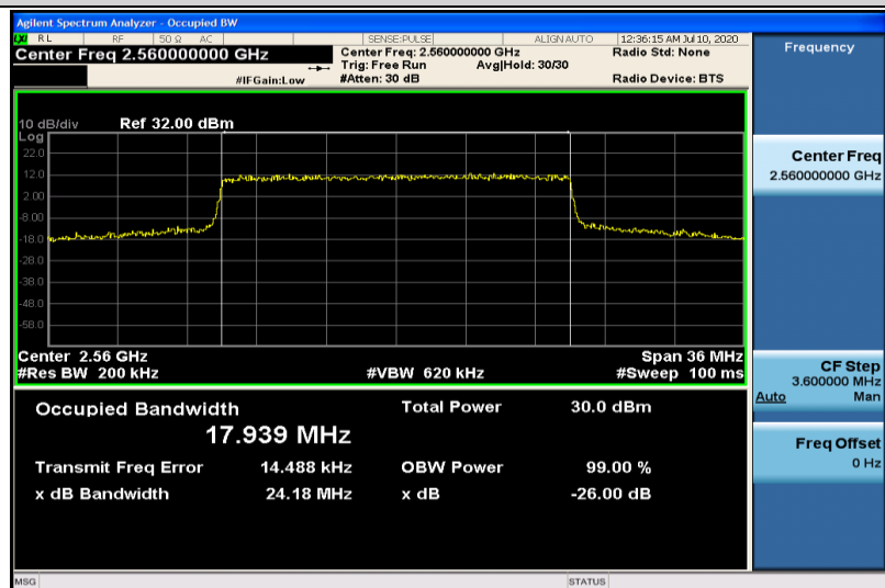
Band7-20MHz-QPSK-21350-100RB#0-17.939
