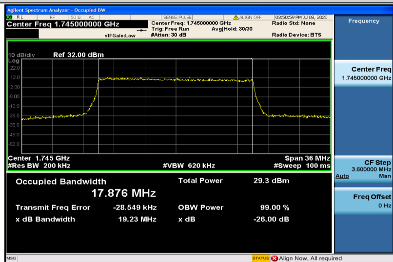
Band4-20MHz-QPSK-20300-100RB#0-17.876
