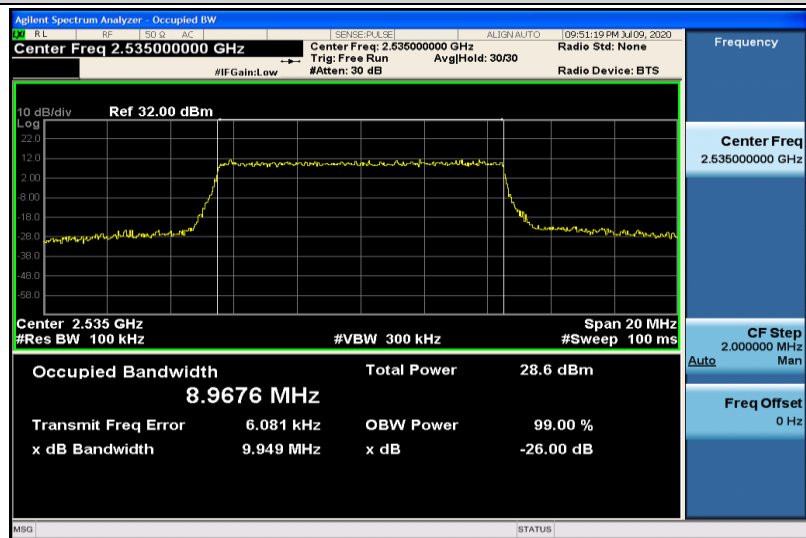
Band7-10MHz-QPSK-21100-50RB#0-8.9676
