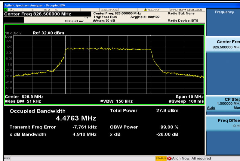
Band5-5MHz-16QAM-20425-25RB#0-4.4763
