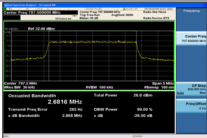
Band12-3MHz-QPSK-23095-15RB#0-2.6816
