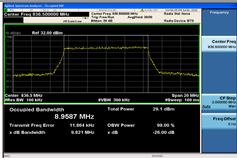
Band5-10MHz-QPSK-20525-50RB#0-8.9587
