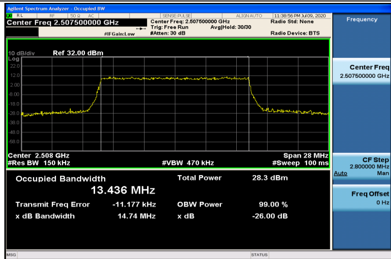
Band7-15MHz-16QAM-20825-75RB#0-13.436
