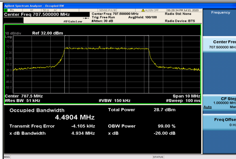
Band12-5MHz-16QAM-23095-25RB#0-4.4904
