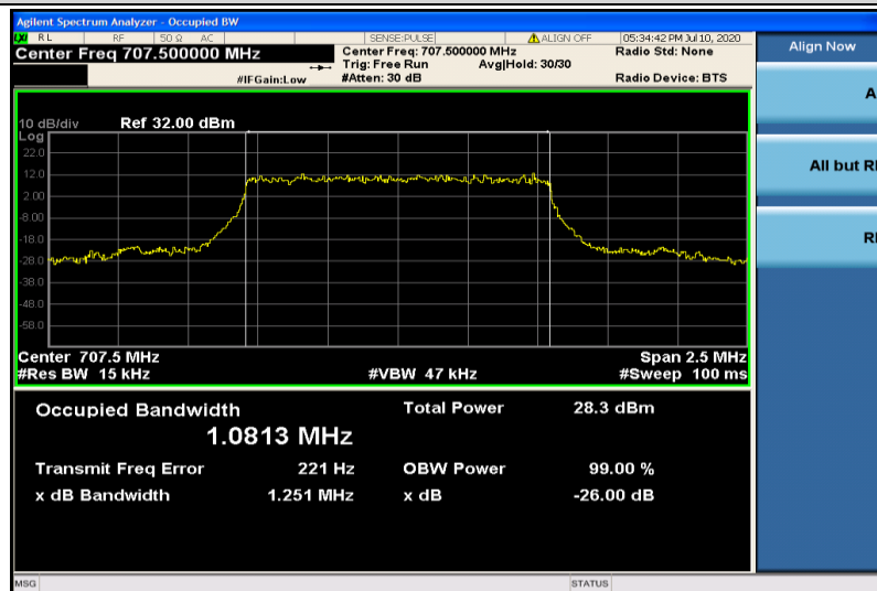
Band12-1.4MHz-QPSK-23095-6RB#0-1.0813
