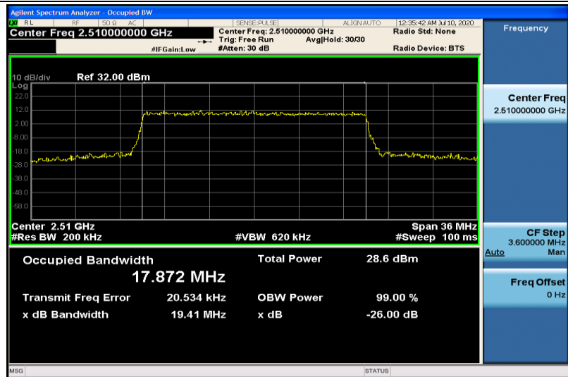
Band7-20MHz-16QAM-20850-100RB#0-17.872
