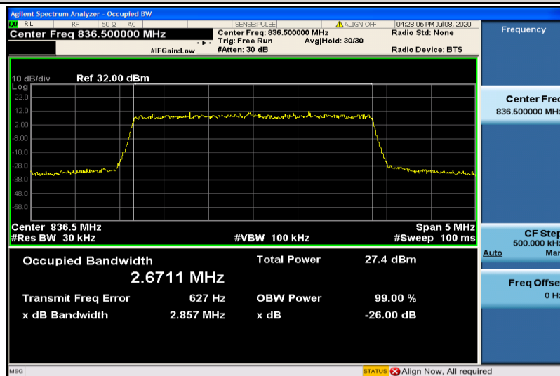
Band5-3MHz-16QAM-20525-15RB#0-2.6711
