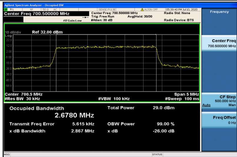
Band12-3MHz-QPSK-23025-15RB#0-2.6780
