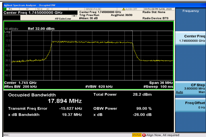
Band4-20MHz-16QAM-20300-100RB#0-17.894
