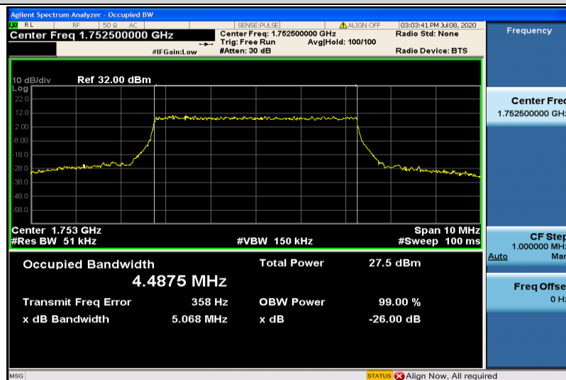
Band4-5MHz-16QAM-20375-25RB#0-4.4875
