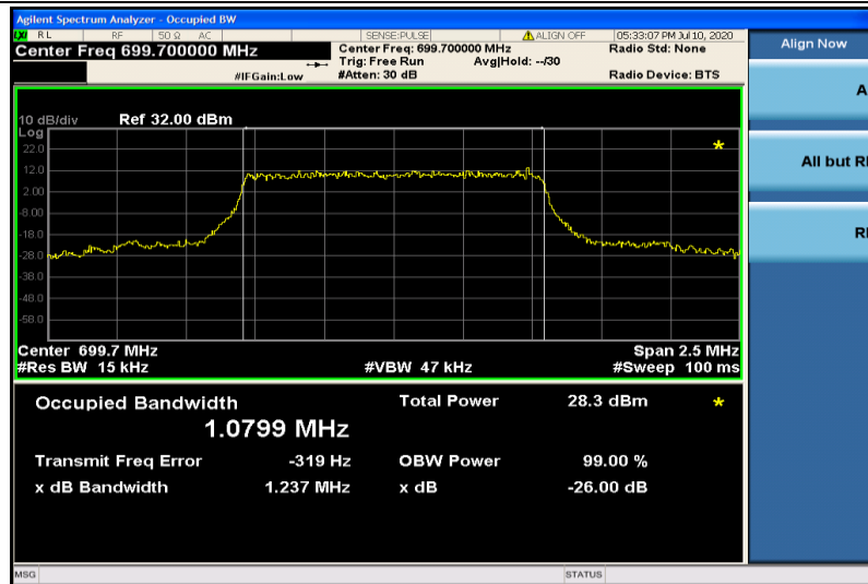
Band12-1.4MHz-QPSK-23017-6RB#0-1.0799
