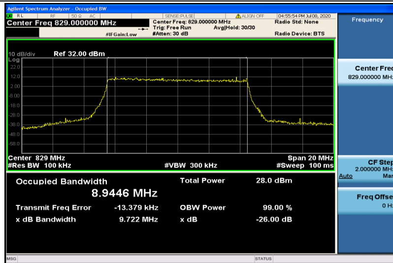
Band5-10MHz-16QAM-20450-50RB#0-8.9446
