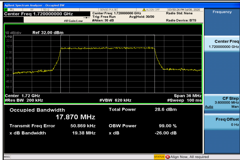
Band4-20MHz-16QAM-20050-100RB#0-17.870
