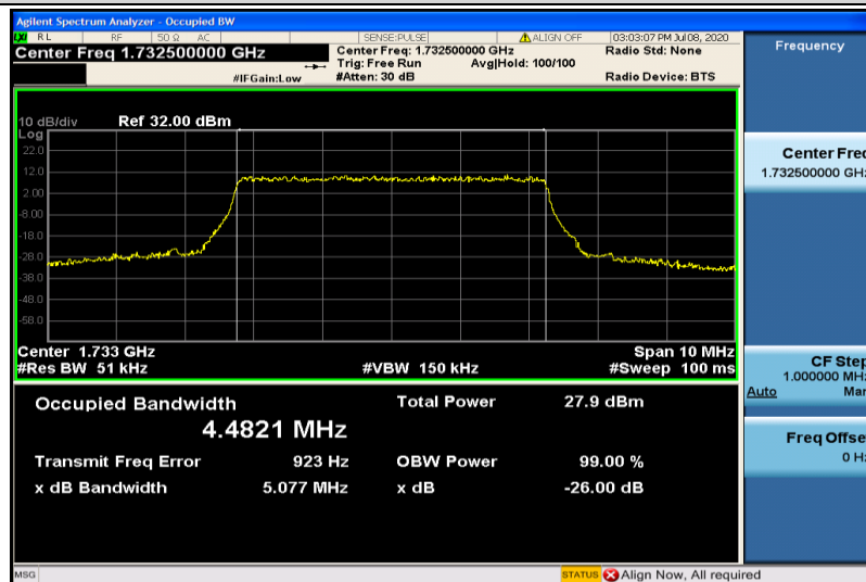
Band4-5MHz-16QAM-20175-25RB#0-4.4821
