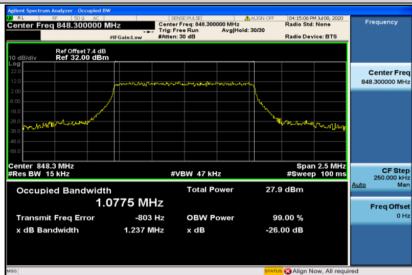
Band5-1.4MHz-QPSK-20643-6RB#0-1.0775
