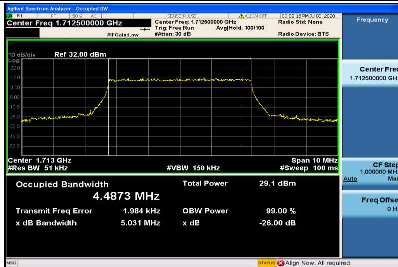
Band4-5MHz-QPSK-19975-25RB#0-4.4873
