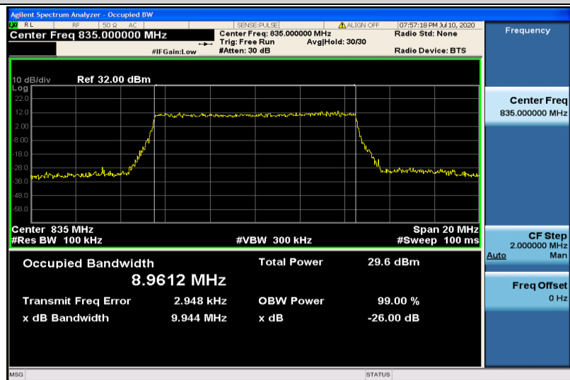
Band19-10MHz-QPSK-24050-50RB#0-8.9612
