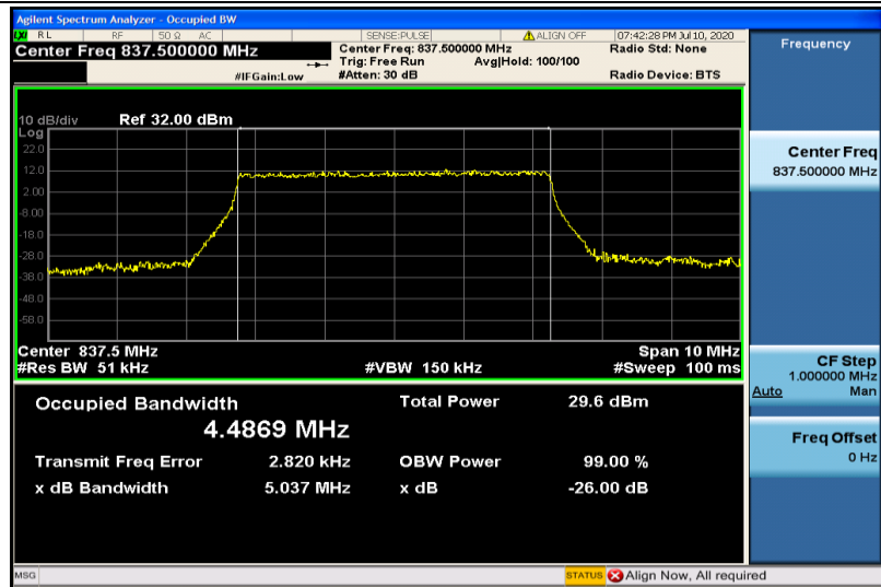
Band19-5MHz-QPSK-24075-25RB#0-4.4869
