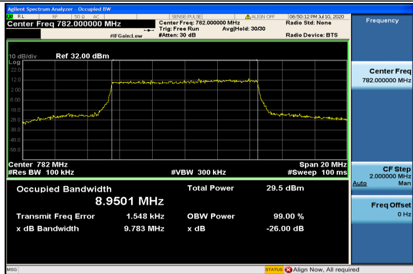
Band13-10MHz-QPSK-23230-50RB#0-8.9501
