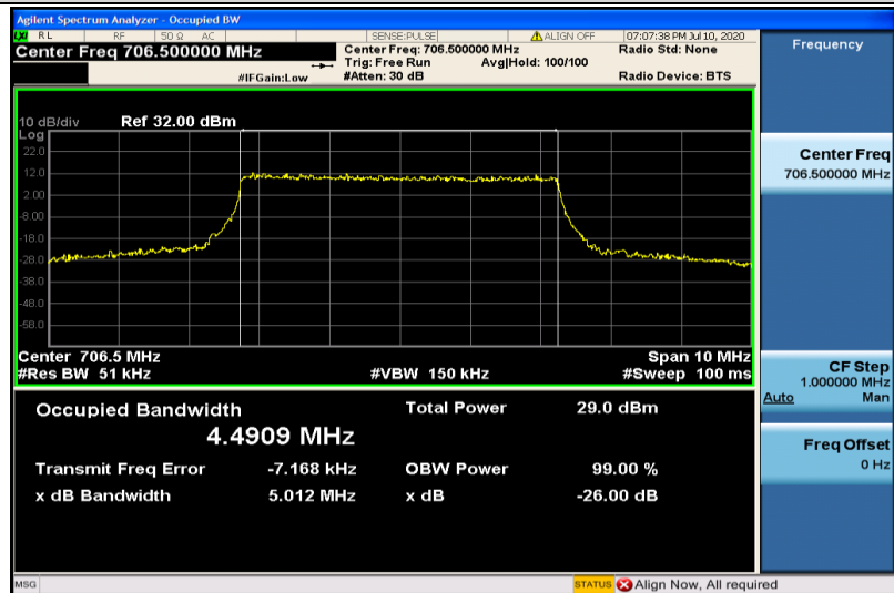
Band17-5MHz-QPSK-23755-25RB#0-4.4909
