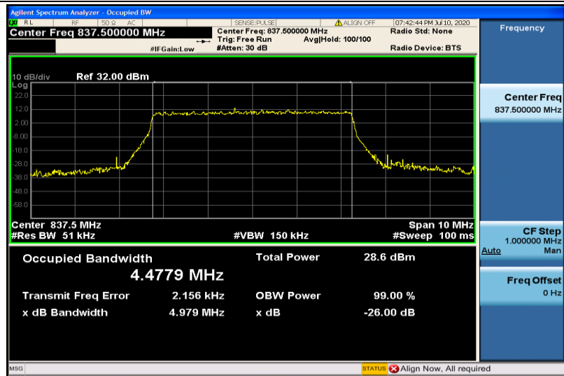
Band19-5MHz-16QAM-24075-25RB#0-4.4779
