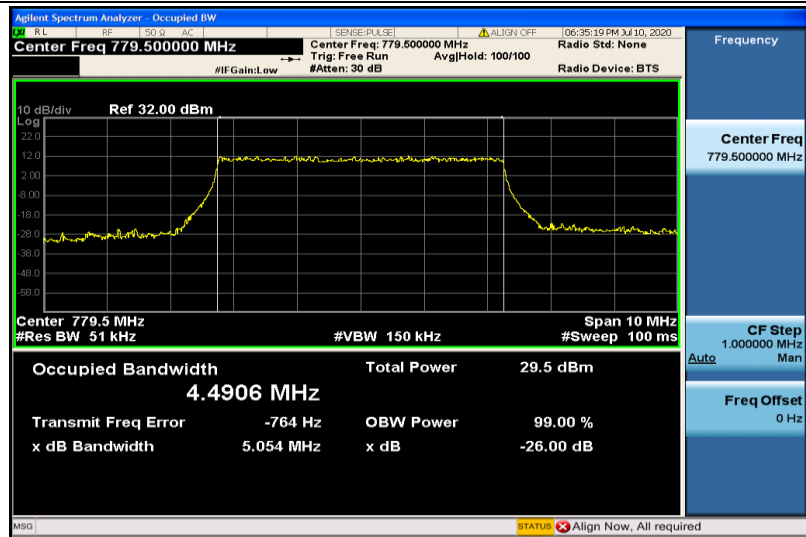
Band13-5MHz-QPSK-23205-25RB#0-4.4906
