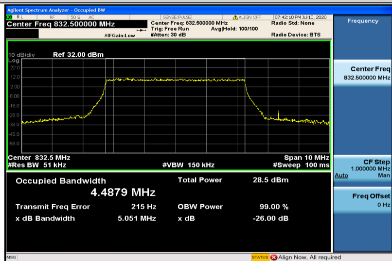
Band19-5MHz-16QAM-24025-25RB#0-4.4879
