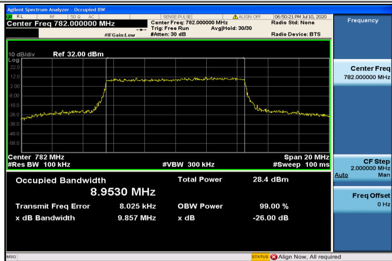
Band13-10MHz-16QAM-23230-50RB#0-8.9530
