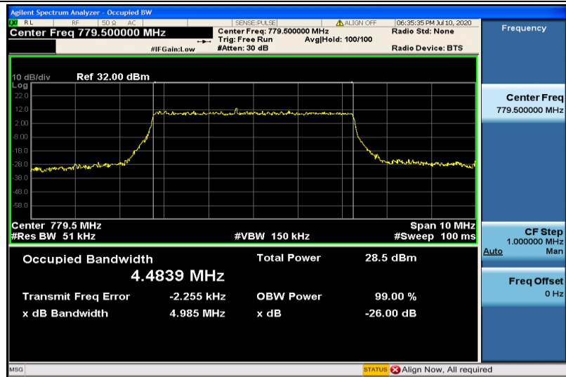
Band13-5MHz-16QAM-23205-25RB#0-4.4839
