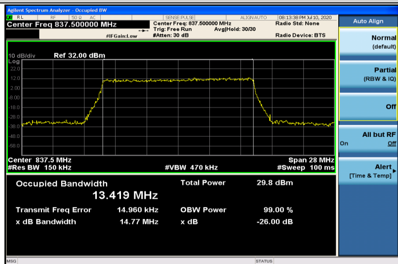
Band19-15MHz-QPSK-24075-75RB#0-13.419
