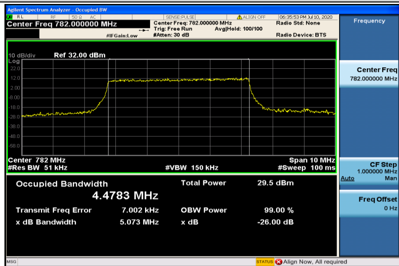
Band13-5MHz-QPSK-23230-25RB#0-4.4783
