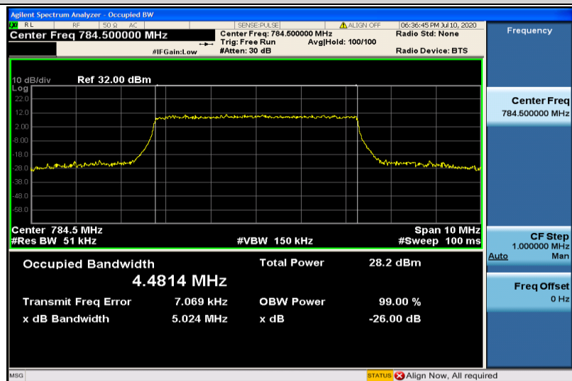
Band13-5MHz-16QAM-23255-25RB#0-4.4814
