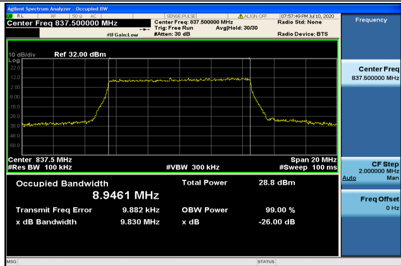
Band19-10MHz-16QAM-24075-50RB#0-8.9461
