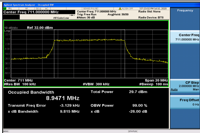
Band17-10MHz-QPSK-23800-50RB#0-8.9471
