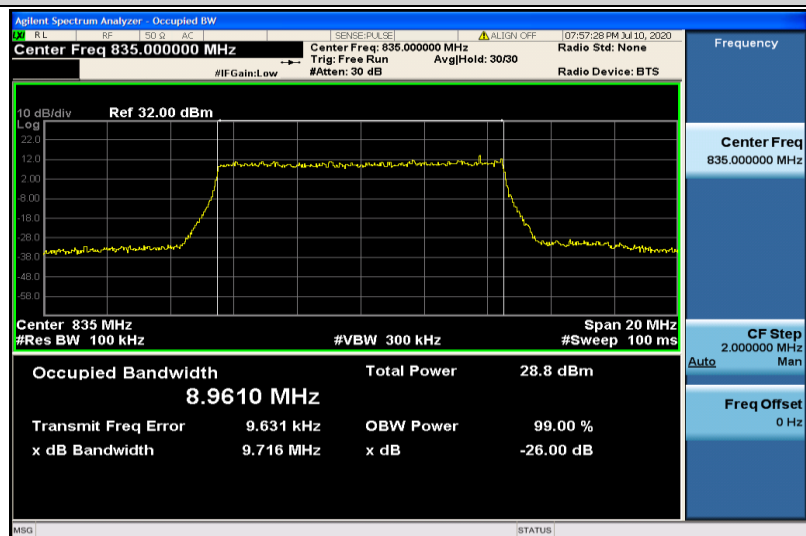
Band19-10MHz-16QAM-24050-50RB#0-8.9610
