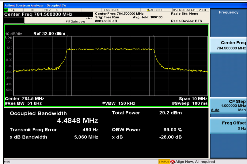
Band13-5MHz-QPSK-23255-25RB#0-4.4848
