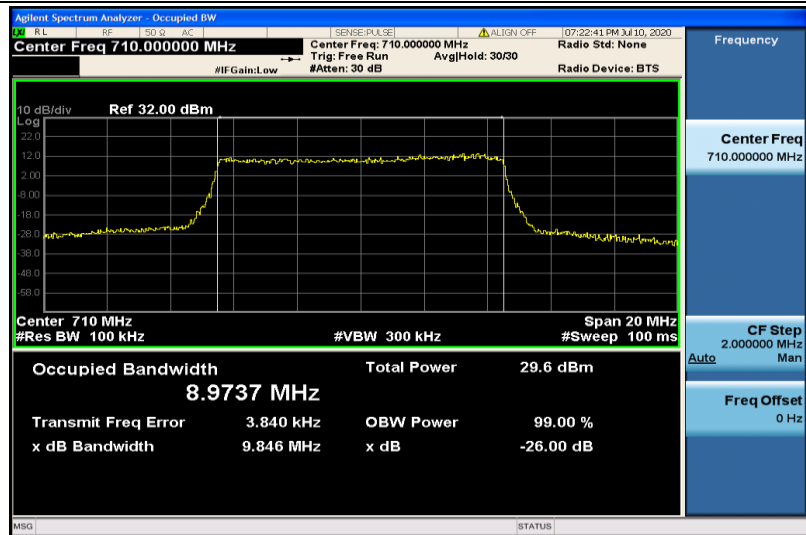
Band17-10MHz-QPSK-23790-50RB#0-8.9737
