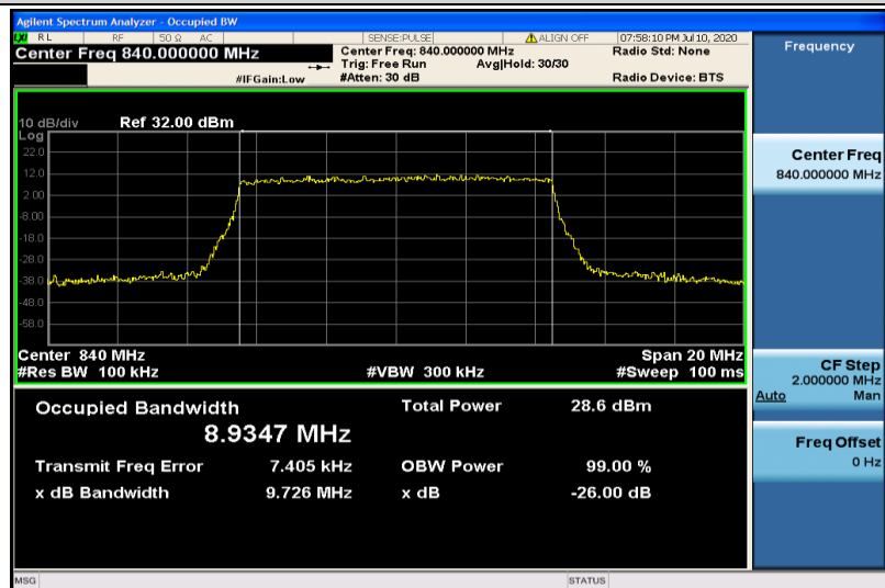
Band19-10MHz-16QAM-24100-50RB#0-8.9347
