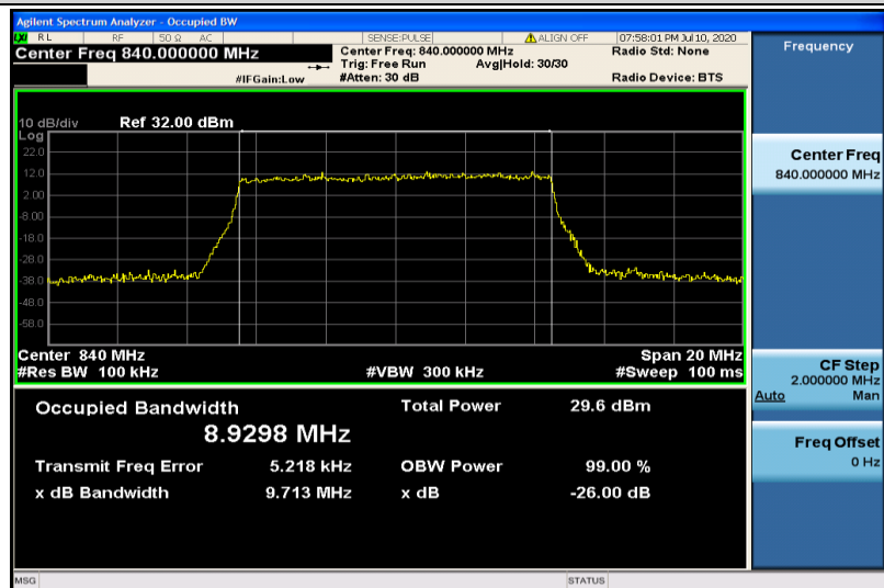
Band19-10MHz-QPSK-24100-50RB#0-8.9298
