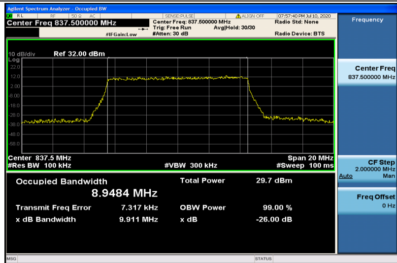
Band19-10MHz-QPSK-24075-50RB#0-8.9484
