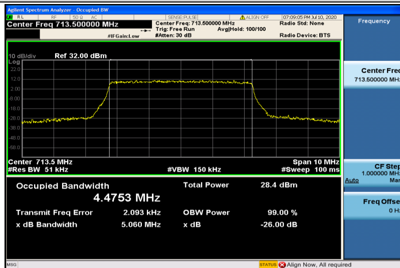
Band17-5MHz-16QAM-23825-25RB#0-4.4753
