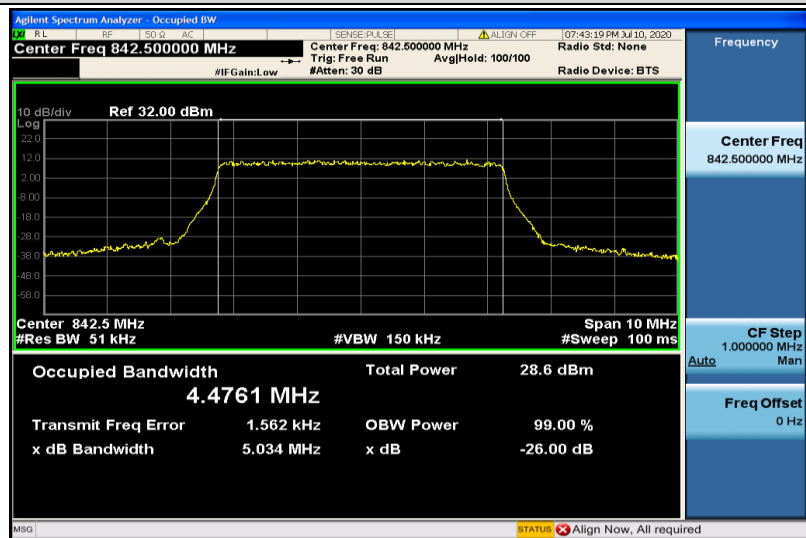
Band19-5MHz-16QAM-24125-25RB#0-4.4761
