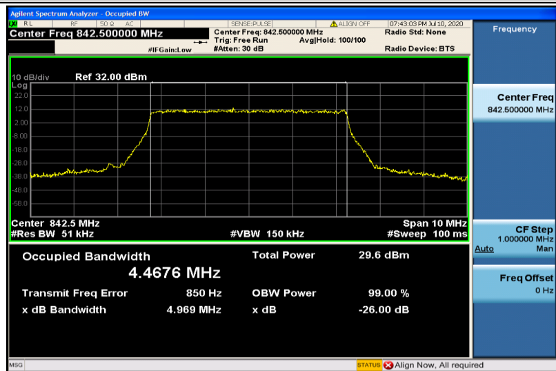
Band19-5MHz-QPSK-24125-25RB#0-4.4676
