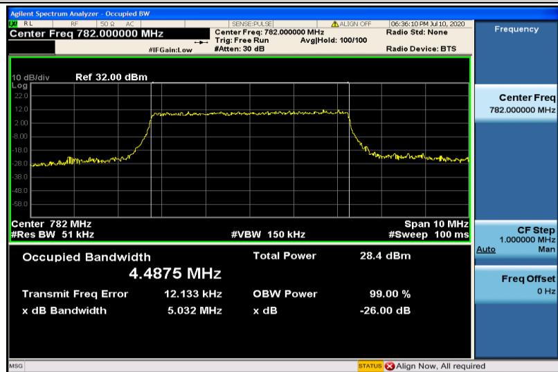
Band13-5MHz-16QAM-23230-25RB#0-4.4875
