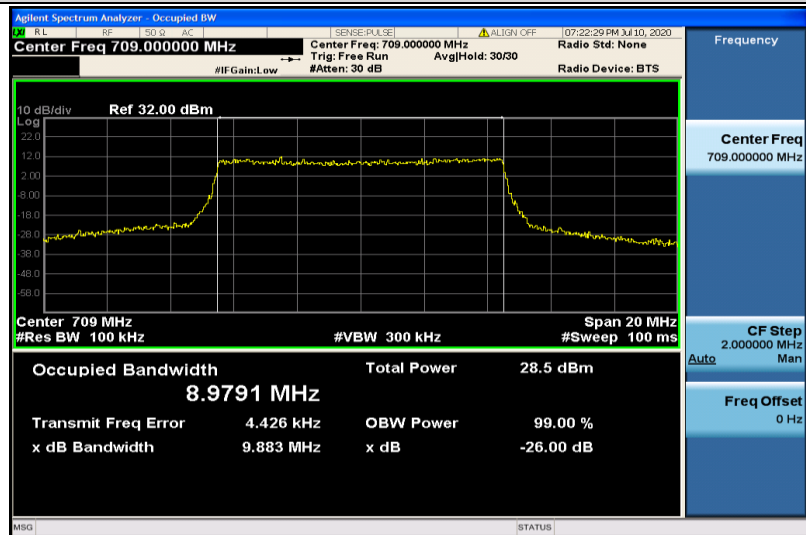
Band17-10MHz-16QAM-23780-50RB#0-8.9791
