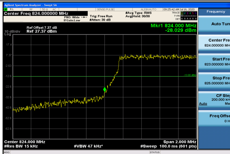
Band26-1.4MHz-16QAM-26797-6RB#0
