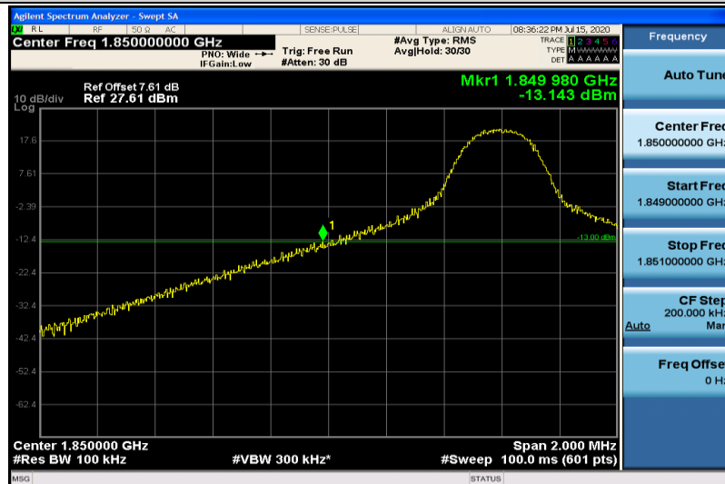
Band25-10MHz-16QAM-26090-1RB#0
