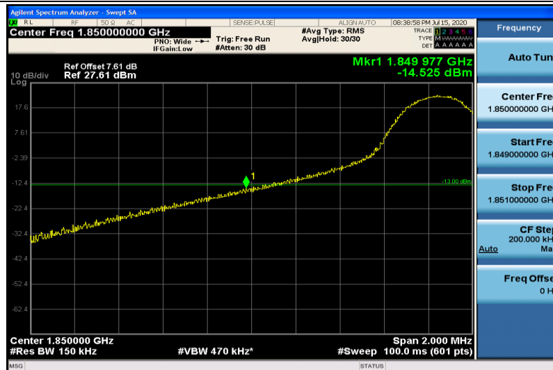
Band25-15MHz-QPSK-26115-1RB#0
