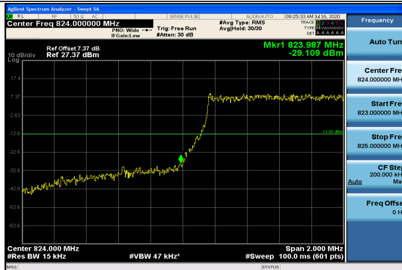
Band26-1.4MHz-QPSK-26797-6RB#0
