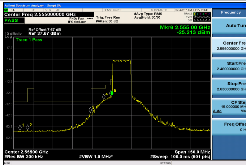
Band41-15MHz-16QAM-40315-75RB#0
