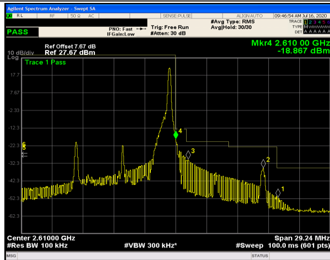
Band41-10MHz-QPSK-40740-1RB#49
