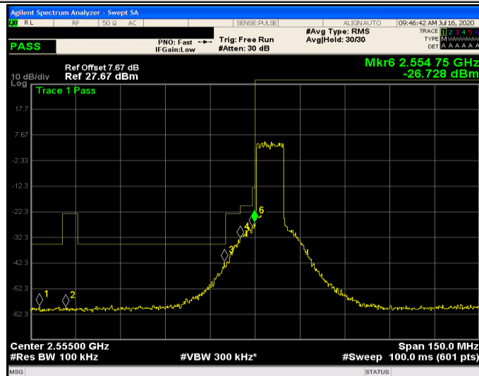
Band41-10MHz-16QAM-40290-50RB#0
