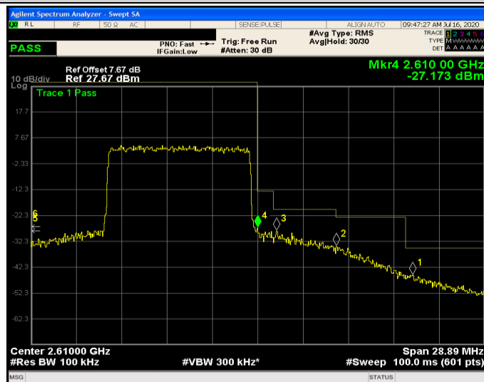
Band41-10MHz-16QAM-40740-50RB#0
