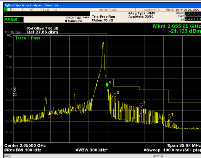
Band41-10MHz-16QAM-41190-1RB#49
