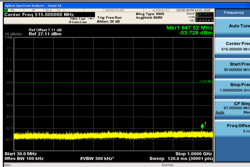
Band2-5MHz-16QAM-19175-1RB#0-30~1000MHz
