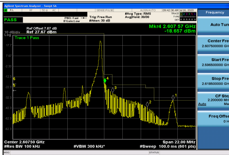
Band41-5MHz-QPSK-40740-1RB#24
