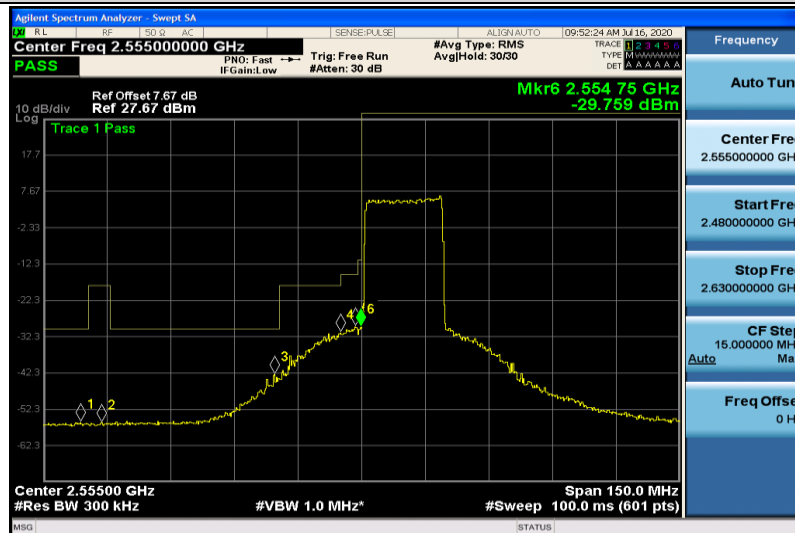
Band41-20MHz-16QAM-40340-100RB#0
