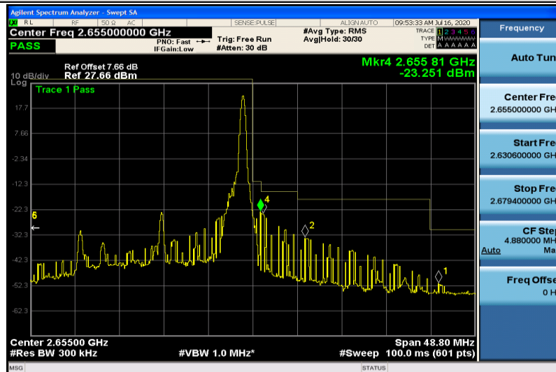
Band41-20MHz-16QAM-41140-1RB#99
