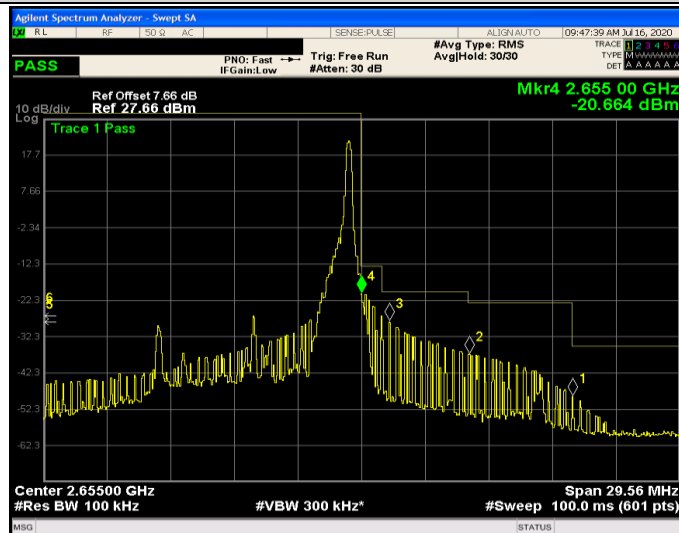
Band41-10MHz-QPSK-41190-1RB#49
