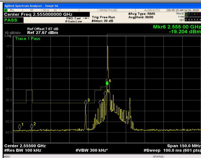
Band41-10MHz-16QAM-40290-1RB#0
