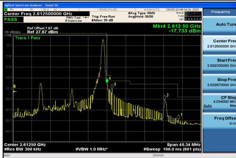
Band41-15MHz-QPSK-40740-1RB#74
