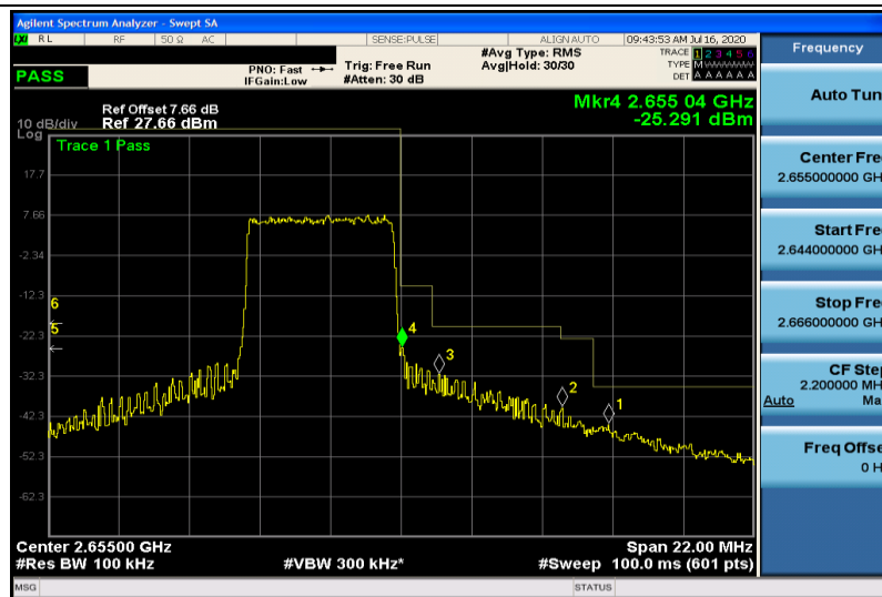
Band41-5MHz-16QAM-41215-25RB#0
