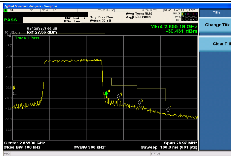
Band41-10MHz-16QAM-41190-50RB#0
