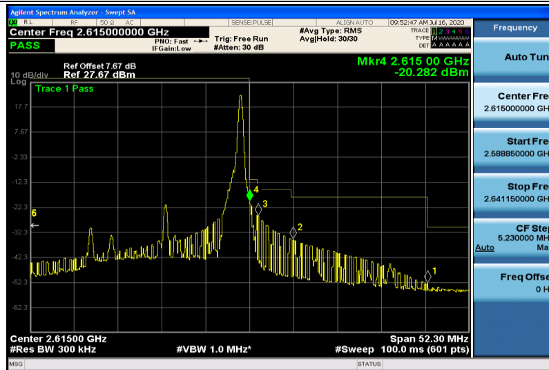
Band41-20MHz-16QAM-40740-1RB#99
