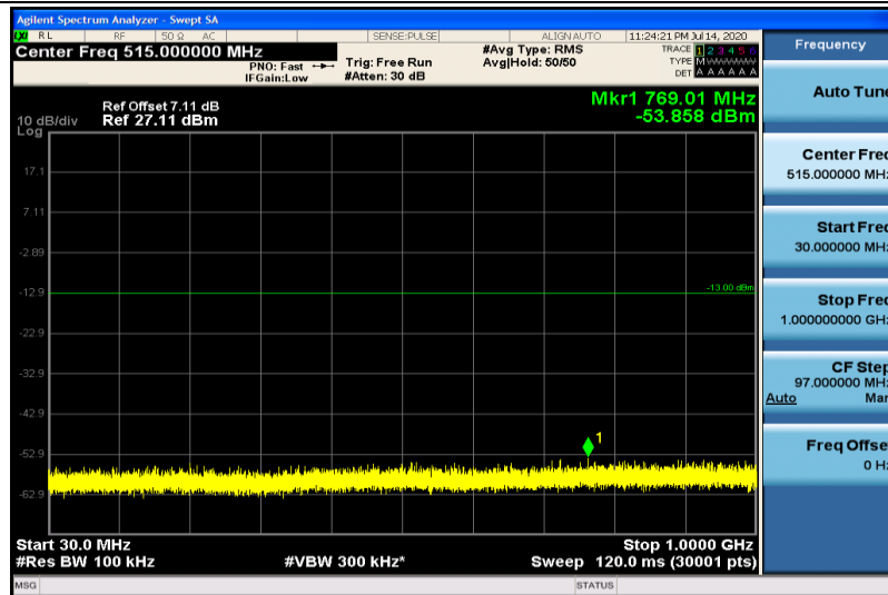
Band25-15MHz-QPSK-26615-1RB#0-30~1000MHz
