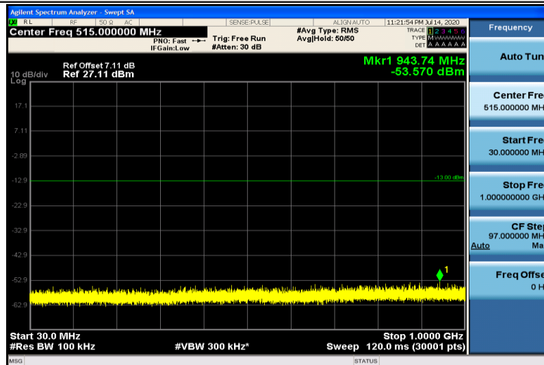
Band25-15MHz-QPSK-26115-1RB#0-30~1000MHz
