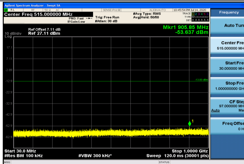
Band25-5MHz-16QAM-26065-1RB#0-30~1000MHz
