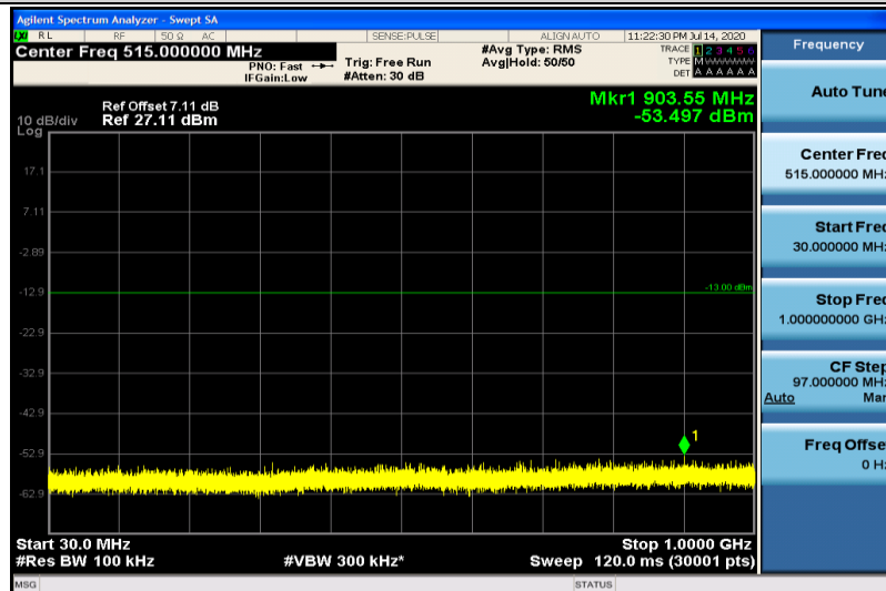
Band25-15MHz-16QAM-26115-1RB#0-30~1000MHz
