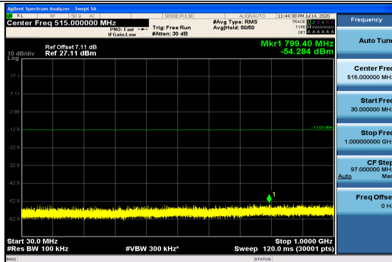
Band25-20MHz-16QAM-26140-1RB#0-30~1000MHz
