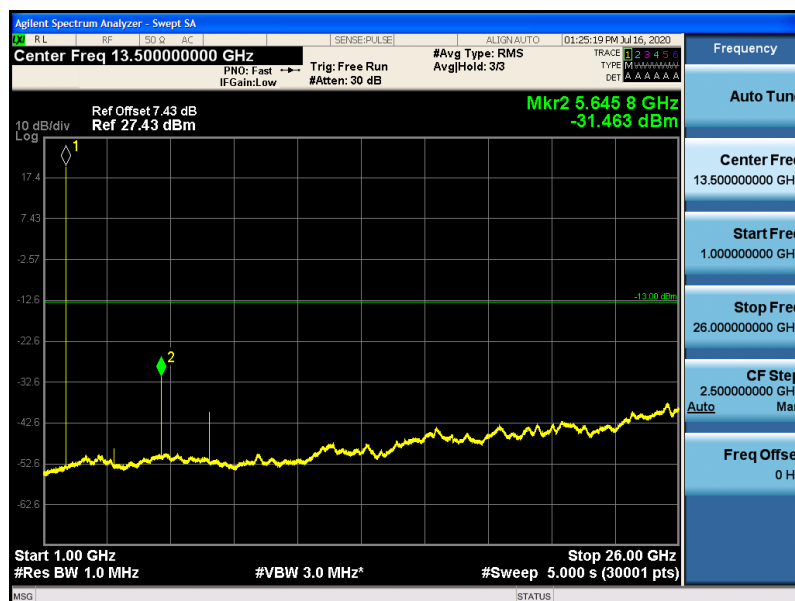
Band25-1.4MHz-16QAM-26365-1RB#0-1000~26000MHz
