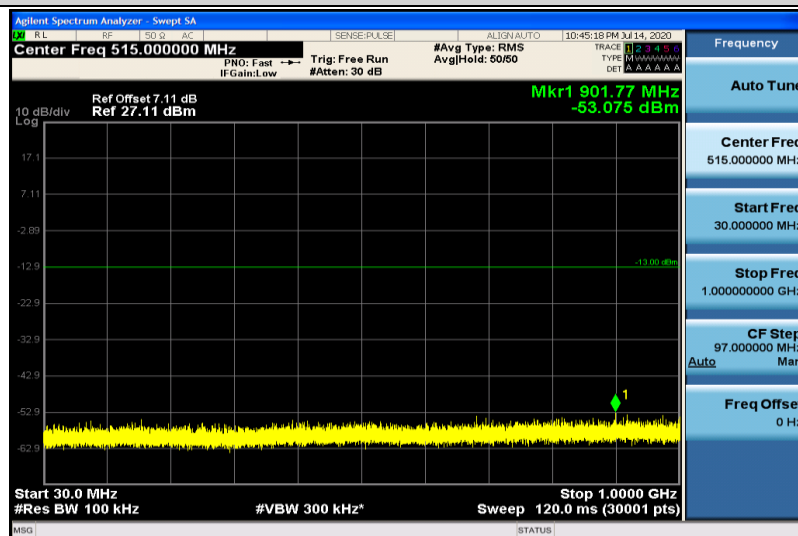
Band25-5MHz-QPSK-26065-1RB#0-30~1000MHz
