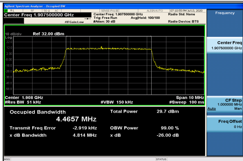
Band2-5MHz-16QAM-19175-25RB#0-4.4657
