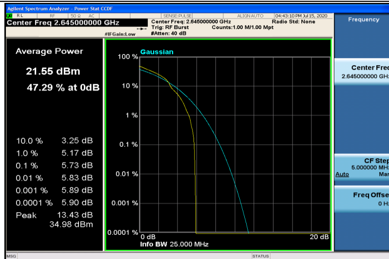
Band41-20MHz-16QAM-41140-1RB#0
