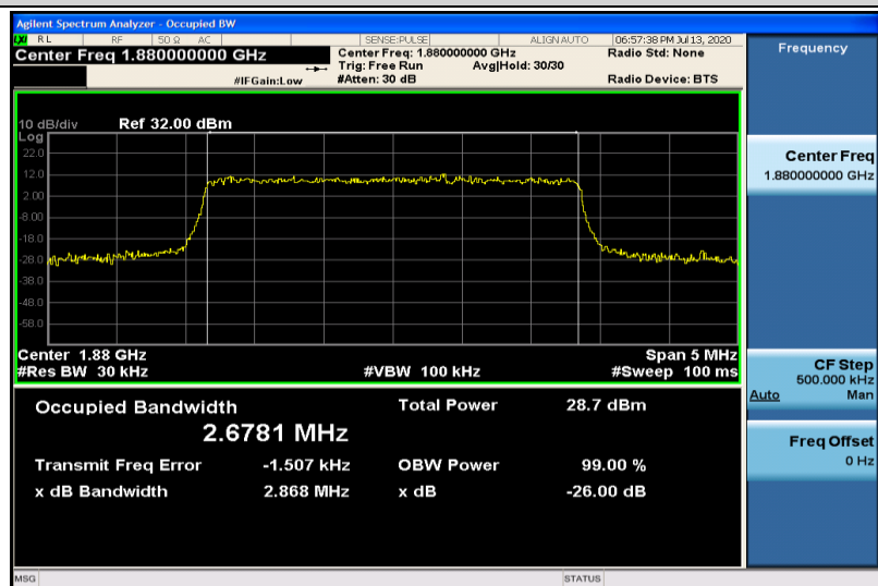
Band2-3MHz-16QAM-18900-15RB#0-2.6781
