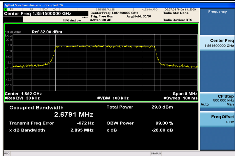
Band2-3MHz-QPSK-18615-15RB#0-2.6791
