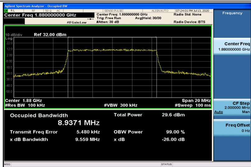
Band2-10MHz-16QAM-18900-50RB#0-8.9371
