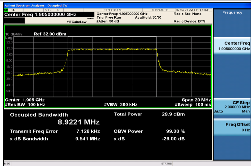
Band2-10MHz-16QAM-19150-50RB#0-8.9221
