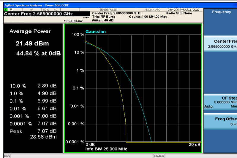
Band41-20MHz-16QAM-40340-100RB#0
