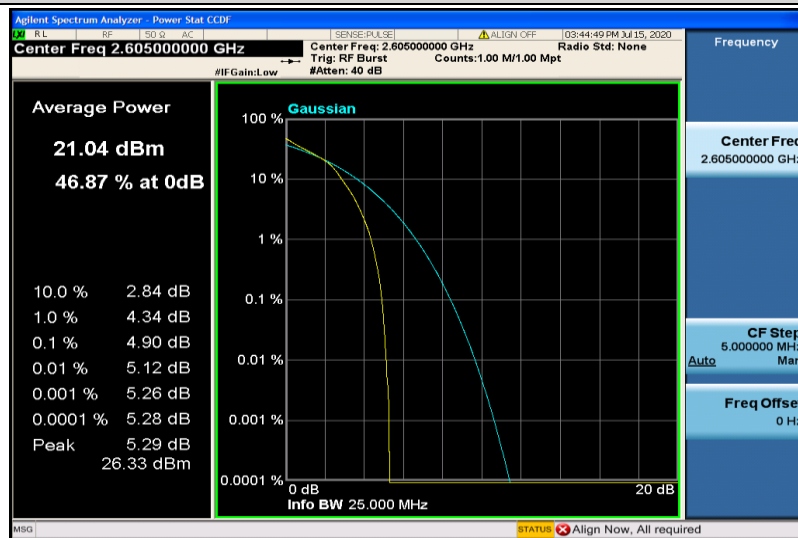
Band41-10MHz-16QAM-40740-50RB#0
