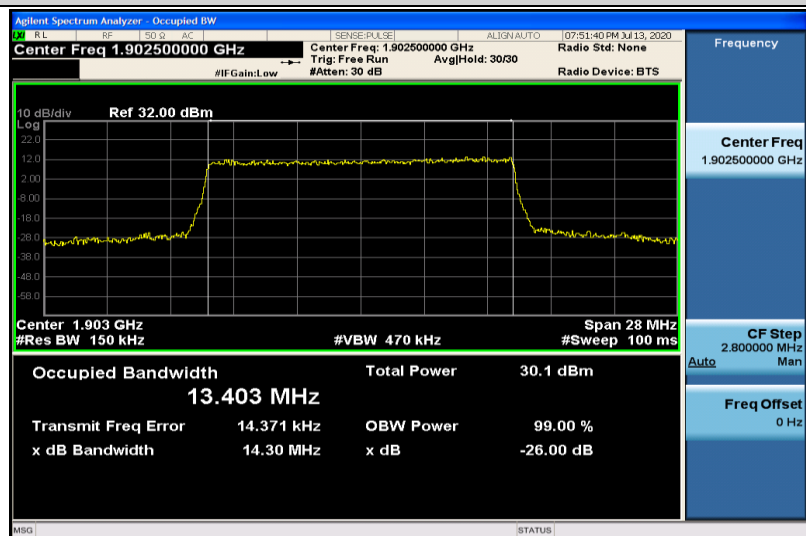
Band2-15MHz-16QAM-19125-75RB#0-13.403
