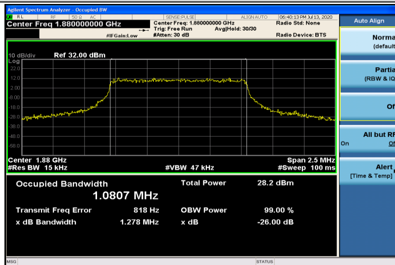
Band2-1.4MHz-16QAM-18900-6RB#0-1.0807
