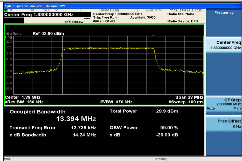
Band2-15MHz-16QAM-18900-75RB#0-13.394
