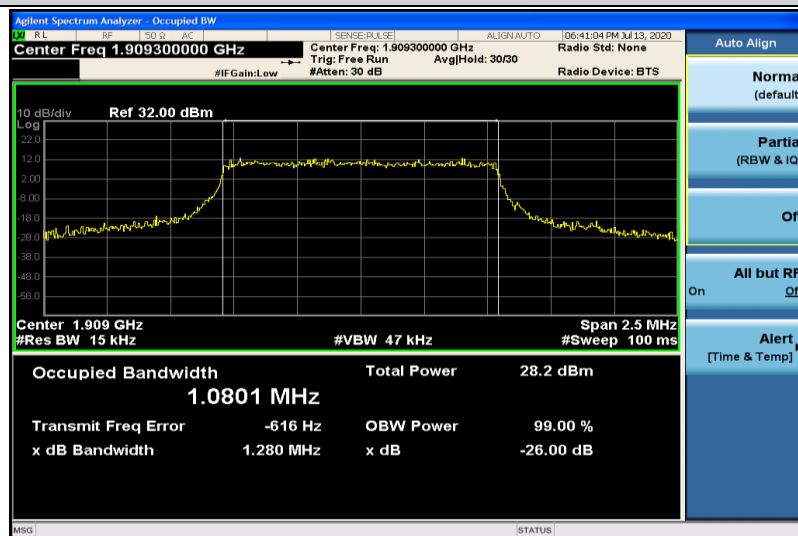
Band2-1.4MHz-16QAM-19193-6RB#0-1.0801
