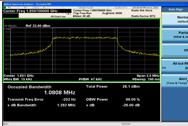
Band2-1.4MHz-16QAM-18607-6RB#0-1.0808
