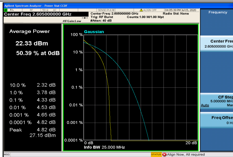
Band41-15MHz-QPSK-40740-75RB#0
