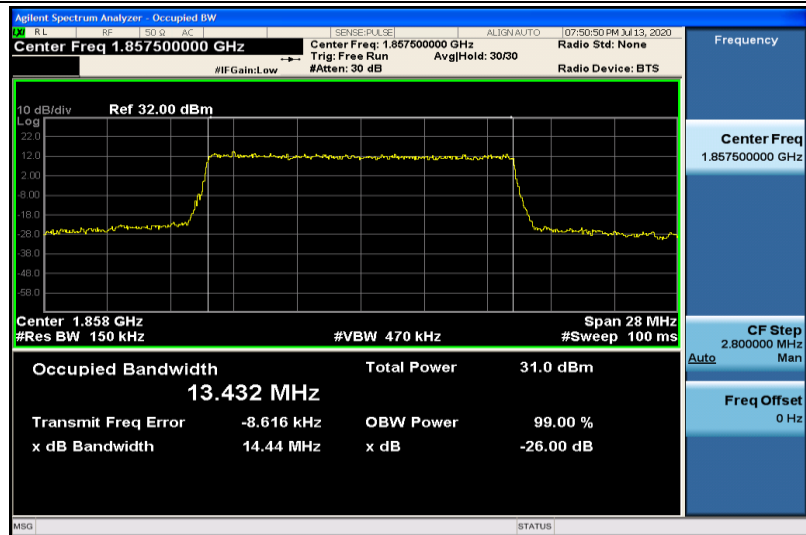
Band2-15MHz-QPSK-18675-75RB#0-13.432
