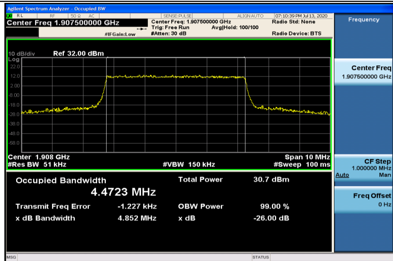
Band2-5MHz-QPSK-19175-25RB#0-4.4723
