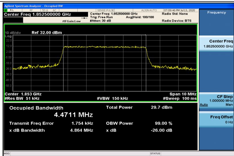
Band2-5MHz-16QAM-18625-25RB#0-4.4711
