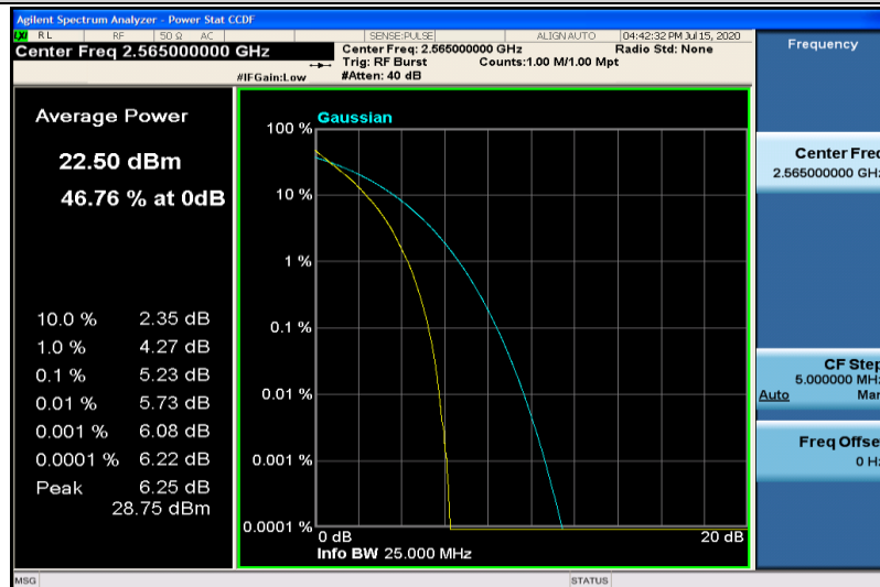
Band41-20MHz-QPSK-40340-100RB#0
