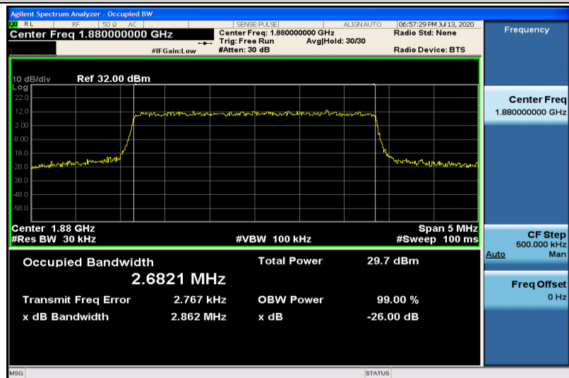
Band2-3MHz-QPSK-18900-15RB#0-2.6821
