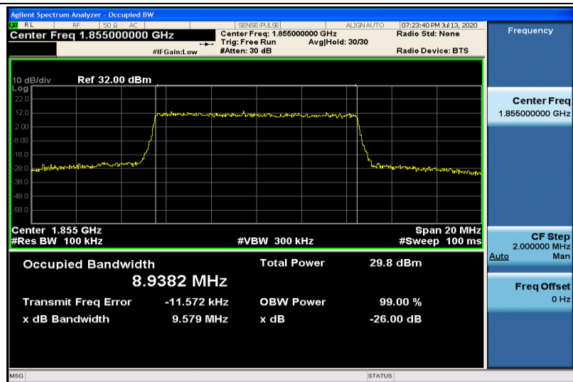
Band2-10MHz-16QAM-18650-50RB#0-8.9382
