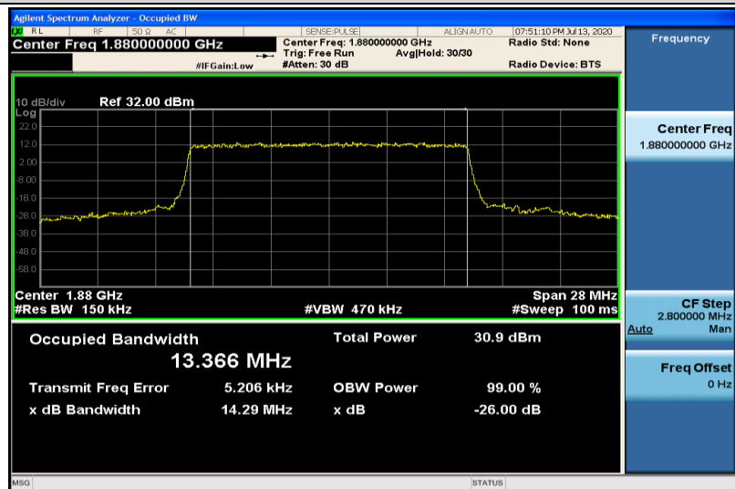
Band2-15MHz-QPSK-18900-75RB#0-13.366
