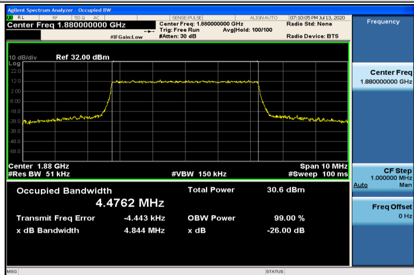
Band2-5MHz-QPSK-18900-25RB#0-4.4762
