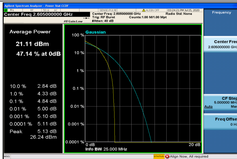
Band41-5MHz-16QAM-40740-25RB#0
