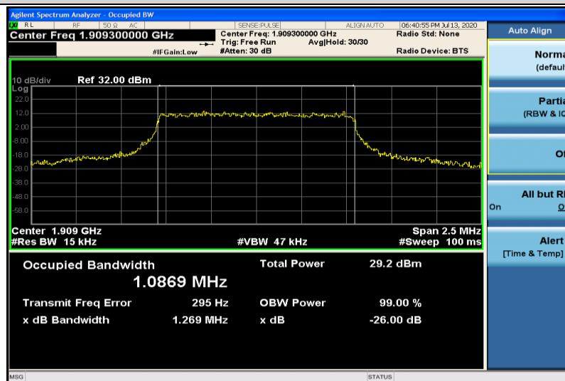
Band2-1.4MHz-QPSK-19193-6RB#0-1.0869
