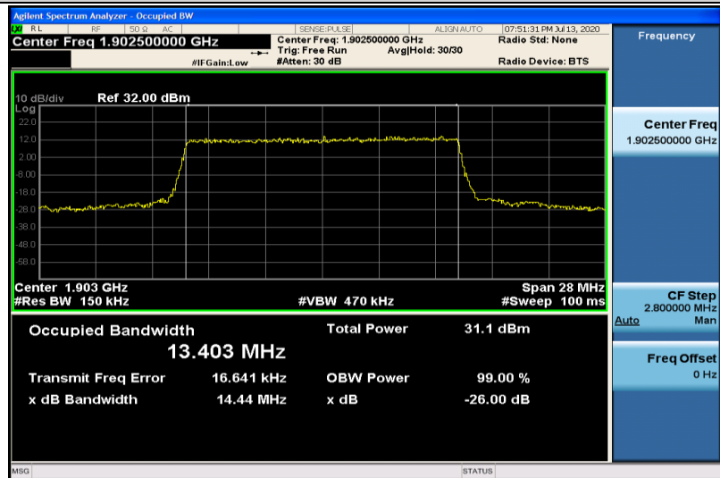
Band2-15MHz-QPSK-19125-75RB#0-13.403
