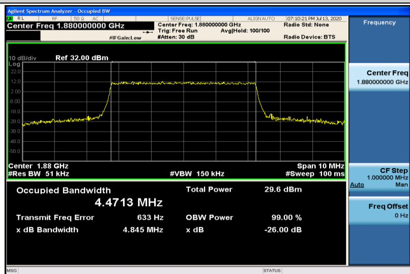
Band2-5MHz-16QAM-18900-25RB#0-4.4713
