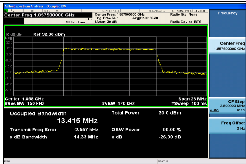
Band2-15MHz-16QAM-18675-75RB#0-13.415
