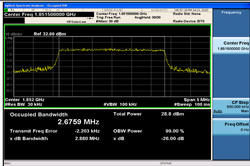
Band2-3MHz-16QAM-18615-15RB#0-2.6759
