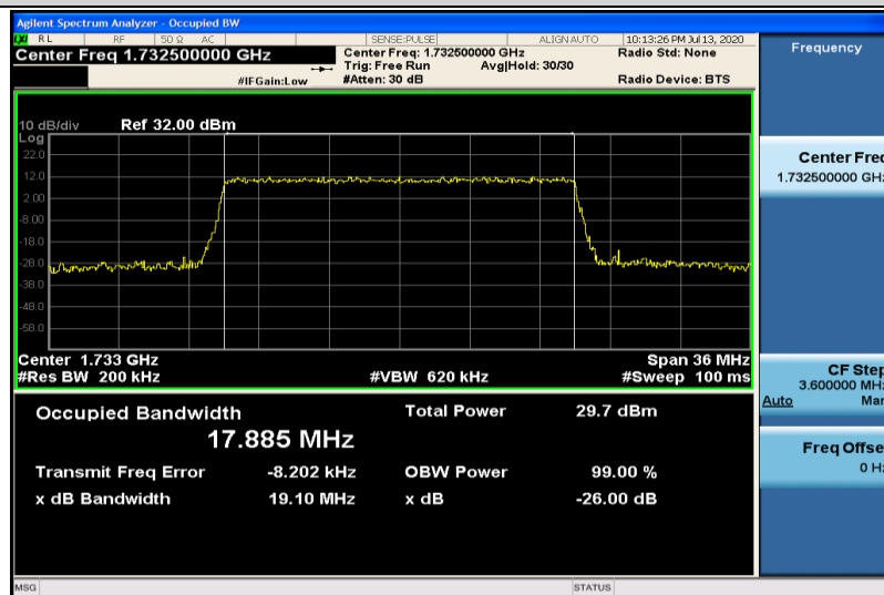
Band4-20MHz-QPSK-20175-100RB#0-17.885
