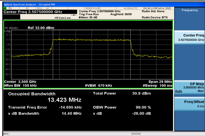
Band7-15MHz-QPSK-20825-75RB#0-13.423
