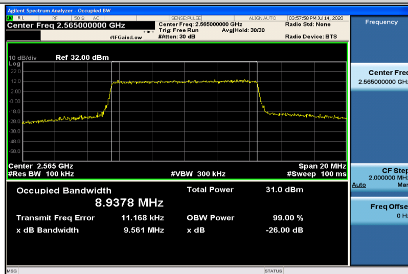
Band7-10MHz-QPSK-21400-50RB#0-8.9378
