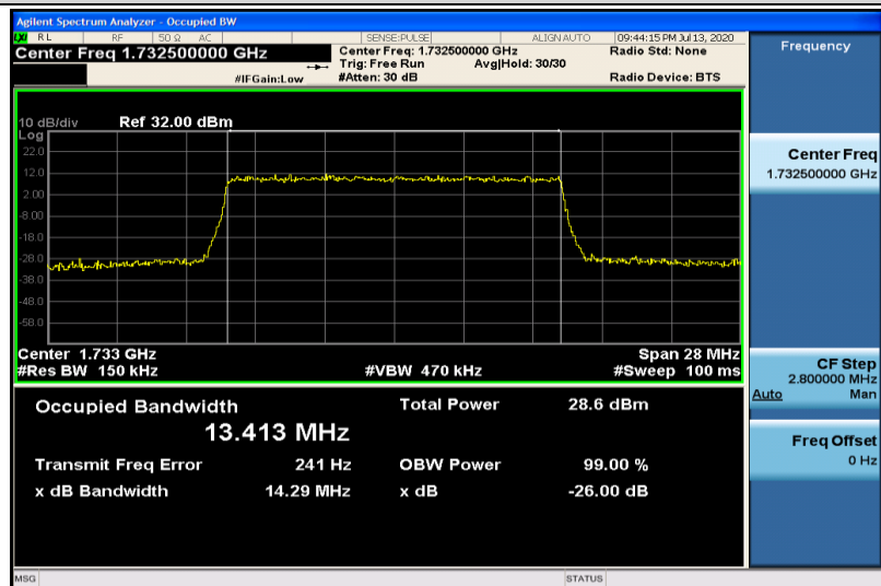
Band4-15MHz-16QAM-20175-75RB#0-13.413
