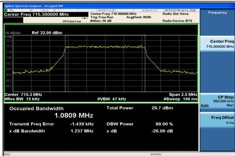
Band12-1.4MHz-QPSK-23173-6RB#0-1.0809
