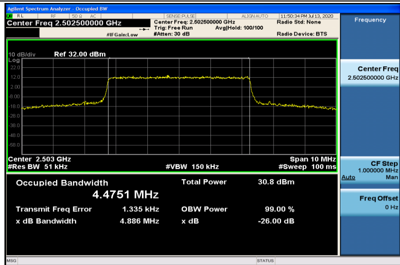
Band7-5MHz-QPSK-20775-25RB#0-4.4751
