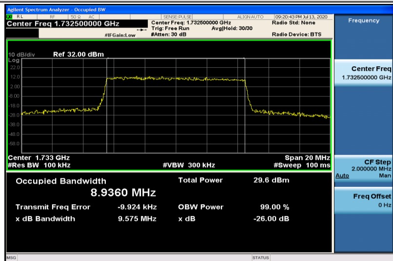
Band4-10MHz-16QAM-20175-50RB#0-8.9360
