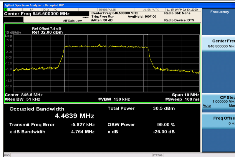
Band5-5MHz-16QAM-20625-25RB#0-4.4639
