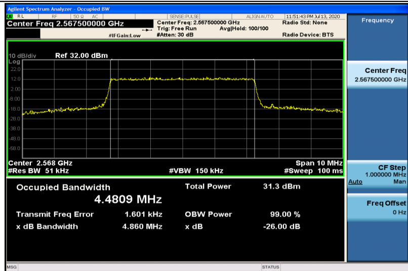
Band7-5MHz-QPSK-21425-25RB#0-4.4809
