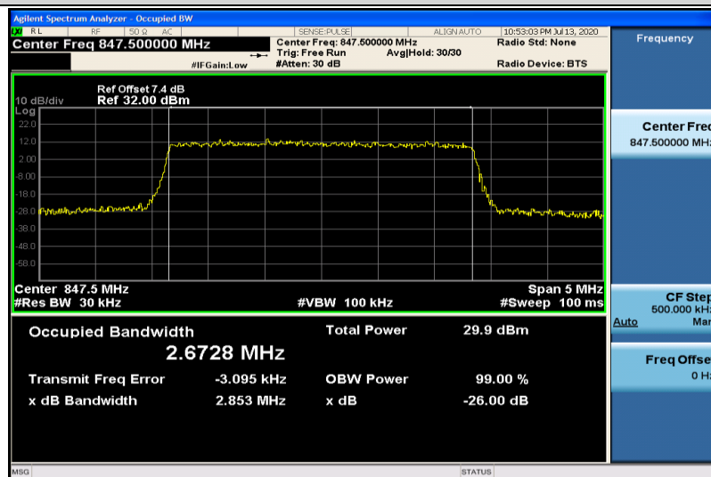
Band5-3MHz-16QAM-20635-15RB#0-2.6728
