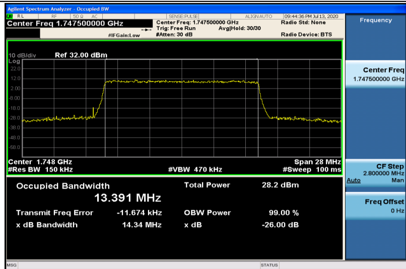
Band4-15MHz-16QAM-20325-75RB#0-13.391
