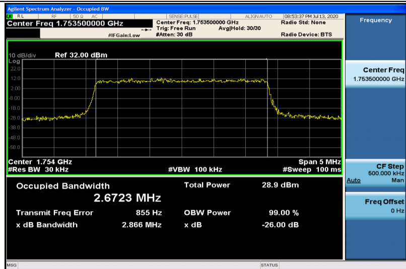
Band4-3MHz-16QAM-20385-15RB#0-2.6723
