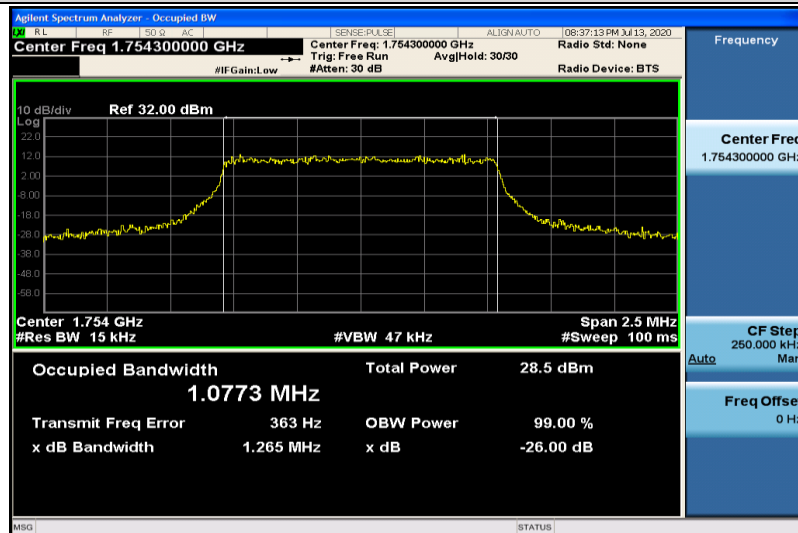
Band4-1.4MHz-16QAM-20393-6RB#0-1.0773
