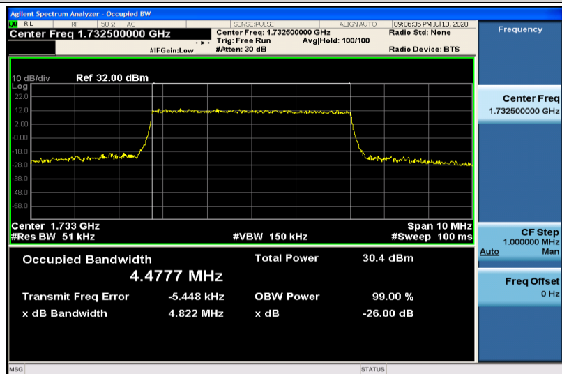
Band4-5MHz-QPSK-20175-25RB#0-4.4777
