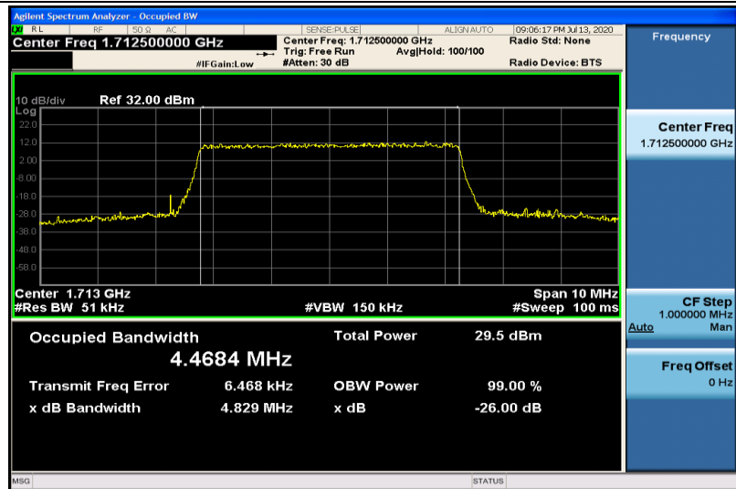
Band4-5MHz-16QAM-19975-25RB#0-4.4684
