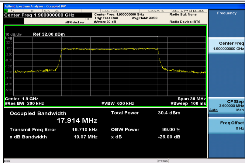
Band2-20MHz-16QAM-19100-100RB#0-17.914
