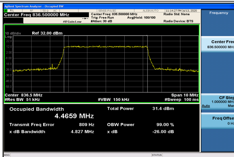
Band5-5MHz-QPSK-20525-25RB#0-4.4659
