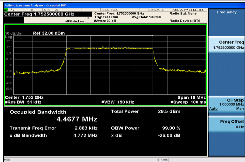
Band4-5MHz-16QAM-20375-25RB#0-4.4677
