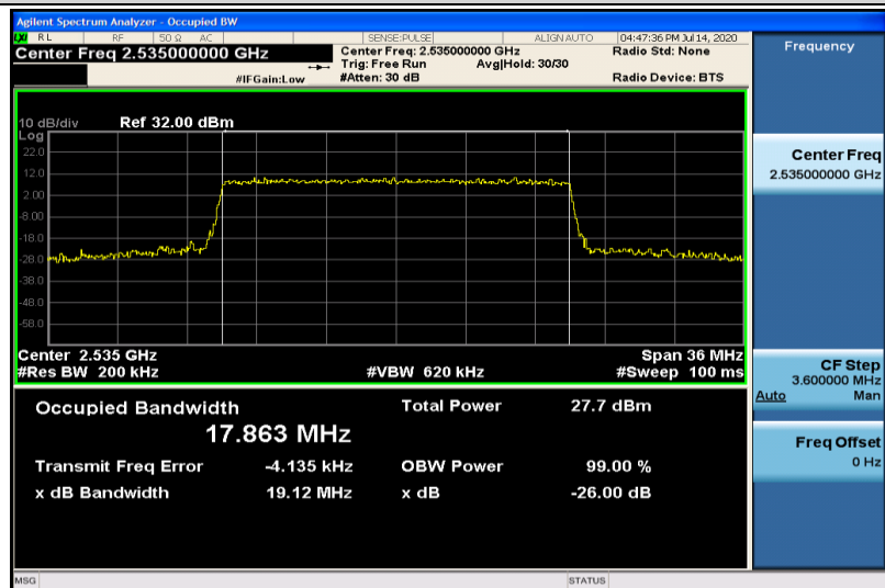
Band7-20MHz-16QAM-21100-100RB#0-17.863
