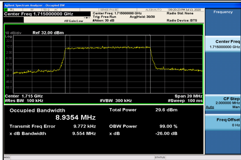
Band4-10MHz-16QAM-20000-50RB#0-8.9354
