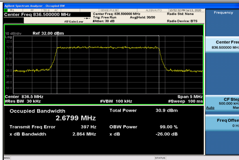
Band5-3MHz-QPSK-20525-15RB#0-2.6799
