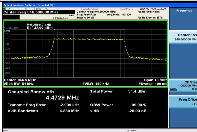
Band5-5MHz-QPSK-20625-25RB#0-4.4729
