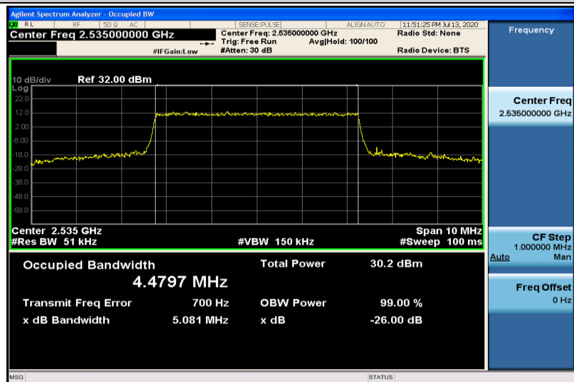
Band7-5MHz-16QAM-21100-25RB#0-4.4797
