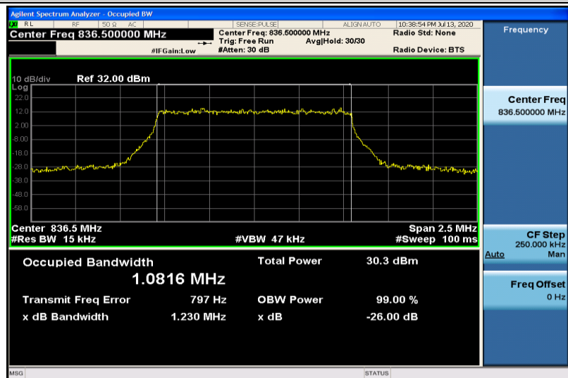
Band5-1.4MHz-QPSK-20525-6RB#0-1.0816
