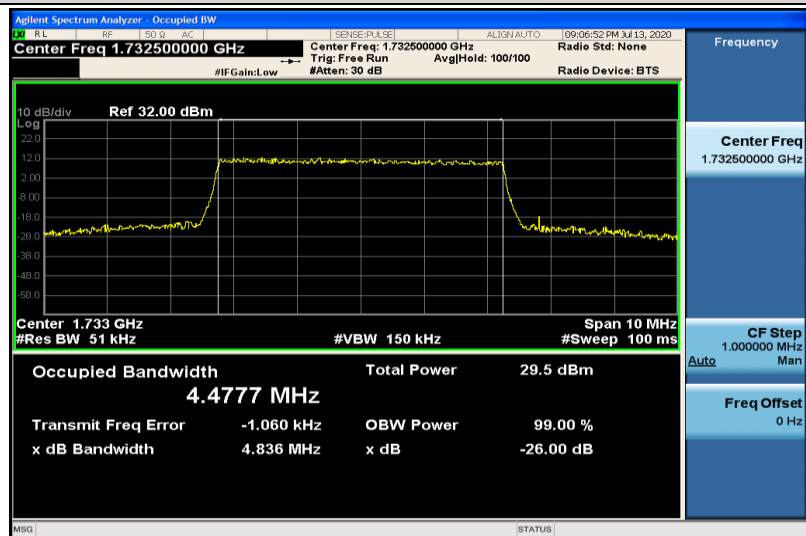
Band4-5MHz-16QAM-20175-25RB#0-4.4777
