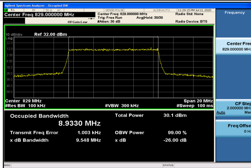
Band5-10MHz-16QAM-20450-50RB#0-8.9330
