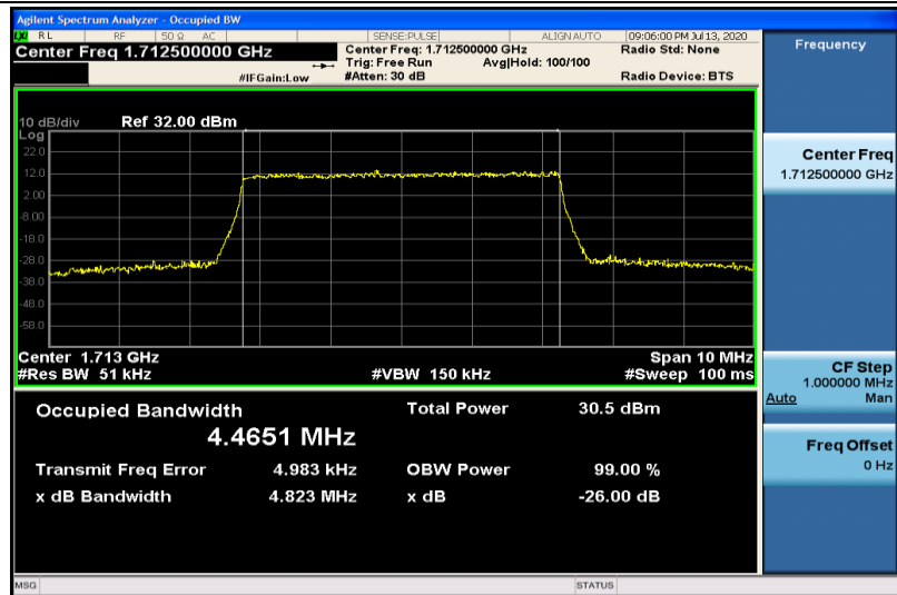
Band4-5MHz-QPSK-19975-25RB#0-4.4651
