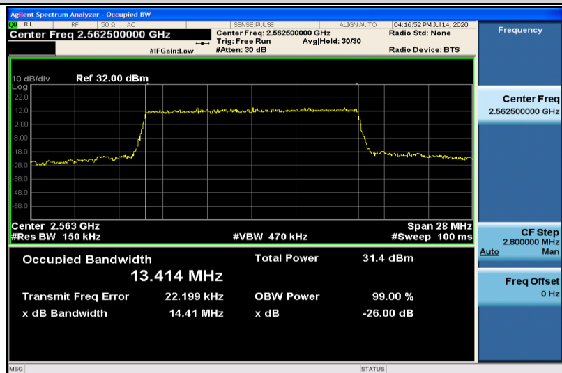
Band7-15MHz-QPSK-21375-75RB#0-13.414
