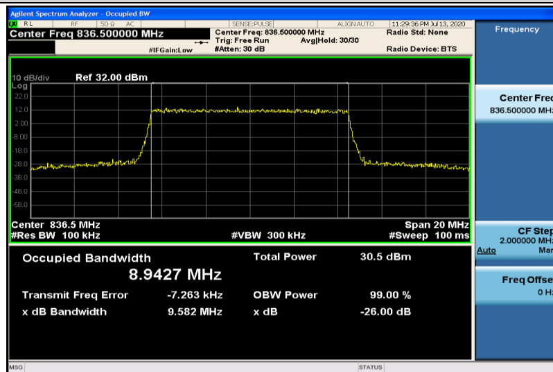
Band5-10MHz-16QAM-20525-50RB#0-8.9427
