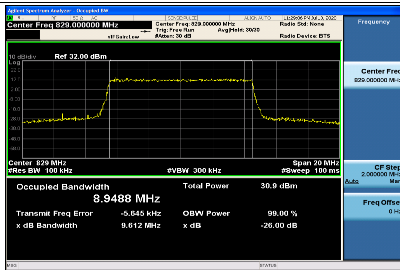
Band5-10MHz-QPSK-20450-50RB#0-8.9488
