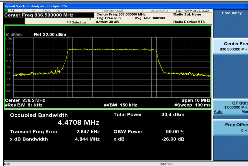
Band5-5MHz-16QAM-20525-25RB#0-4.4708
