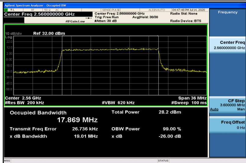
Band7-20MHz-QPSK-21350-100RB#0-17.869
