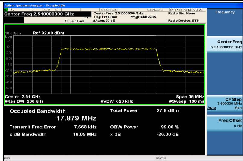
Band7-20MHz-16QAM-20850-100RB#0-17.879
