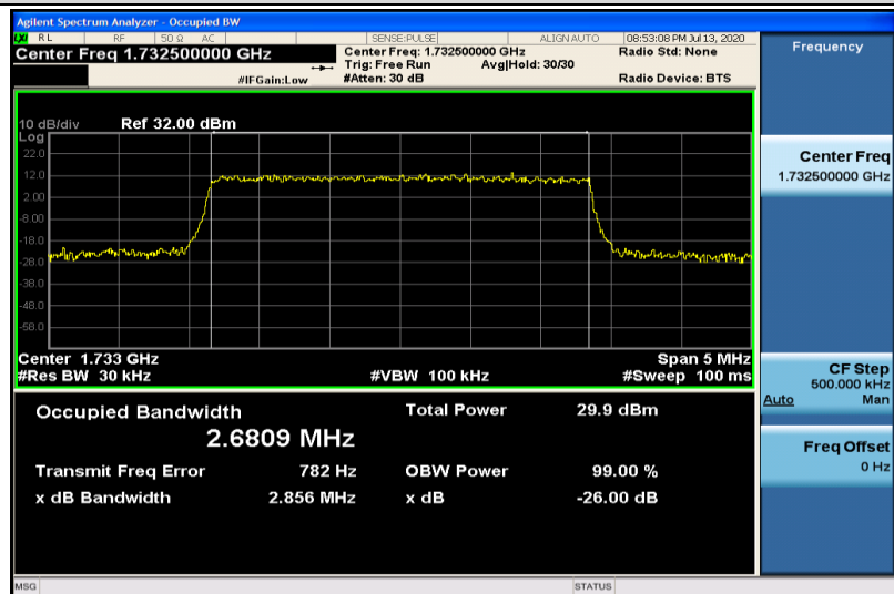
Band4-3MHz-QPSK-20175-15RB#0-2.6809
