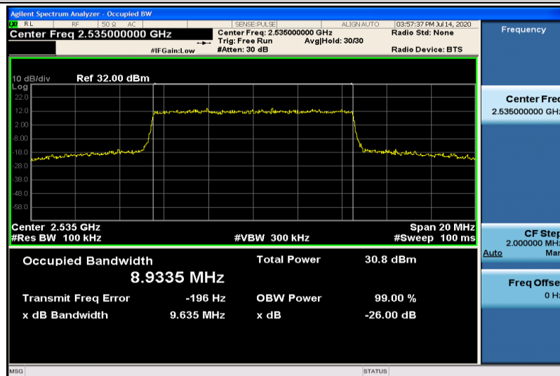
Band7-10MHz-QPSK-21100-50RB#0-8.9335
