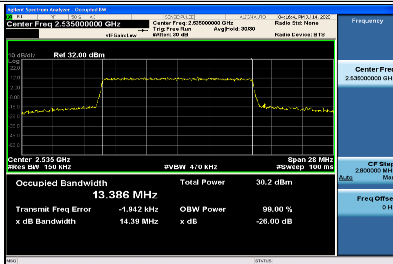
Band7-15MHz-16QAM-21100-75RB#0-13.386
