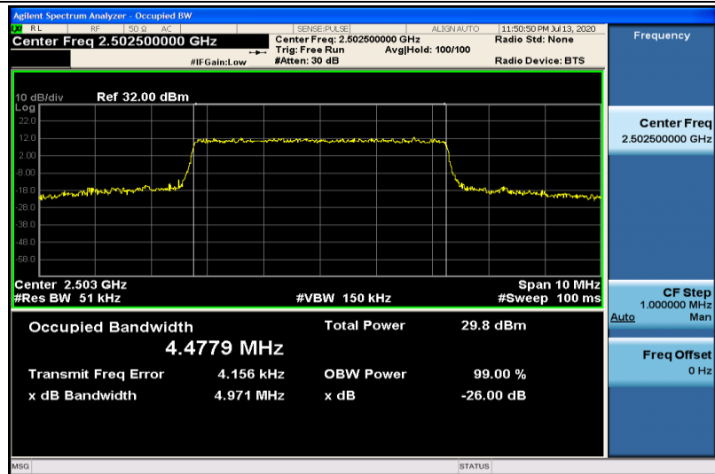
Band7-5MHz-16QAM-20775-25RB#0-4.4779
