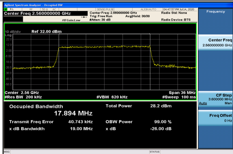
Band7-20MHz-16QAM-21350-100RB#0-17.894
