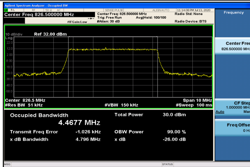
Band5-5MHz-16QAM-20425-25RB#0-4.4677
