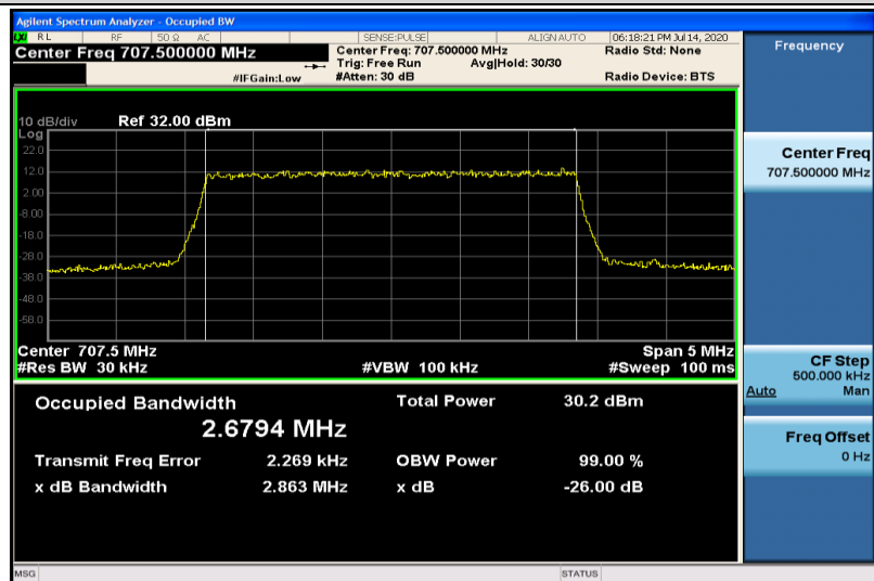
Band12-3MHz-QPSK-23095-15RB#0-2.6794
