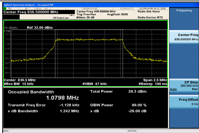
Band5-1.4MHz-16QAM-20525-6RB#0-1.0798
