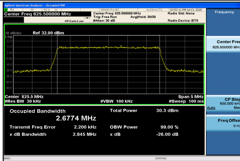
Band5-3MHz-QPSK-20415-15RB#0-2.6774
