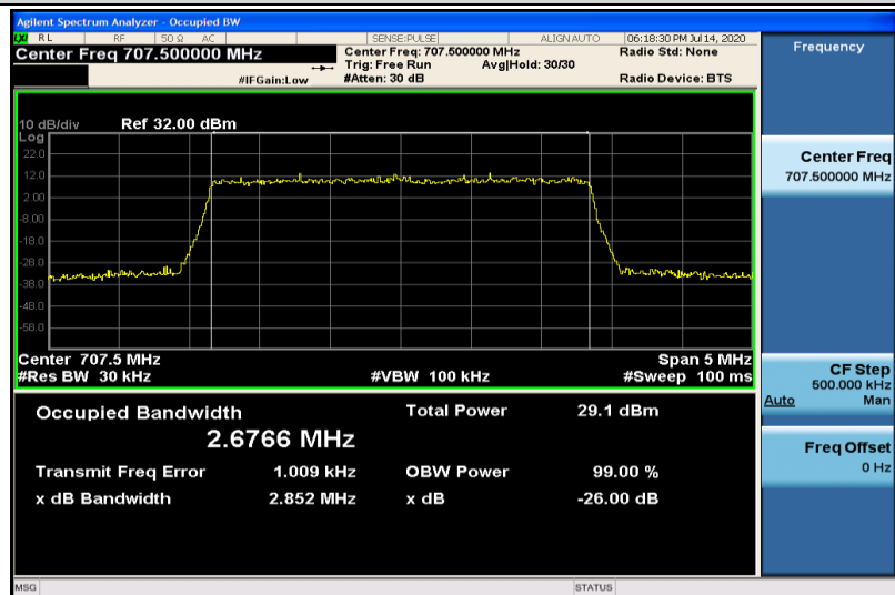
Band12-3MHz-16QAM-23095-15RB#0-2.6766
