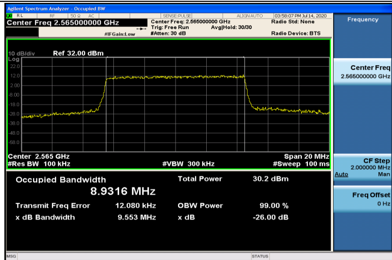
Band7-10MHz-16QAM-21400-50RB#0-8.9316
