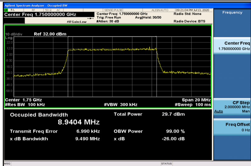
Band4-10MHz-16QAM-20350-50RB#0-8.9404
