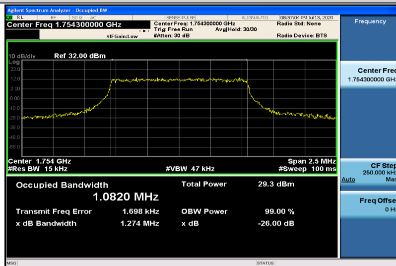
Band4-1.4MHz-QPSK-20393-6RB#0-1.0820
