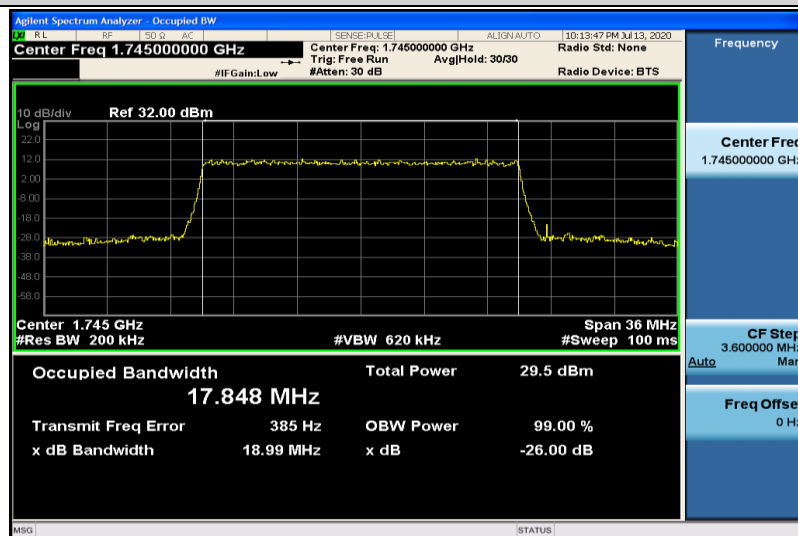
Band4-20MHz-QPSK-20300-100RB#0-17.848
