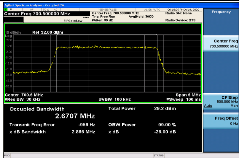
Band12-3MHz-16QAM-23025-15RB#0-2.6707
