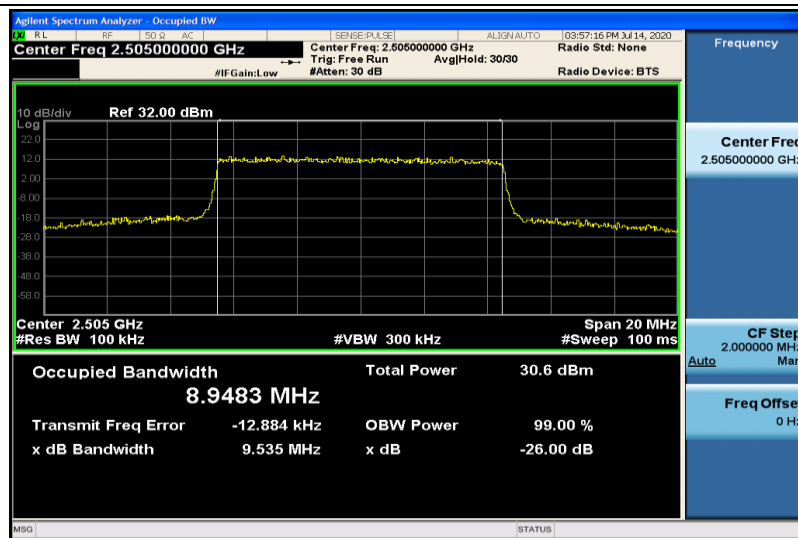
Band7-10MHz-QPSK-20800-50RB#0-8.9483
