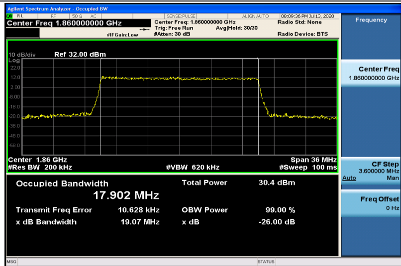
Band2-20MHz-16QAM-18700-100RB#0-17.902
