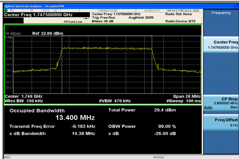
Band4-15MHz-QPSK-20325-75RB#0-13.400
