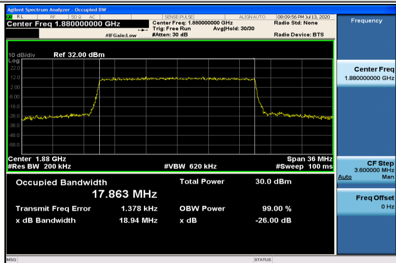
Band2-20MHz-16QAM-18900-100RB#0-17.863
