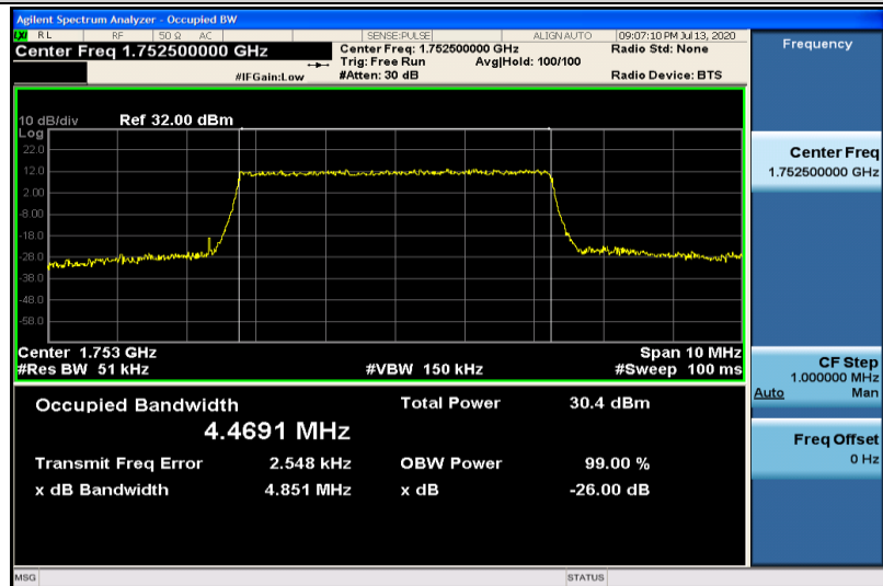
Band4-5MHz-QPSK-20375-25RB#0-4.4691
