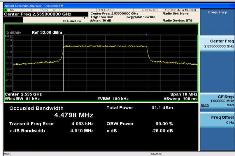
Band7-5MHz-QPSK-21100-25RB#0-4.4798
