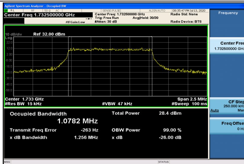
Band4-1.4MHz-16QAM-20175-6RB#0-1.0782
