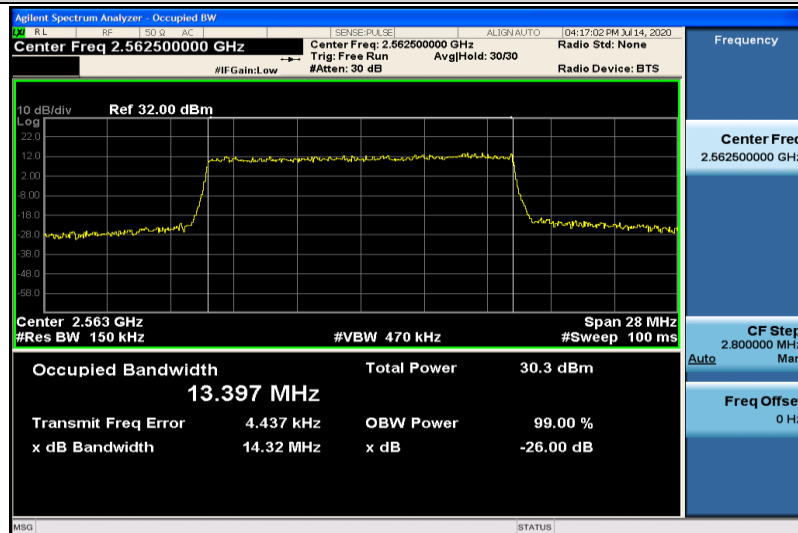
Band7-15MHz-16QAM-21375-75RB#0-13.397
