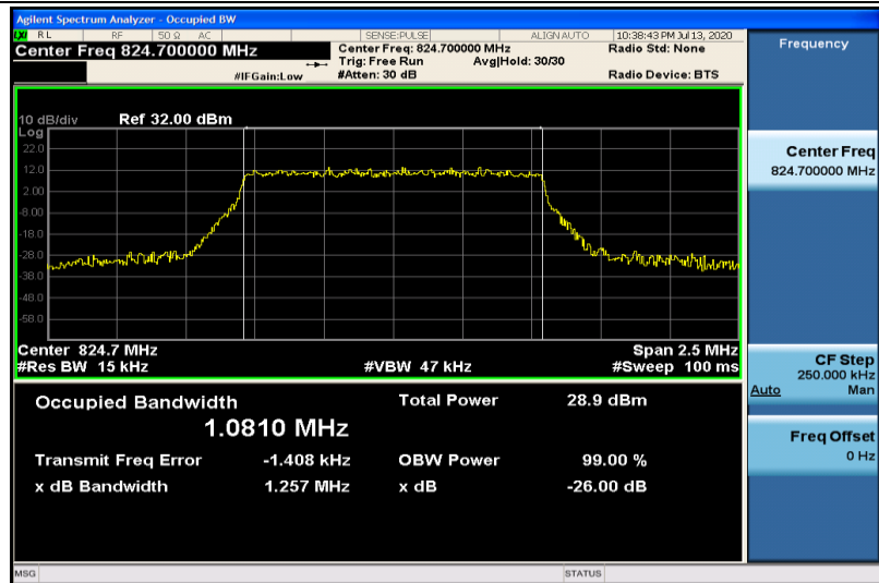
Band5-1.4MHz-16QAM-20407-6RB#0-1.0810
