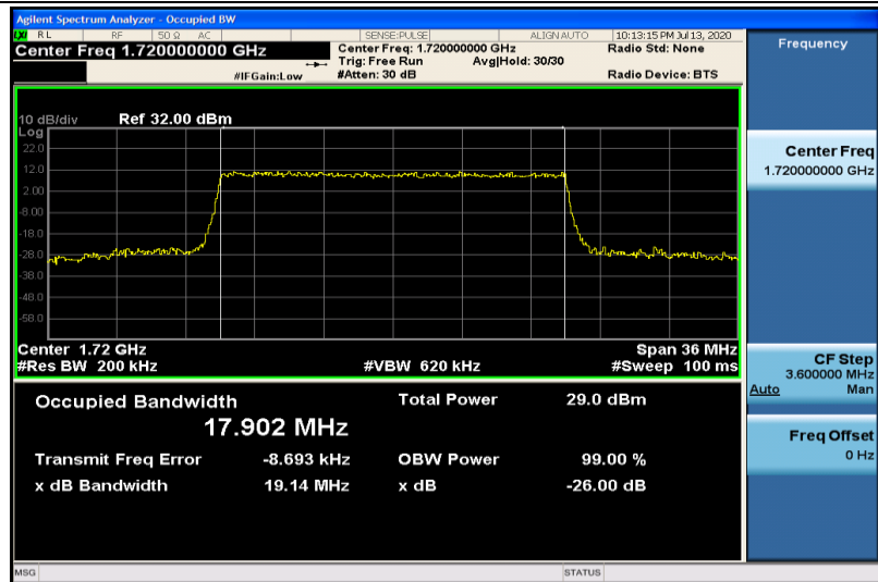
Band4-20MHz-16QAM-20050-100RB#0-17.902
