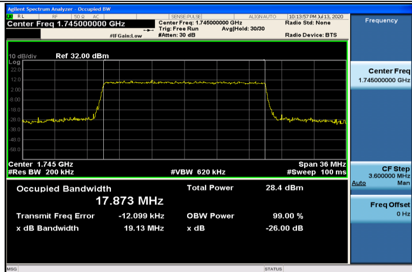
Band4-20MHz-16QAM-20300-100RB#0-17.873
