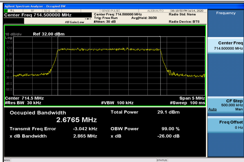
Band12-3MHz-16QAM-23165-15RB#0-2.6765
