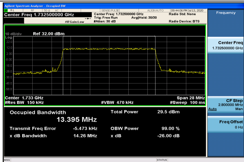
Band4-15MHz-QPSK-20175-75RB#0-13.395
