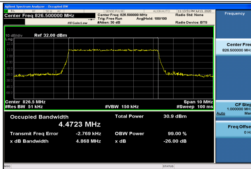
Band5-5MHz-QPSK-20425-25RB#0-4.4723
