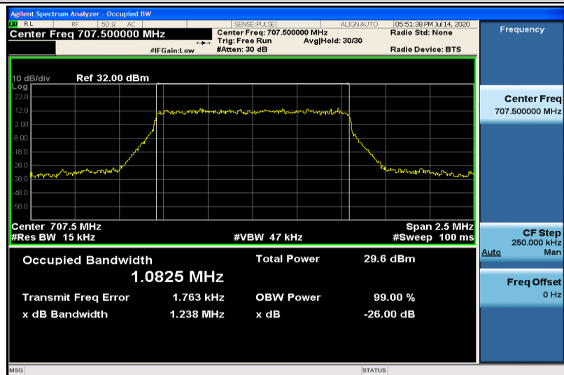
Band12-1.4MHz-QPSK-23095-6RB#0-1.0825
