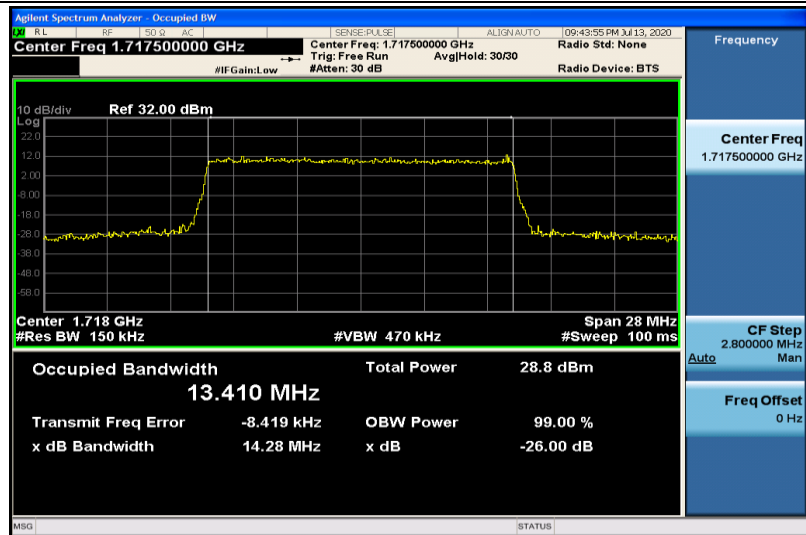
Band4-15MHz-16QAM-20025-75RB#0-13.410
