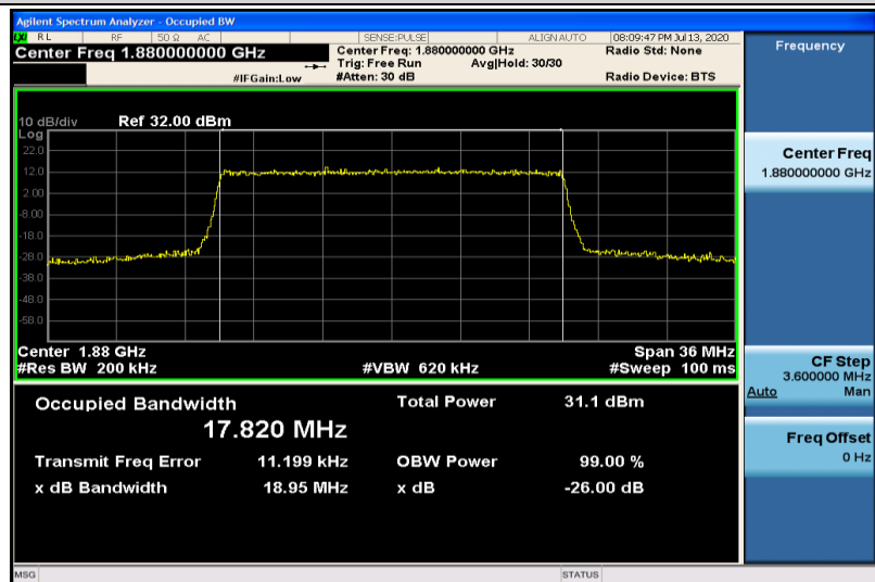
Band2-20MHz-QPSK-18900-100RB#0-17.820
