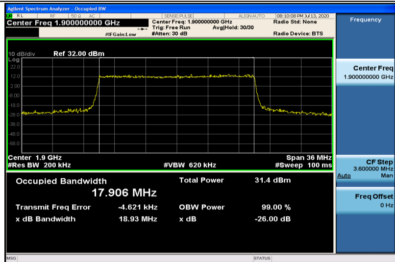
Band2-20MHz-QPSK-19100-100RB#0-17.906
