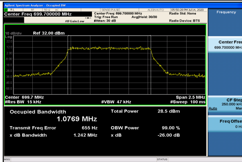
Band12-1.4MHz-16QAM-23017-6RB#0-1.0769
