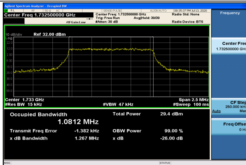
Band4-1.4MHz-QPSK-20175-6RB#0-1.0812
