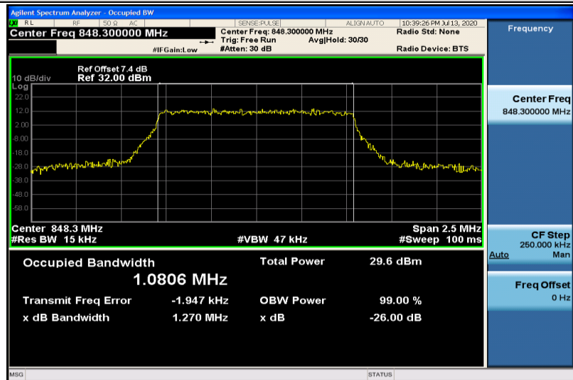
Band5-1.4MHz-16QAM-20643-6RB#0-1.0806
