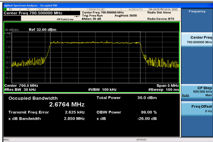
Band12-3MHz-QPSK-23025-15RB#0-2.6764
