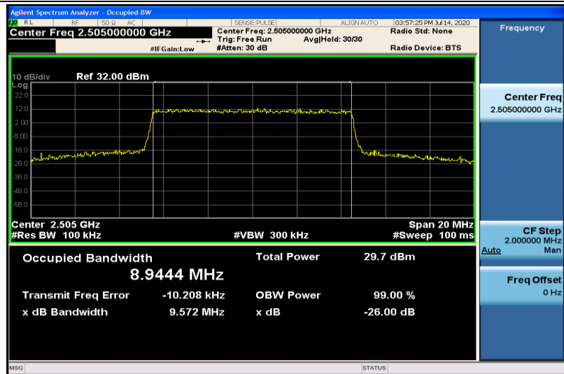
Band7-10MHz-16QAM-20800-50RB#0-8.9444
