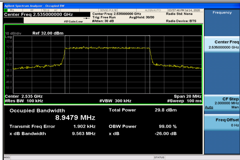
Band7-10MHz-16QAM-21100-50RB#0-8.9479
