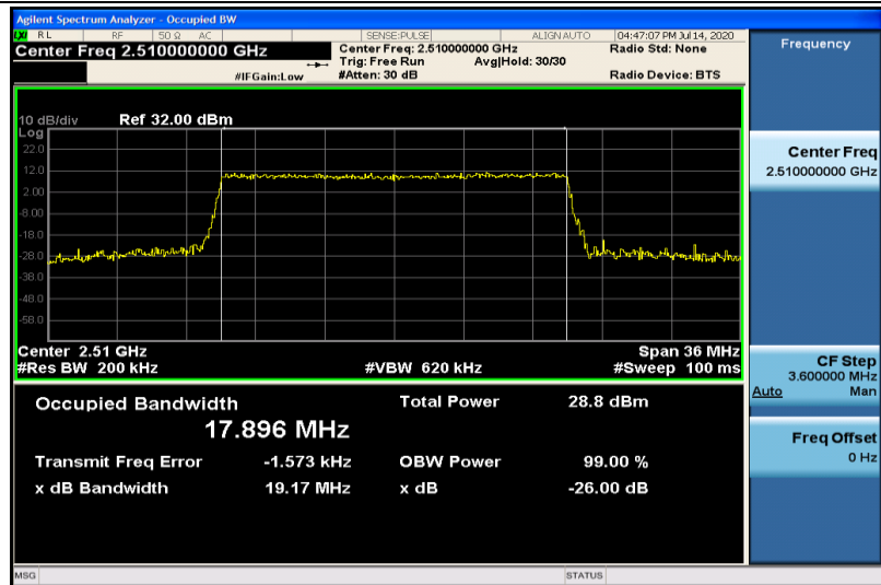
Band7-20MHz-QPSK-20850-100RB#0-17.896
