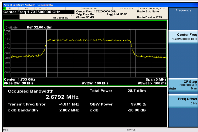
Band4-3MHz-16QAM-20175-15RB#0-2.6792
