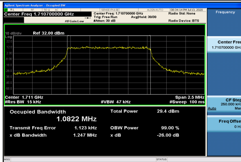
Band4-1.4MHz-QPSK-19957-6RB#0-1.0822
