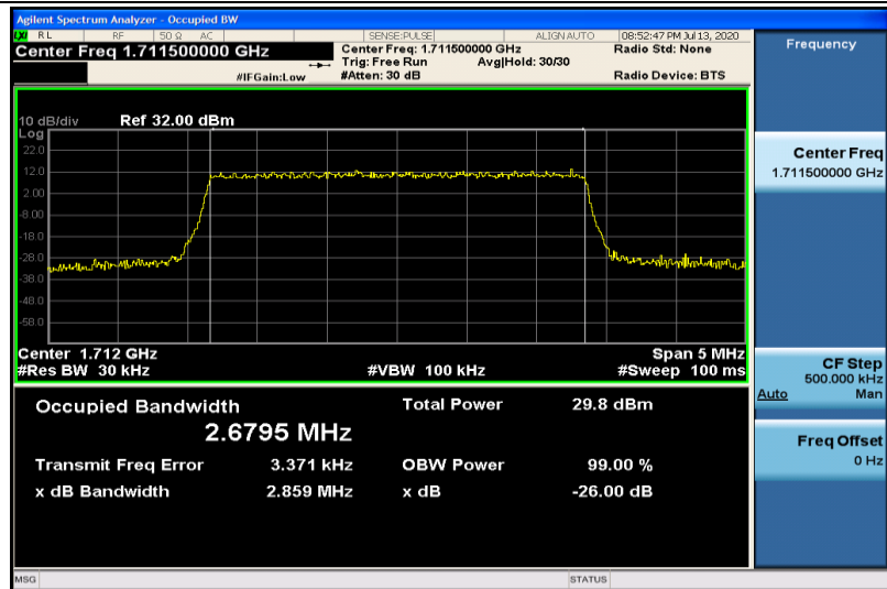
Band4-3MHz-QPSK-19965-15RB#0-2.6795
