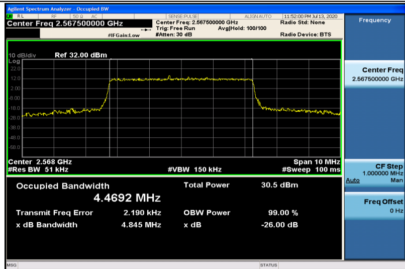
Band7-5MHz-16QAM-21425-25RB#0-4.4692
