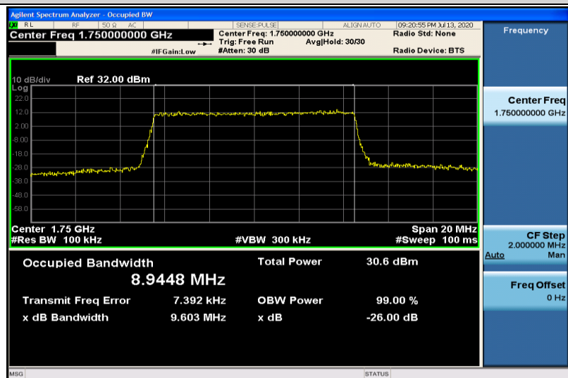
Band4-10MHz-QPSK-20350-50RB#0-8.9448
