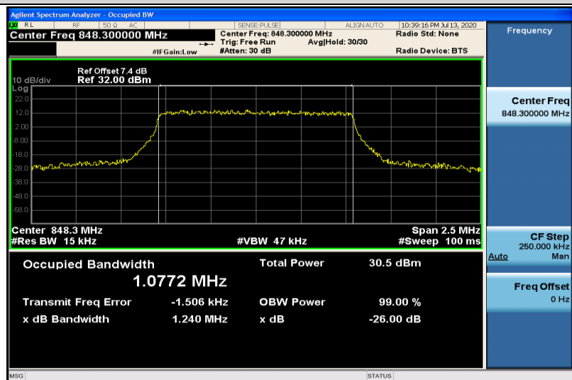
Band5-1.4MHz-QPSK-20643-6RB#0-1.0772
