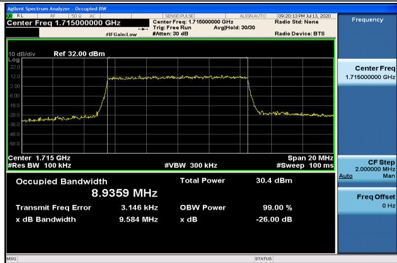
Band4-10MHz-QPSK-20000-50RB#0-8.9359
