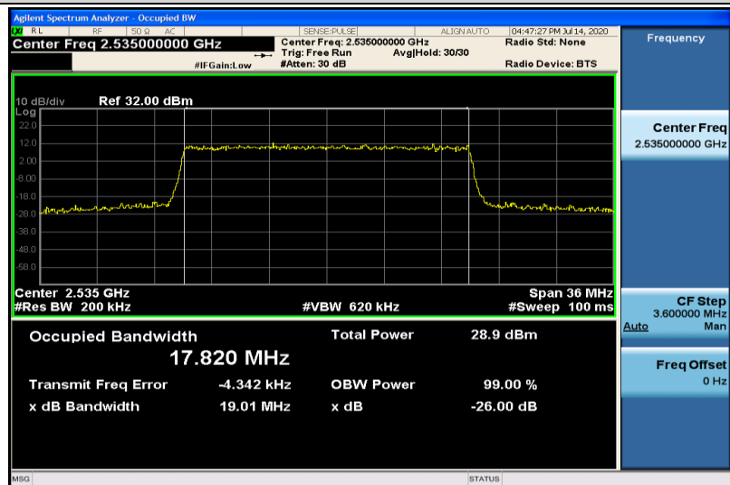
Band7-20MHz-QPSK-21100-100RB#0-17.820
