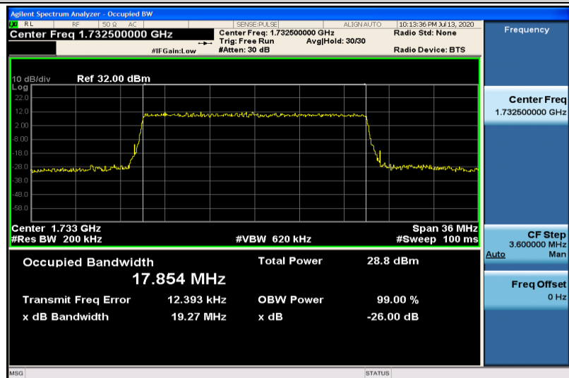
Band4-20MHz-16QAM-20175-100RB#0-17.854
