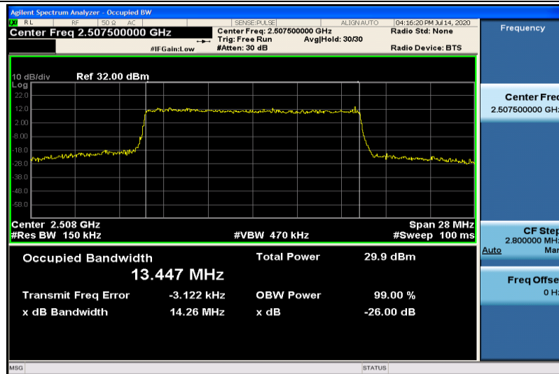
Band7-15MHz-16QAM-20825-75RB#0-13.447
