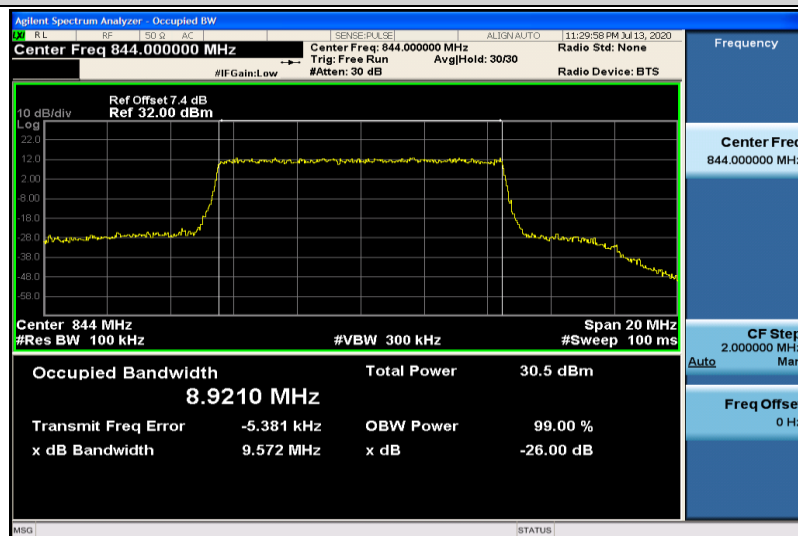
Band5-10MHz-16QAM-20600-50RB#0-8.9210
