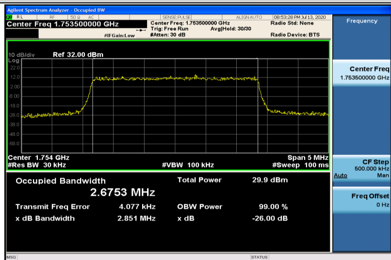
Band4-3MHz-QPSK-20385-15RB#0-2.6753
