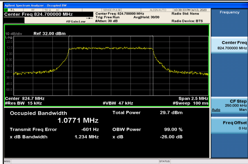
Band5-1.4MHz-QPSK-20407-6RB#0-1.0771
