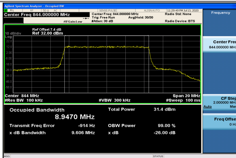
Band5-10MHz-QPSK-20600-50RB#0-8.9470
