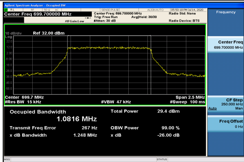
Band12-1.4MHz-QPSK-23017-6RB#0-1.0816
