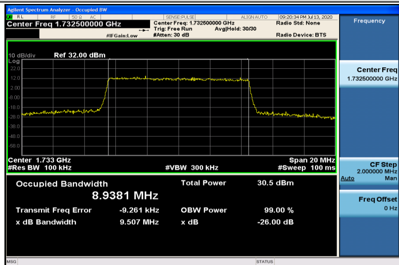
Band4-10MHz-QPSK-20175-50RB#0-8.9381
