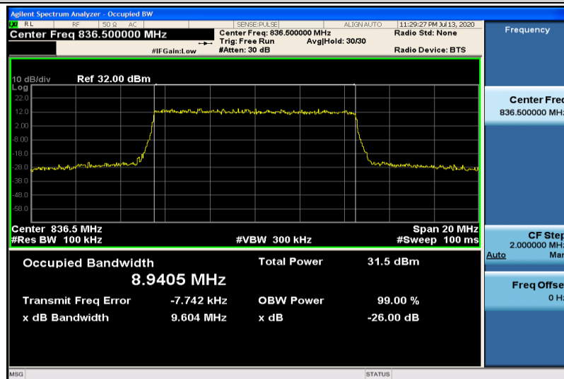
Band5-10MHz-QPSK-20525-50RB#0-8.9405
