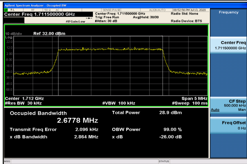
Band4-3MHz-16QAM-19965-15RB#0-2.6778
