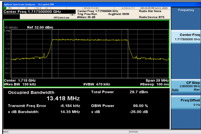
Band4-15MHz-QPSK-20025-75RB#0-13.418
