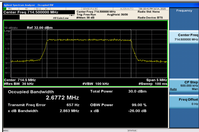
Band12-3MHz-QPSK-23165-15RB#0-2.6772
