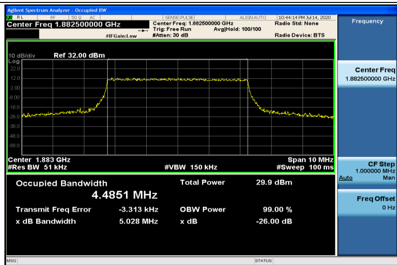
Band25-5MHz-QPSK-26365-25RB#0-4.4851
