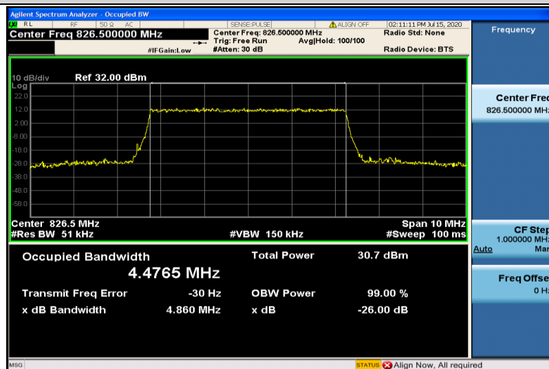
Band26-5MHz-QPSK-26815-25RB#0-4.4765
