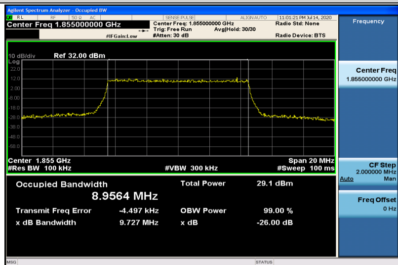
Band25-10MHz-16QAM-26090-50RB#0-8.9564
