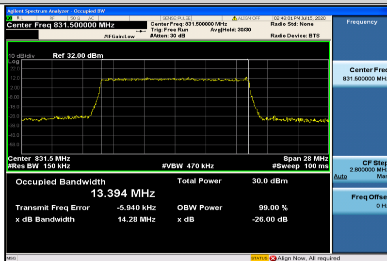
Band26-15MHz-16QAM-26865-75RB#0-13.394
