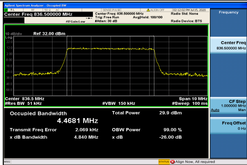
Band26-5MHz-16QAM-26915-25RB#0-4.4681
