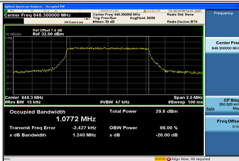
Band26-1.4MHz-QPSK-27033-6RB#0-1.0772
