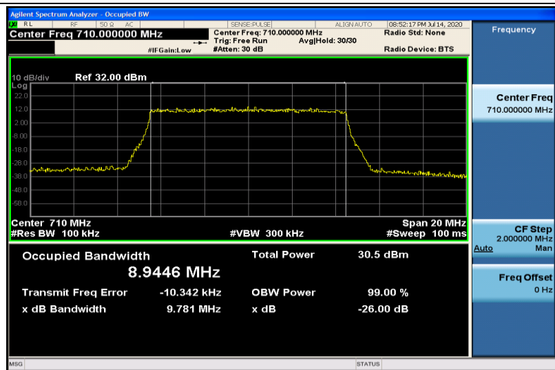
Band17-10MHz-QPSK-23790-50RB#0-8.9446
