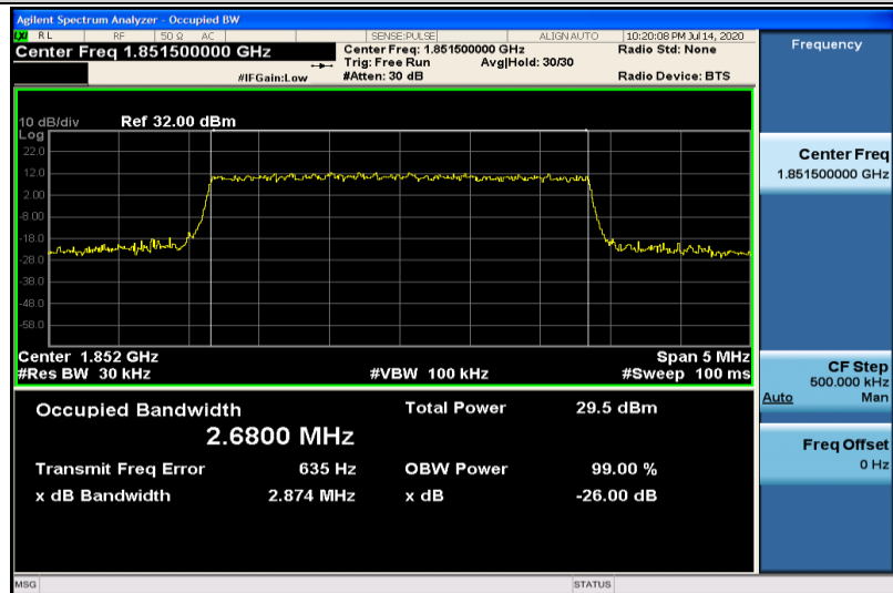
Band25-3MHz-QPSK-26055-15RB#0-2.6800
