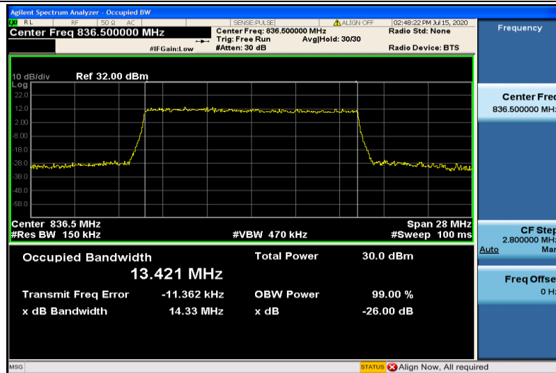
Band26-15MHz-16QAM-26915-75RB#0-13.421
