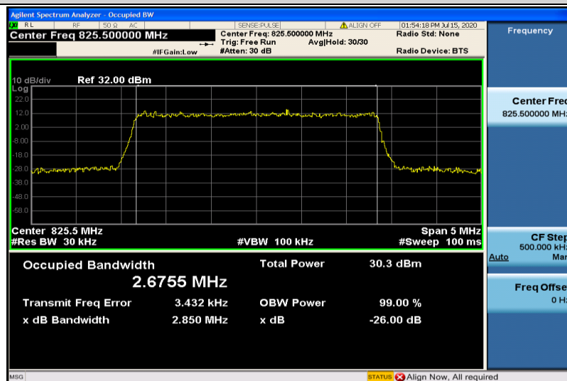
Band26-3MHz-QPSK-26805-15RB#0-2.6755
