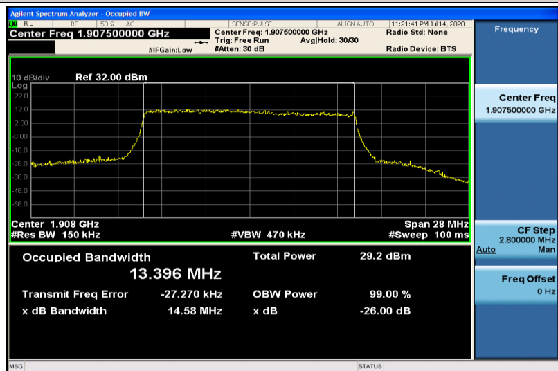
Band25-15MHz-16QAM-26615-75RB#0-13.396
