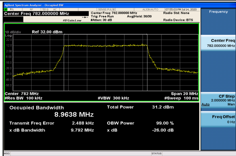
Band13-10MHz-QPSK-23230-50RB#0-8.9638
