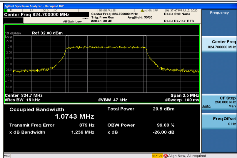
Band26-1.4MHz-QPSK-26797-6RB#0-1.0743
