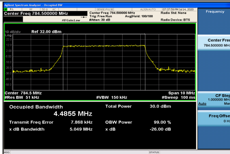
Band13-5MHz-16QAM-23255-25RB#0-4.4855
