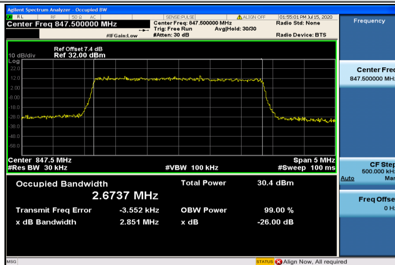
Band26-3MHz-QPSK-27025-15RB#0-2.6737
