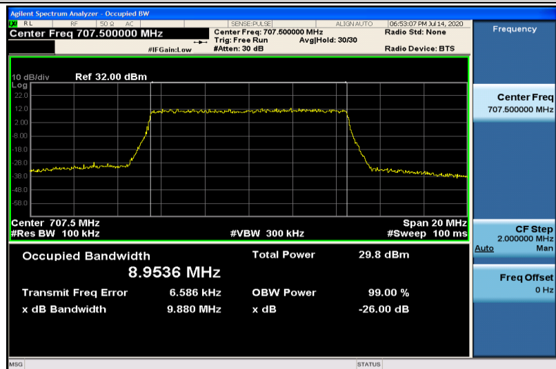
Band12-10MHz-16QAM-23095-50RB#0-8.9536
