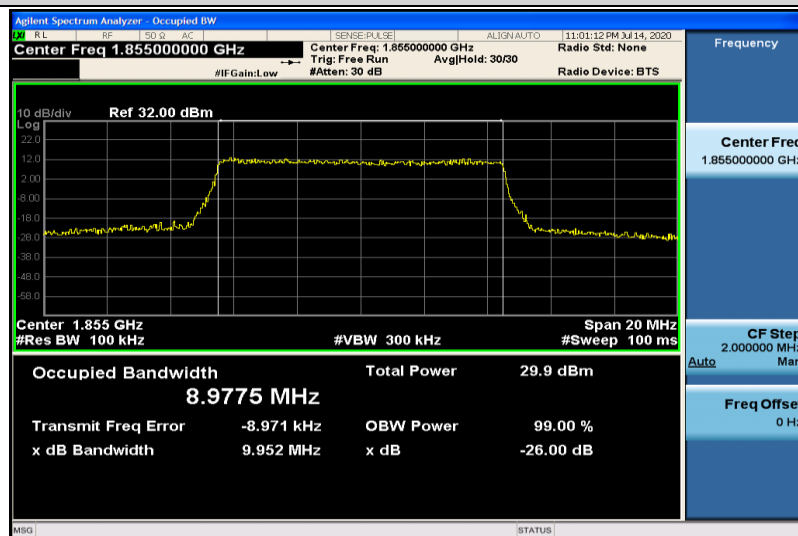
Band25-10MHz-QPSK-26090-50RB#0-8.9775
