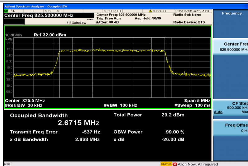
Band26-3MHz-16QAM-26805-15RB#0-2.6715
