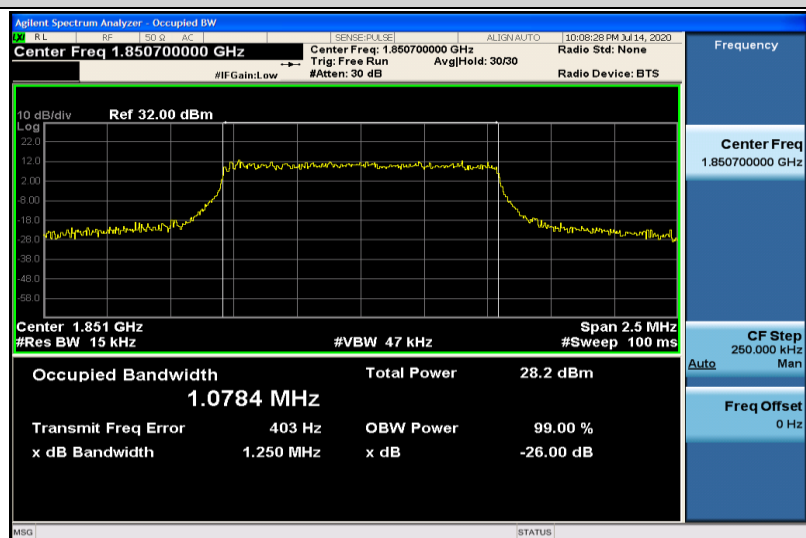
Band25-1.4MHz-16QAM-26047-6RB#0-1.0784
