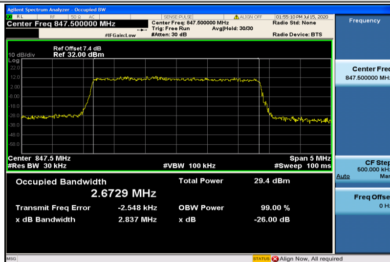
Band26-3MHz-16QAM-27025-15RB#0-2.6729
