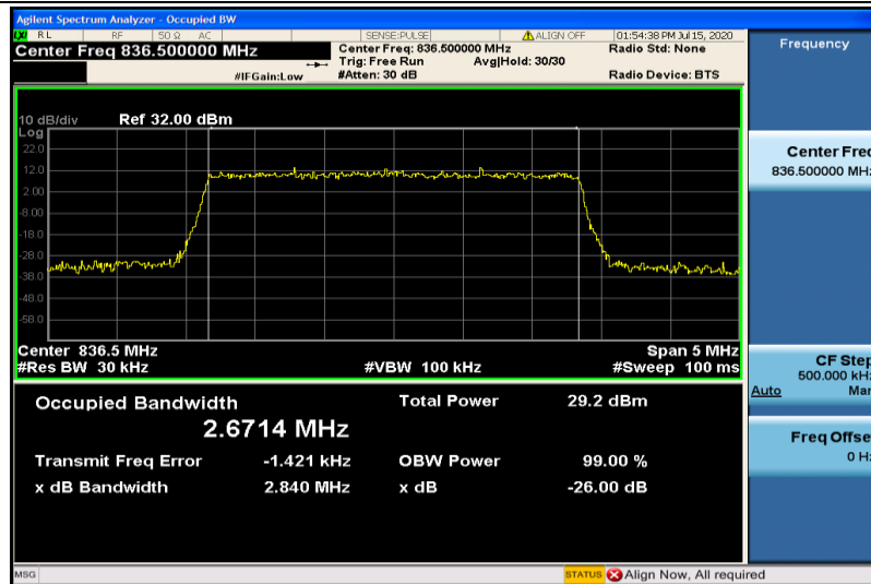
Band26-3MHz-QPSK-26915-15RB#0-2.6714
