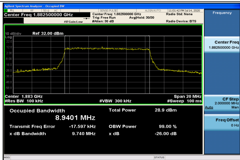
Band25-10MHz-16QAM-26365-50RB#0-8.9401
