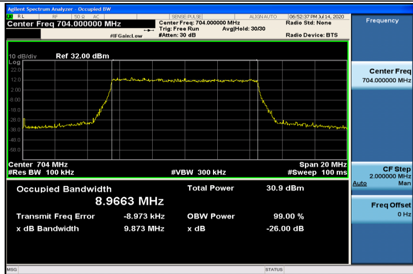
Band12-10MHz-QPSK-23060-50RB#0-8.9663
