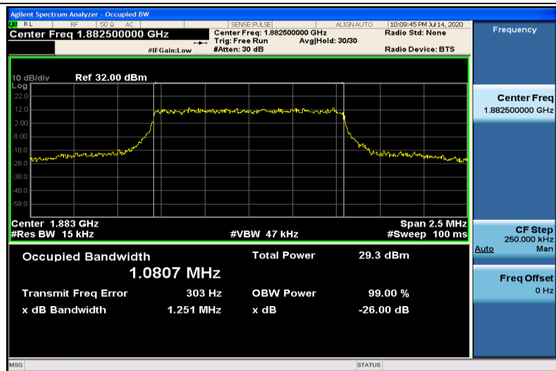
Band25-1.4MHz-QPSK-26365-6RB#0-1.0807
