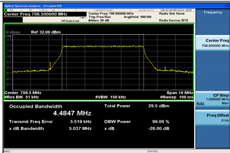
Band17-5MHz-16QAM-23755-25RB#0-4.4847
