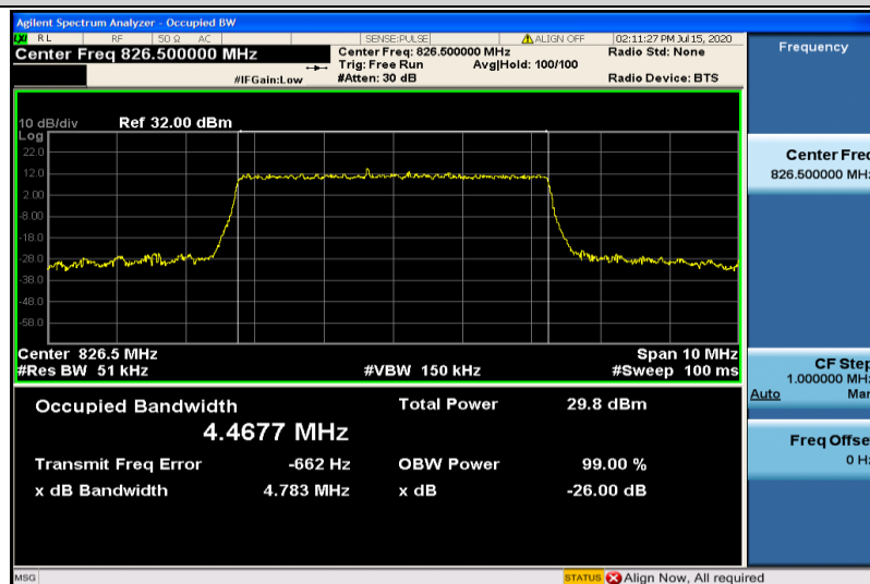
Band26-5MHz-16QAM-26815-25RB#0-4.4677
