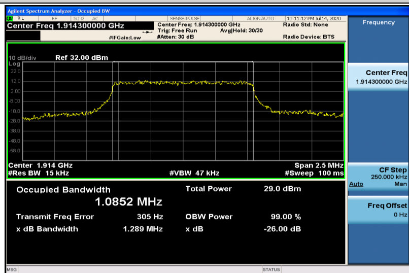
Band25-1.4MHz-QPSK-26683-6RB#0-1.0852
