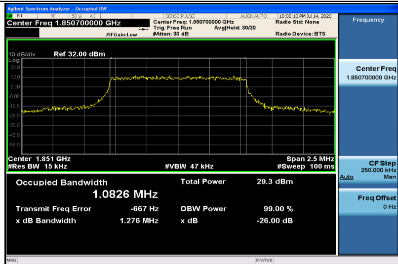
Band25-1.4MHz-QPSK-26047-6RB#0-1.0826
