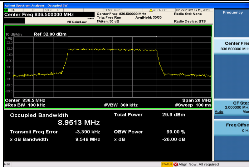
Band26-10MHz-16QAM-26915-50RB#0-8.9513
