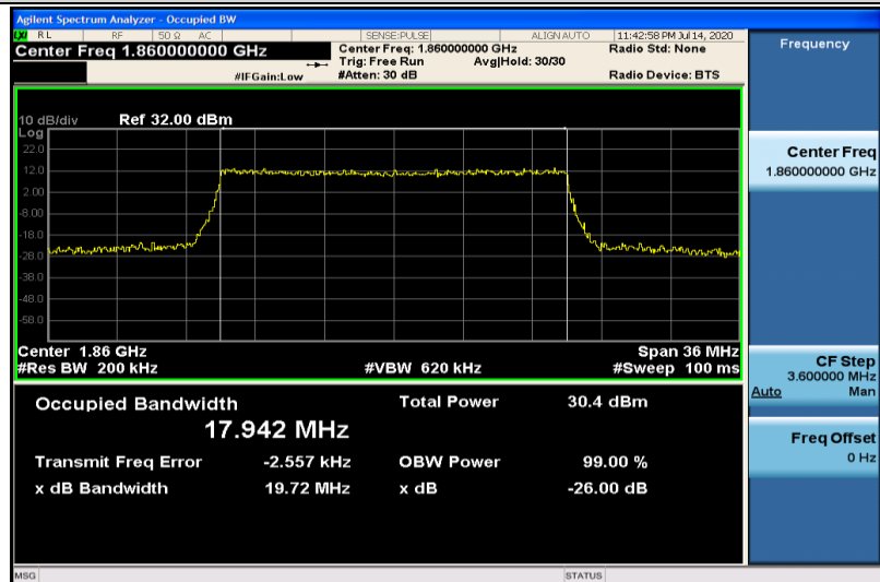
Band25-20MHz-QPSK-26140-100RB#0-17.942
