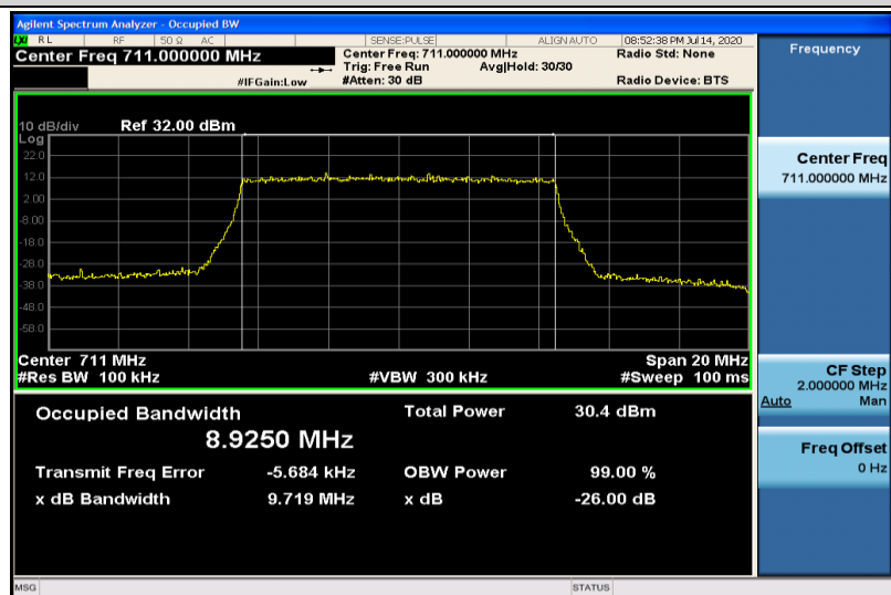
Band17-10MHz-QPSK-23800-50RB#0-8.9250
