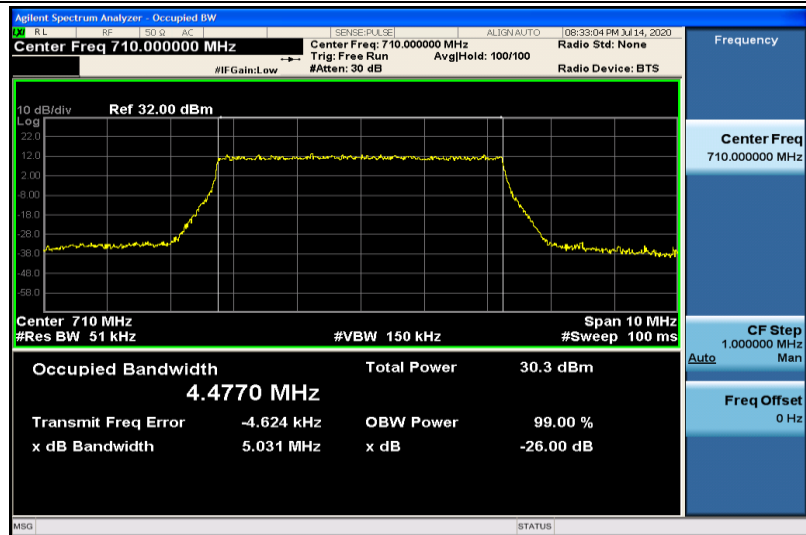
Band17-5MHz-QPSK-23790-25RB#0-4.4770
