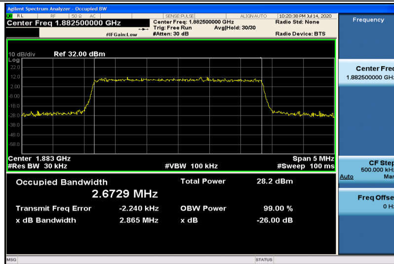
Band25-3MHz-16QAM-26365-15RB#0-2.6729
