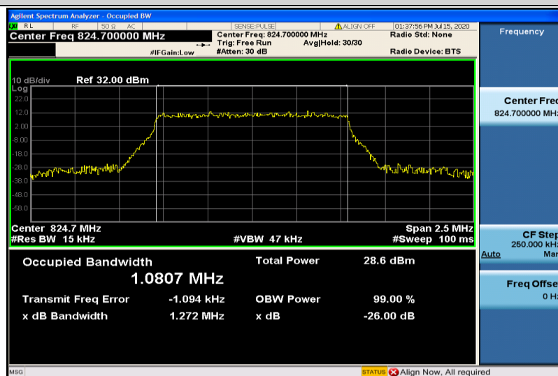
Band26-1.4MHz-16QAM-26797-6RB#0-1.0807
