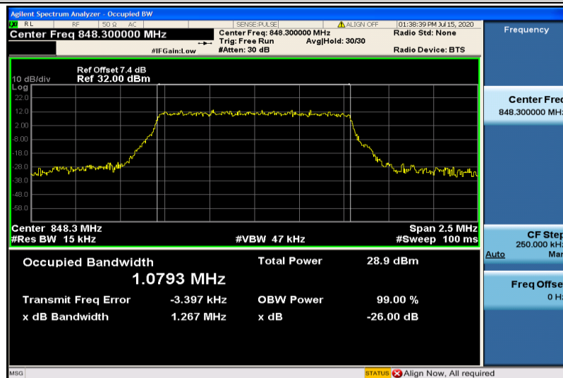
Band26-1.4MHz-16QAM-27033-6RB#0-1.0793
