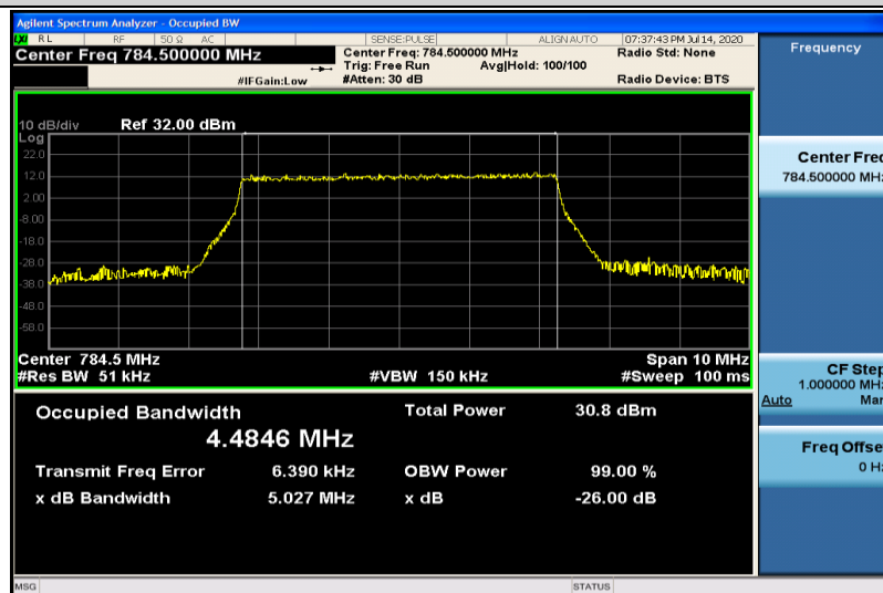
Band13-5MHz-QPSK-23255-25RB#0-4.4846
