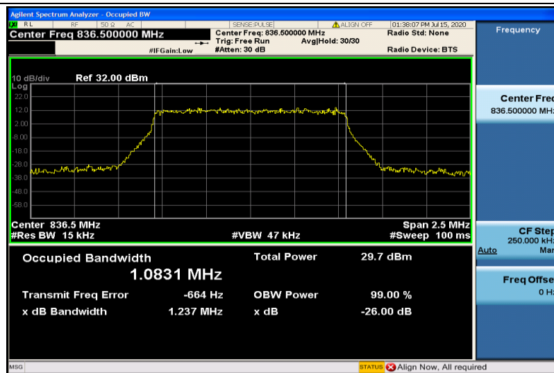
Band26-1.4MHz-QPSK-26915-6RB#0-1.0831
