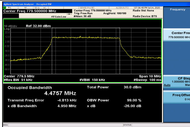
Band13-5MHz-16QAM-23205-25RB#0-4.4757
