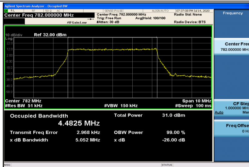
Band13-5MHz-QPSK-23230-25RB#0-4.4825
