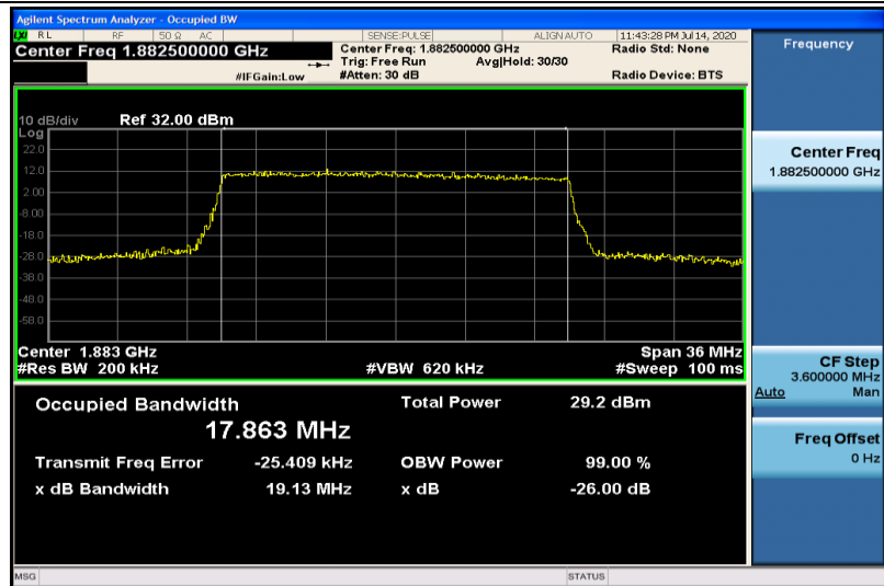
Band25-20MHz-16QAM-26365-100RB#0-17.863
