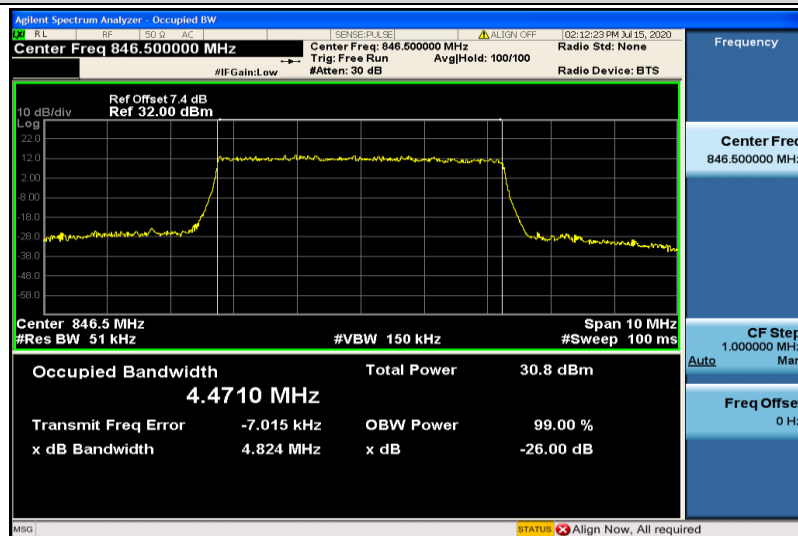
Band26-5MHz-QPSK-27015-25RB#0-4.4710
