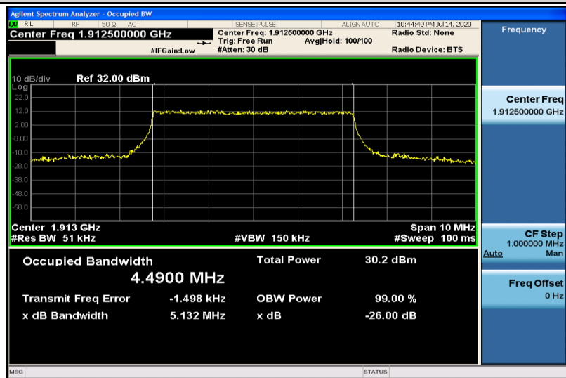
Band25-5MHz-QPSK-26665-25RB#0-4.4900
