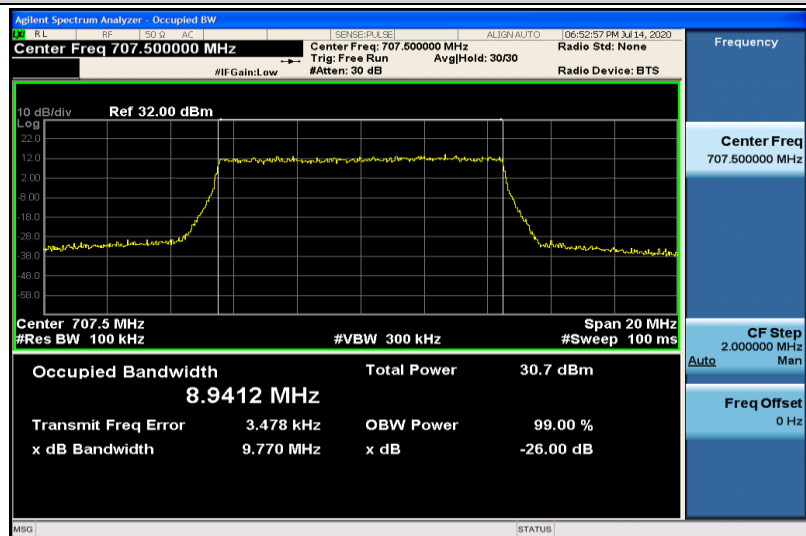
Band12-10MHz-QPSK-23095-50RB#0-8.9412
