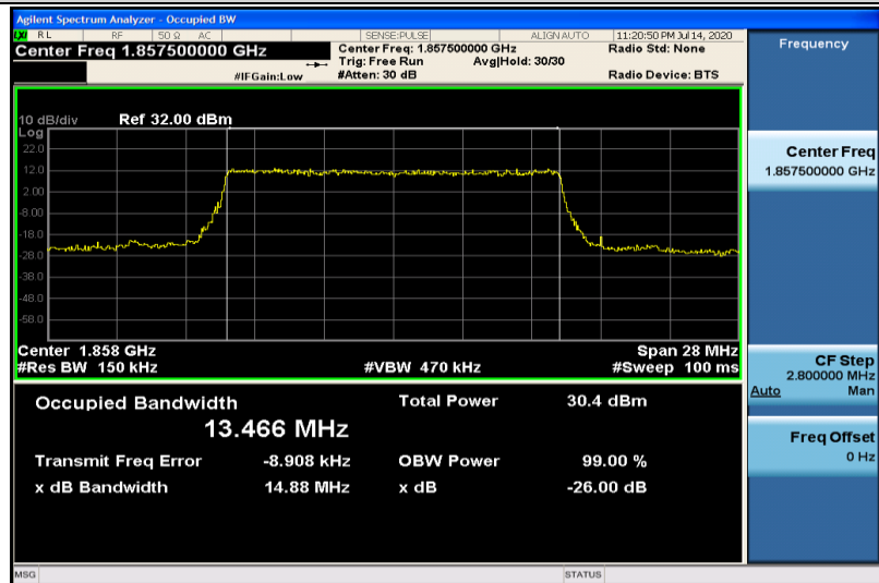
Band25-15MHz-QPSK-26115-75RB#0-13.466
