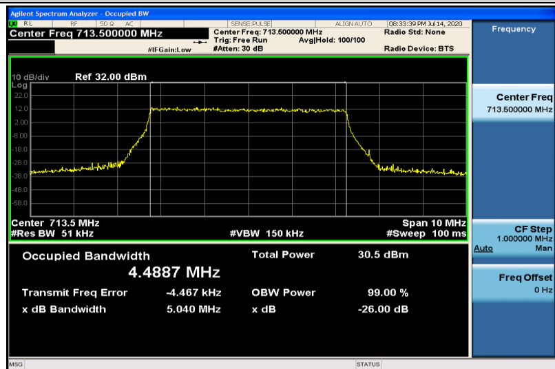
Band17-5MHz-QPSK-23825-25RB#0-4.4887
