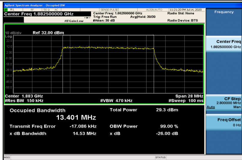
Band25-15MHz-16QAM-26365-75RB#0-13.401
