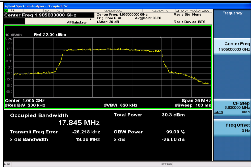
Band25-20MHz-QPSK-26590-100RB#0-17.845
