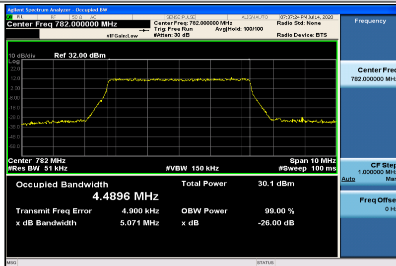
Band13-5MHz-16QAM-23230-25RB#0-4.4896
