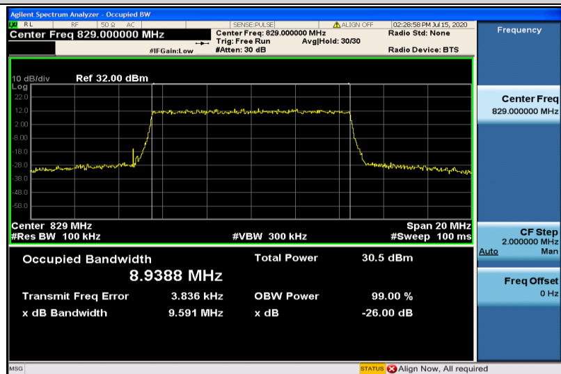
Band26-10MHz-QPSK-26840-50RB#0-8.9388
