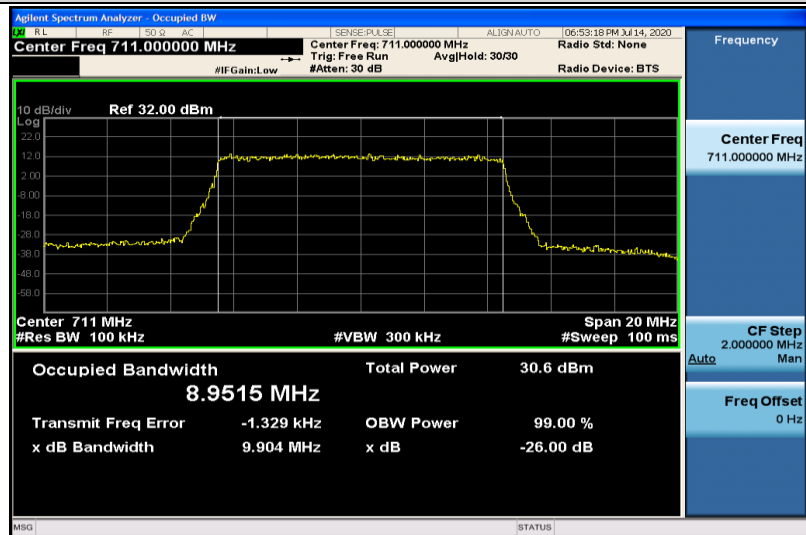
Band12-10MHz-QPSK-23130-50RB#0-8.9515
