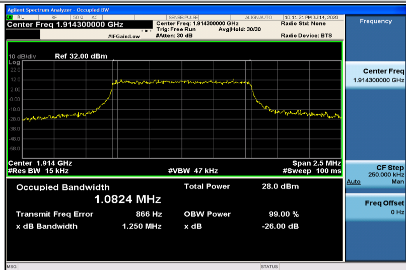
Band25-1.4MHz-16QAM-26683-6RB#0-1.0824
