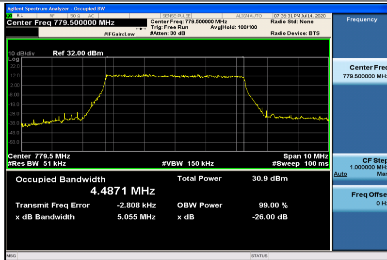
Band13-5MHz-QPSK-23205-25RB#0-4.4871
