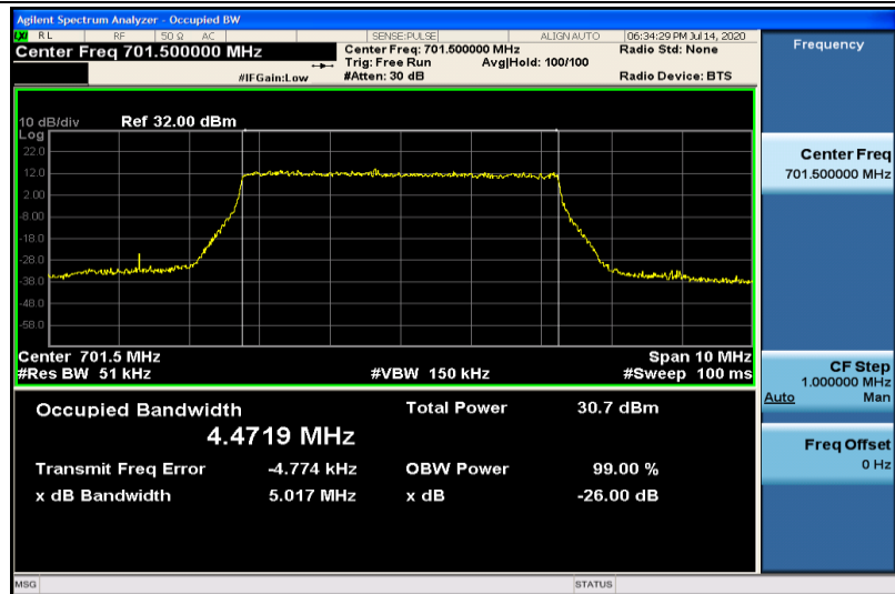
Band12-5MHz-QPSK-23035-25RB#0-4.4719
