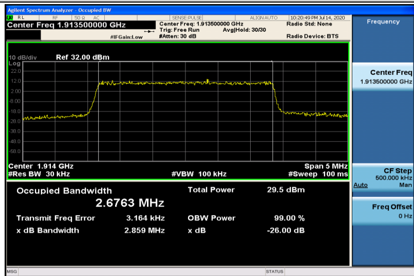
Band25-3MHz-QPSK-26675-15RB#0-2.6763
