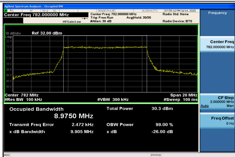
Band13-10MHz-16QAM-23230-50RB#0-8.9750
