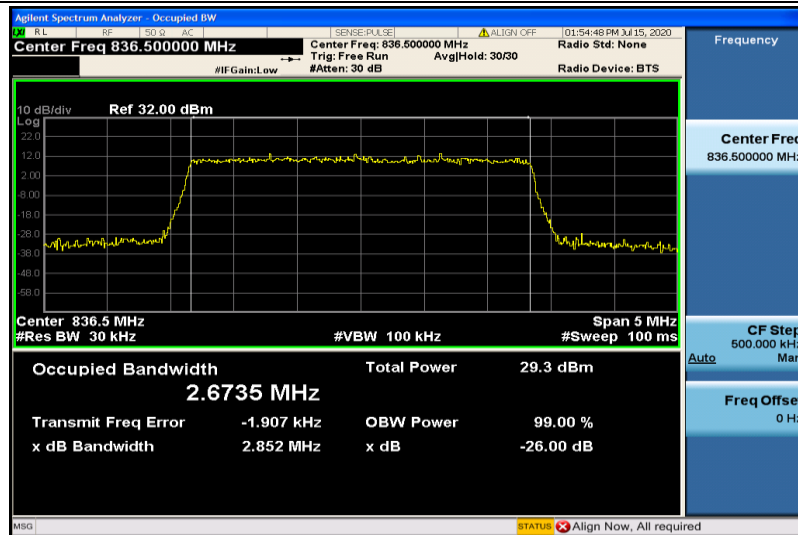
Band26-3MHz-16QAM-26915-15RB#0-2.6735
