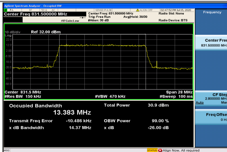
Band26-15MHz-QPSK-26865-75RB#0-13.383
