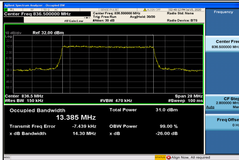
Band26-15MHz-QPSK-26915-75RB#0-13.385
