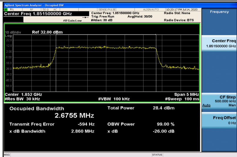
Band25-3MHz-16QAM-26055-15RB#0-2.6755
