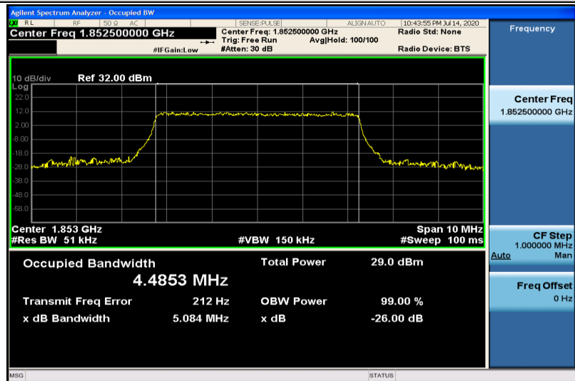
Band25-5MHz-16QAM-26065-25RB#0-4.4853
