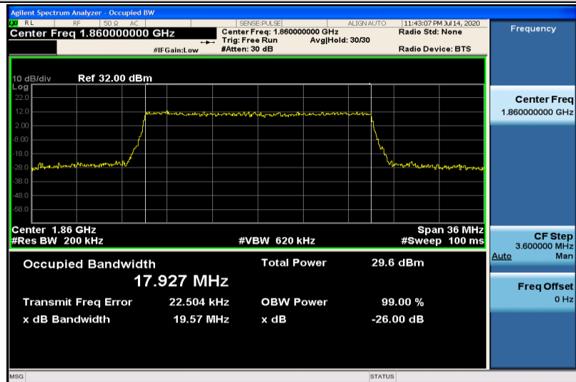
Band25-20MHz-16QAM-26140-100RB#0-17.927
