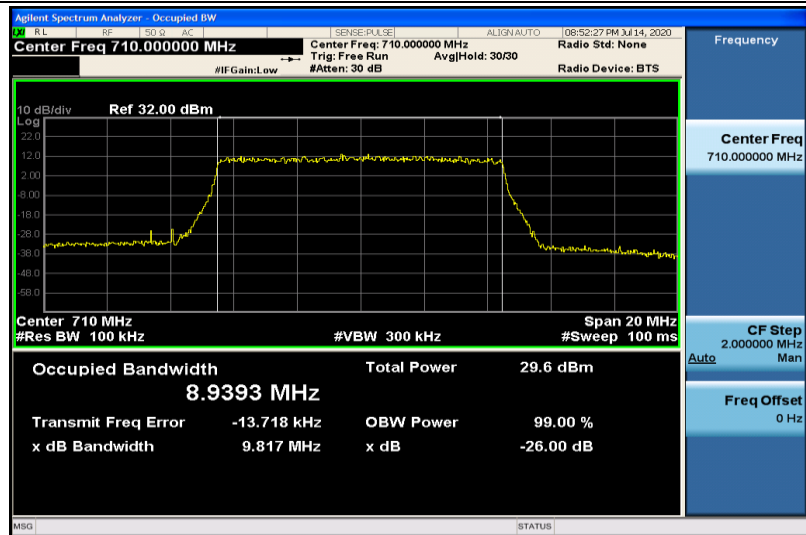
Band17-10MHz-16QAM-23790-50RB#0-8.9393
