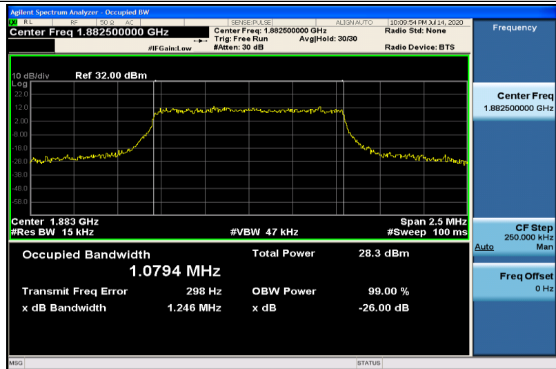
Band25-1.4MHz-16QAM-26365-6RB#0-1.0794
