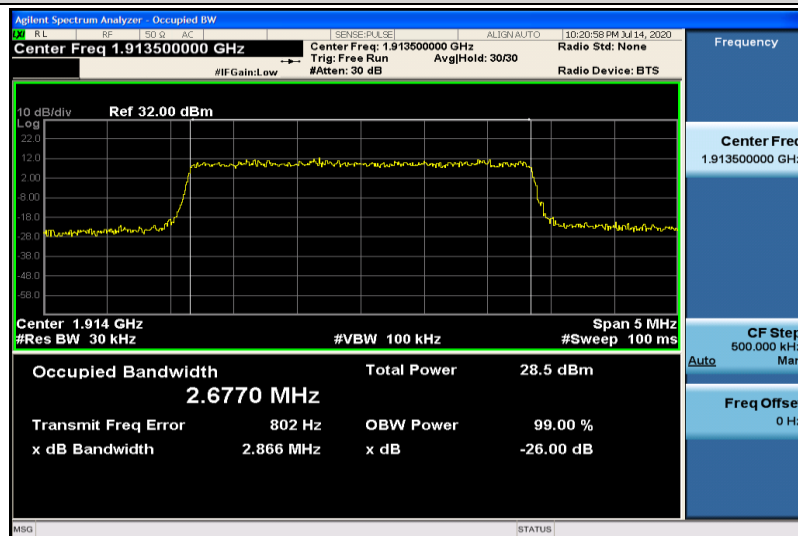
Band25-3MHz-16QAM-26675-15RB#0-2.6770
