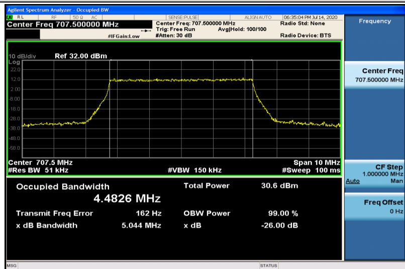
Band12-5MHz-QPSK-23095-25RB#0-4.4826
