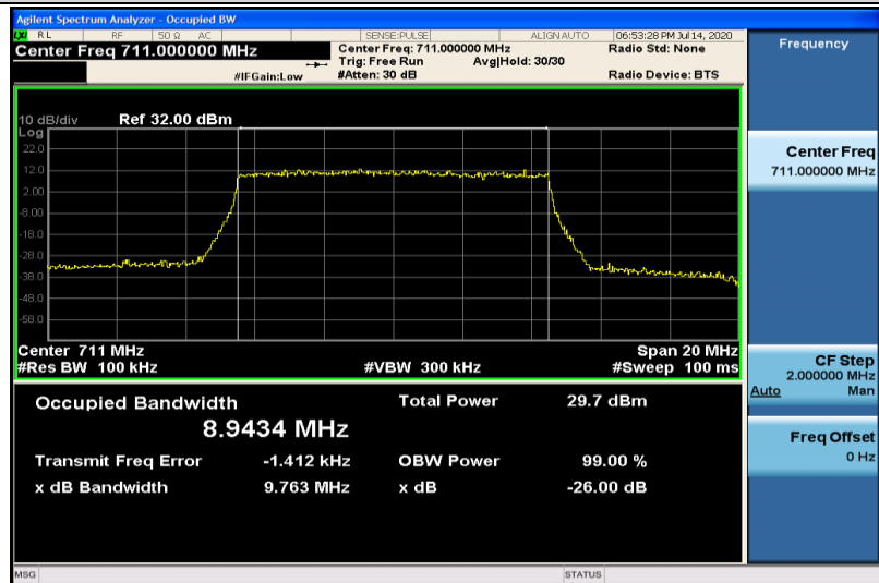
Band12-10MHz-16QAM-23130-50RB#0-8.9434
