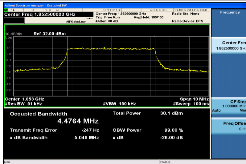
Band25-5MHz-QPSK-26065-25RB#0-4.4764
