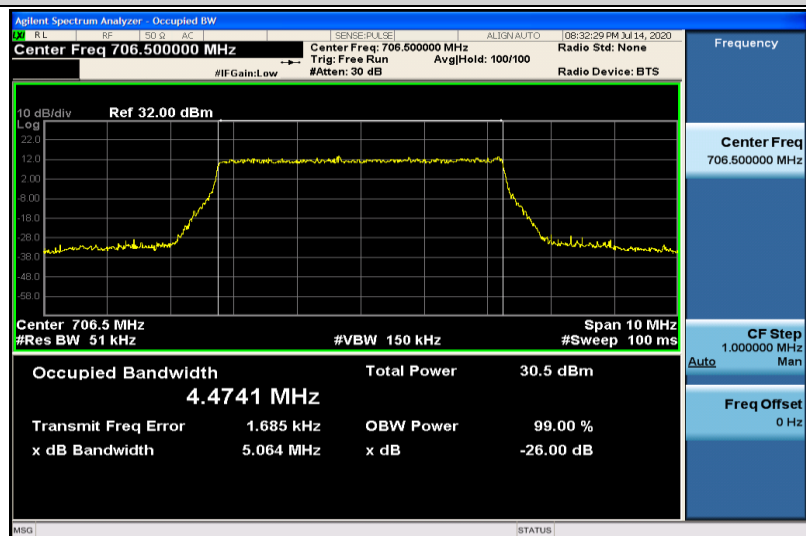
Band17-5MHz-QPSK-23755-25RB#0-4.4741
