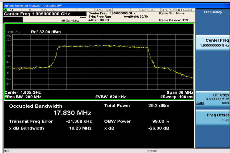
Band25-20MHz-16QAM-26590-100RB#0-17.830
