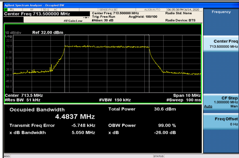
Band12-5MHz-QPSK-23155-25RB#0-4.4837
