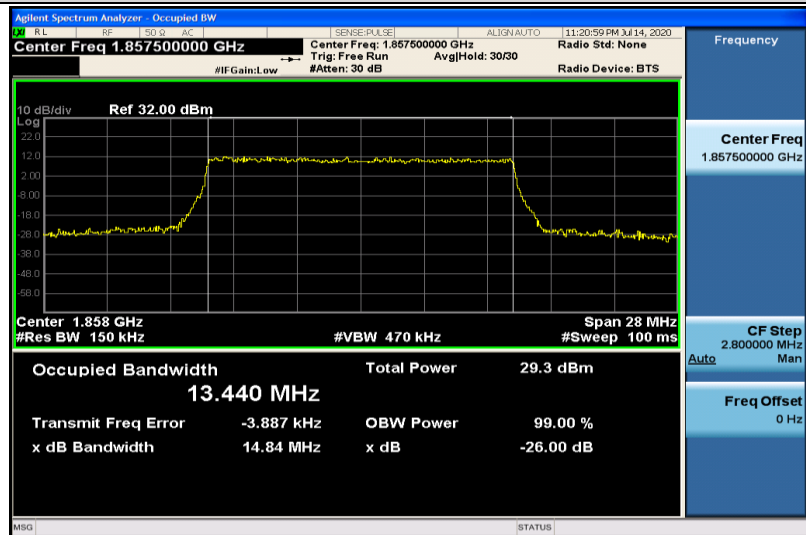
Band25-15MHz-16QAM-26115-75RB#0-13.440
