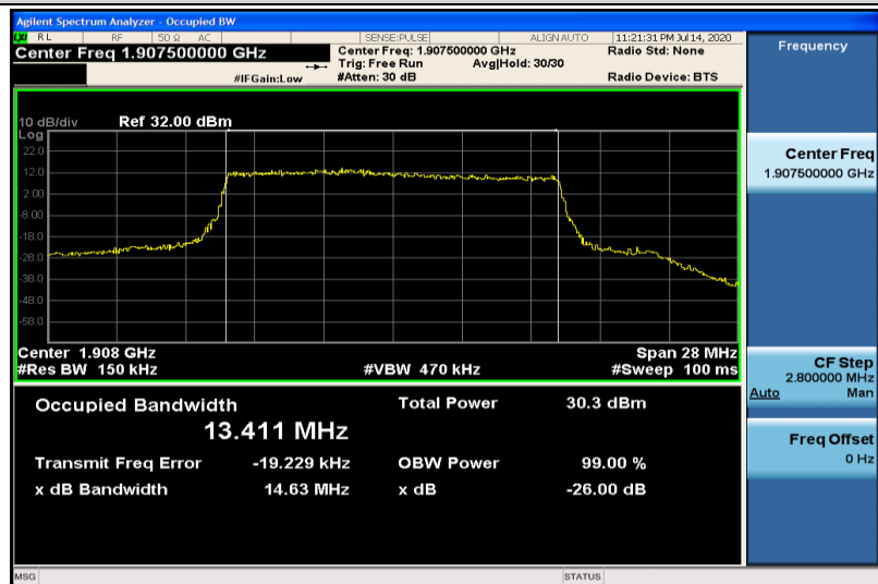
Band25-15MHz-QPSK-26615-75RB#0-13.411
