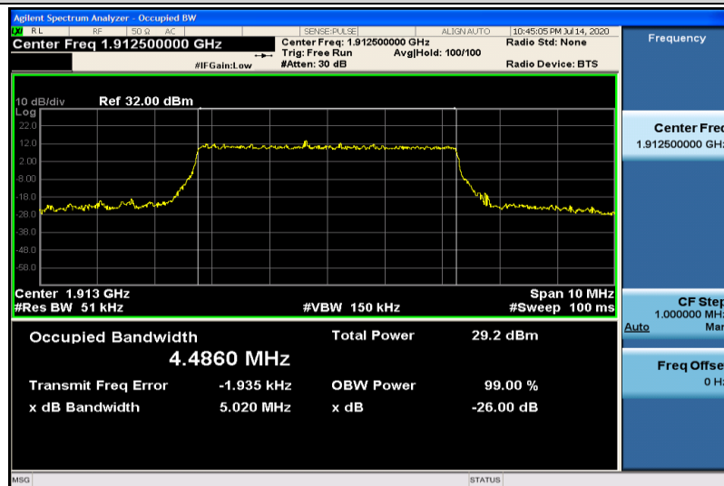
Band25-5MHz-16QAM-26665-25RB#0-4.4860
