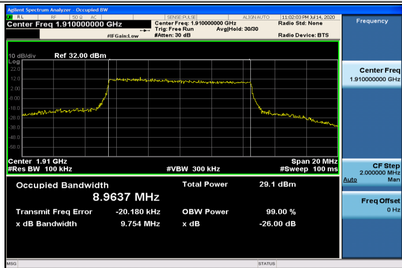
Band25-10MHz-16QAM-26640-50RB#0-8.9637
