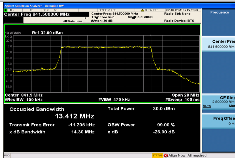
Band26-15MHz-16QAM-26965-75RB#0-13.412
