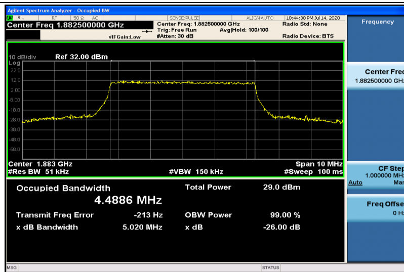
Band25-5MHz-16QAM-26365-25RB#0-4.4886
