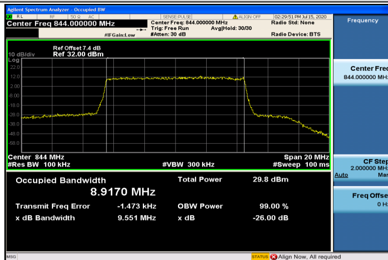
Band26-10MHz-16QAM-26990-50RB#0-8.9170
