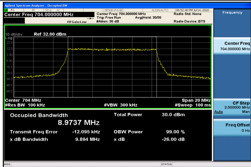
Band12-10MHz-16QAM-23060-50RB#0-8.9737
