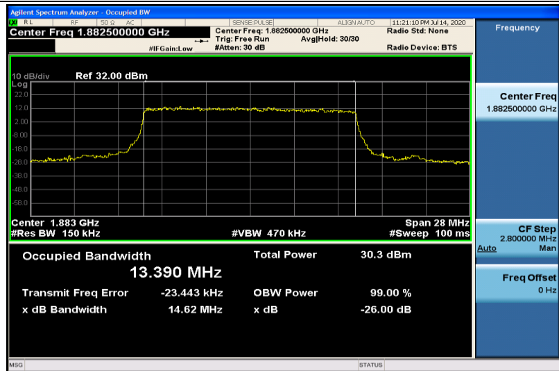
Band25-15MHz-QPSK-26365-75RB#0-13.390
