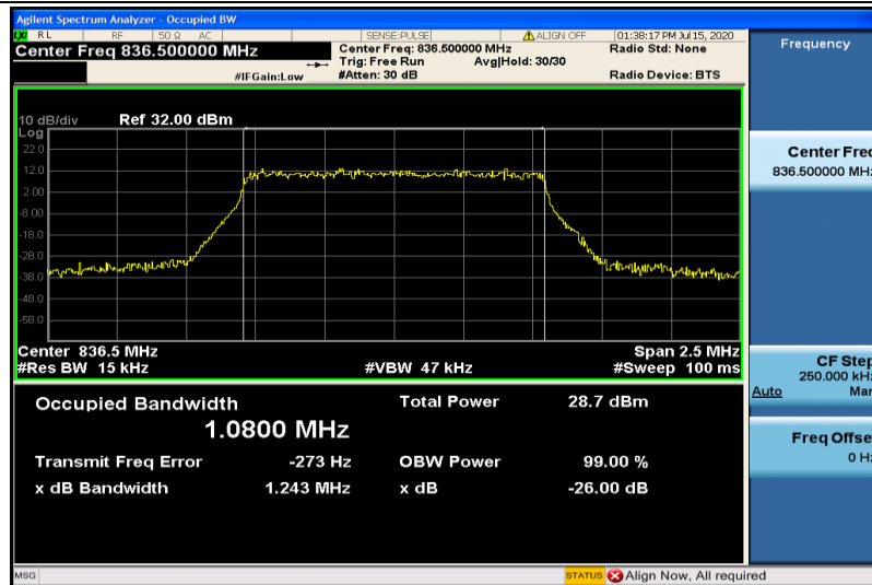
Band26-1.4MHz-16QAM-26915-6RB#0-1.0800
