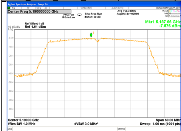
W52_11n40_Lower_Power Spectrum Density
