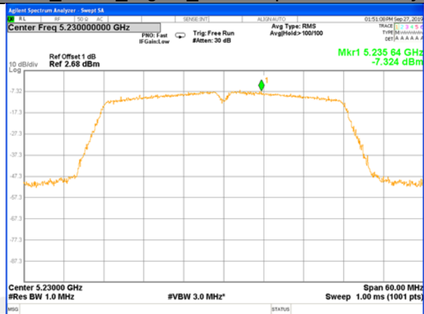
W52_11n40_Higher_Power Spectrum Density
