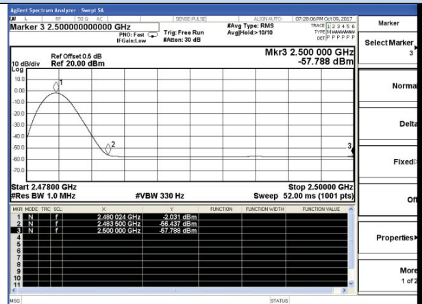
Channel 78 / 2480 MHz –Peak
