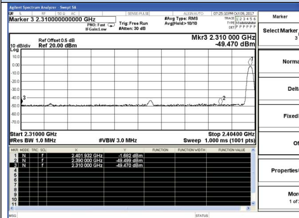
Channel 0 / 2402 MHz – Peak
