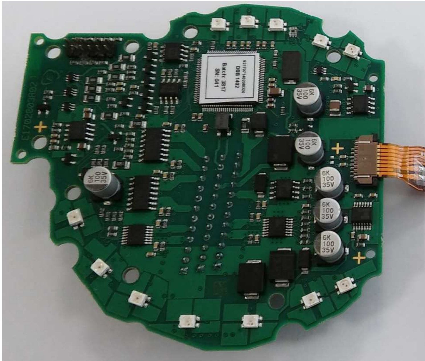
Dashboard (Internal PCB)
