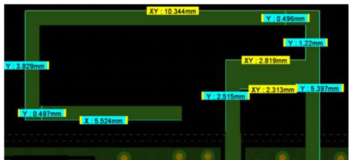
BT PCB ANTENNA DIMENSIONS:
