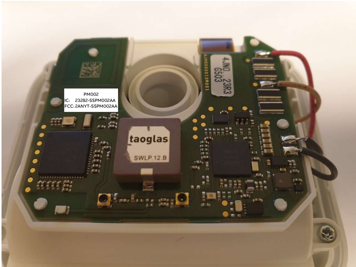
Figure 1 PM002 Processor module WirelessHART contained in "Smart Sensor HCHC. Transceiver for WirelessHART is mounted. Bluetooth transceiver connected to small chip antenna for short range communication, commissioning and local reading of sensor. Location and text for ISED / FCC is indicated with drawing. In production the label will be laser written into the surface of the module.
