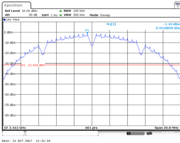
802.11b on channel 01
