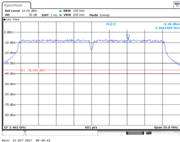
802.11g on channel 11
