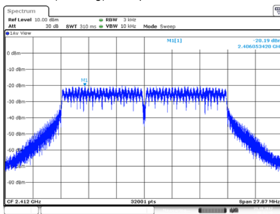
(802.11g) PSD plot on channel 1
