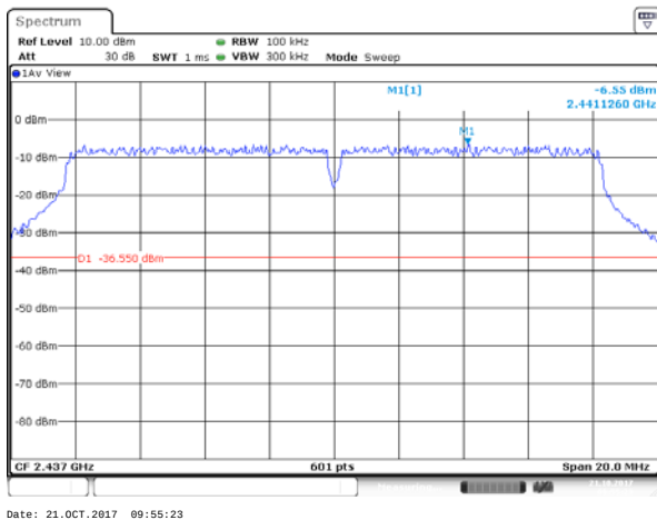
802.11g on channel 06
