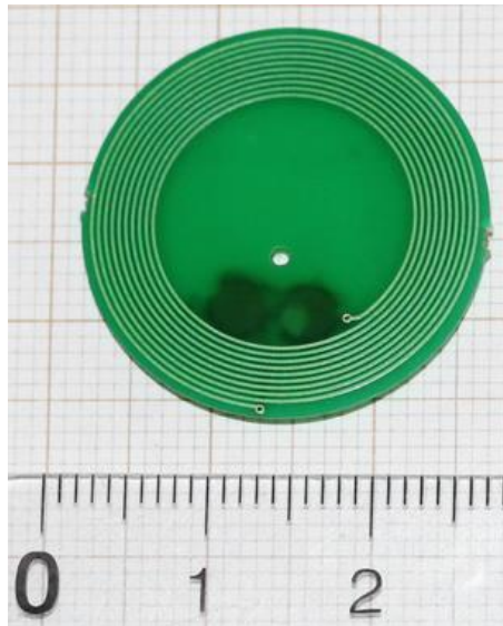
Antenna – RLS-1301-320:
