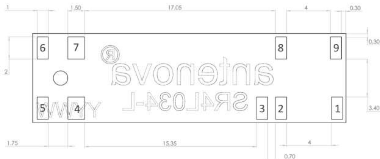
Bottom Side SR4L034-L
