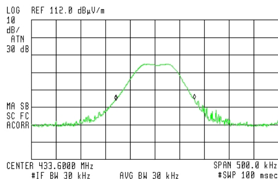
Figure 23. 20dB Bandwidth Results
