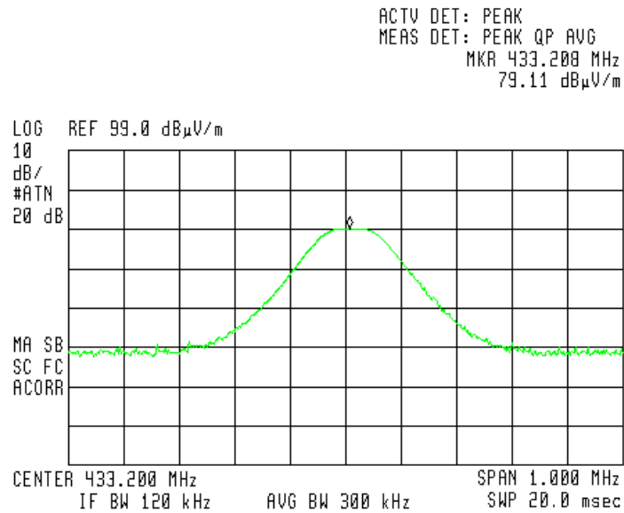
Figure 13. Field Strength of Fundamental - Vertical
