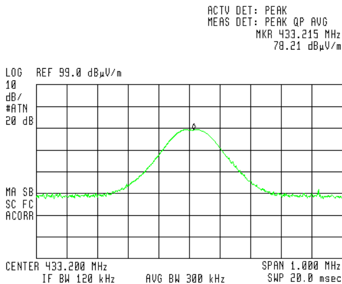
Figure 14. Field Strength of Fundamental -Horizontal
