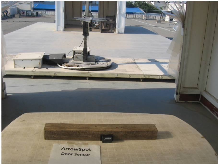
Radiated Emission Test 200-1000.0MHz
