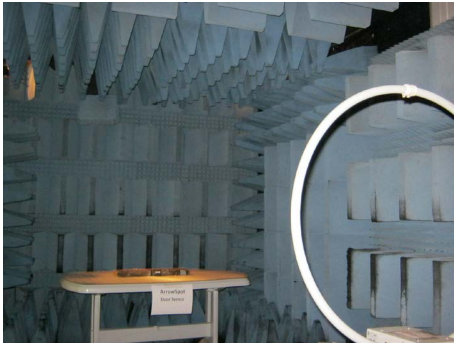
Radiated Emission Test 0.009-30.0MHz
