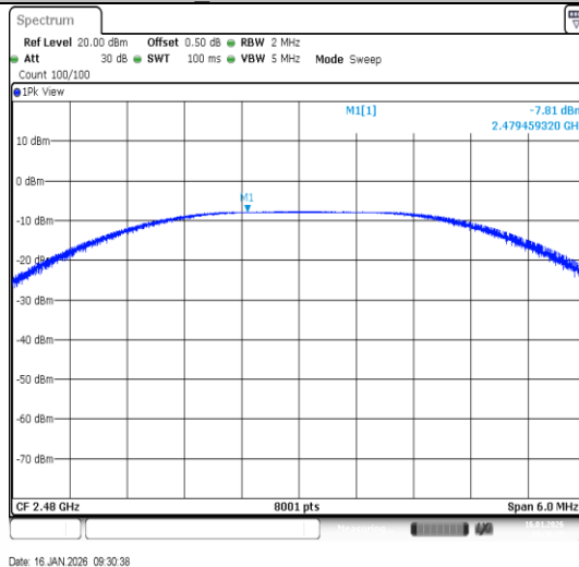
BLE_1M-Ant1-2480-PASS
