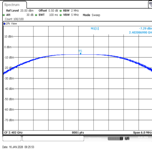
BLE_1M-Ant1-2402-PASS
