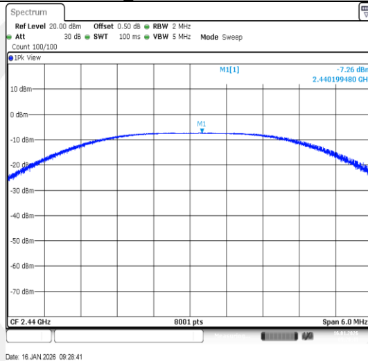
BLE_1M-Ant1-2440-PASS
