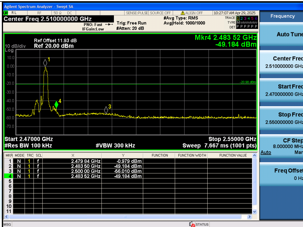
3DH5-Ant1-2480-PASS
