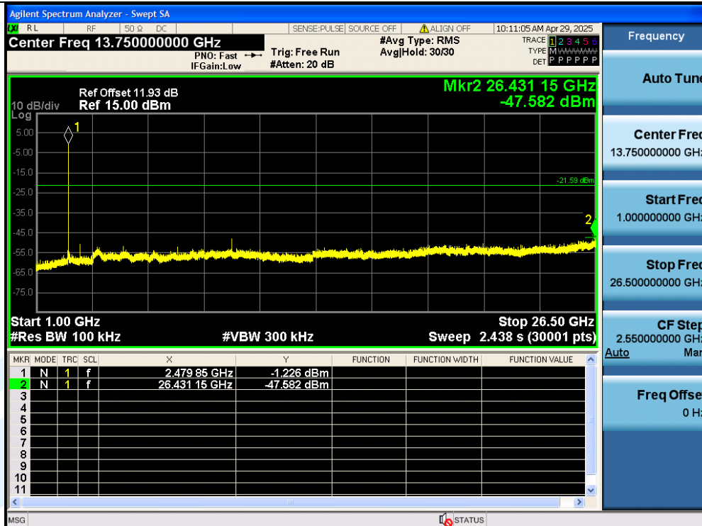
DH5-Ant1-2480-1000~26500-PASS
