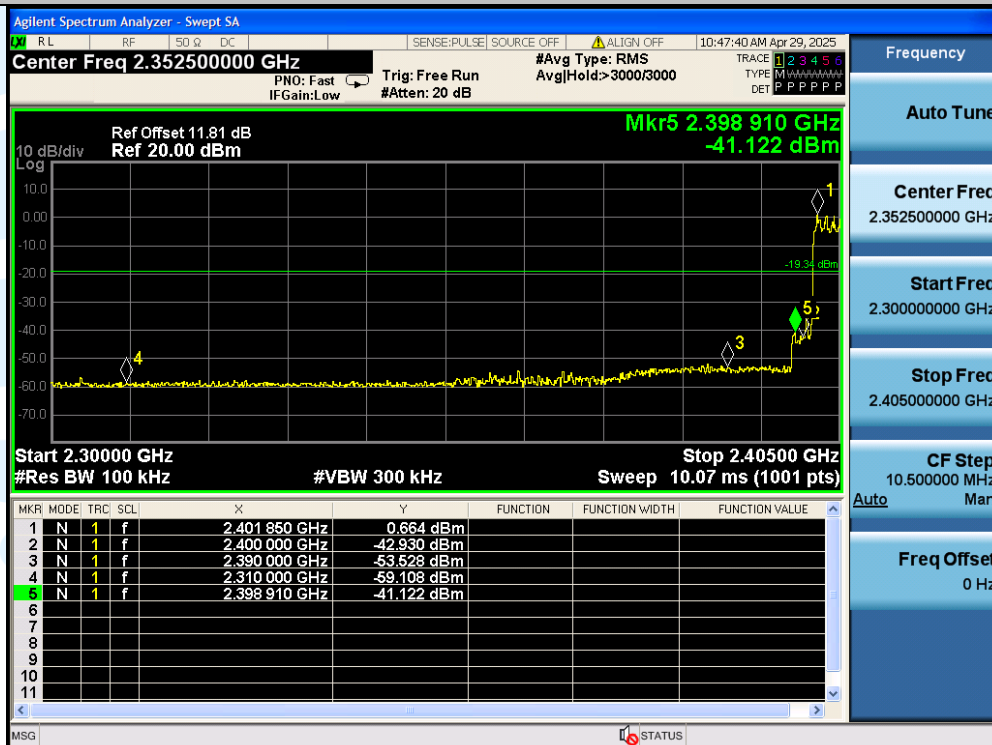
2DH5-Ant1-Hop_2402-PASS
