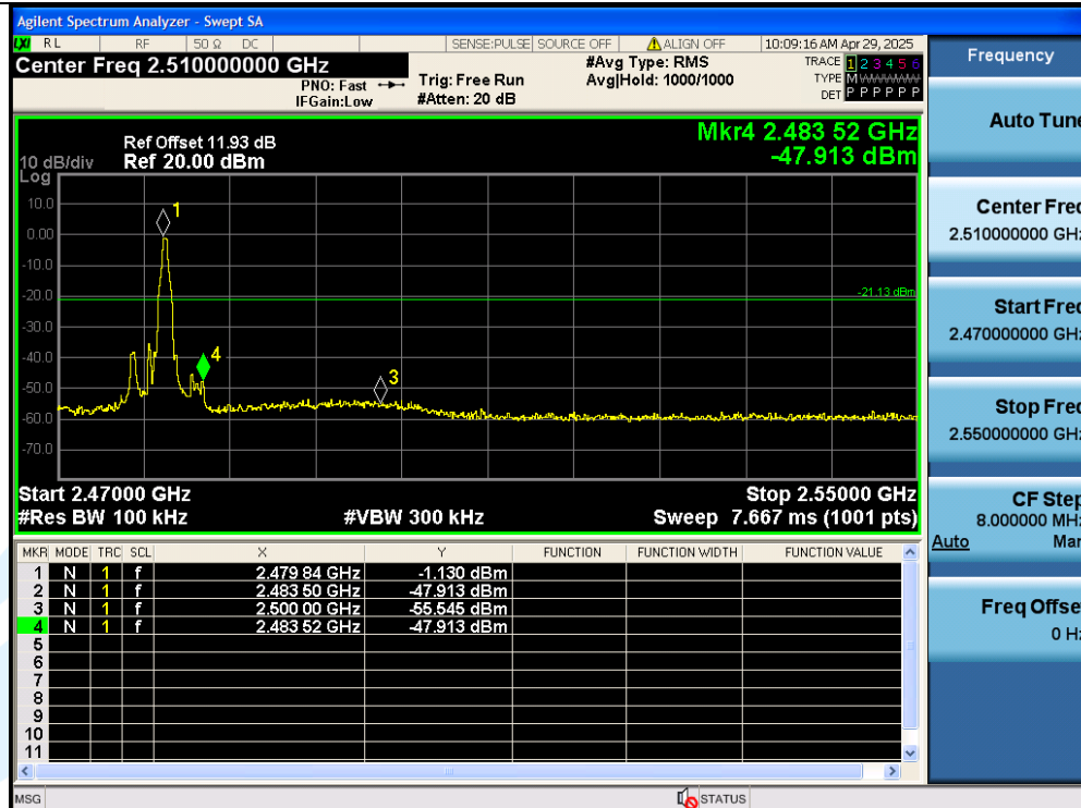
DH5-Ant1-2480-PASS
