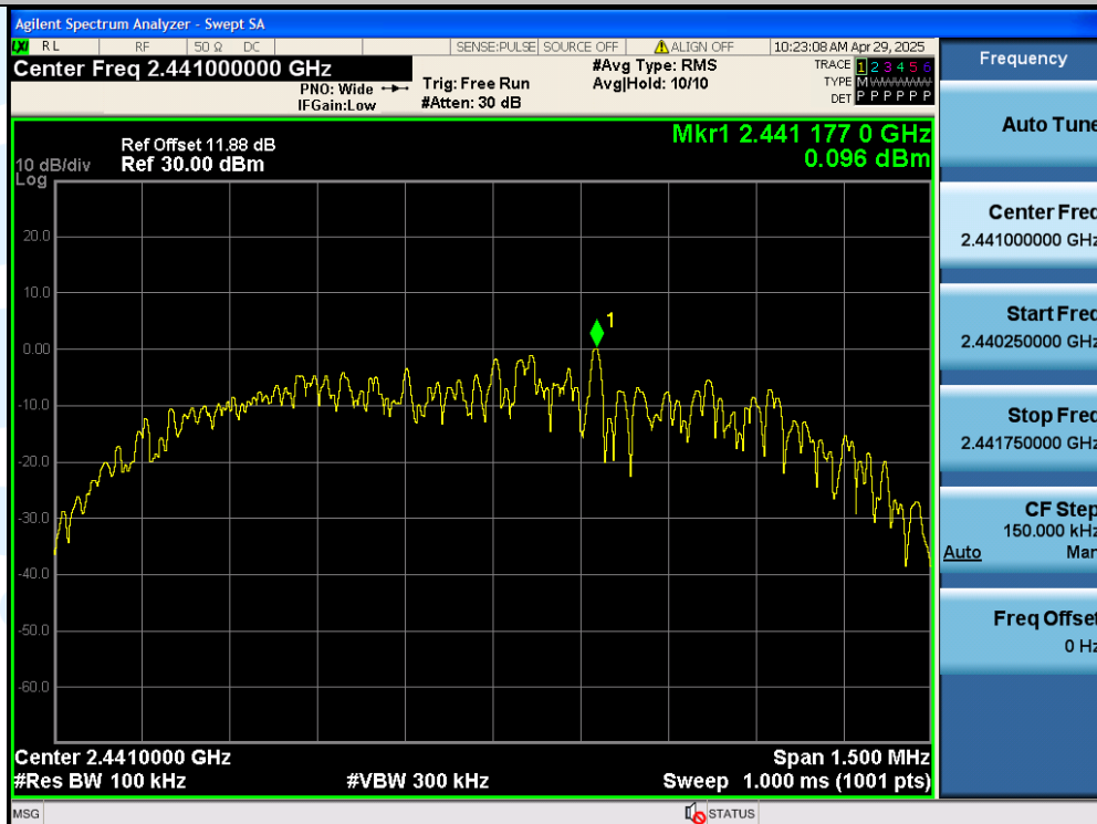
3DH5-Ant1-2441-0~Reference-PASS
