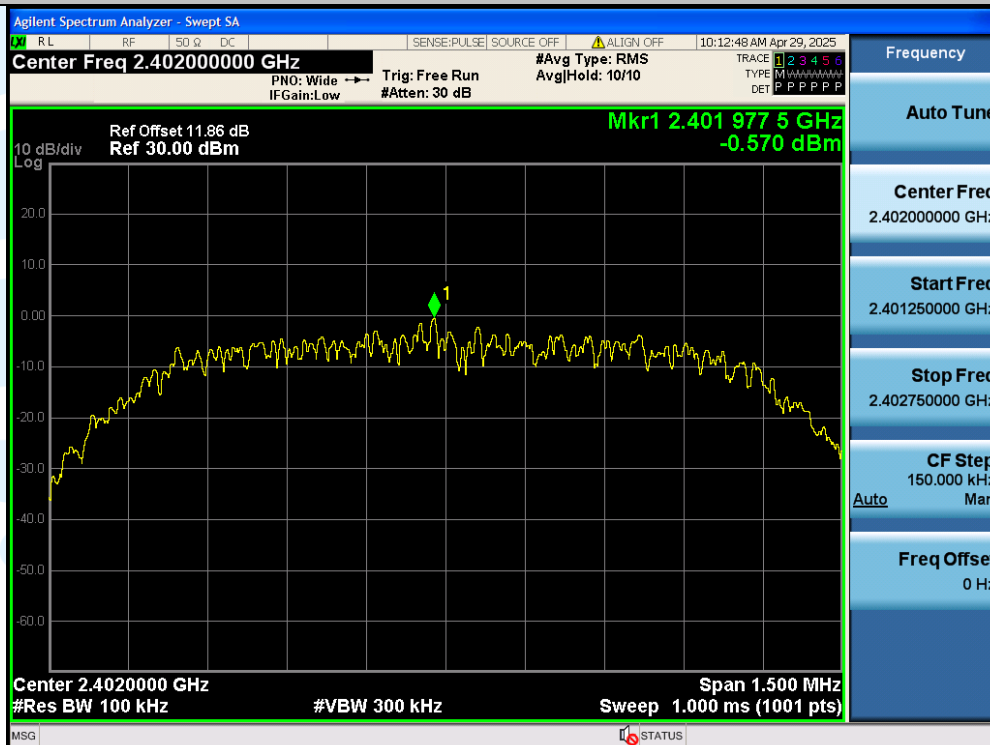
2DH5-Ant1-2402-0~Reference-PASS
