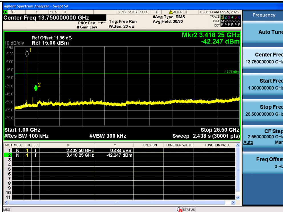
DH5-Ant1-2402-1000~26500-PASS
