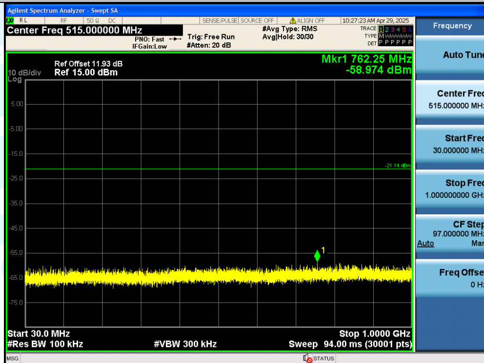
3DH5-Ant1-2480-30~1000-PASS
