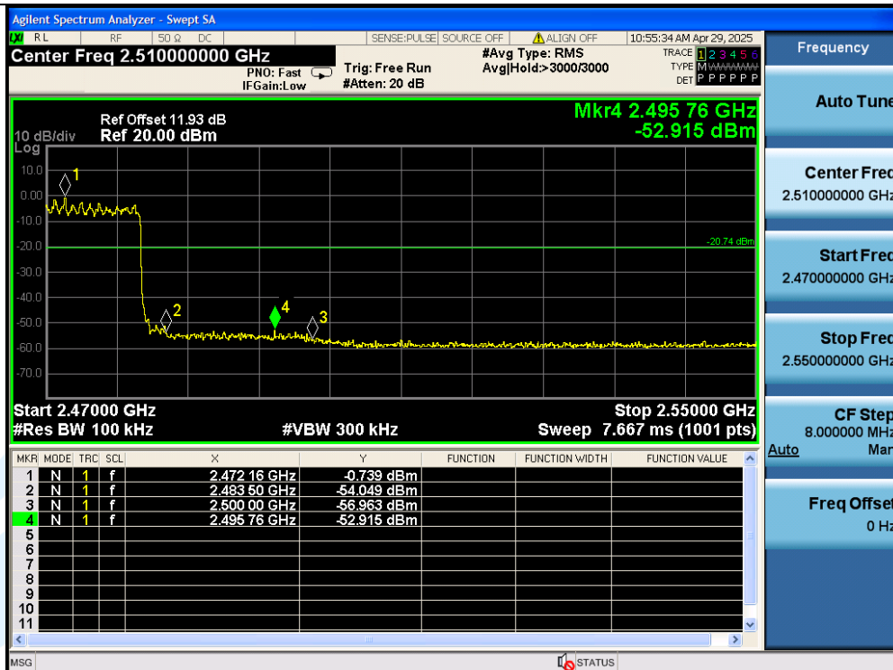
2DH5-Ant1-Hop_2480-PASS
