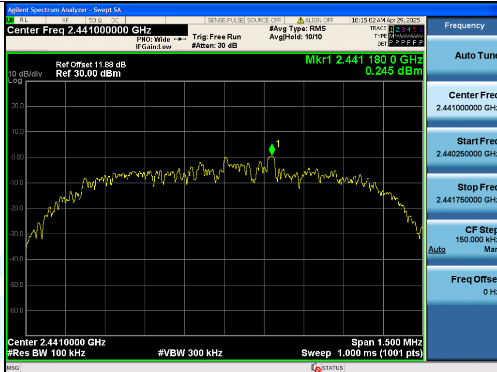
2DH5-Ant1-2441-0~Reference-PASS
