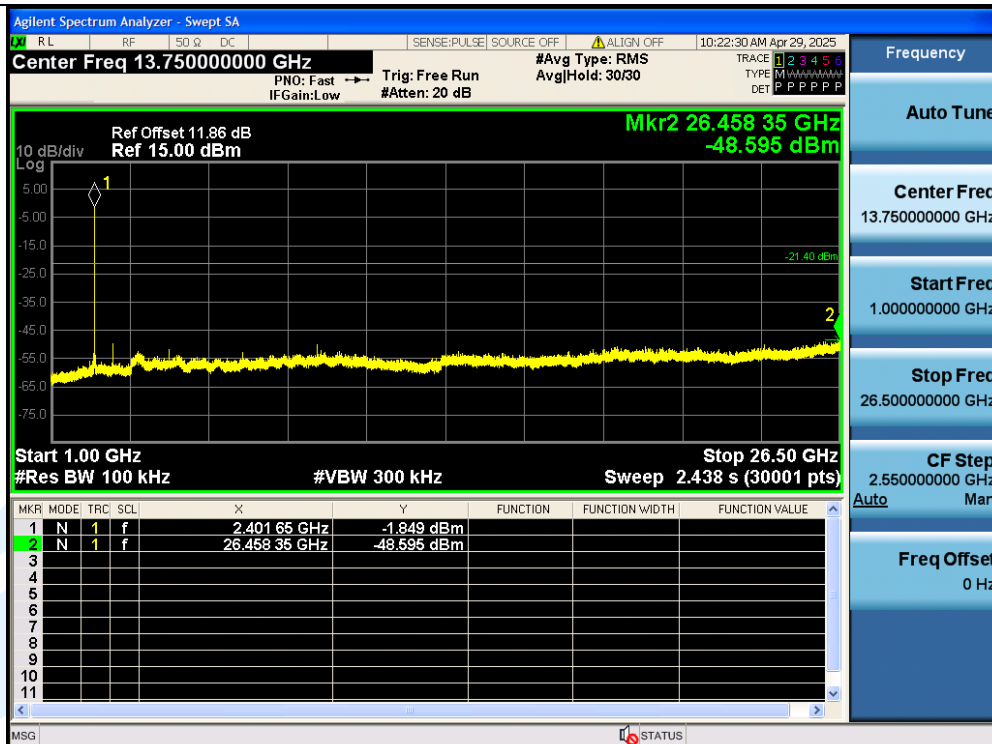
3DH5-Ant1-2402-1000~26500-PASS
