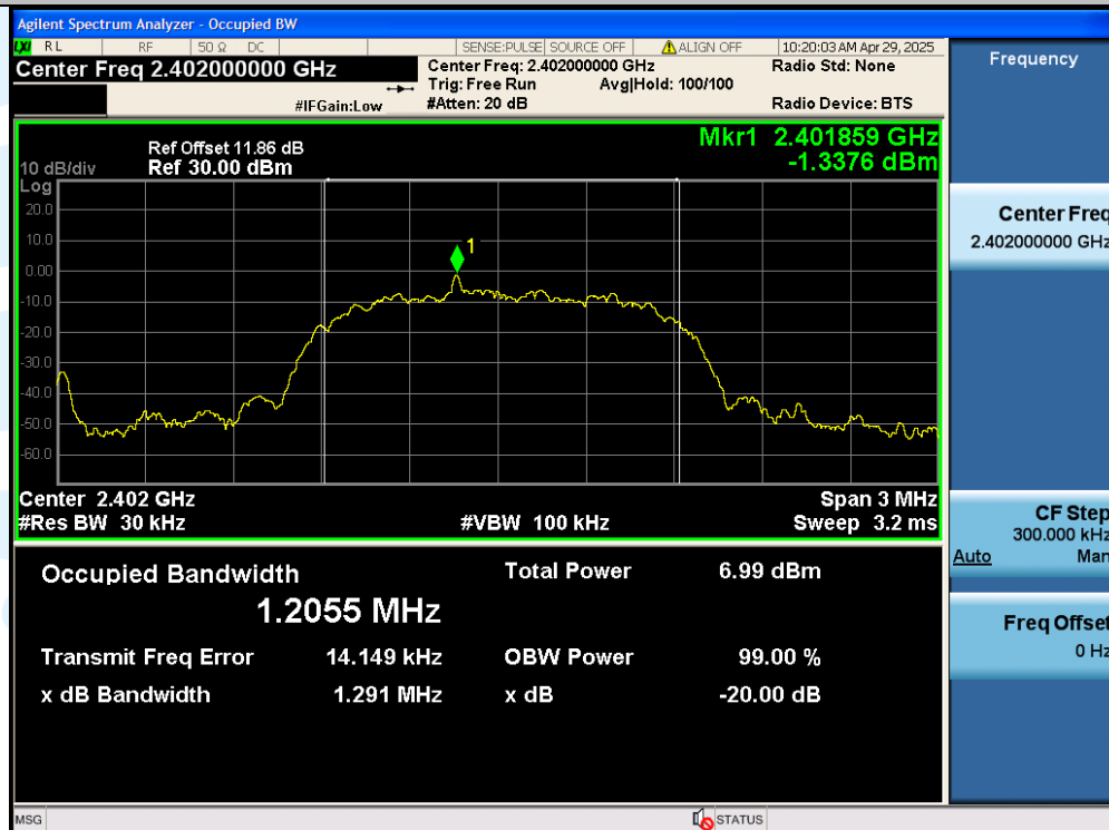
3DH5-Ant1-2402
