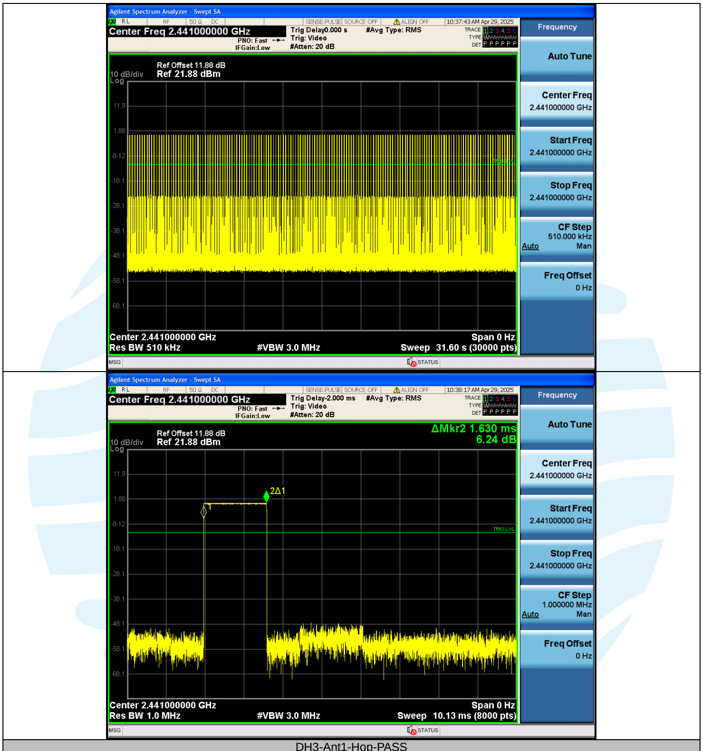
DH3-Ant1-Hop-PASS
