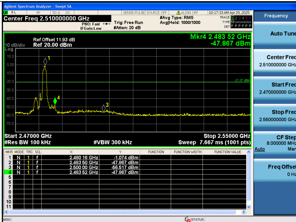
2DH5-Ant1-2480-PASS
