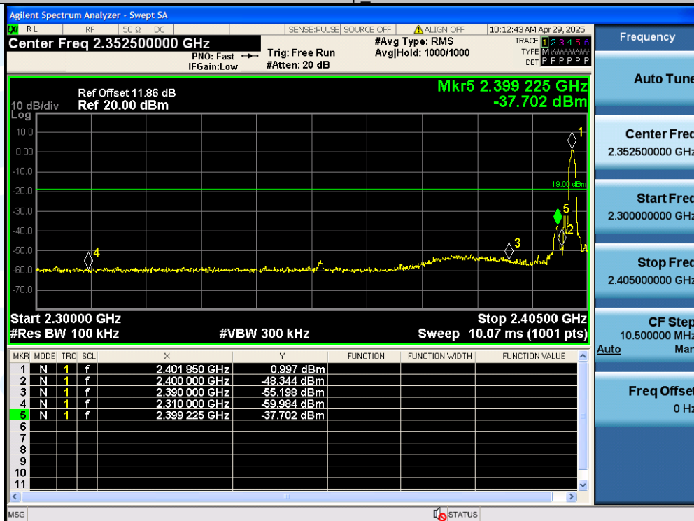
2DH5-Ant1-2402-PASS
