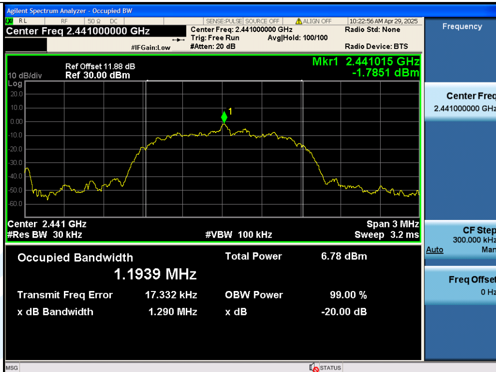
3DH5-Ant1-2441
