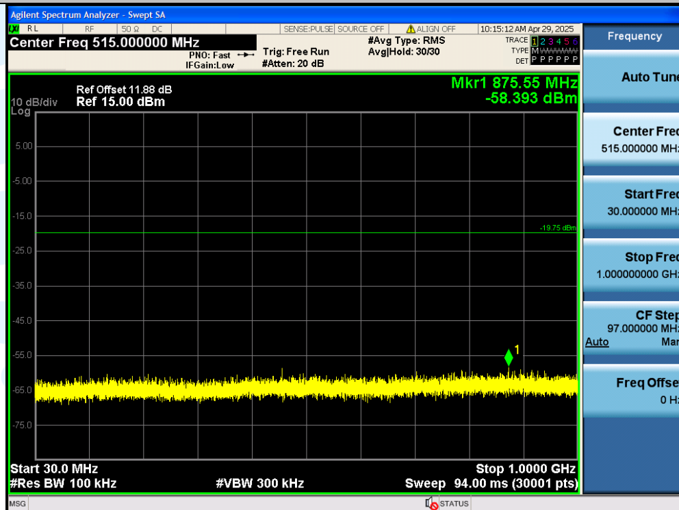
2DH5-Ant1-2441-30~1000-PASS
