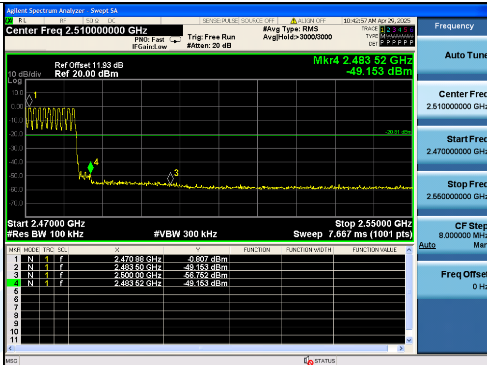
DH5-Ant1-Hop 2480-PASS
