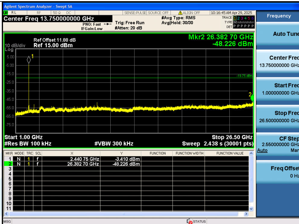
2DH5-Ant1-2441-1000~26500-PASS
