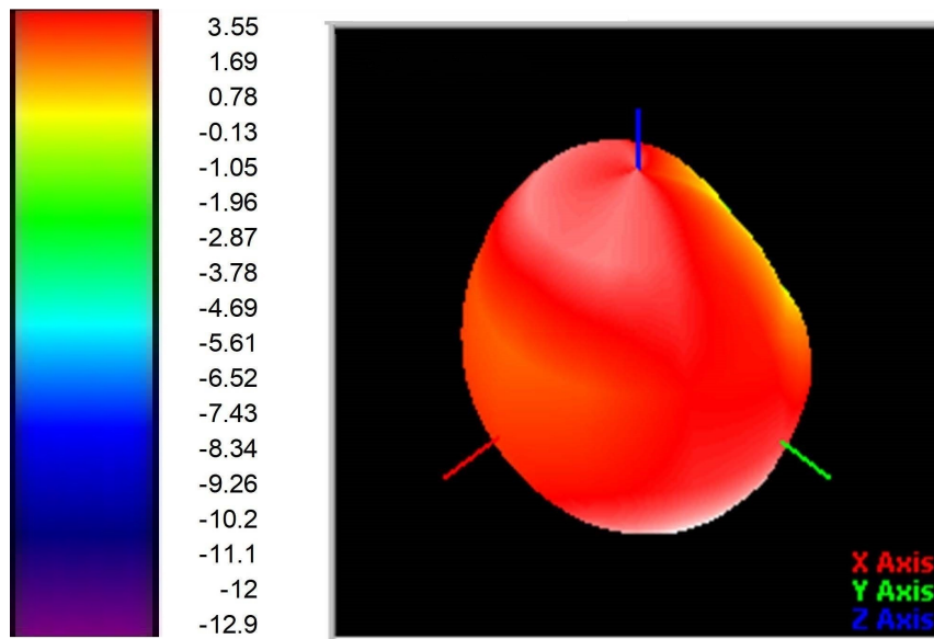
3D Radiation Patterns @2450MHz (Unit:dBi)
