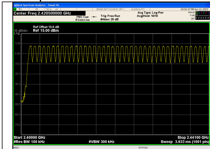
Low End Spectrum Channel Hopping Plot GFSK
