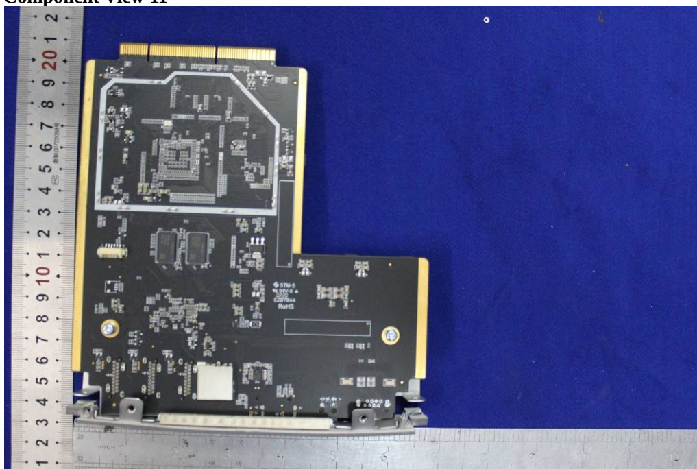
Solder Board-Component View 11
