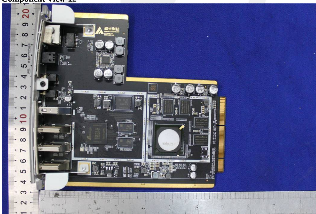
Solder Board-Component View 12
