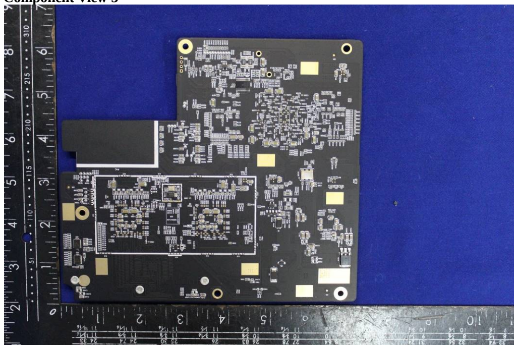
Solder Board-Component View 3
