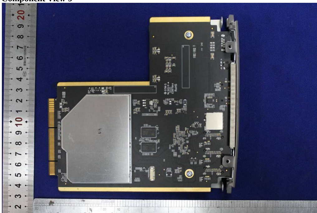
Solder Board-Component View 9
