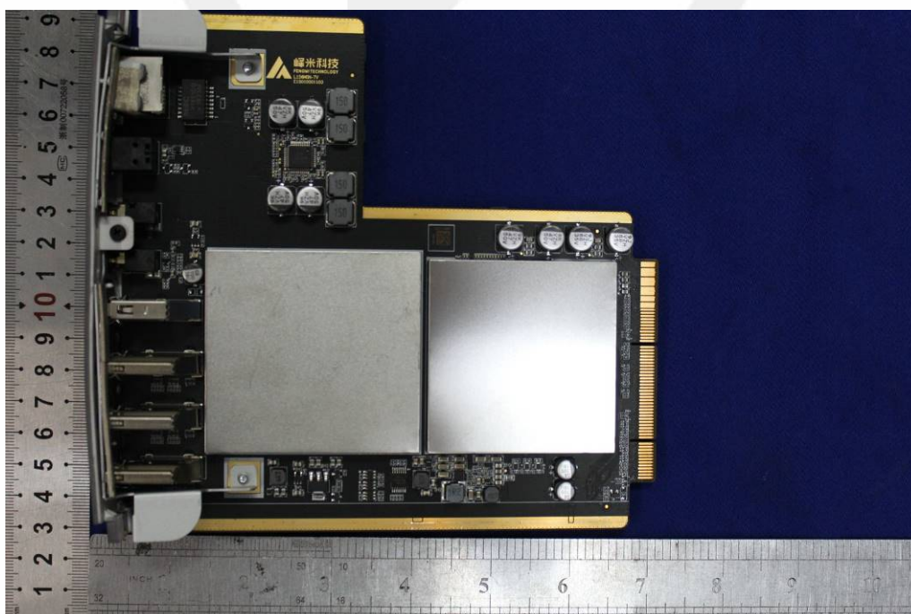
Solder Board-Component View 10
