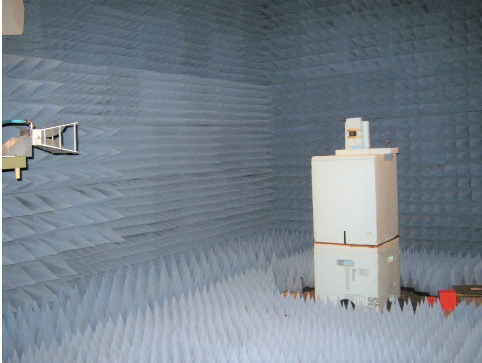
Radiated Emissions above 1 GHz – back
