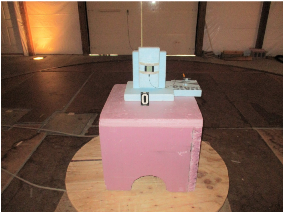
Radiated Emissions below 1 GHz – Position 1
