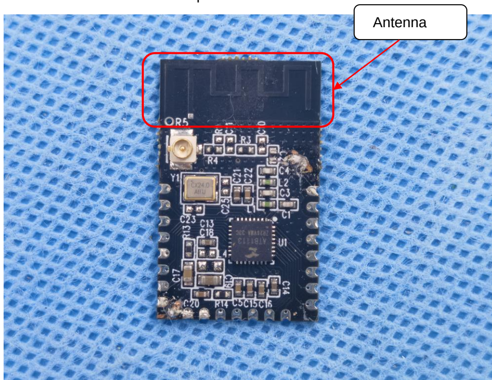
Internal view-1 of EUT
