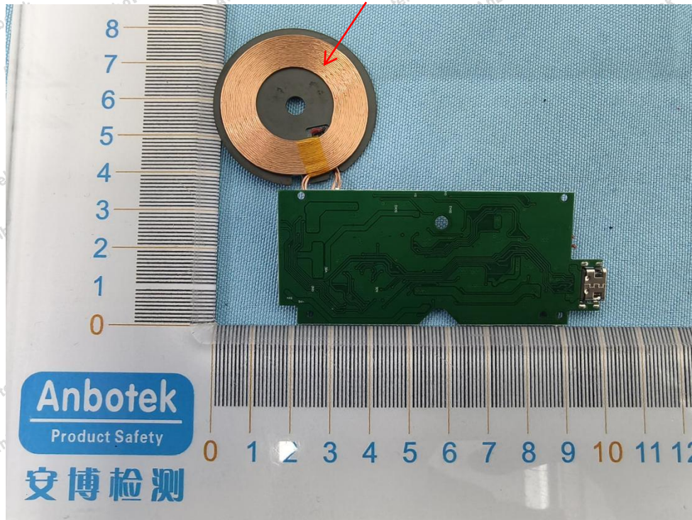
TWS-ANT
