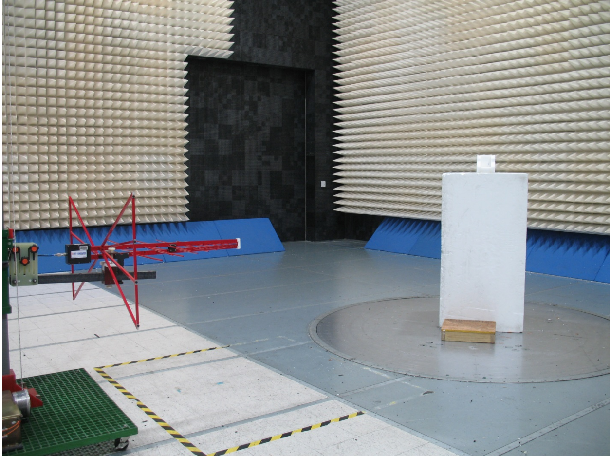
Radiated Emissions 30MHz-1GHz (Transmitting)
