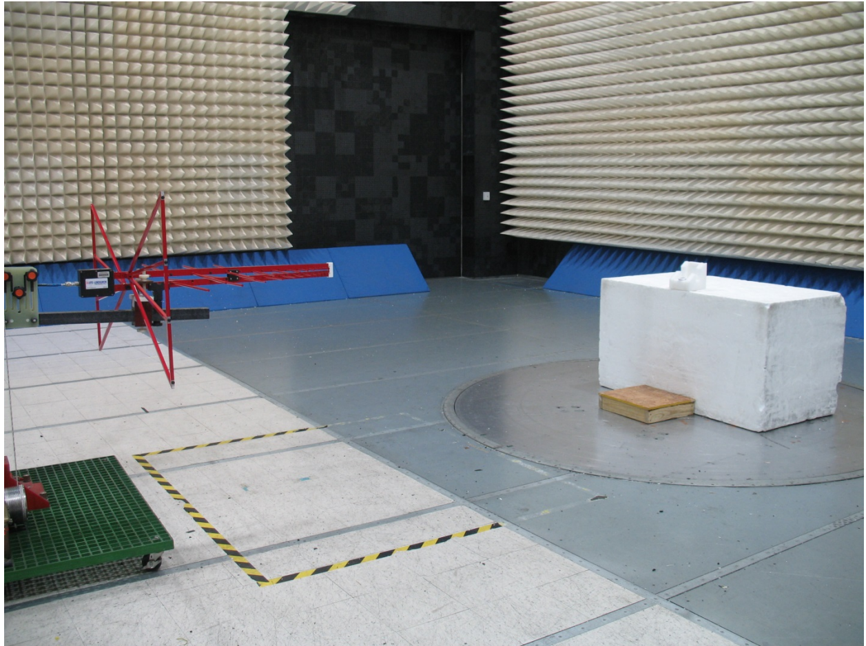
Radiated Emissions 30MHz-1GHz (Idle)
