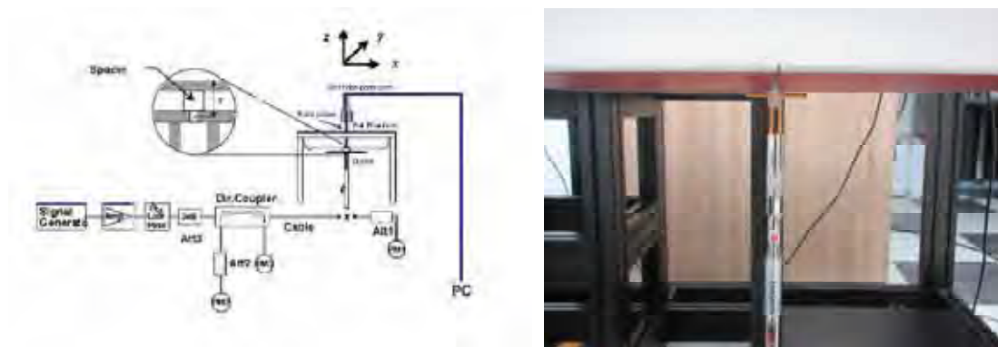
Figure 9-1 System Verification Setup Diagram and Photo
