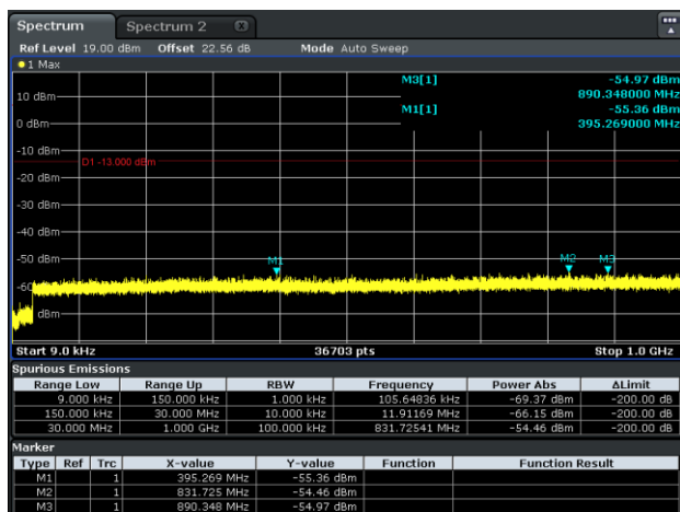
Figure 8.2-1: Conducted spurious emissions 9KHz to 1GHz, 2112.5MHz, 16QAM, 5MHz BW.
