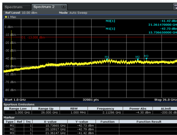
Figure 8.2-2: Conducted spurious emissions 1GHz to 26GHz, 2112.5MHz, 16QAM, 5MHz BW.
