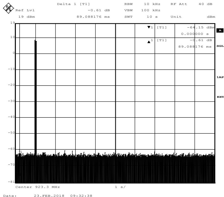
Screen shot: Number of transmission bursts in 10 s measurement period
