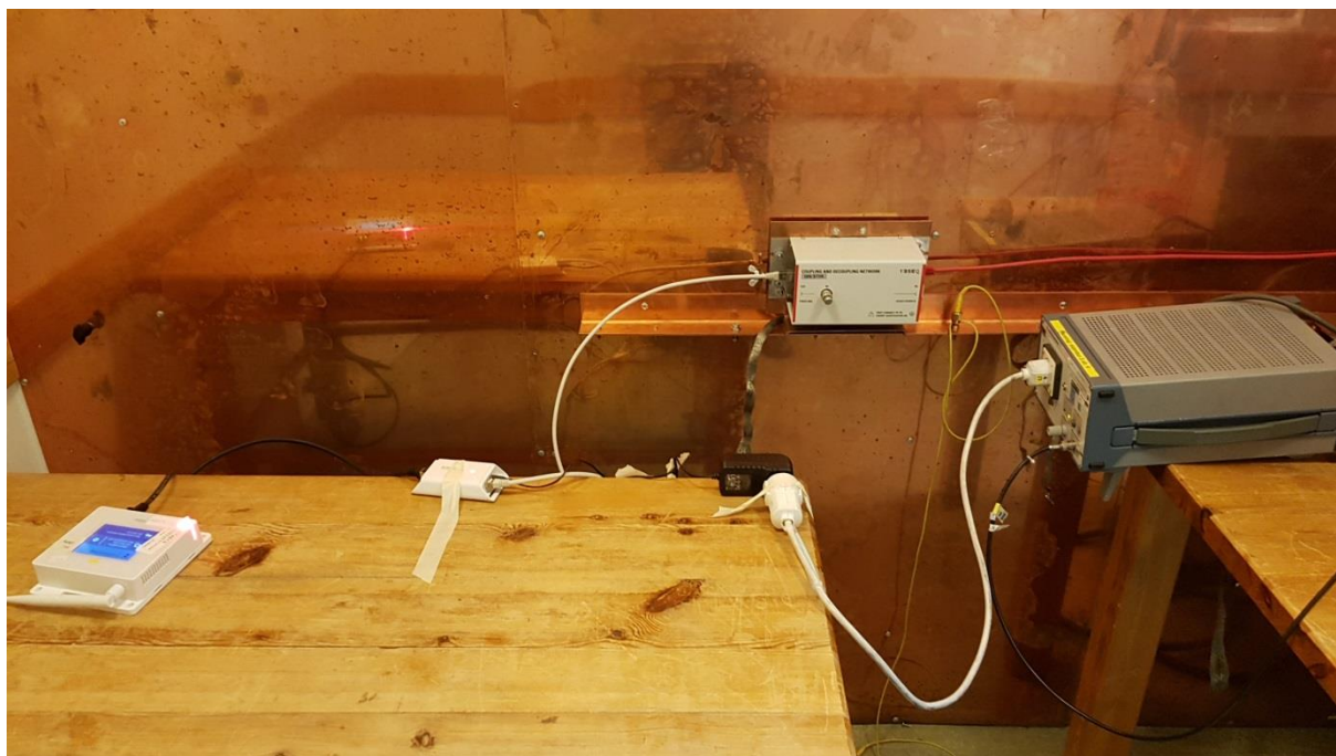
Photo of the test set-up for conducted emission with PoE injector
