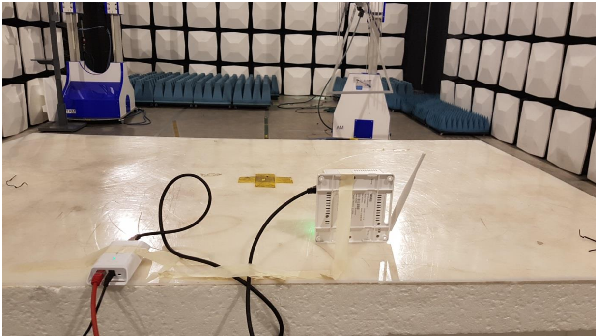
Photo of the test set-up for radiated emission 30 MHz – 1 GHz with PoE injector
