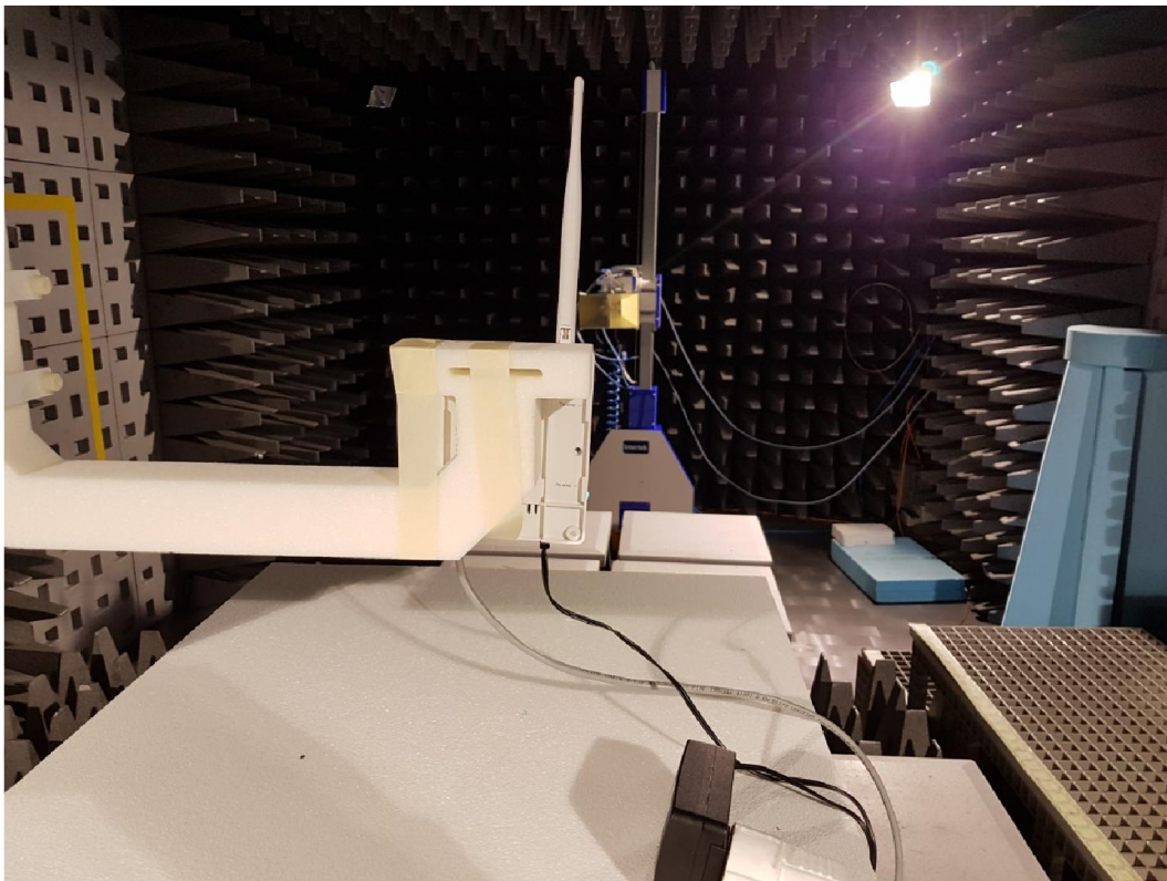
Test set up radiated emission 1GHz – 10 GHz
